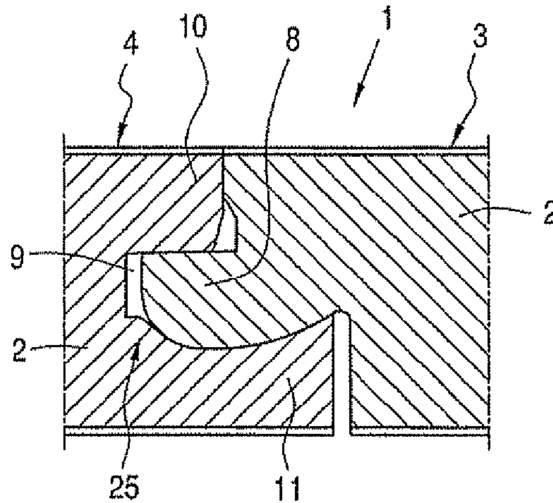
FIG. 5 PRIOR ART
