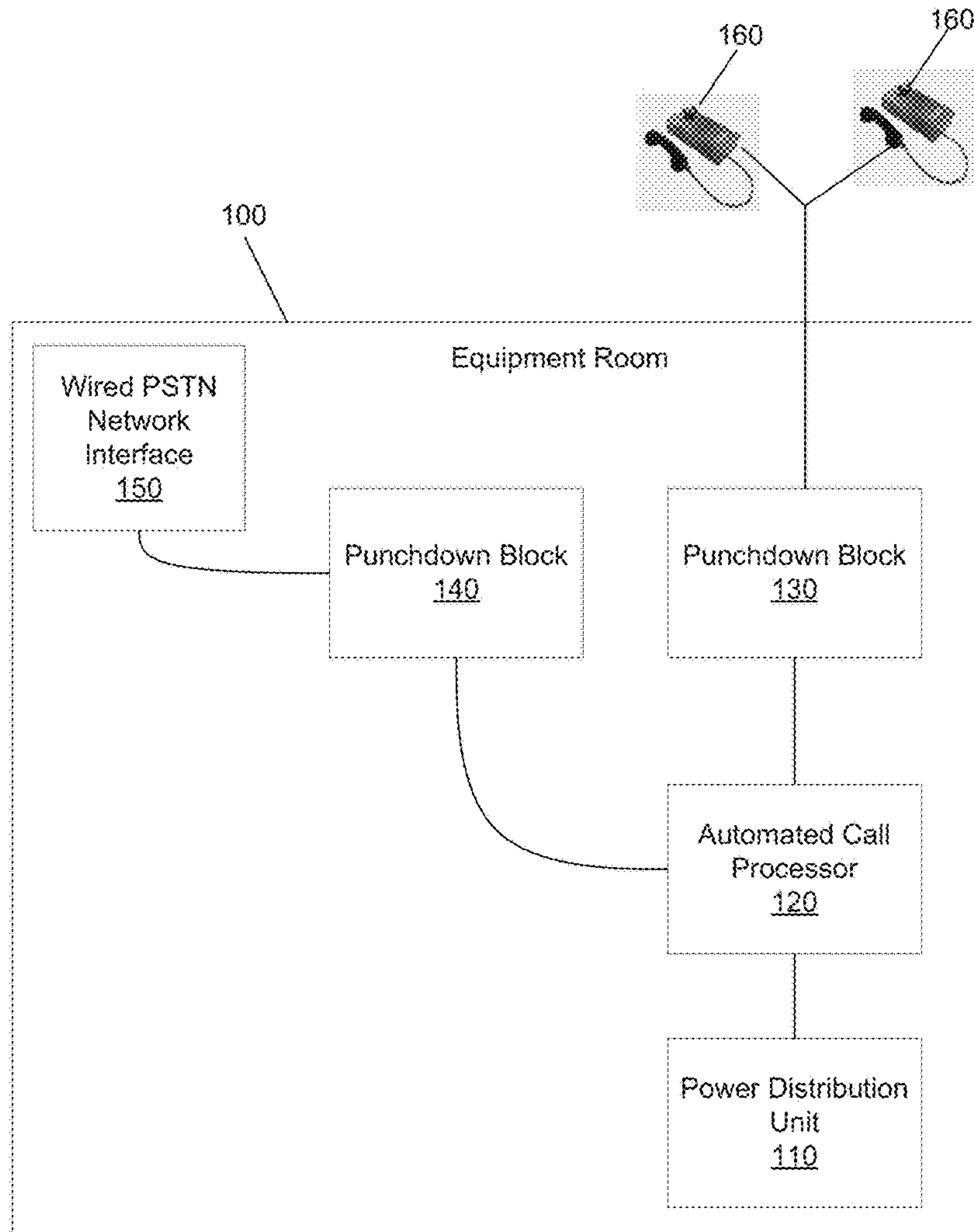
Figure 1 (Prior Art)
