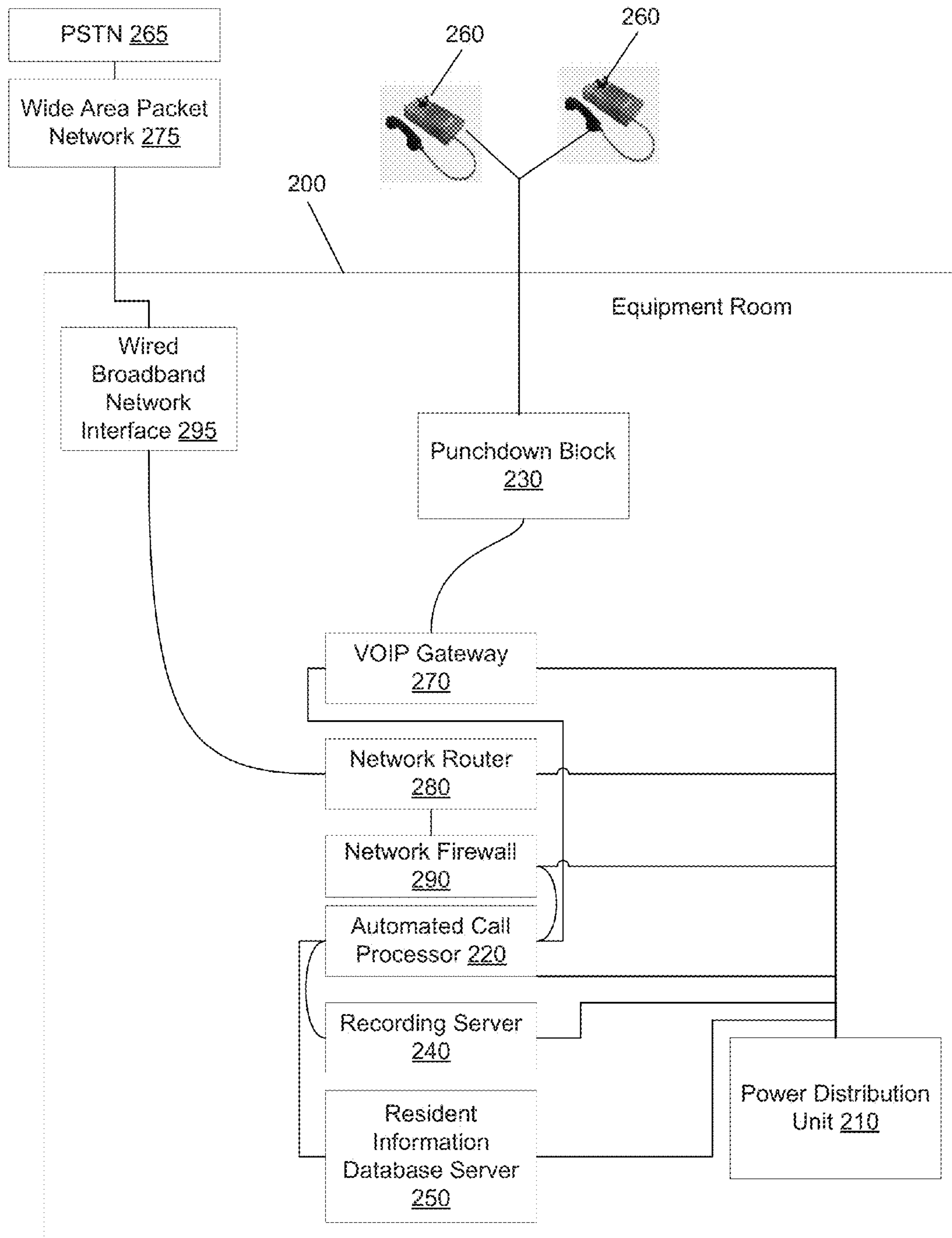
Figure 2 (Prior Art)
