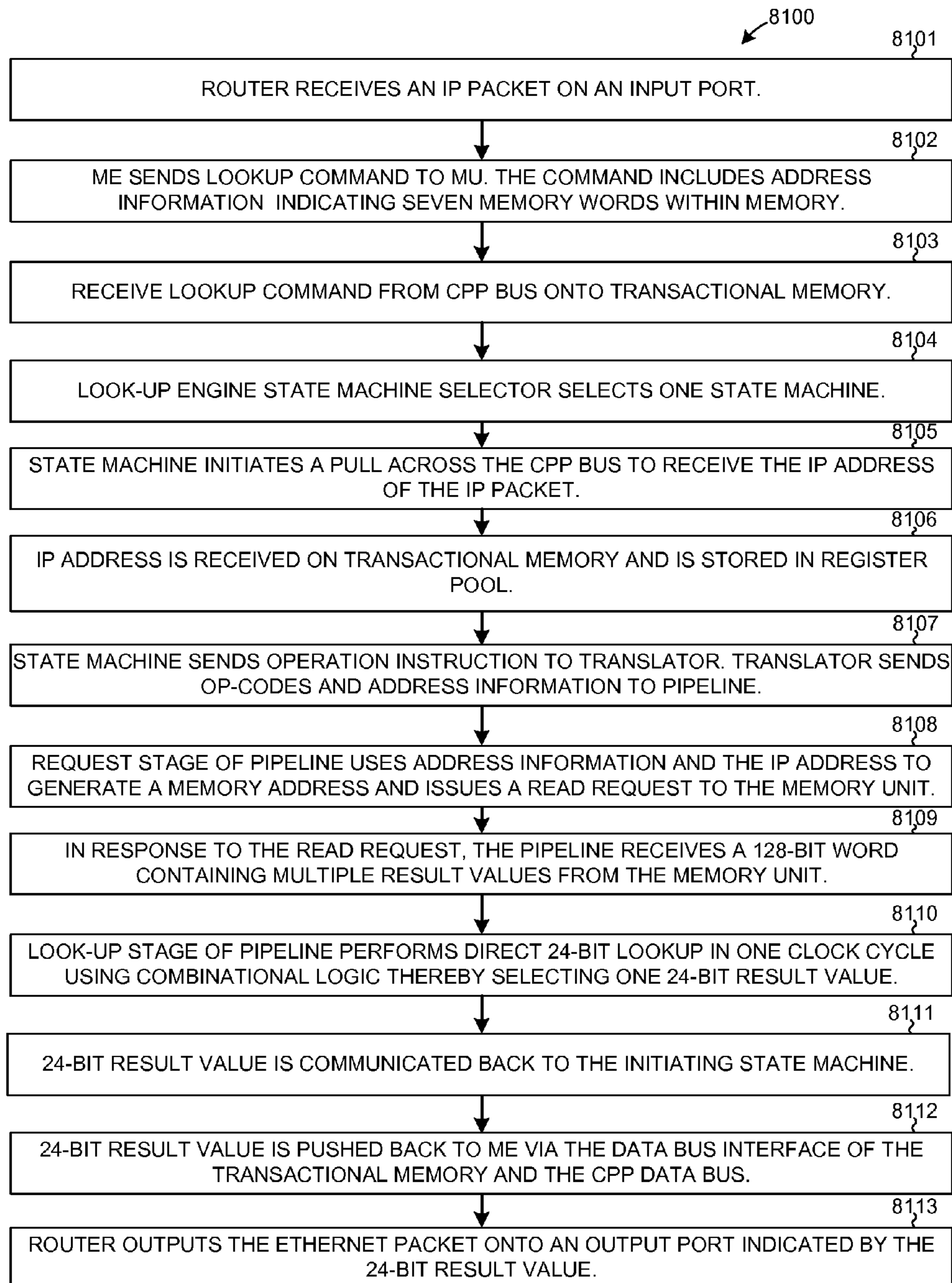
DIRECT 24-BIT LOOK-UP FLOWCHART FIG. 50
