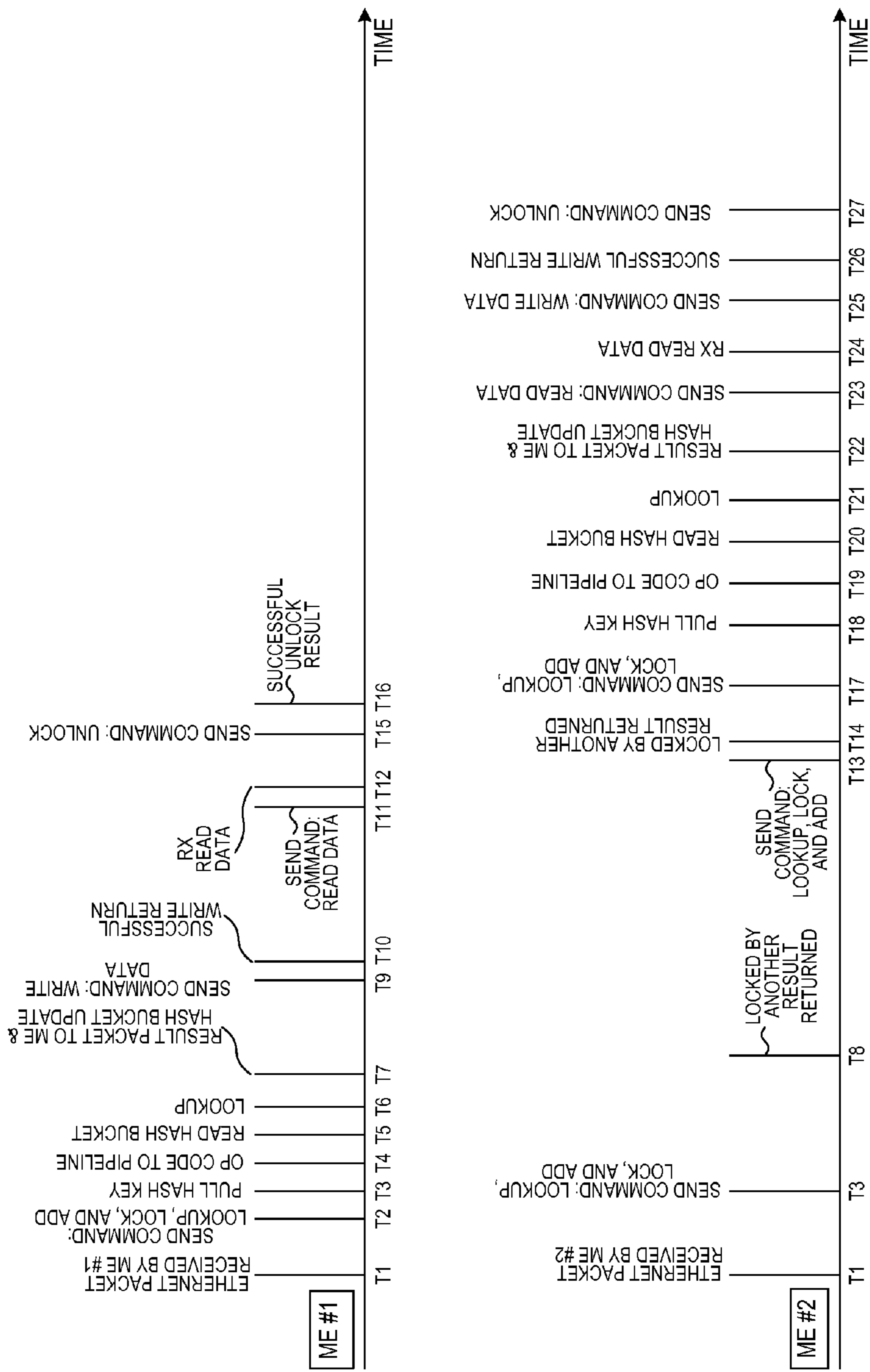
LOOKUP, LOCK, AND ADD TIMING DIAGRAM FIG. 14
