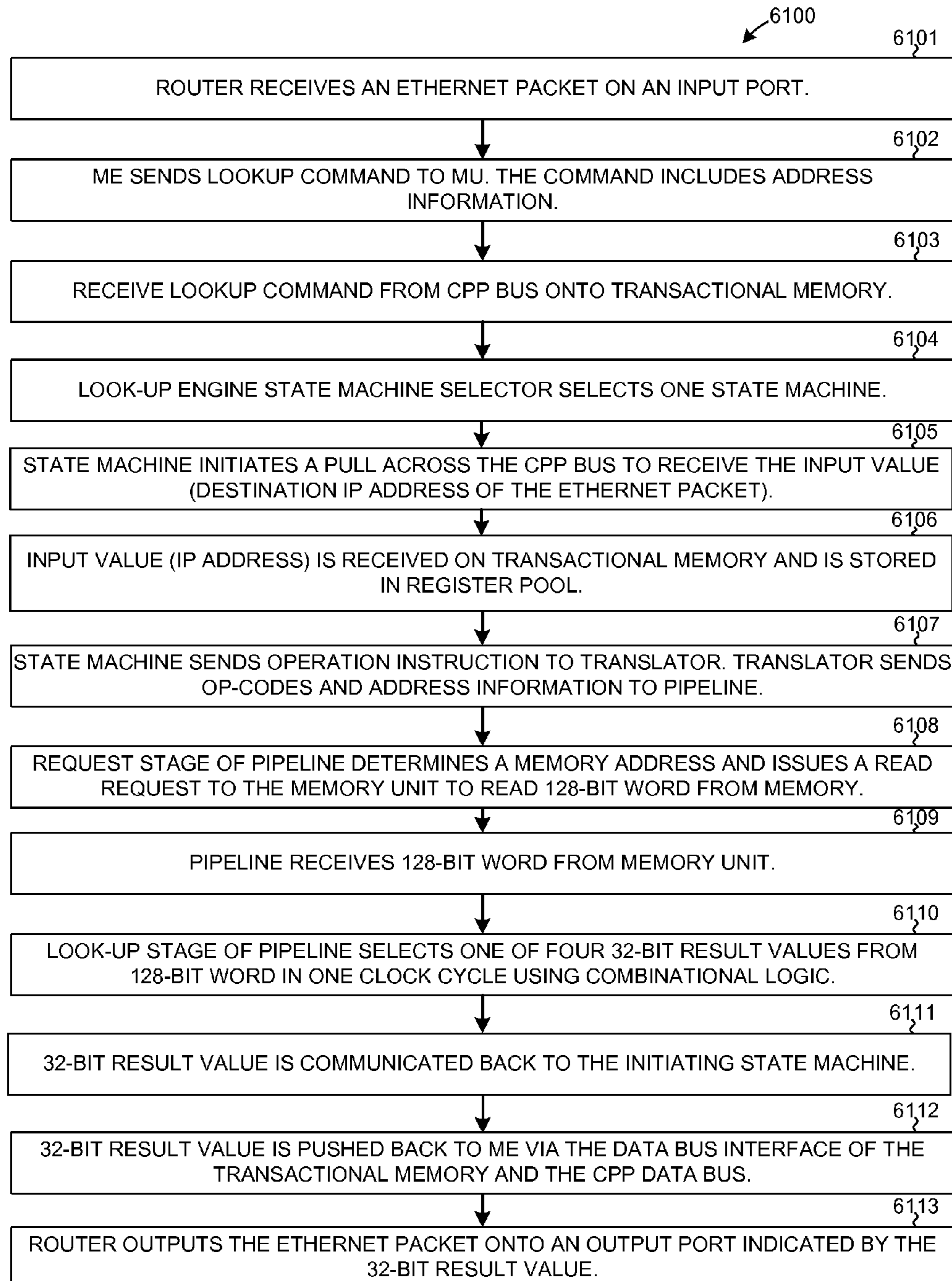
DIRECT 32-BIT LOOKUP FLOWCHART FIG. 44
