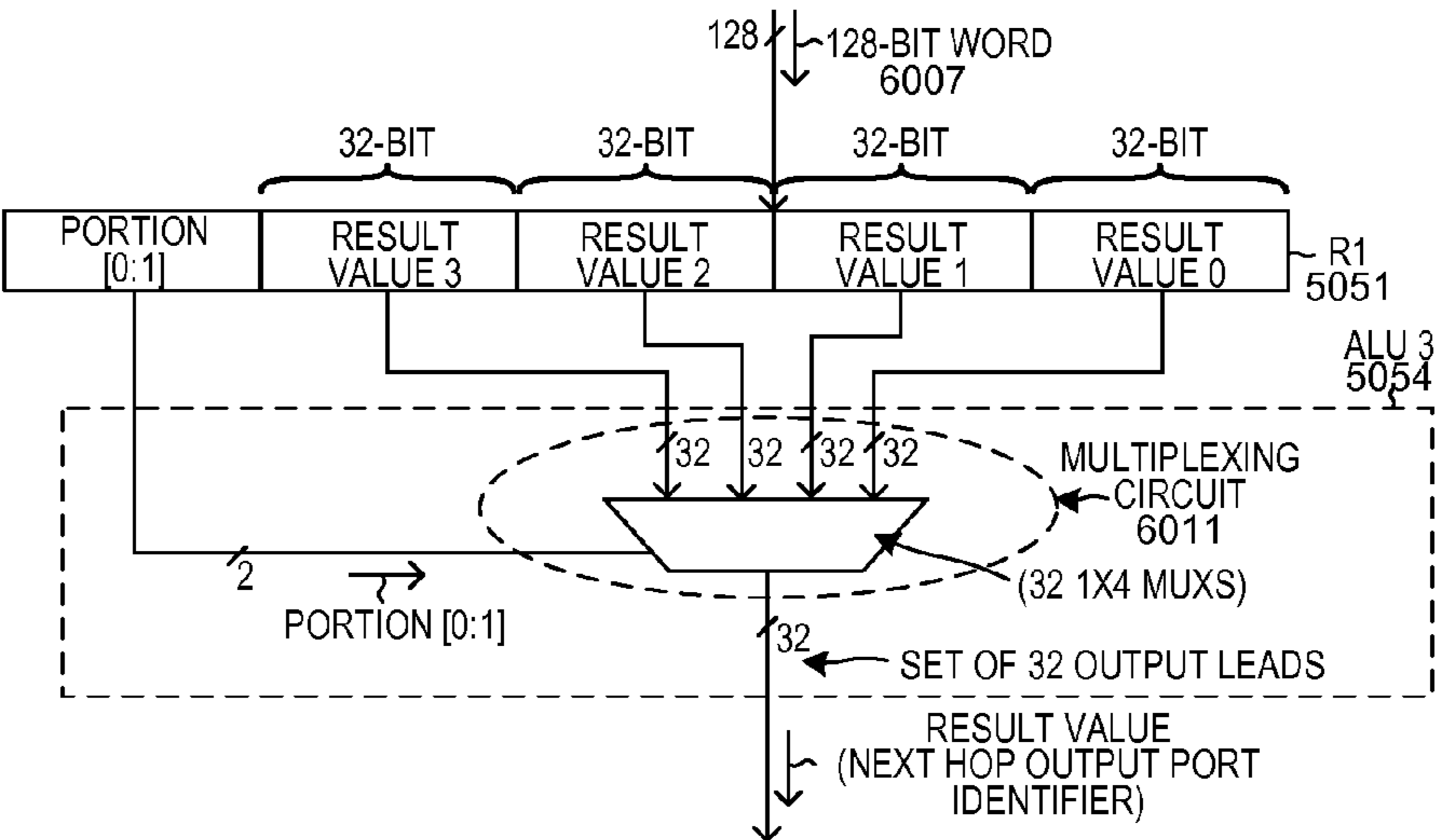
DIRECT 32-BIT LOOKUP STAGE FIG. 42
