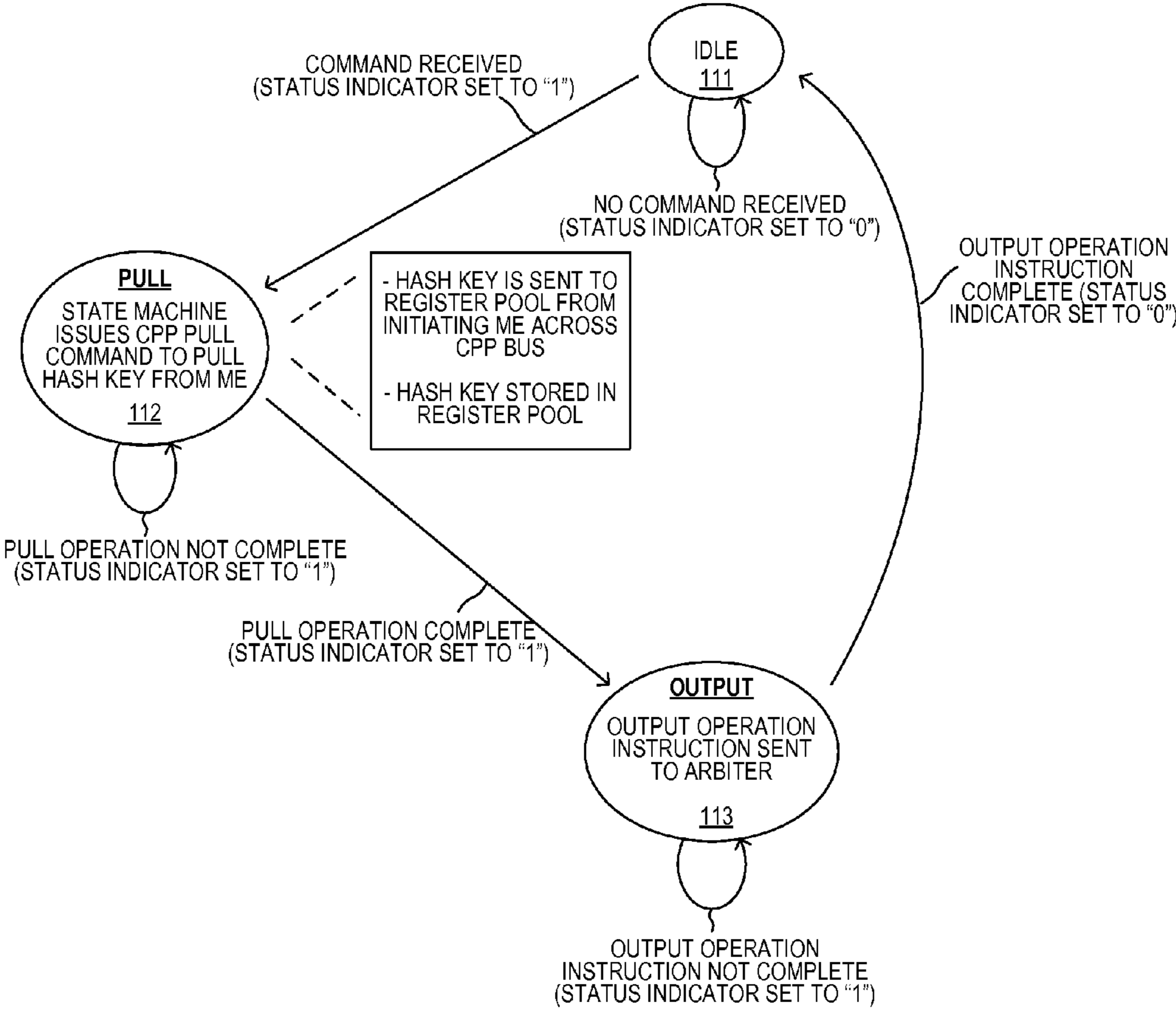
STATE MACHINE STATE DIAGRAM FIG. 16
