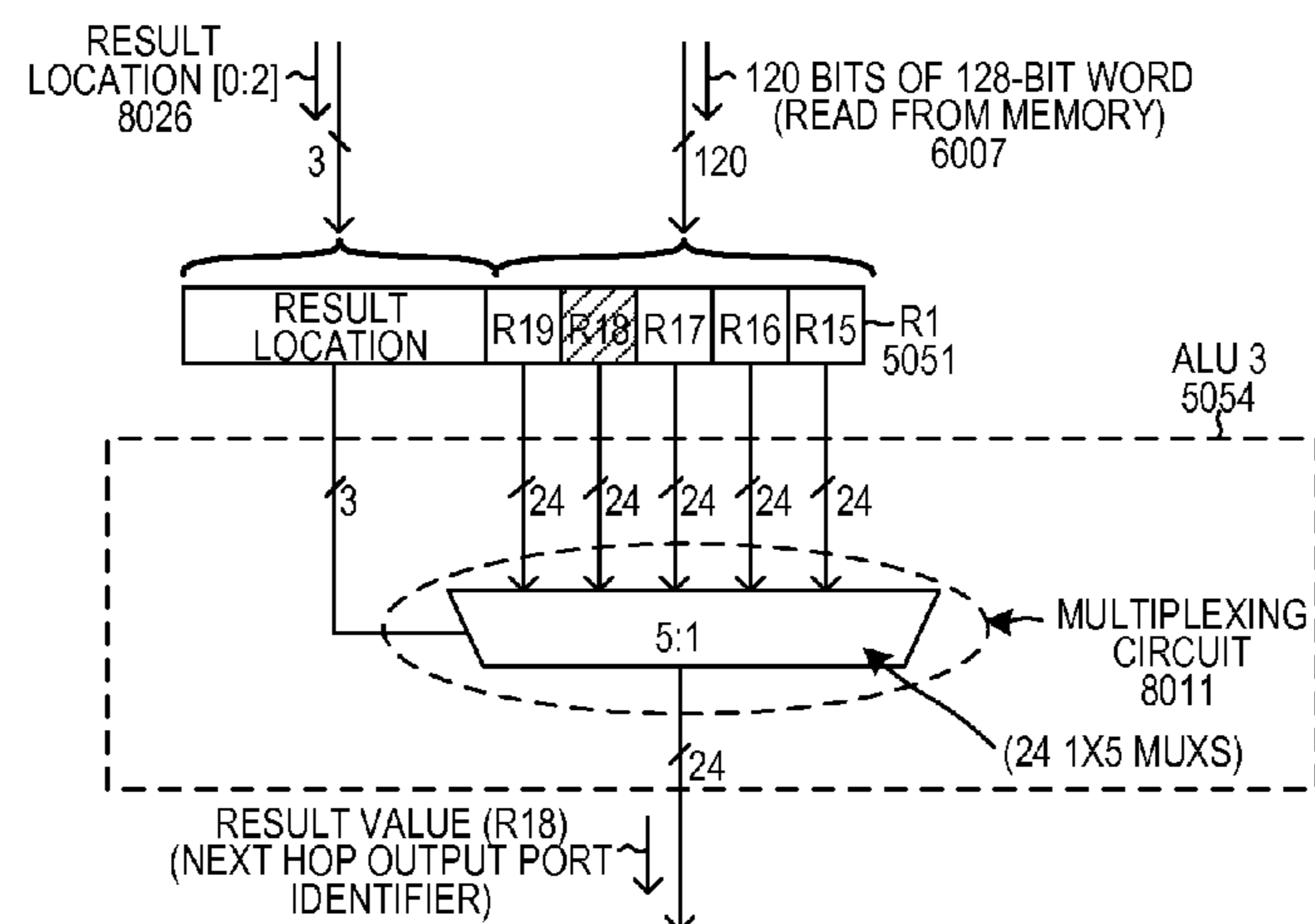
DIRECT 24-BIT LOOK-UP STAGE FIG. 49
