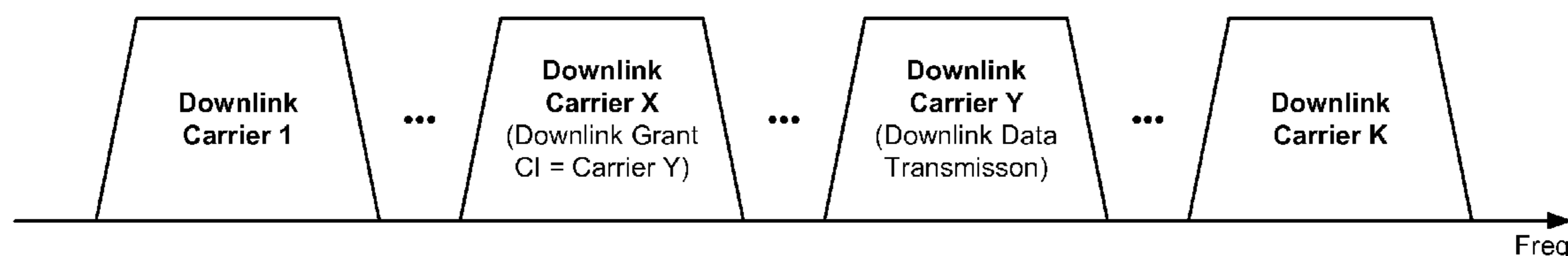
Cross-Carrier Assignment on Downlink
