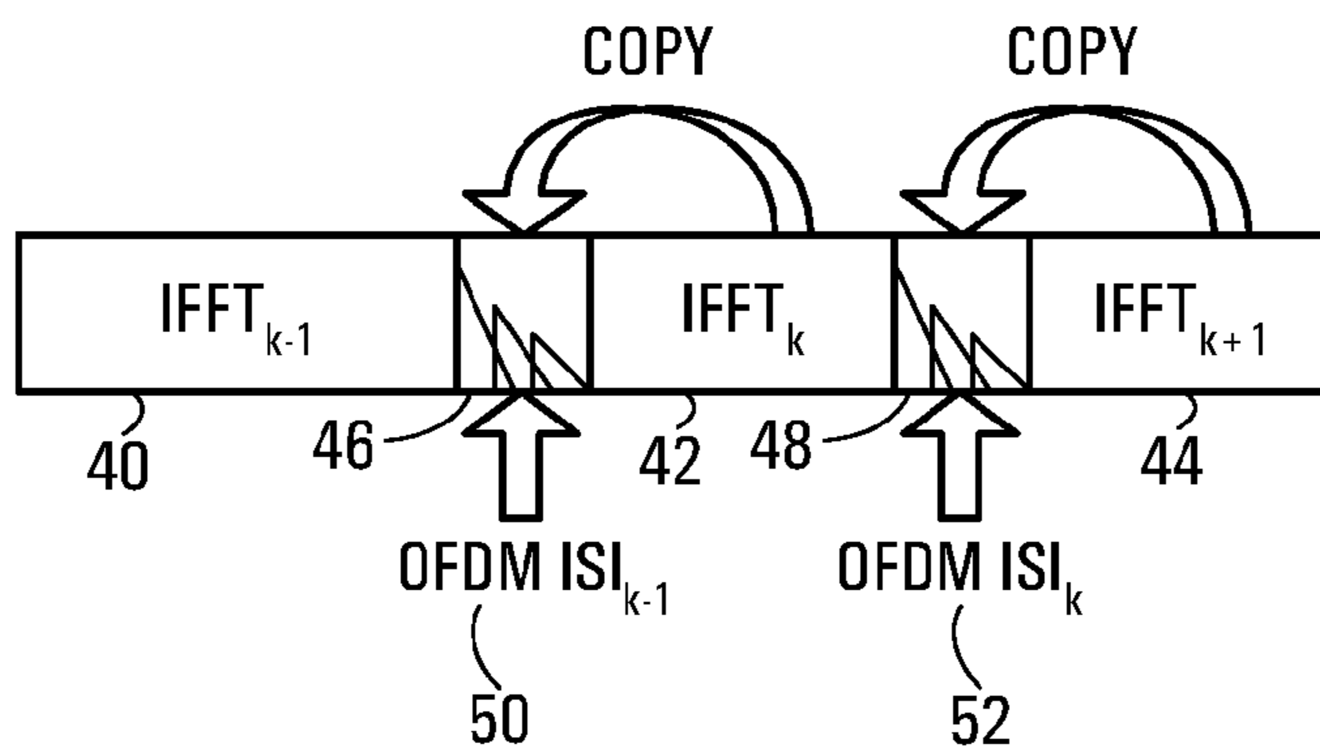
FIG. 2 (PRIOR ART)
