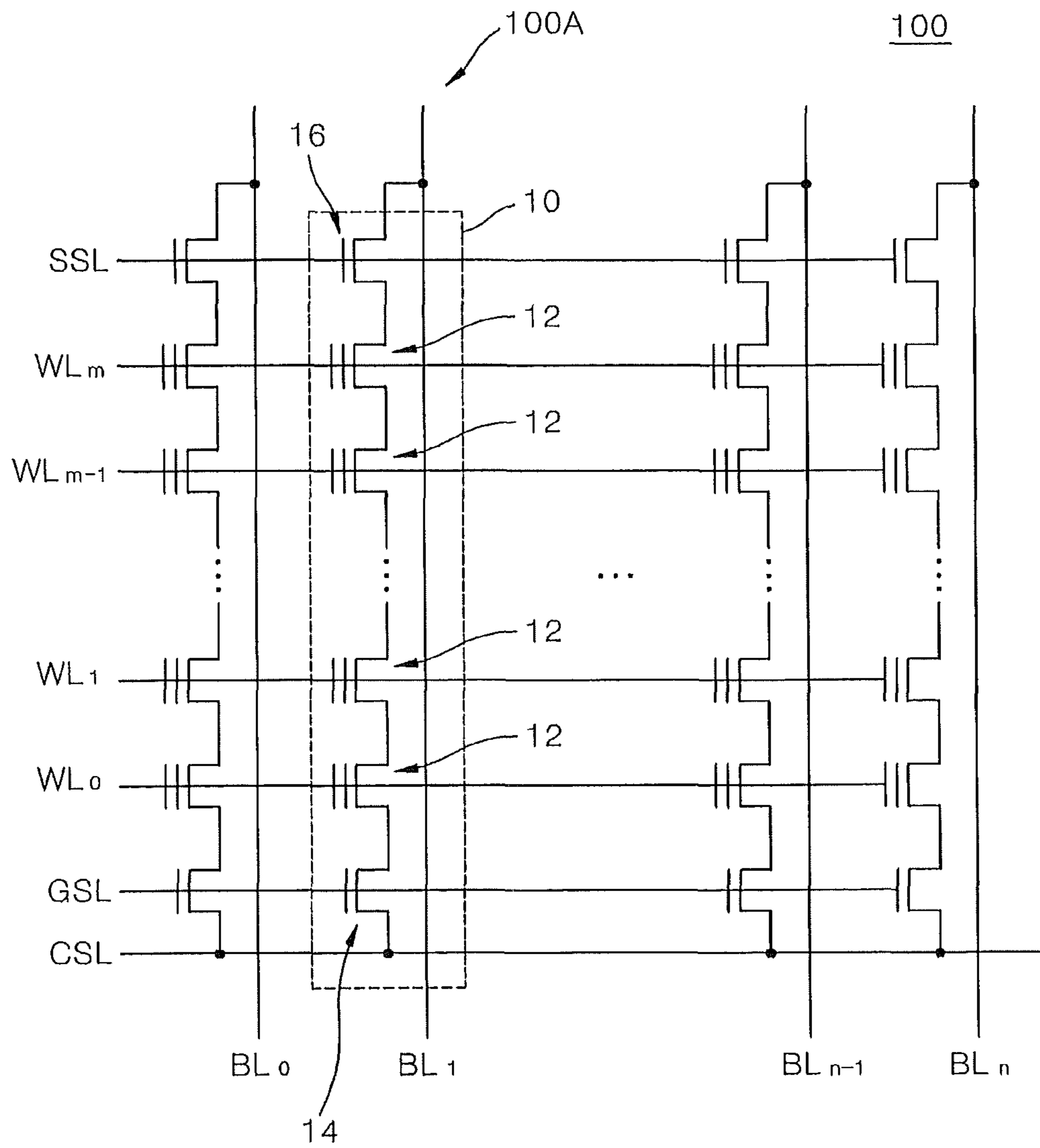
FIG. 2 (PRIOR ART)
