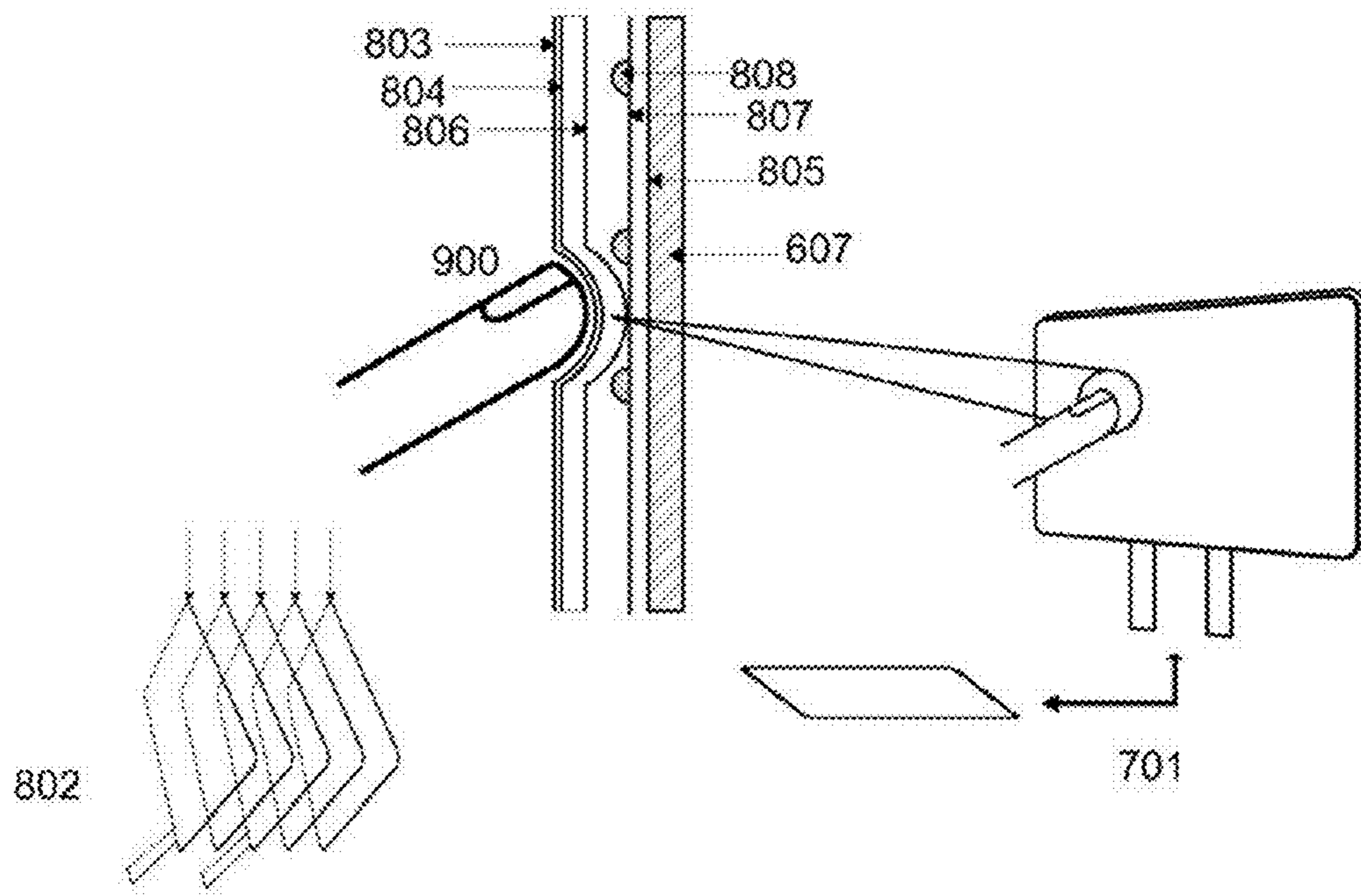
FIG. 2 (PRIOR ART)
