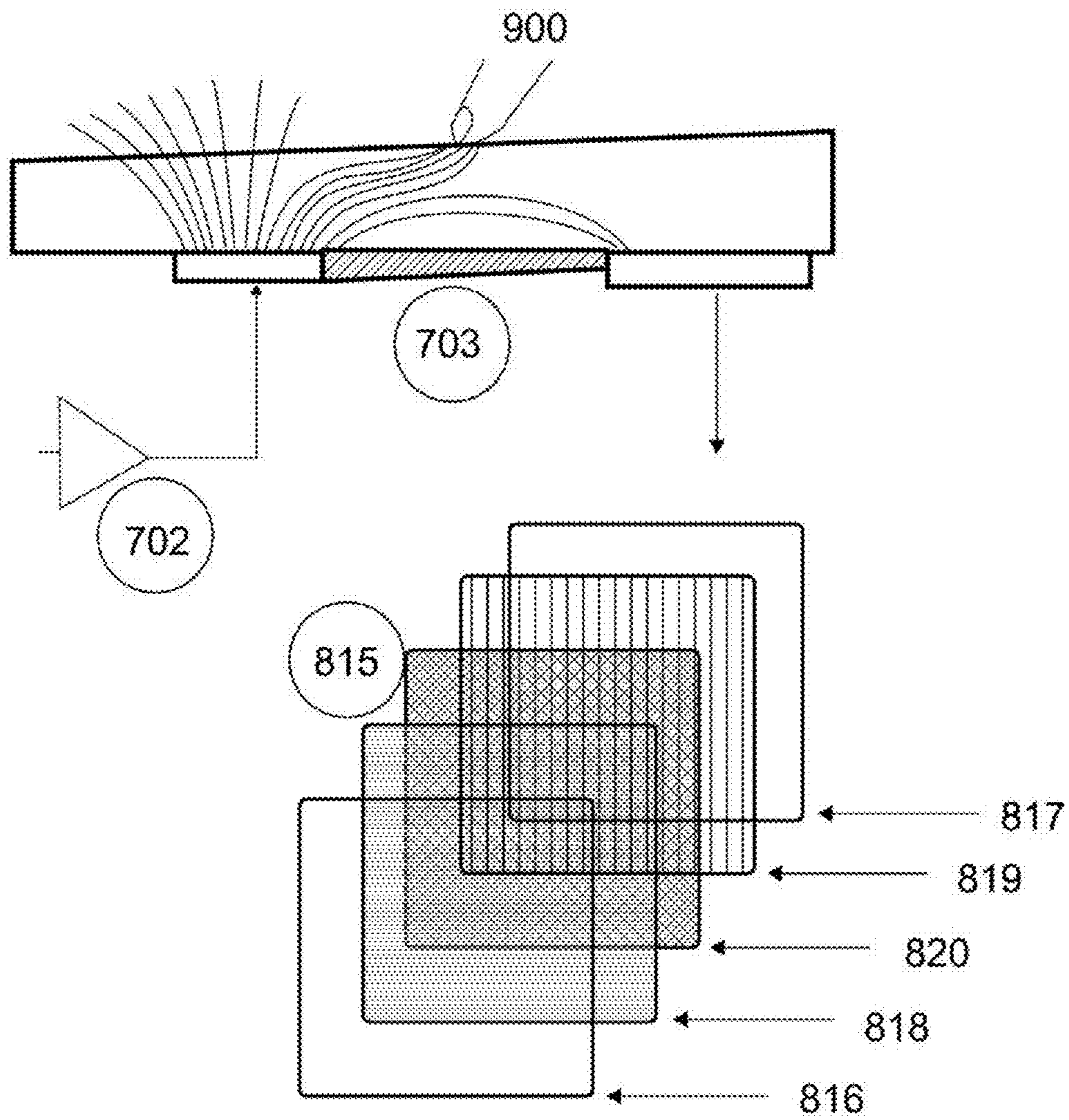
FIG. 4 (PRIOR ART)
