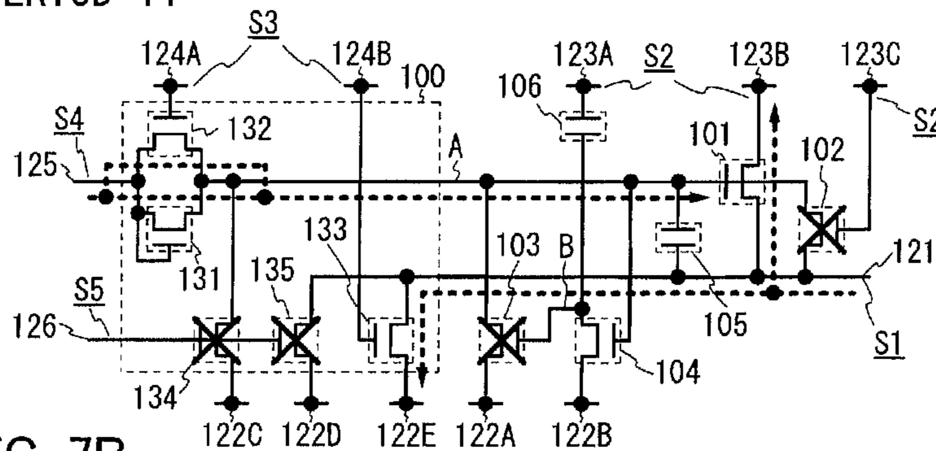
FIG. 7A PERIOD T1
