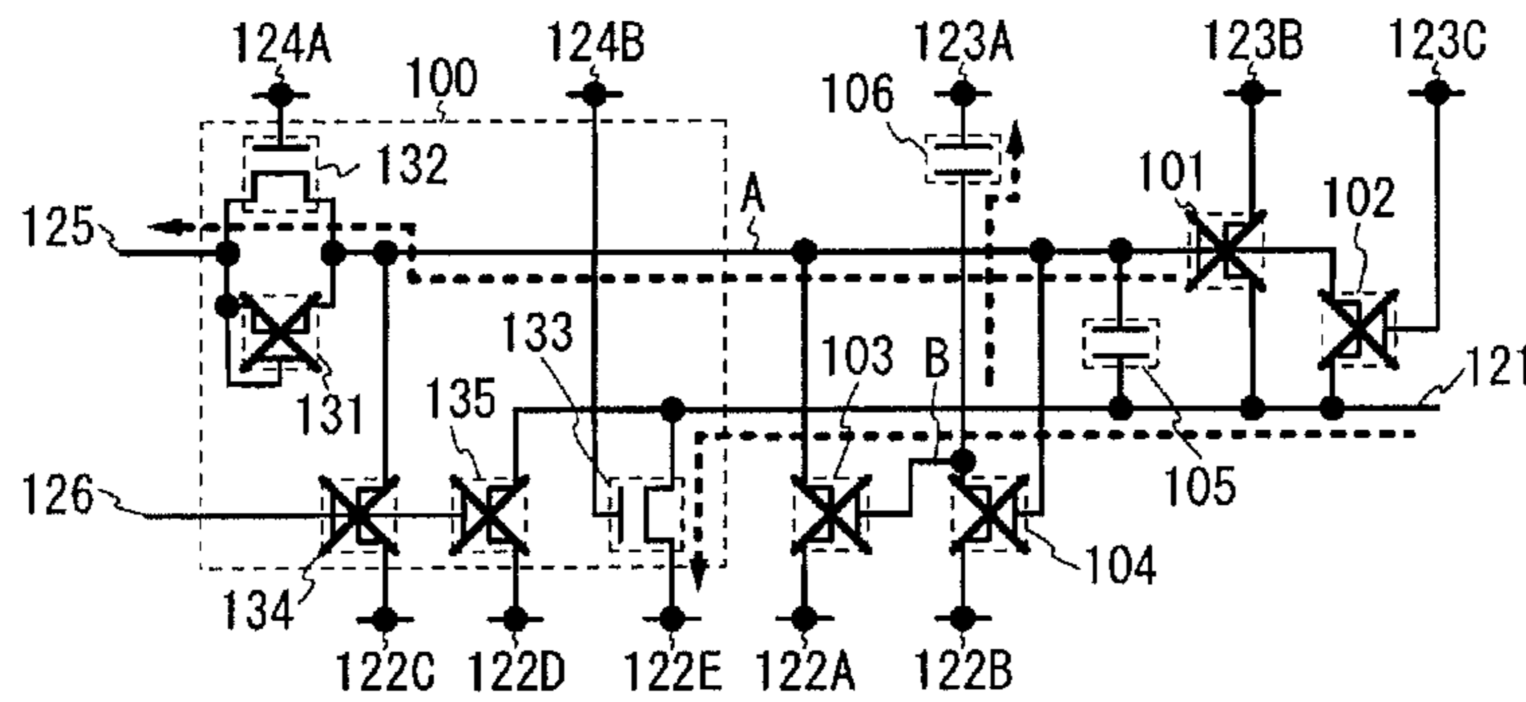
FIG. 8B PERIOD T5
