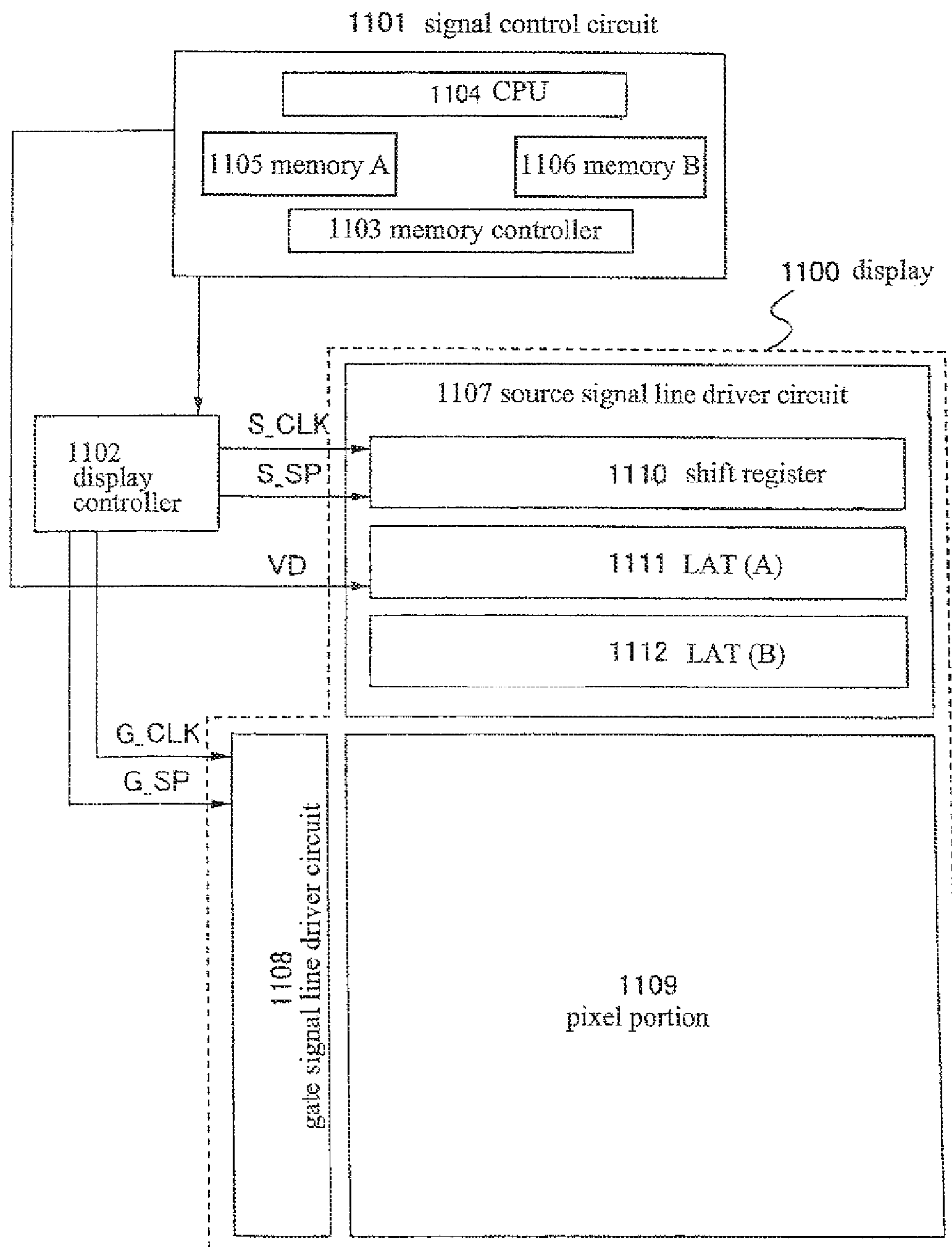
Fig.10 (PRIOR ART)
