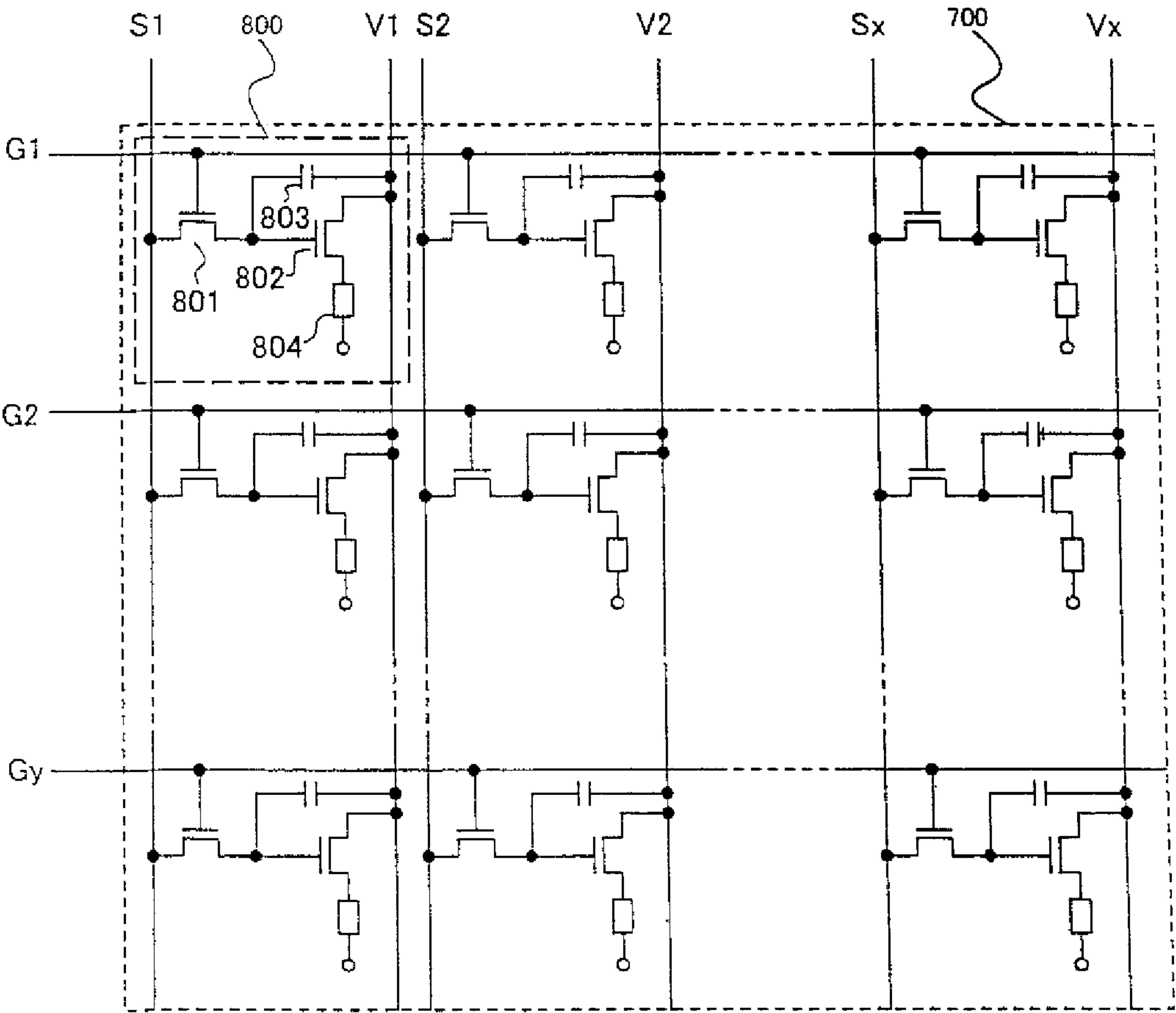
Fig.7 (PRIOR ART)
