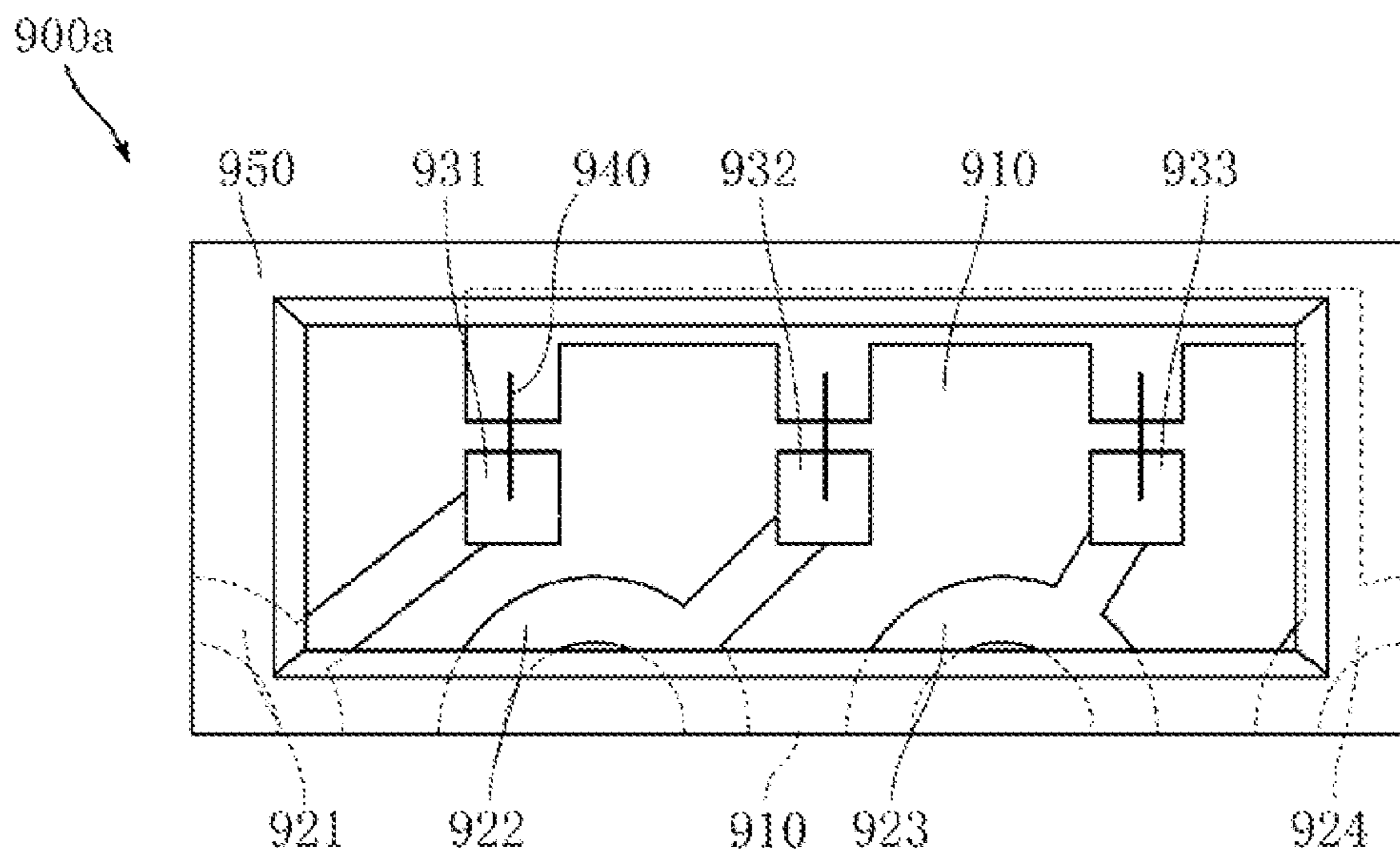
FIG. 75 (PRIOR ART)
