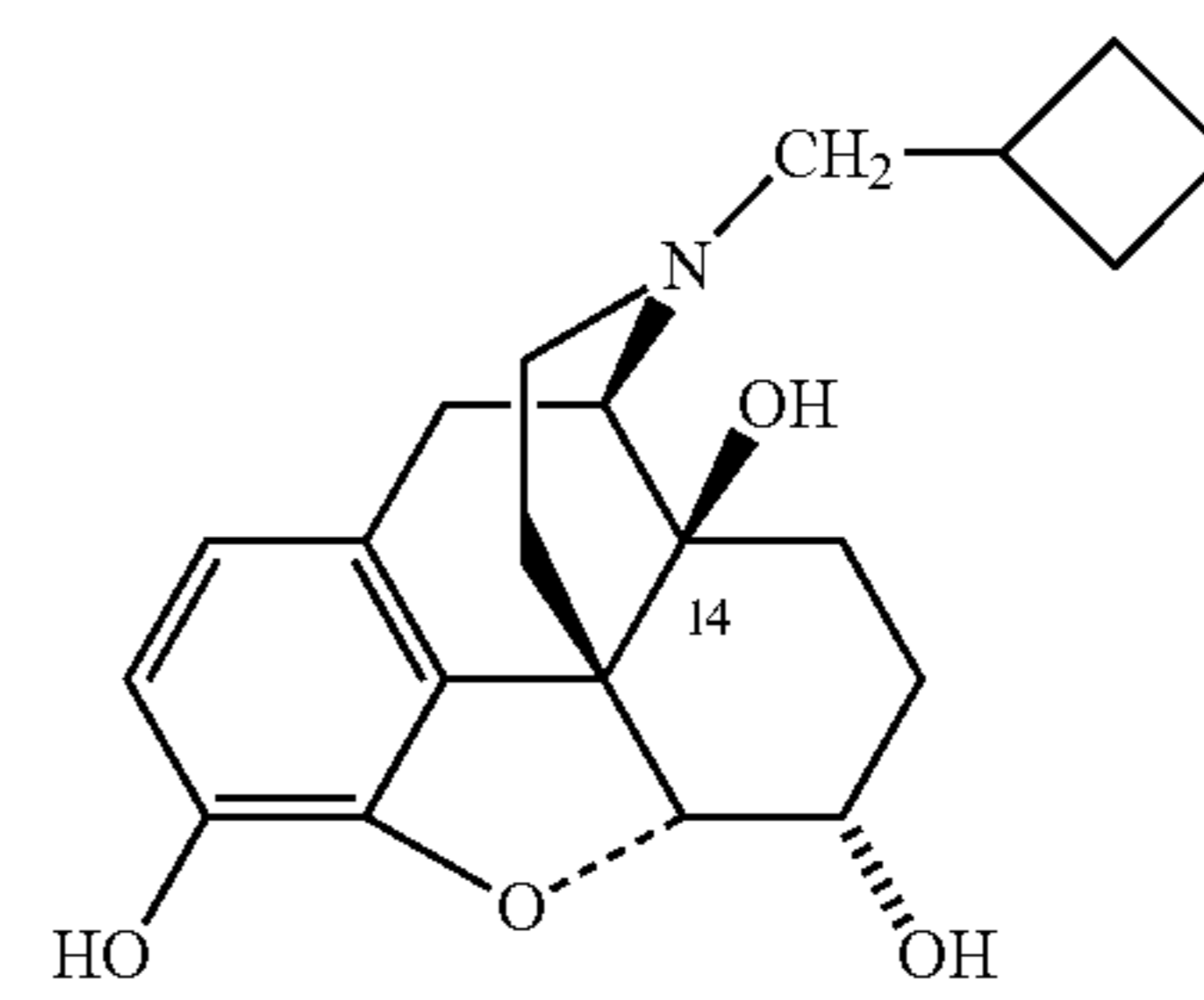
Nalbuphine
