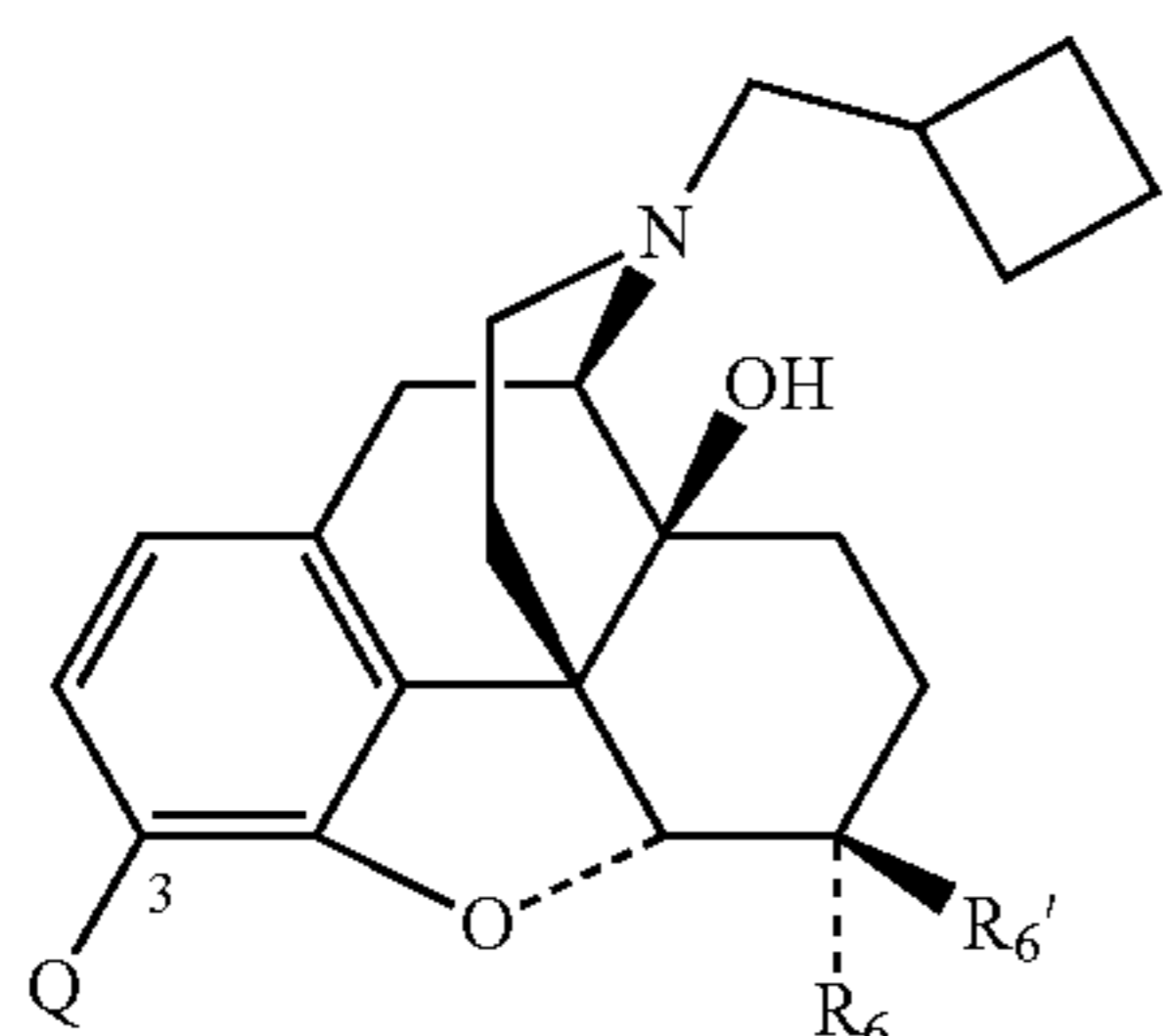
Nalbuphine core
