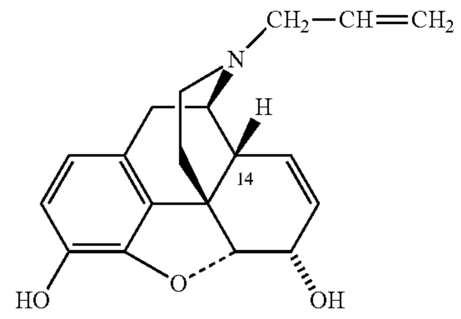
Nalorphine
