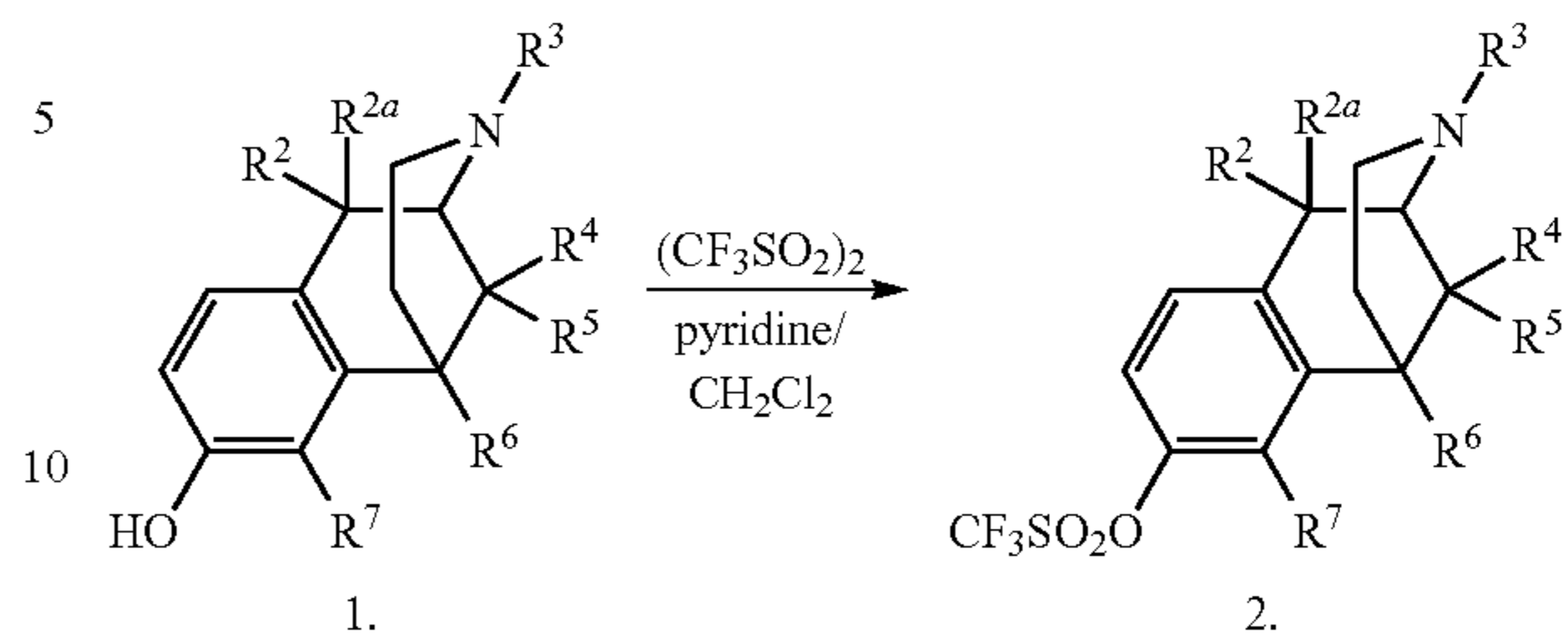
Scheme 2
