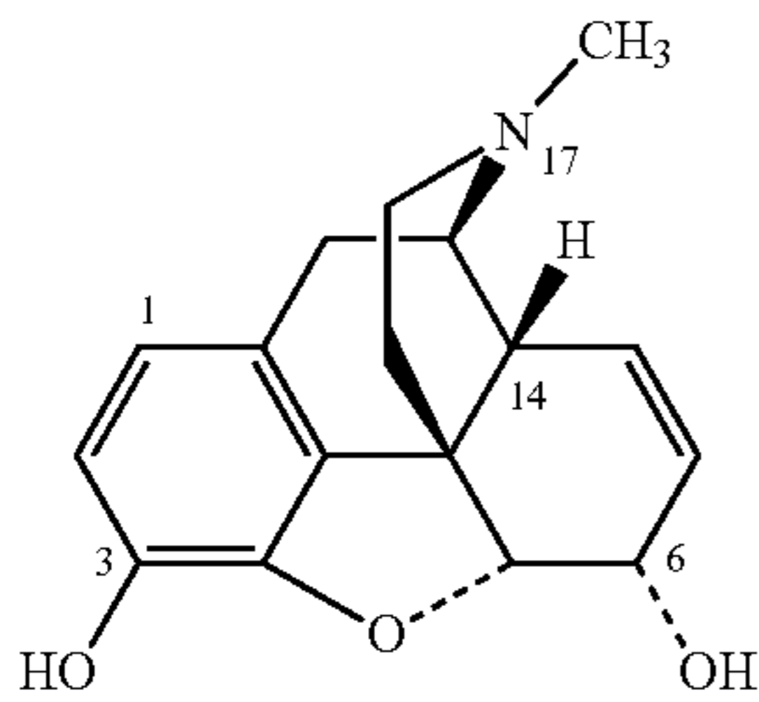
Morphine
