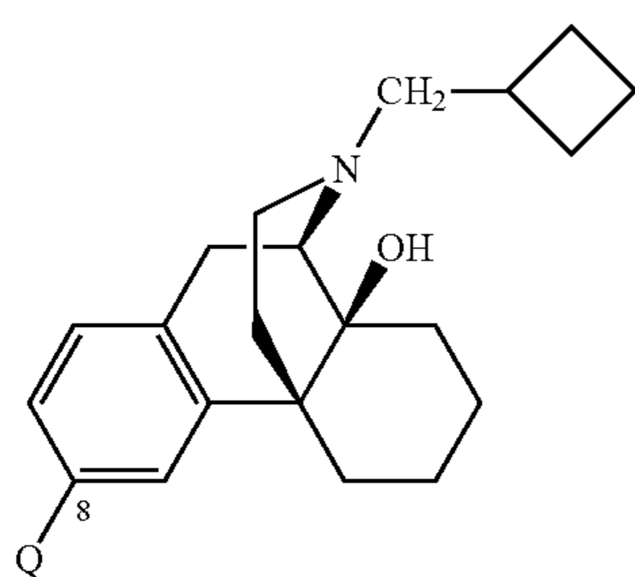
Butorphanol core
