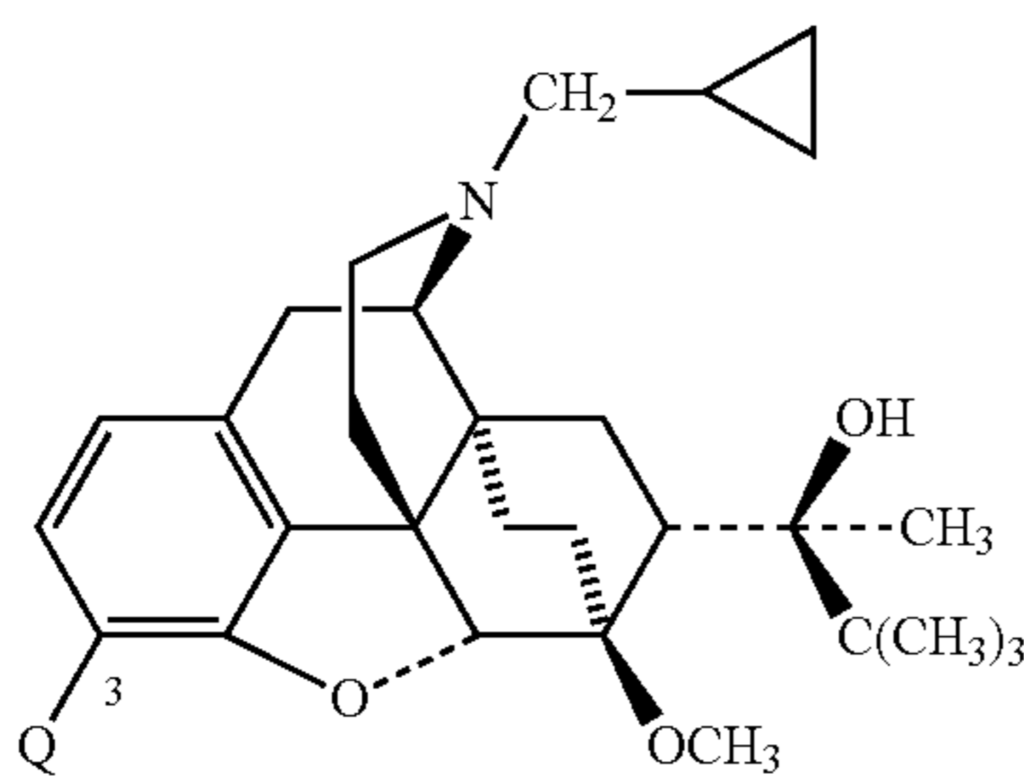
Buprenorphine core
