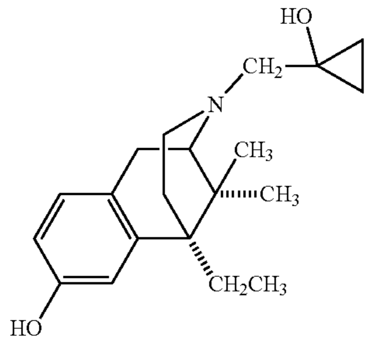
Bremazocine
