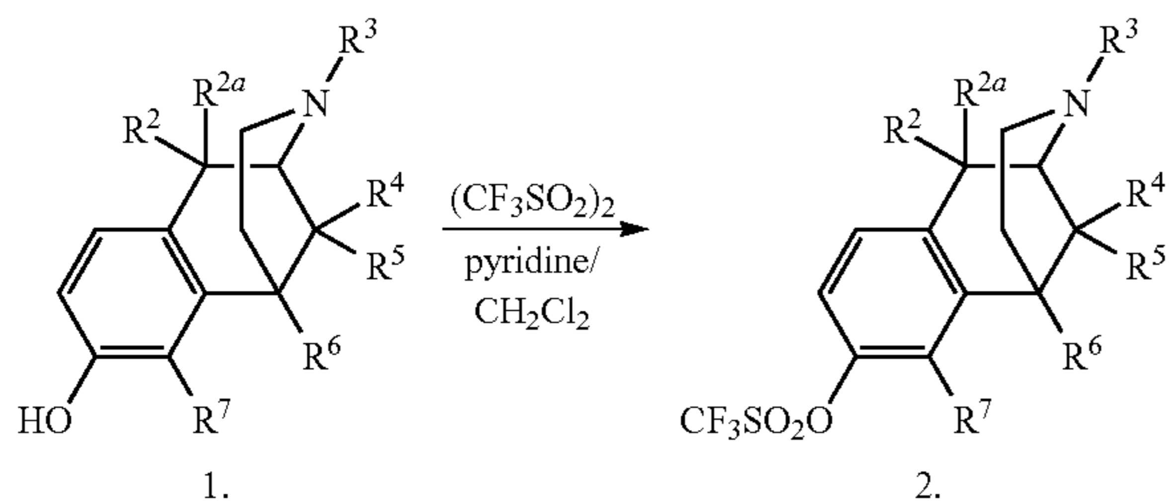
Scheme 1
