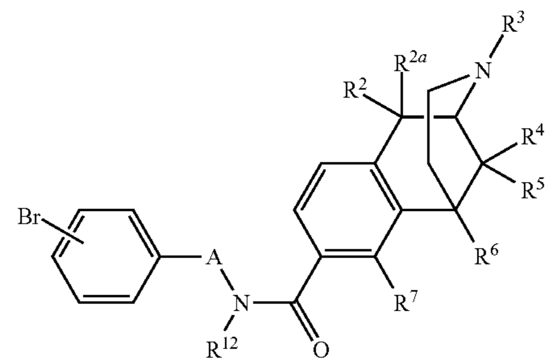
Scheme 3
