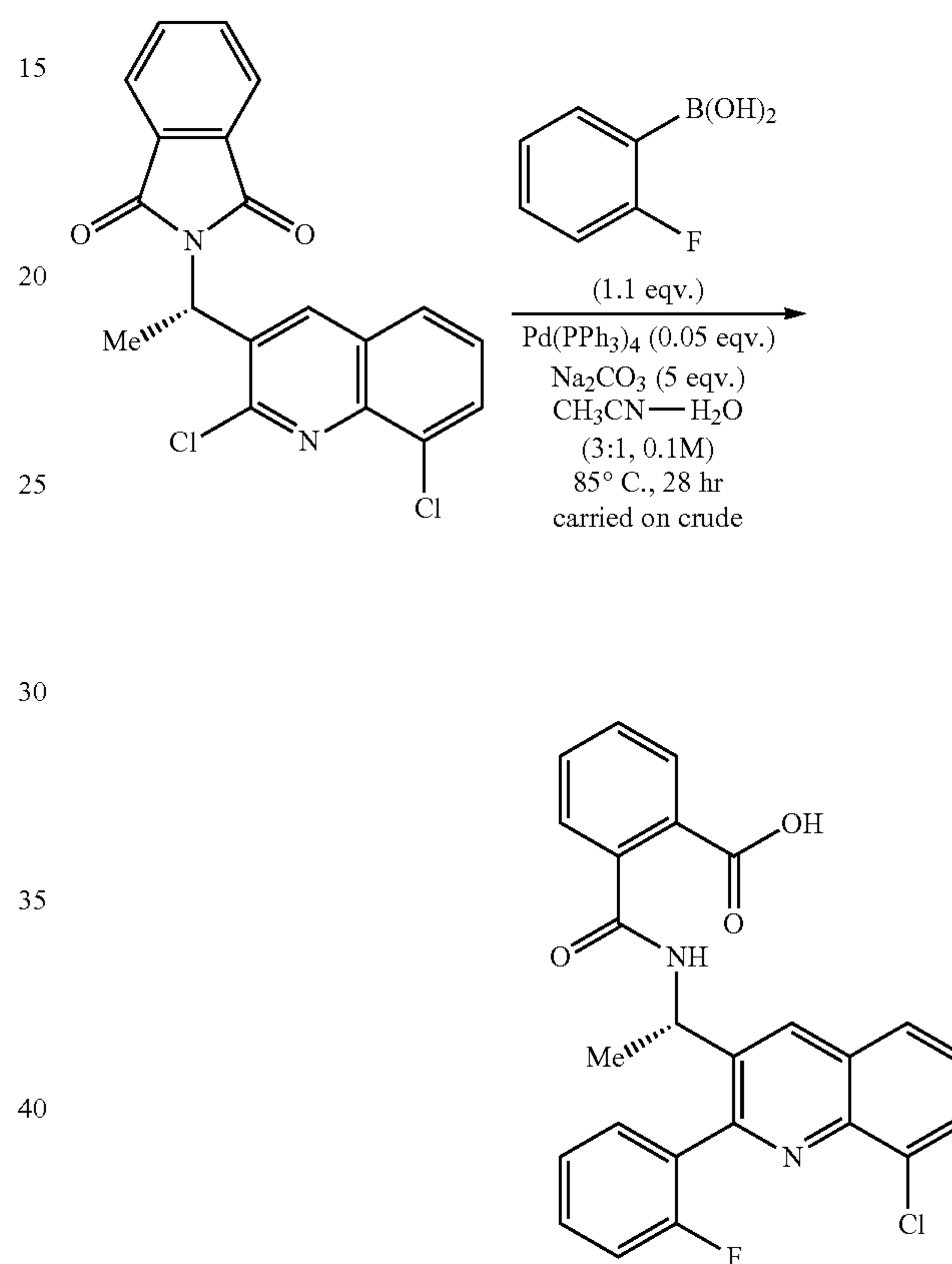
N-((2-(3-Fluorophenyl)-8-methoxyquinolin-3-yl)methyl)-9H-purin-6-amine
