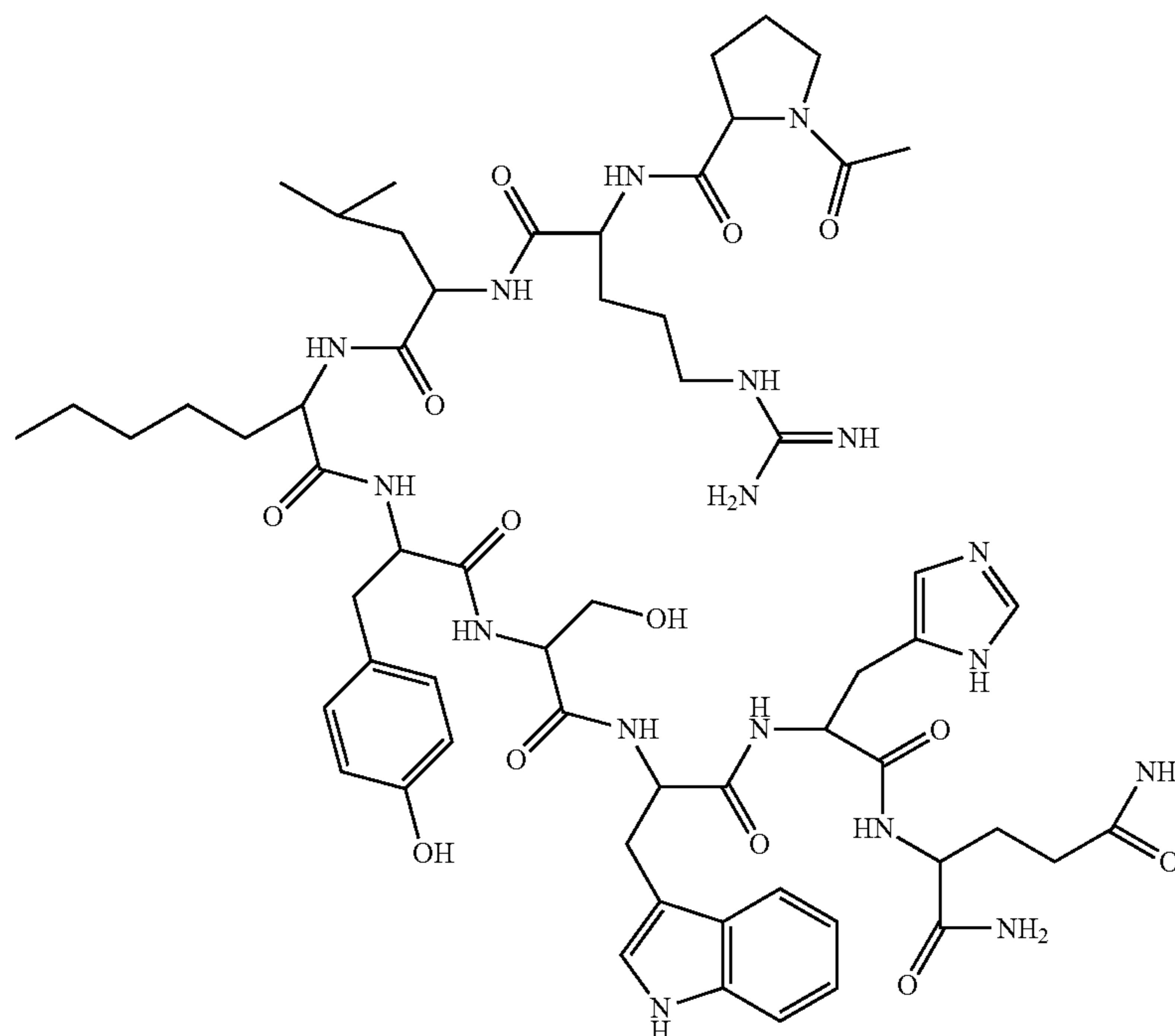
LHRH-dioleoyl monoamine
