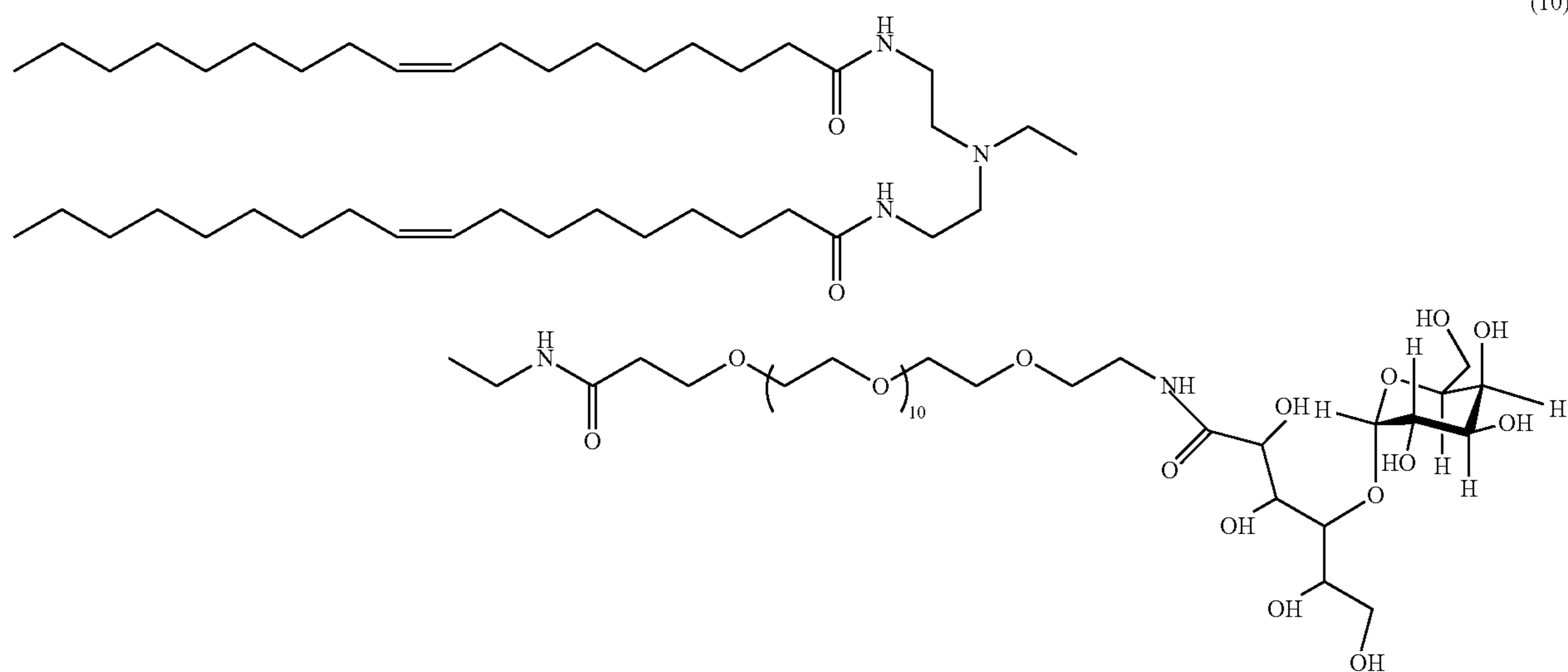
lactobionyl-dioleoyl monoamine
