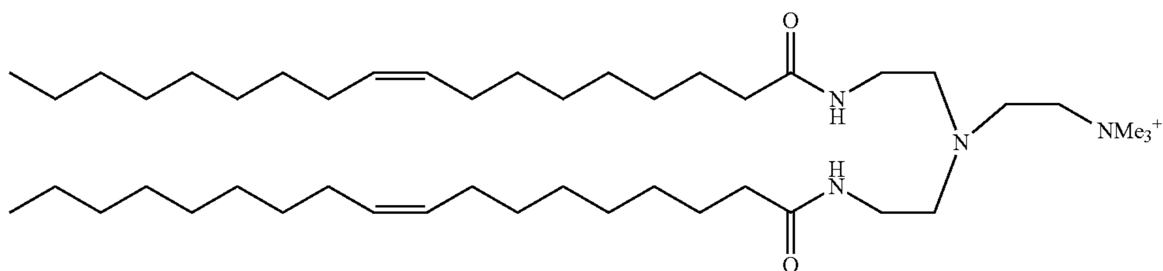
Methyl-dioleoyl monoamine
