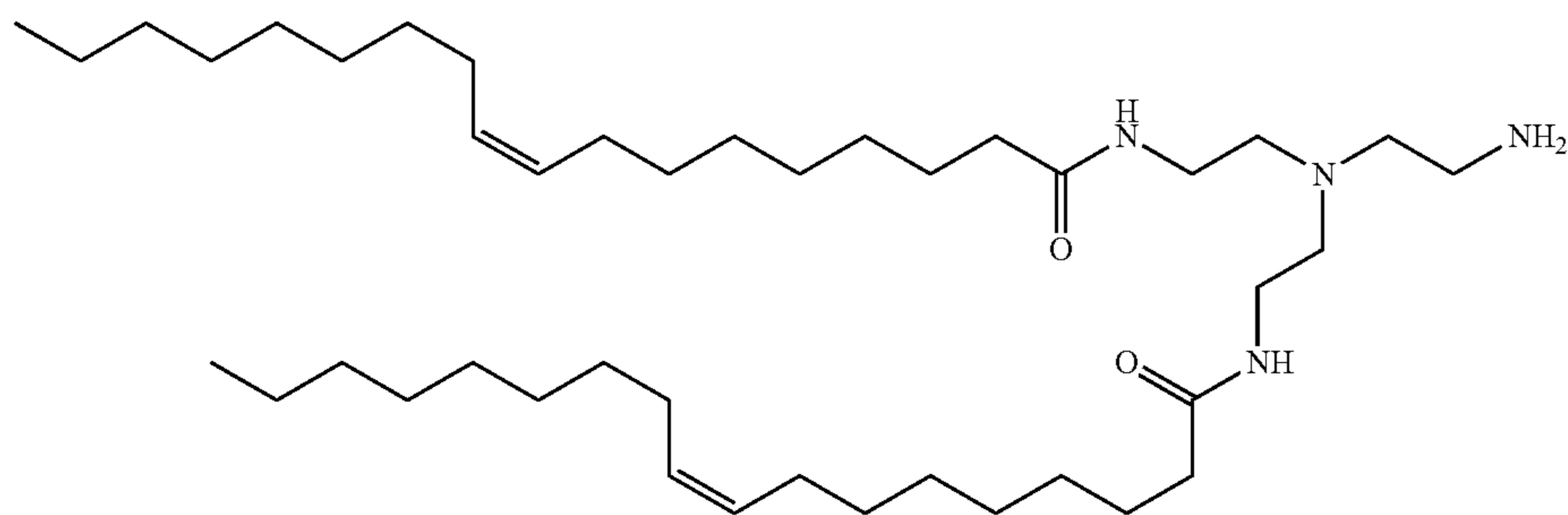
dioleoyl monoamine
