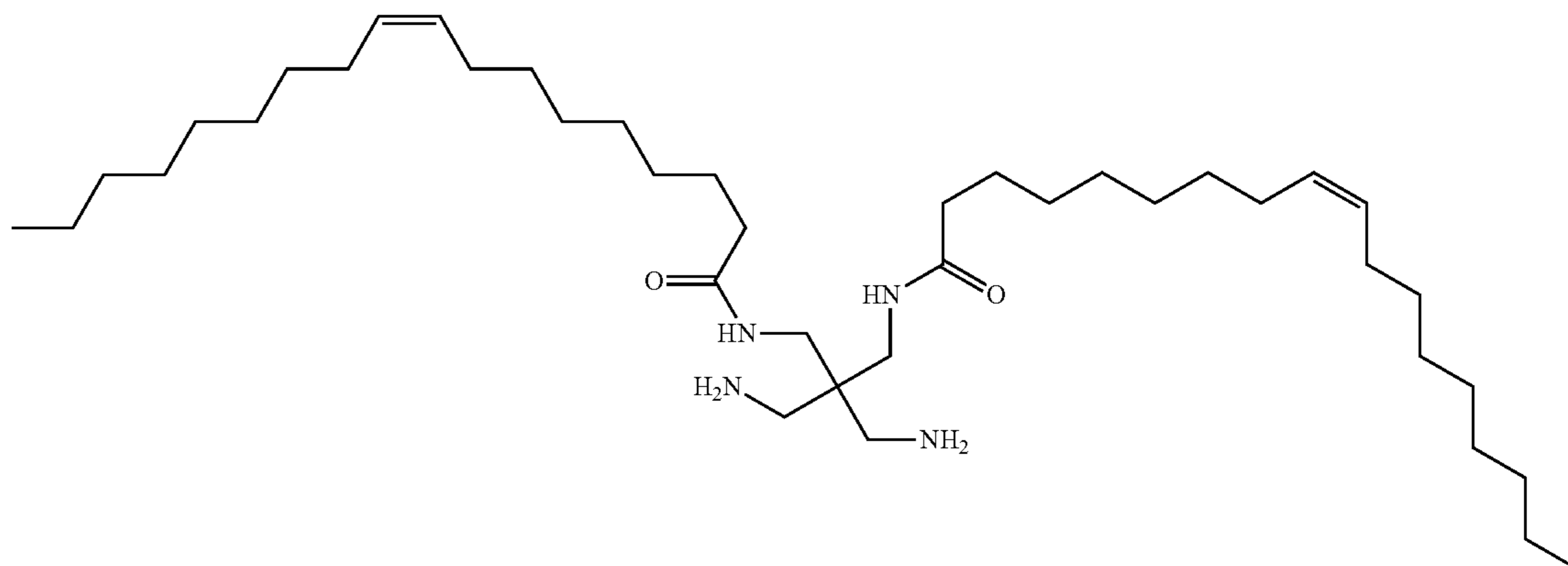
dioleoyl crossamine
