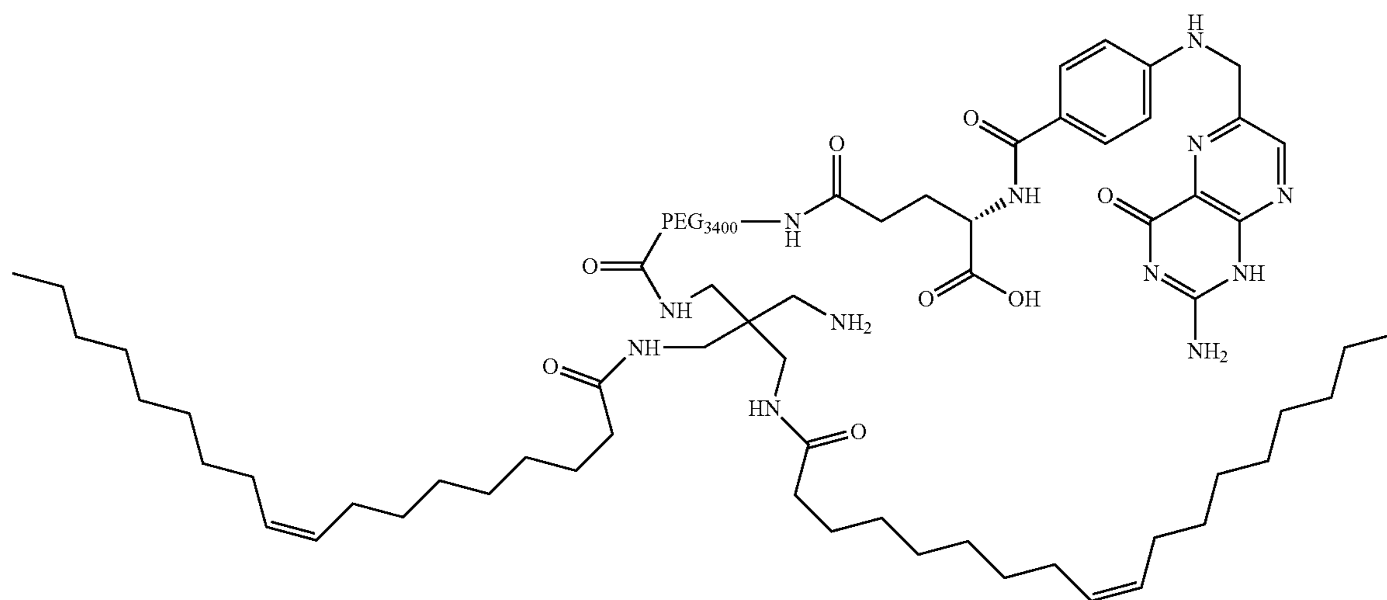
folate-PEG-dioleoyl crossamine
