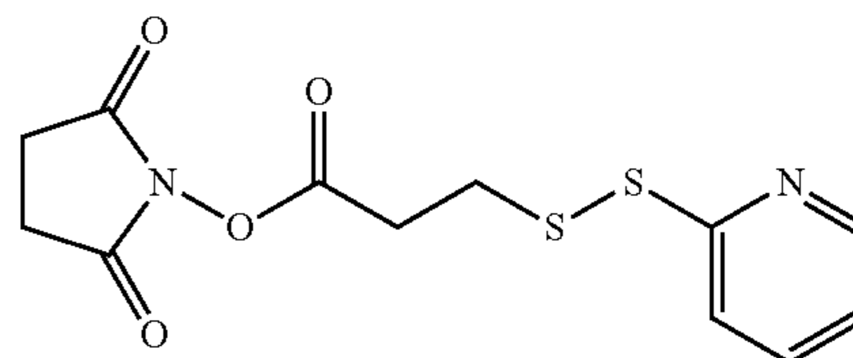
N-succinimidyl-3-(2-pyridyldithio)-propionate
