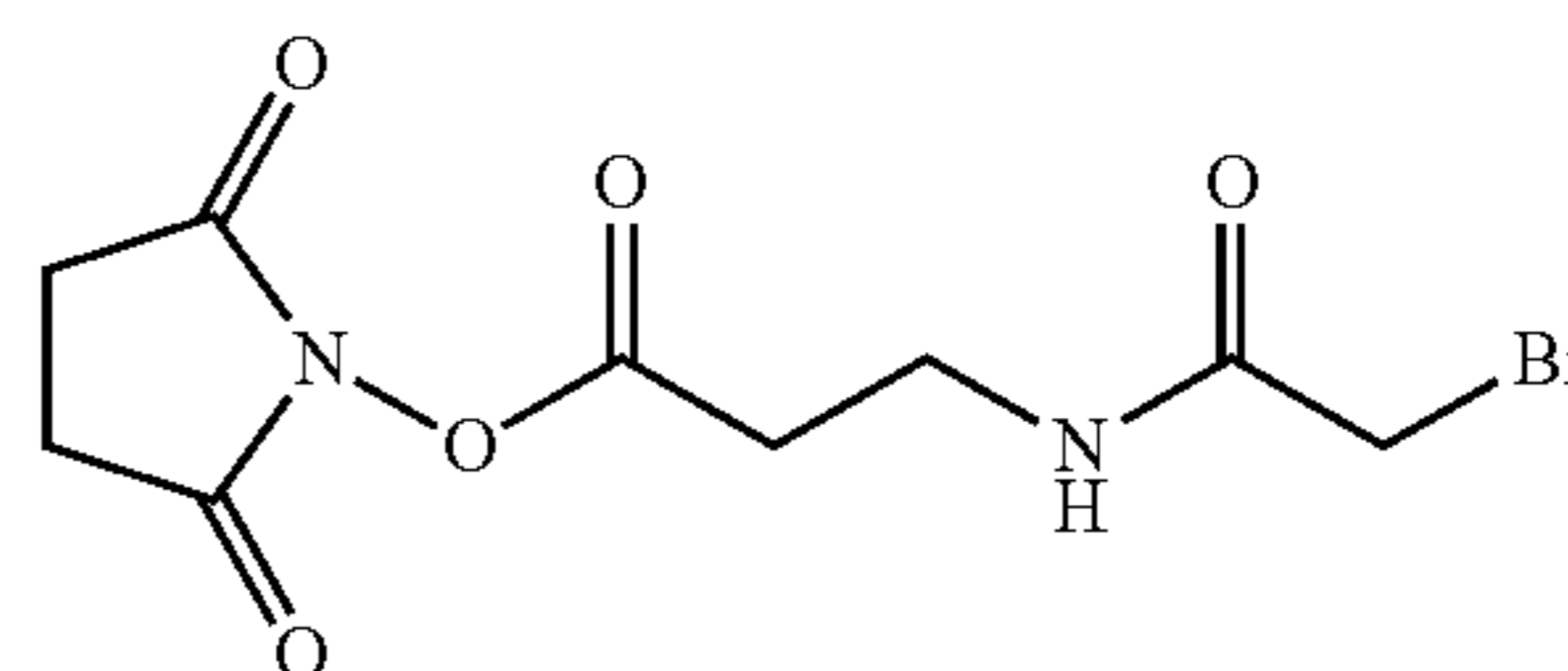
N-succinimidyl-3-bromoacetamidopropionate
