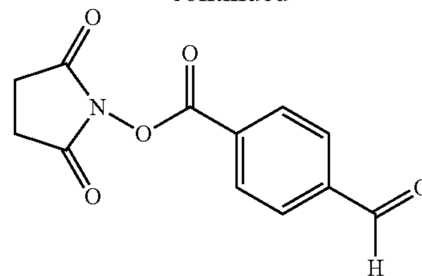
N-succinimidyl-4-formylbenzoate
