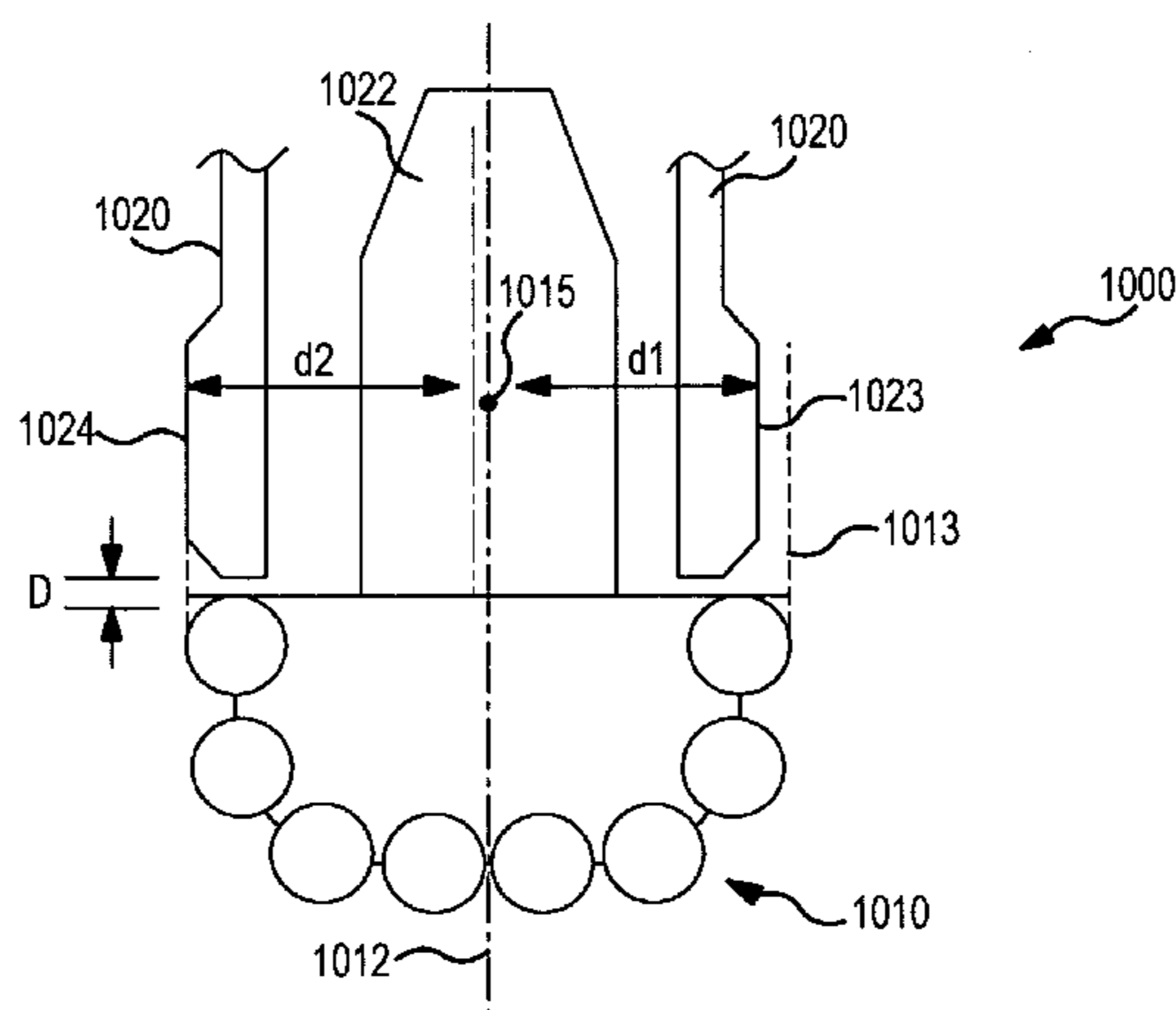
GAUGE PAD ASSEMBLY WITH CUTTER PROFILE.
