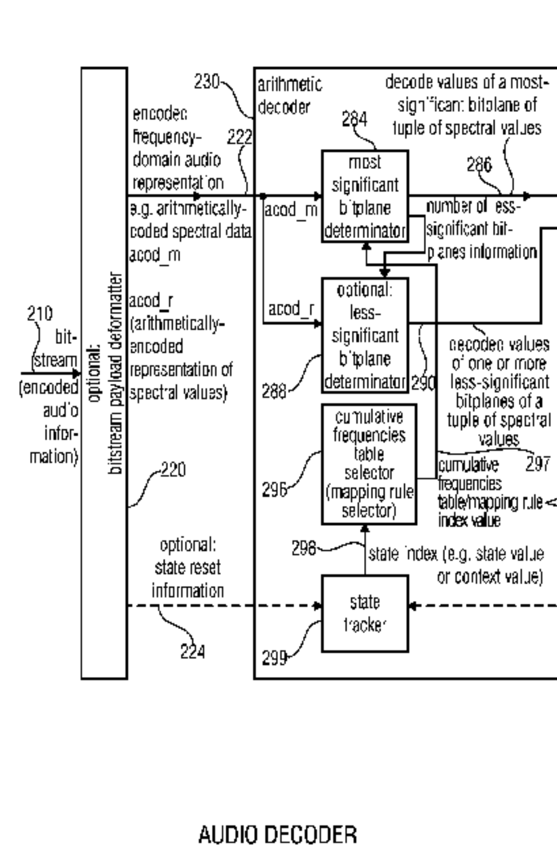
AUDIO DECODER
