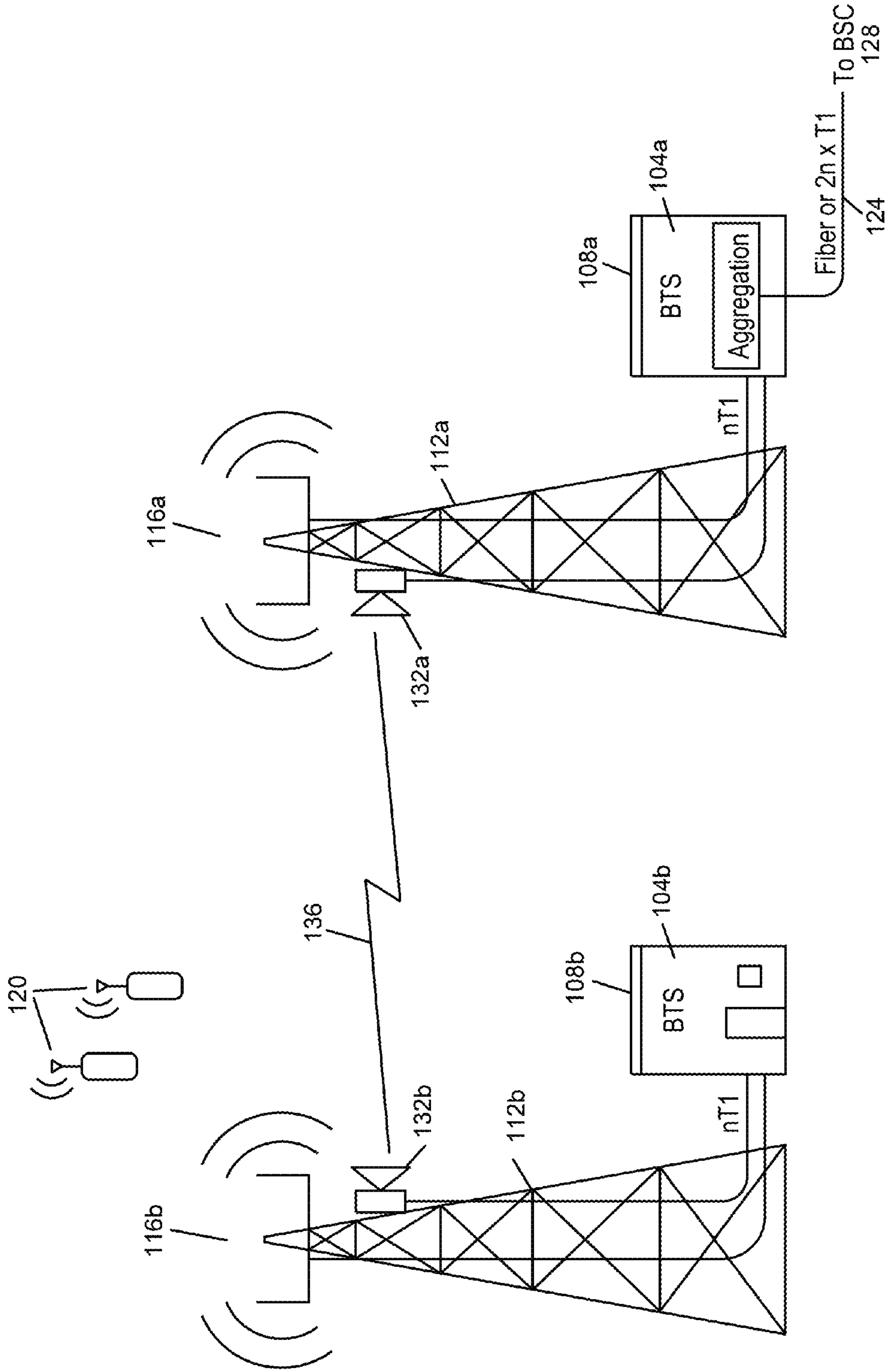
FIG. 1 (Prior Art)
