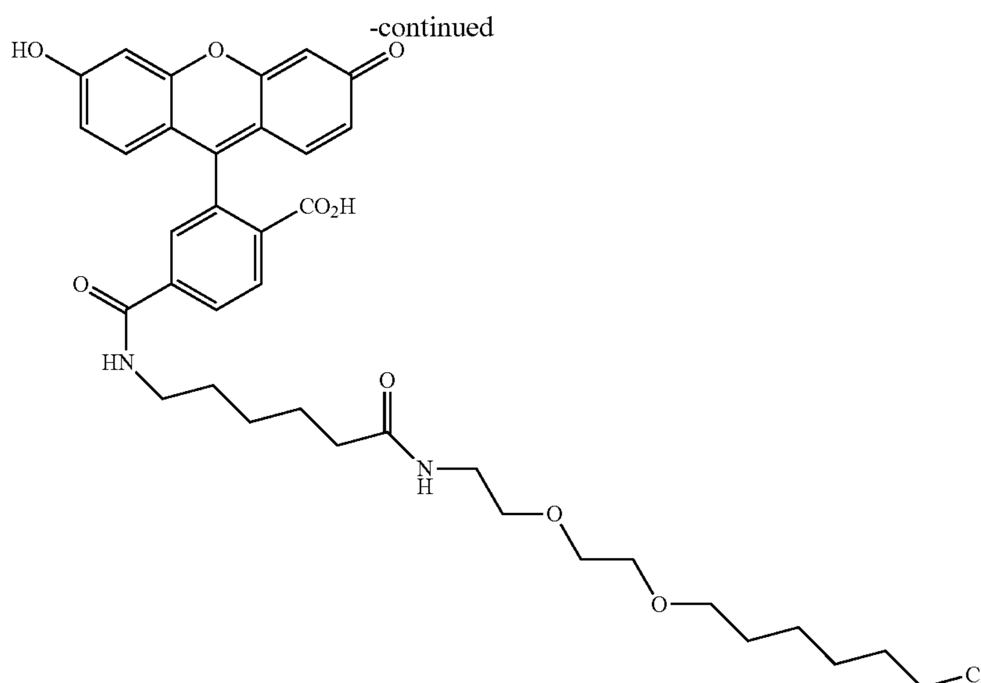
a compound of formula XXIV
