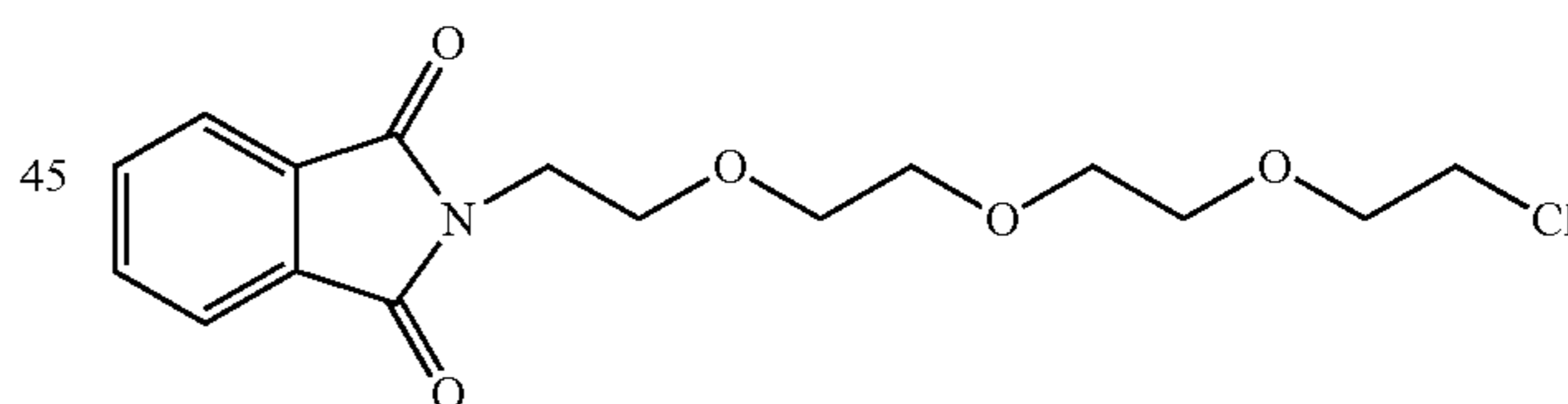
a compound of formula XXVI
