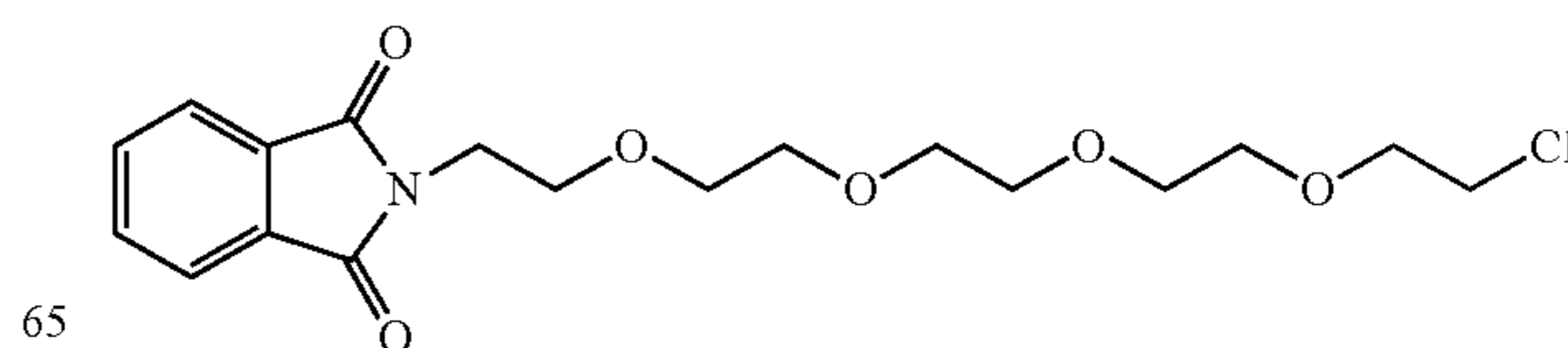
a compound of formula XXVII
