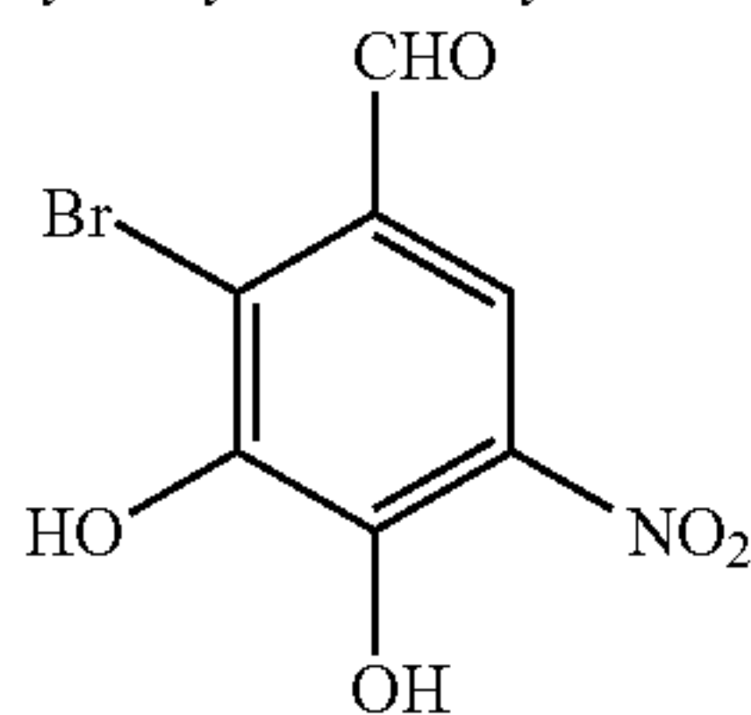
2-Bromo-3,4-dihydroxy-5- nitrobenzaldehyde
