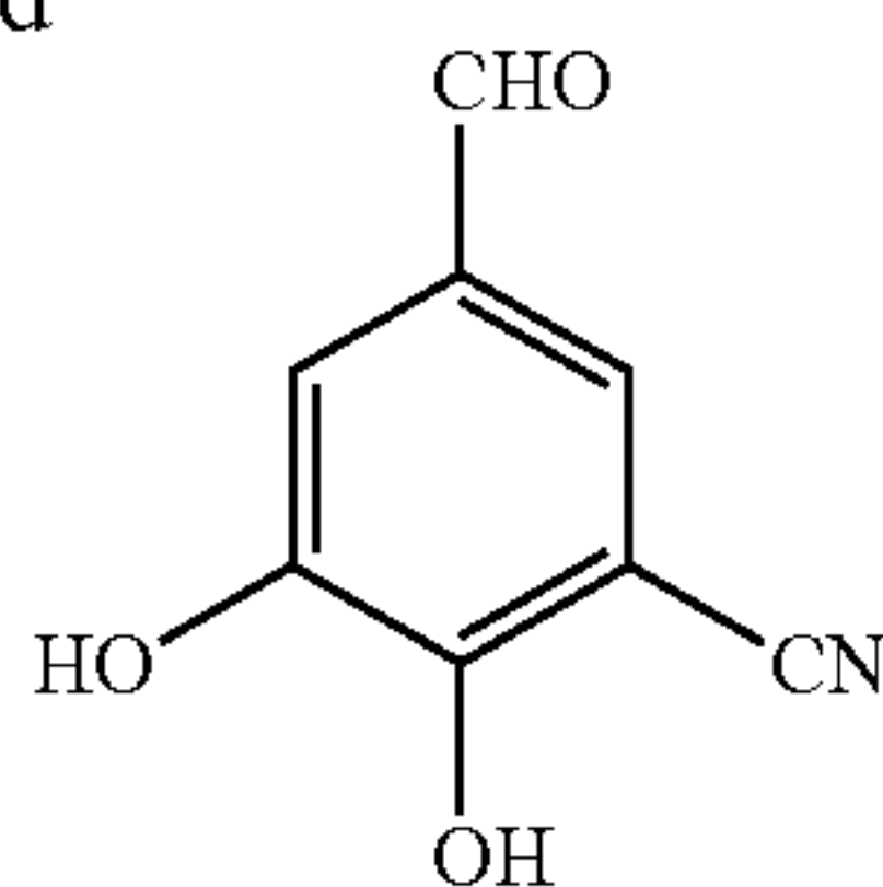
5-Formyl-2,3- dihydroxybenzonitrile
