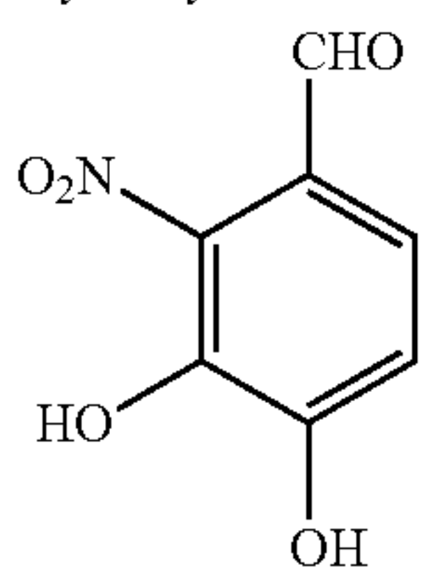
3,4-Dihydroxy-2- nitrobenzaldehyde
