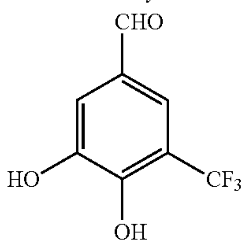
3,4-Dihydroxy-5- (trifluoromethyl) benzaldehyde
