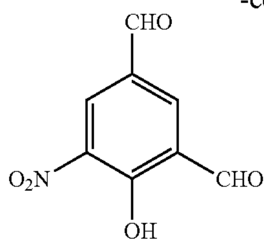
4-Hydroxy-3-Nitro-m- Phthaldialdehyde
