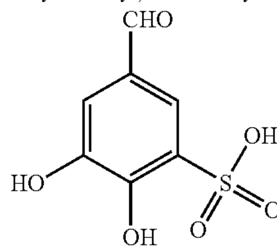
5-formyl-2,3- dihydroxybenzenesulfonic acid
