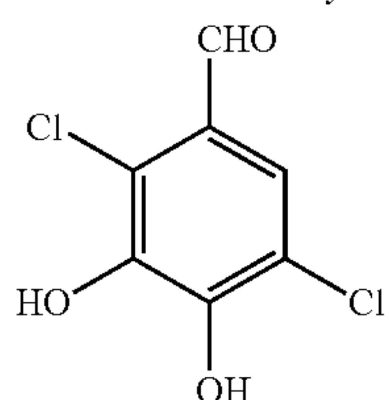
2,5-Dichloro-3,4- dihydroxybenzaldehyde
