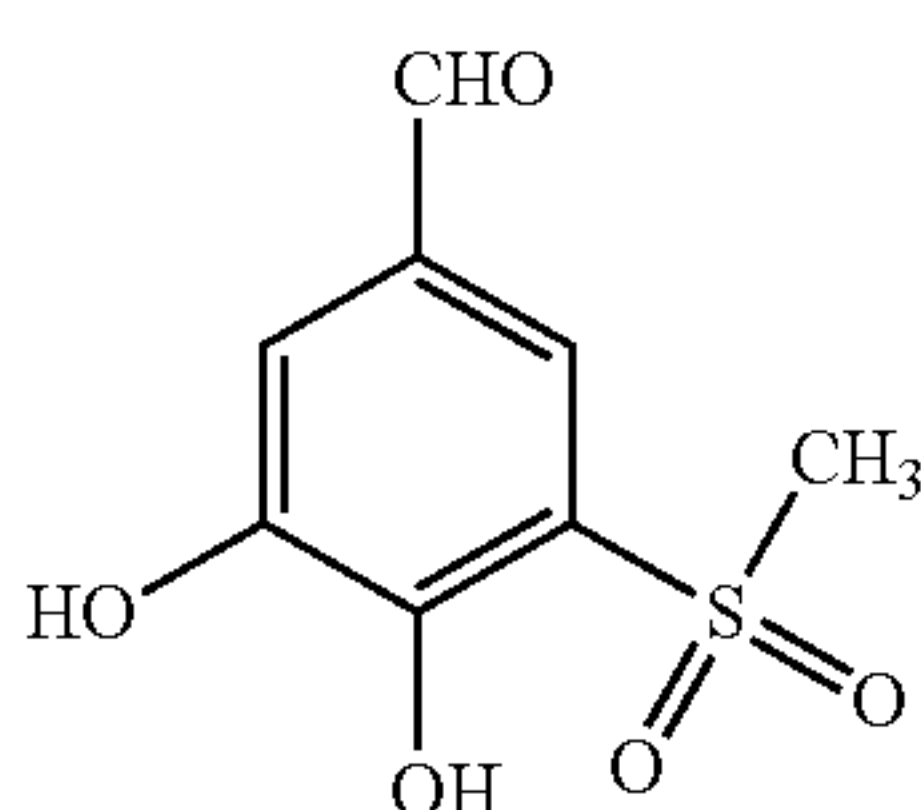
3,4-Dihydroxy-5- (methylsulfonyl)benzaldehyde
