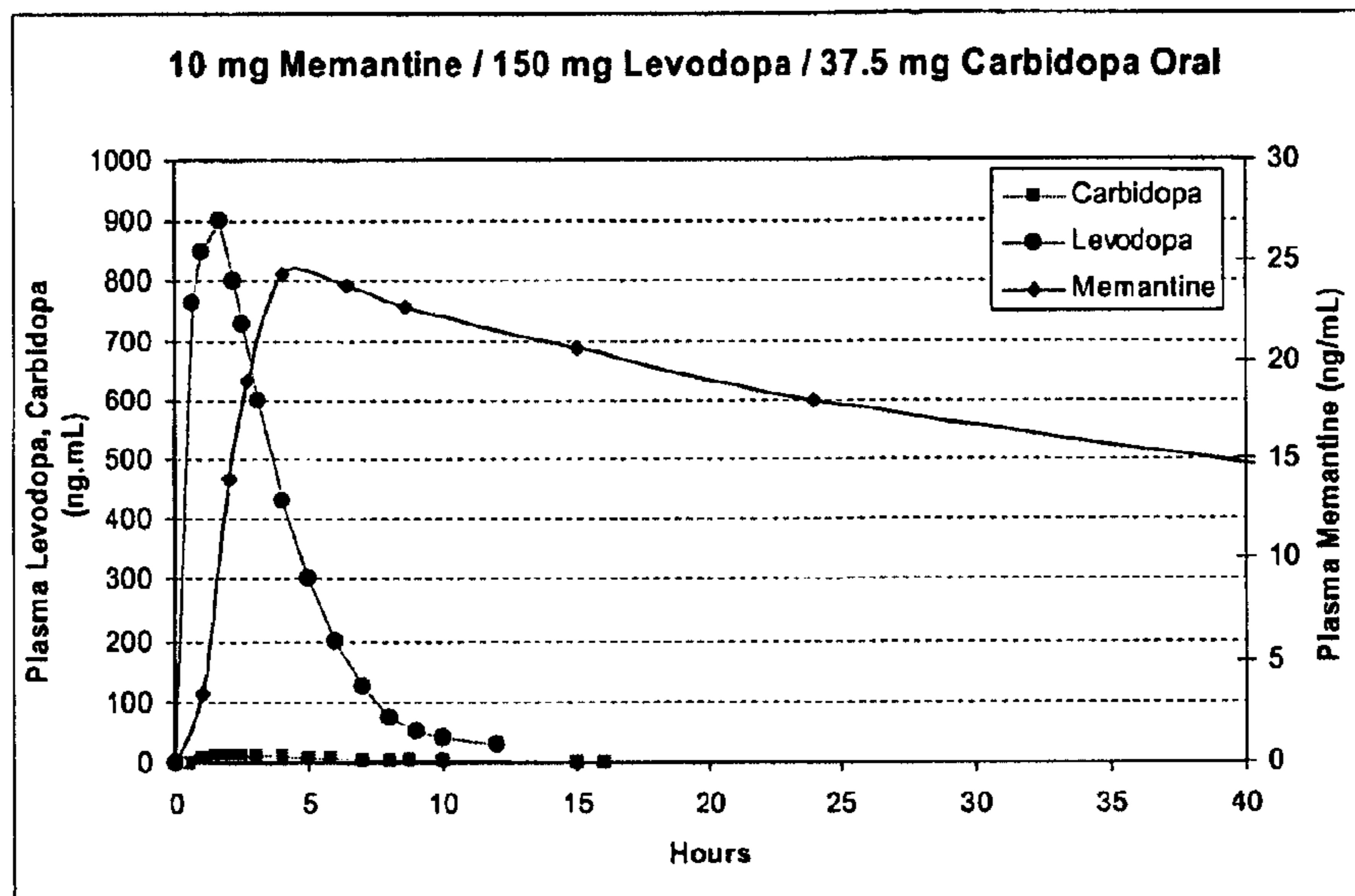
Figure 7: Target Pharmacokinetics
