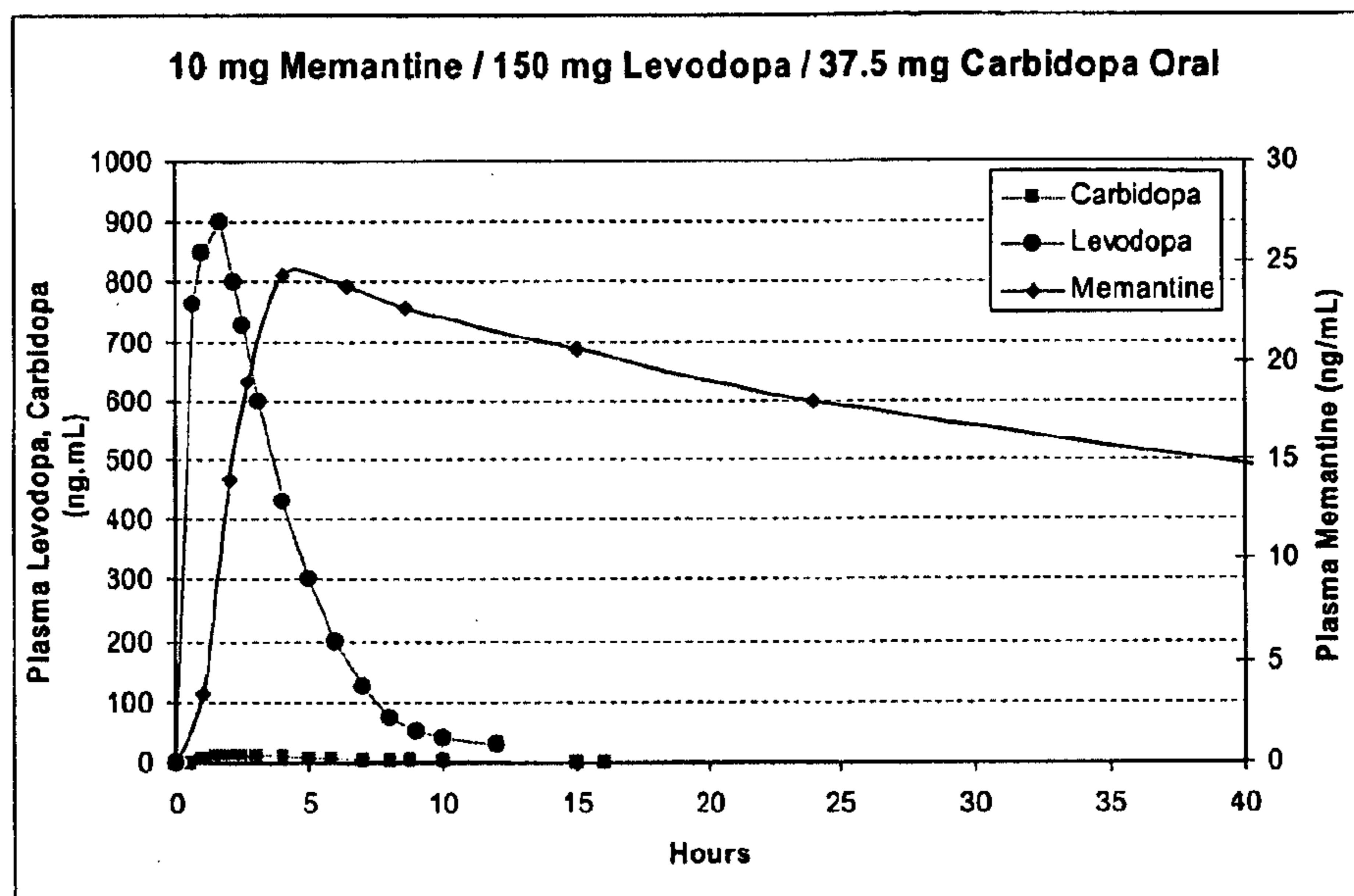
Figure 7: Target Pharmacokinetics
