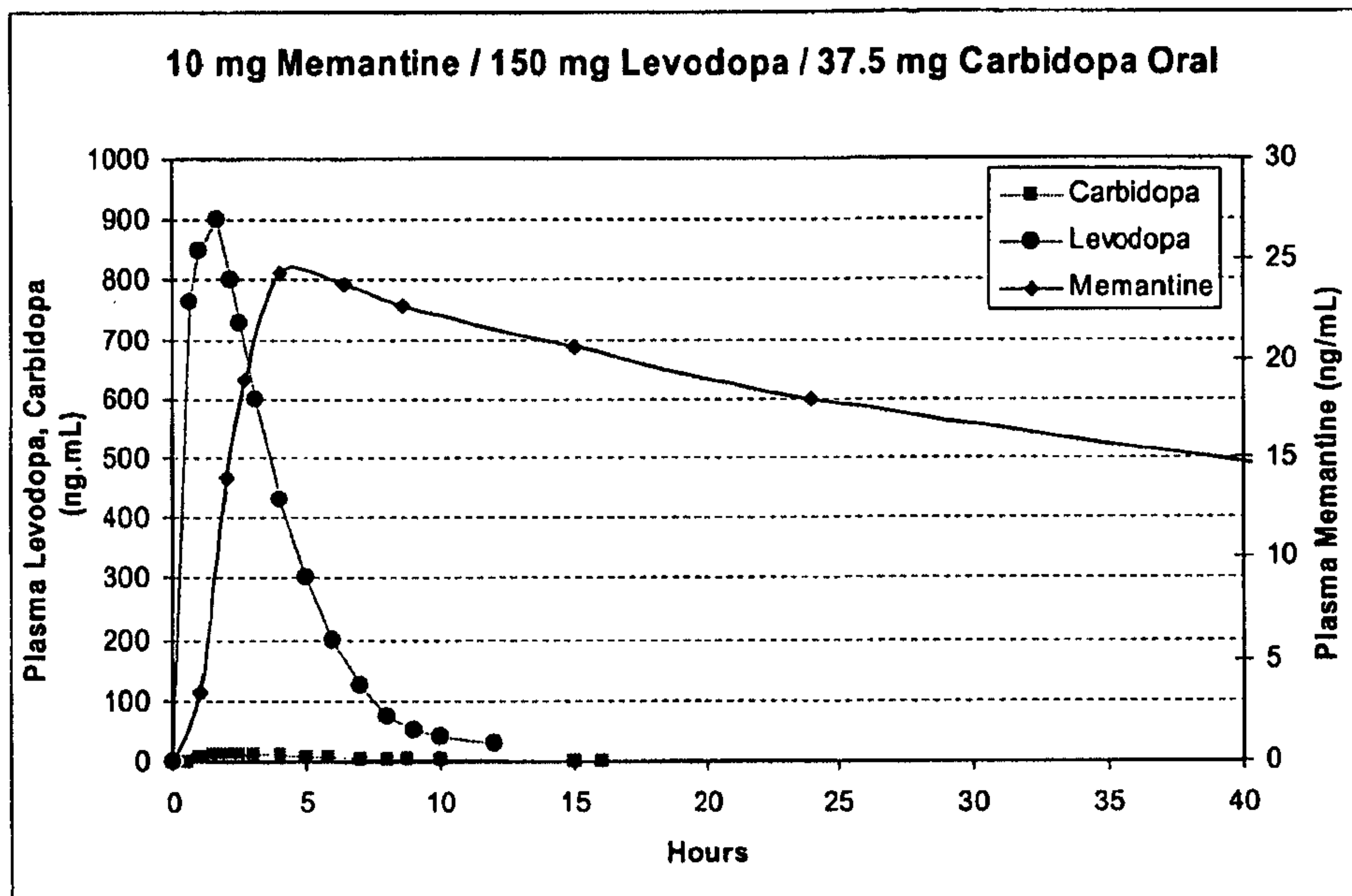
Figure 7: Target Pharmacokinetics
