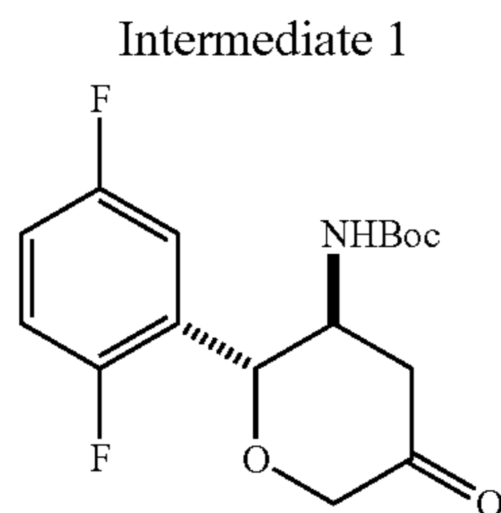
tert-Butyl [(2R,3S)-5-oxo-2-(2,5-difluorophenyl)tetrahydro-2H-pyran-3-yl]carbamate
