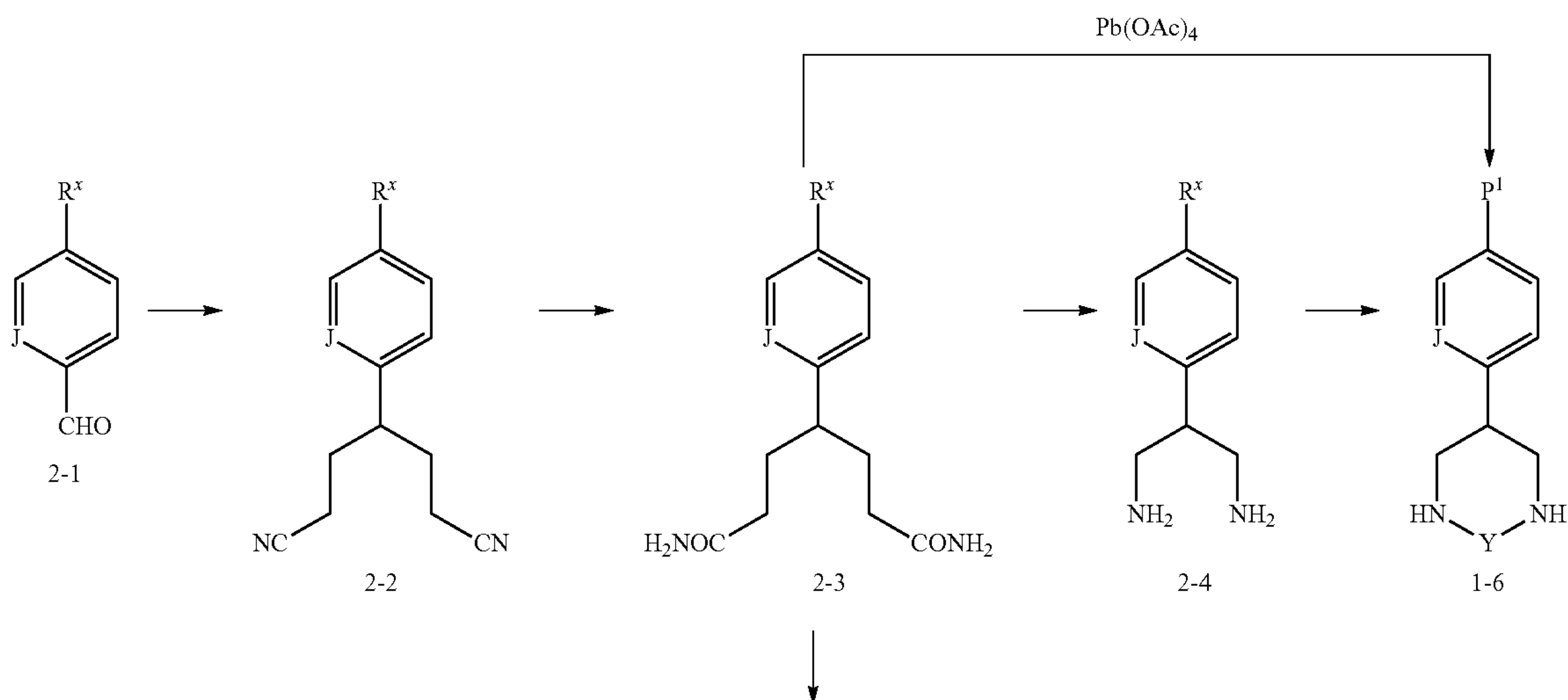
Scheme 2
