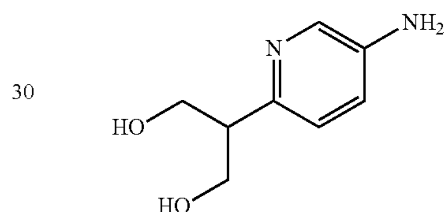
b) 2-(5-Amino-pyridin-2-yl)-propane-1,3-diol
