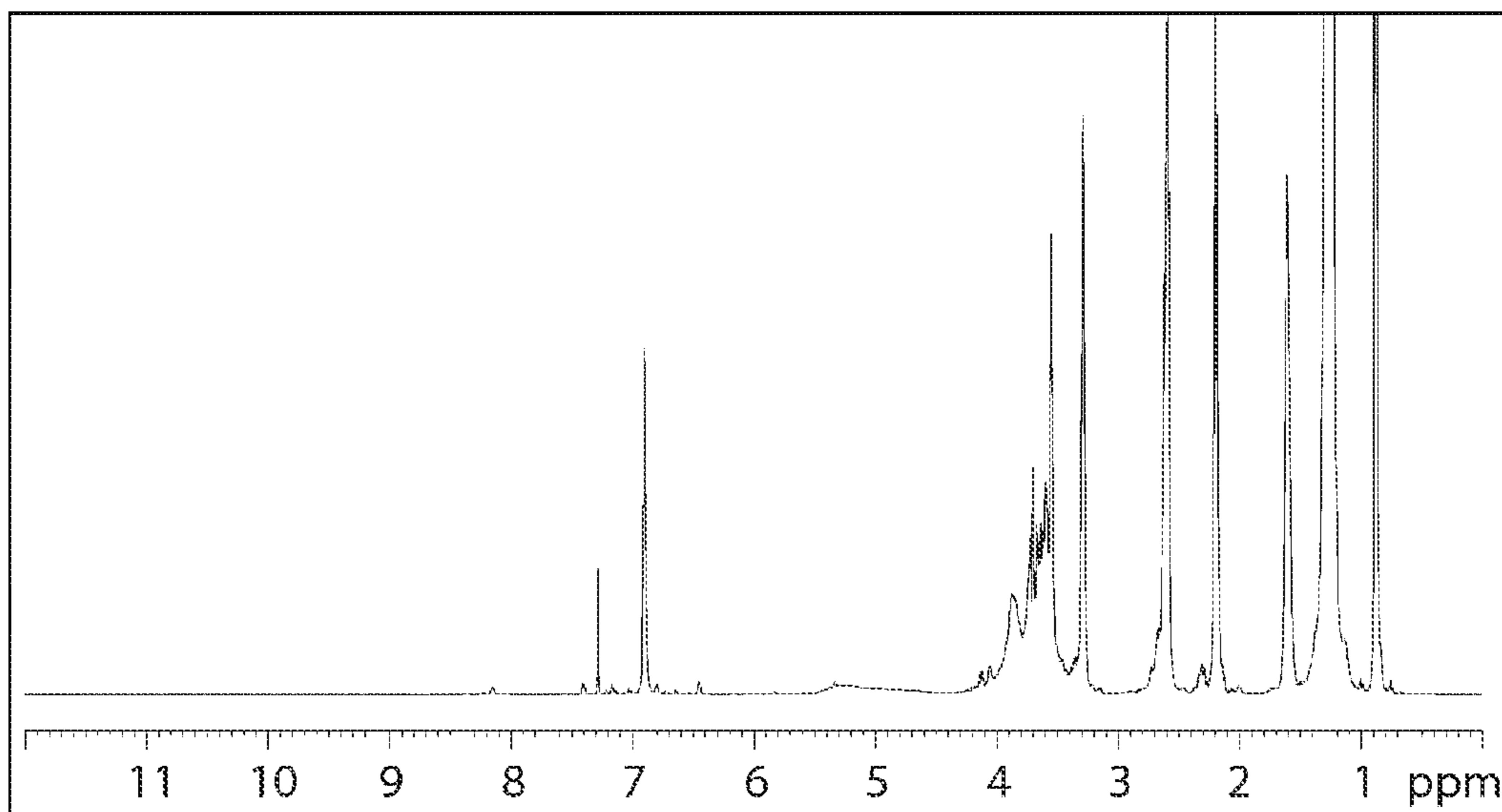
1 H NMR spectrum of Varisoft 510
