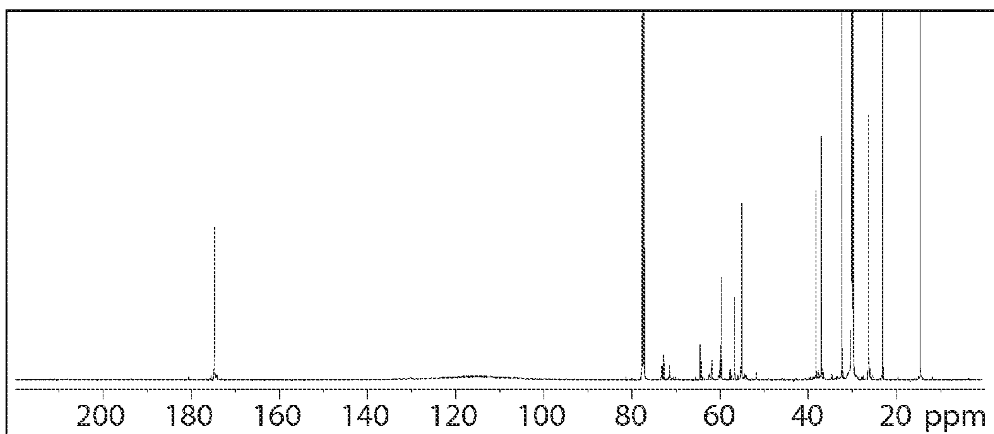
13 C NMR spectrum of Varisoft 510
