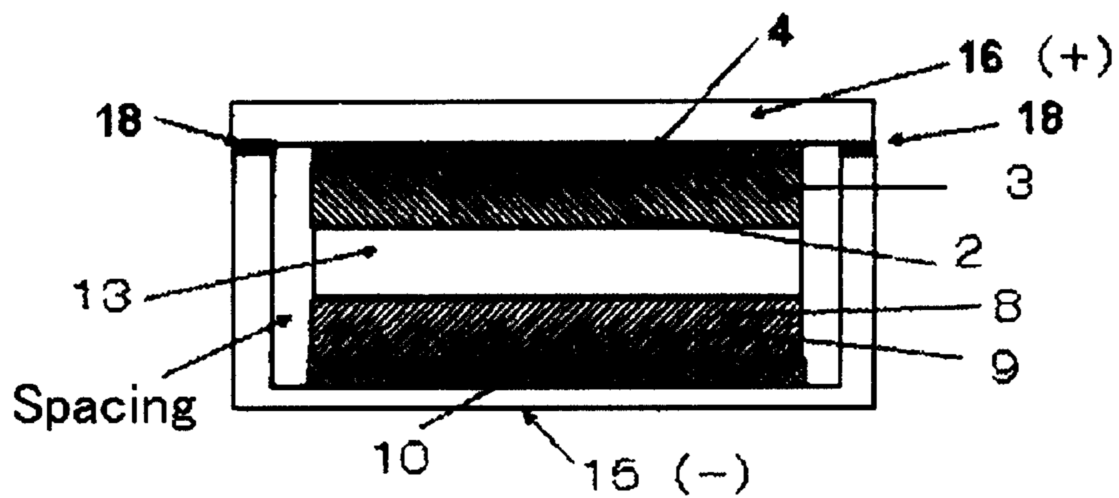
Vertical section view of all-solid lithium secondary battery of conventional type
