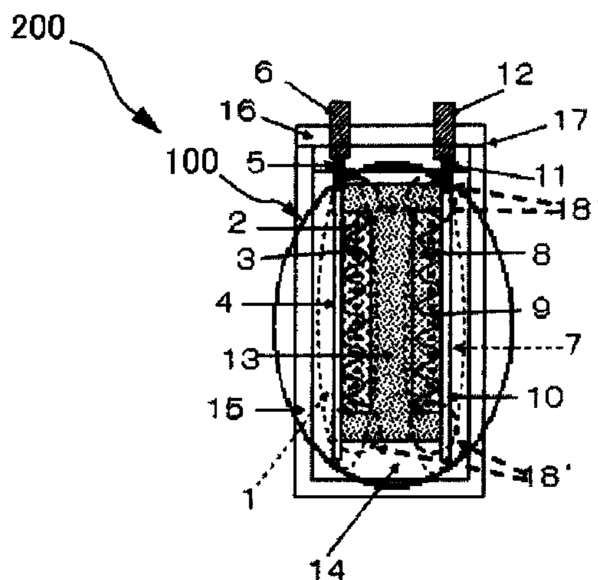
Battery device of present invention
