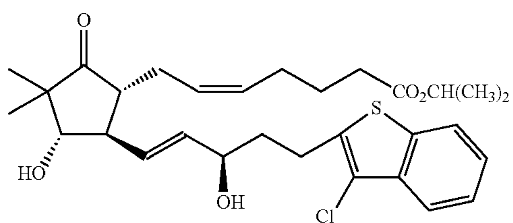
Compound 2
