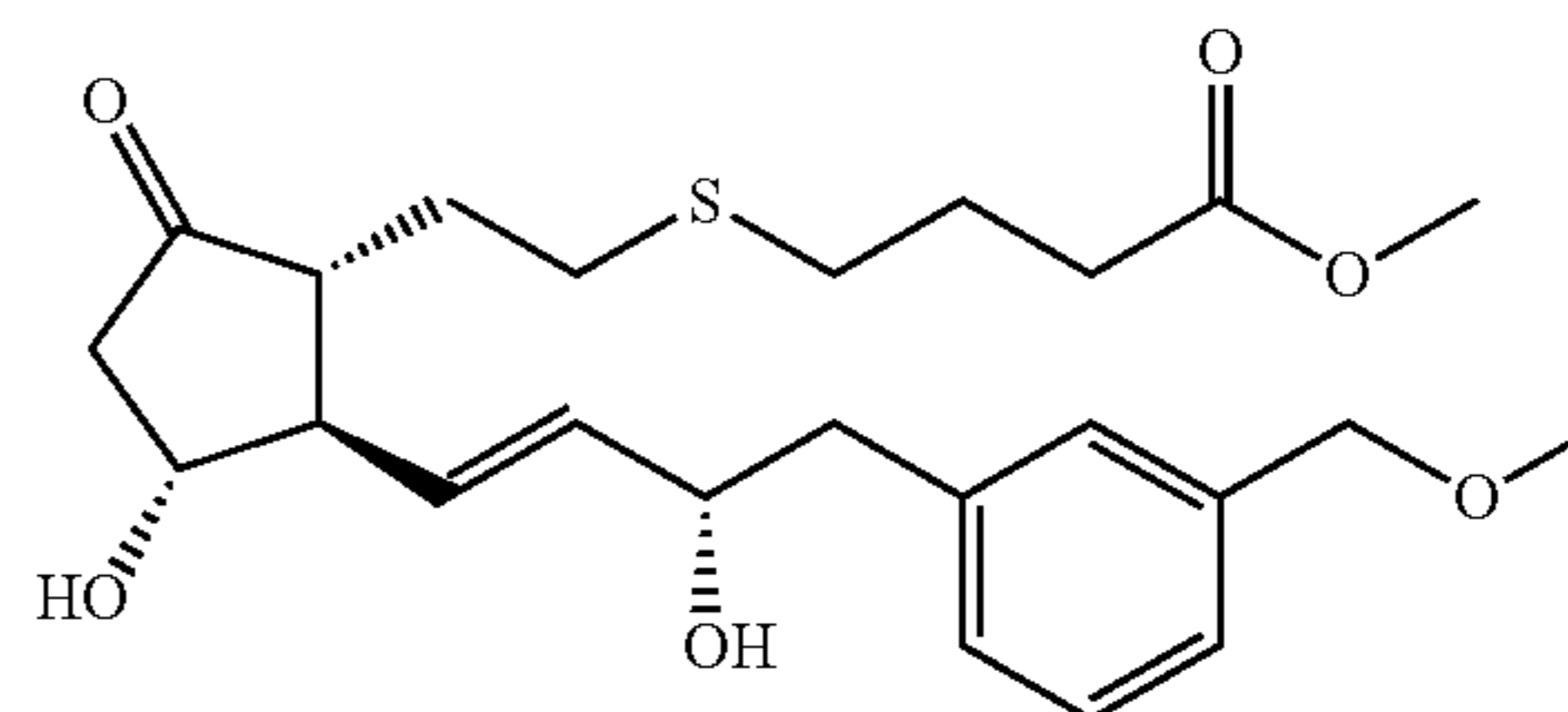
Compound 6
