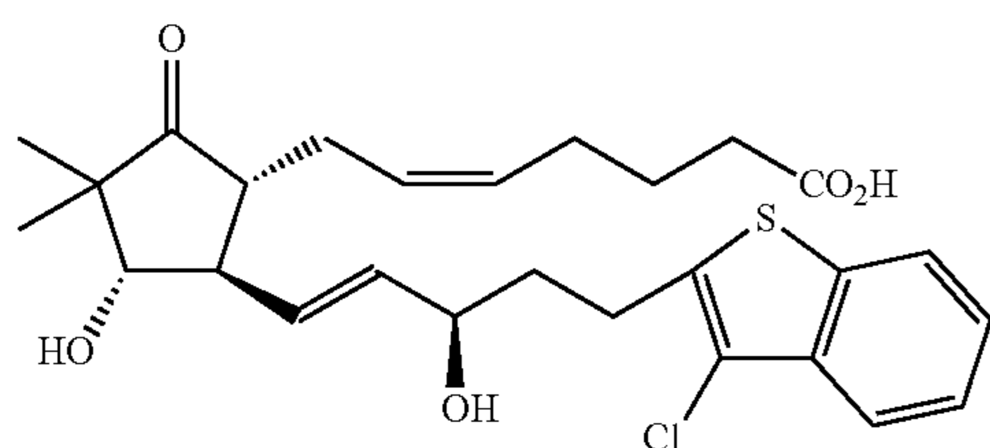
Compound 1
