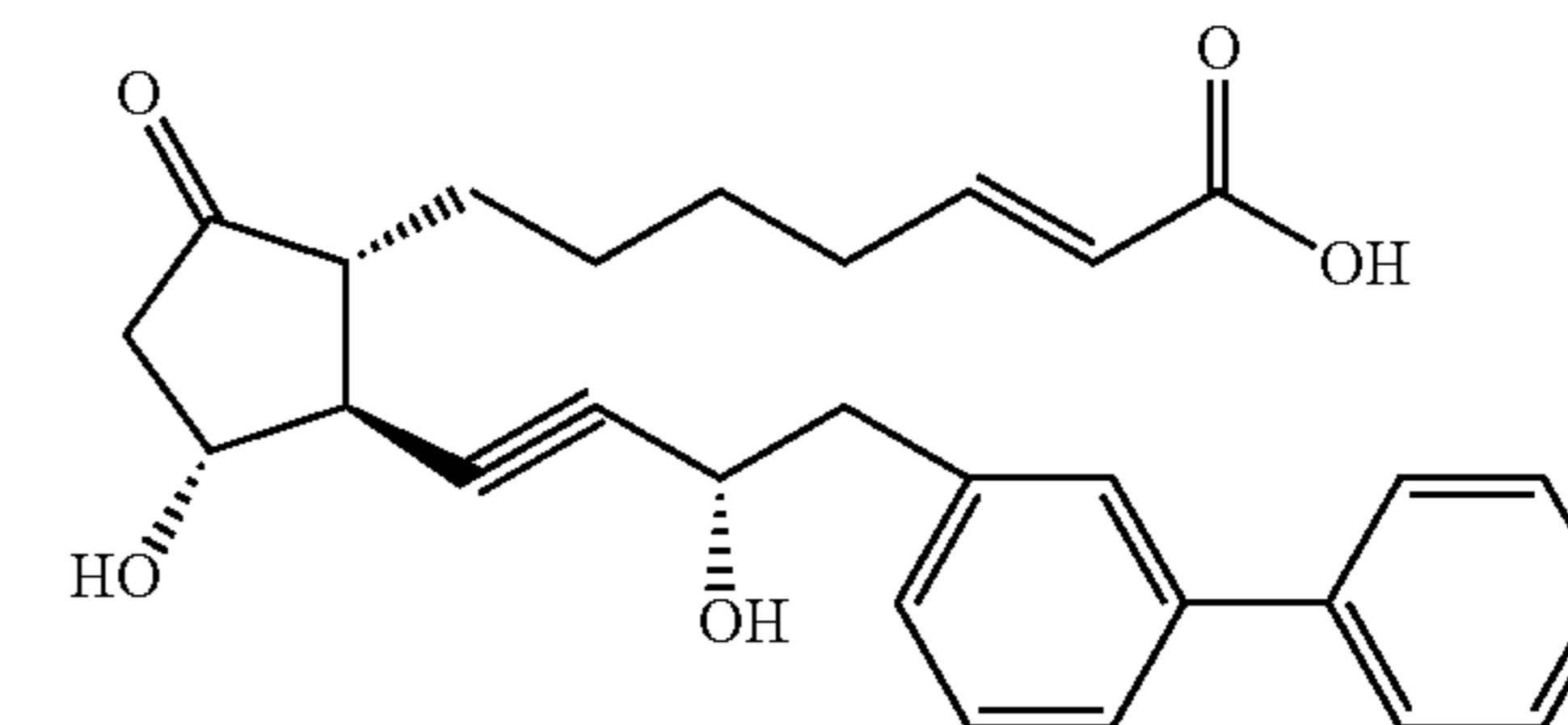
Compound 11
