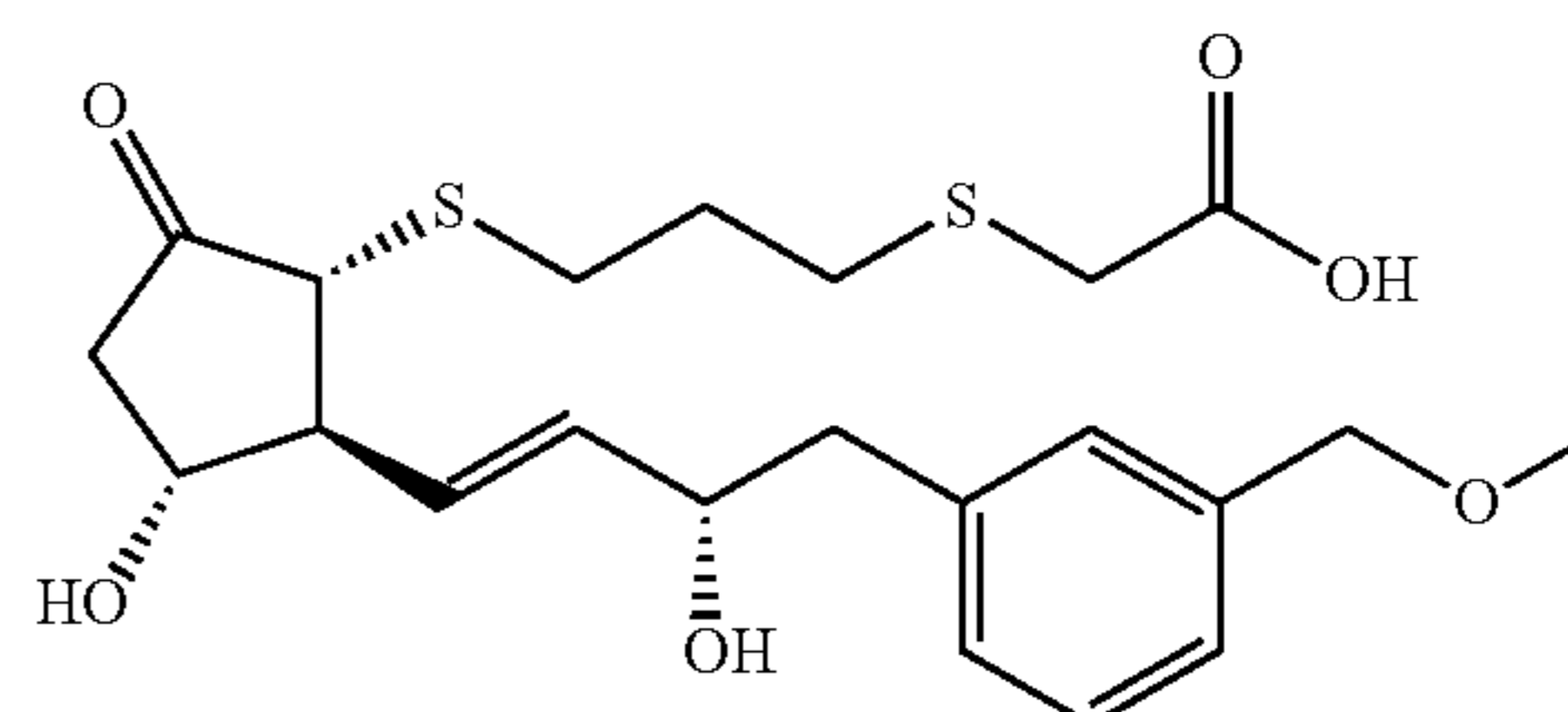
Compound 8
