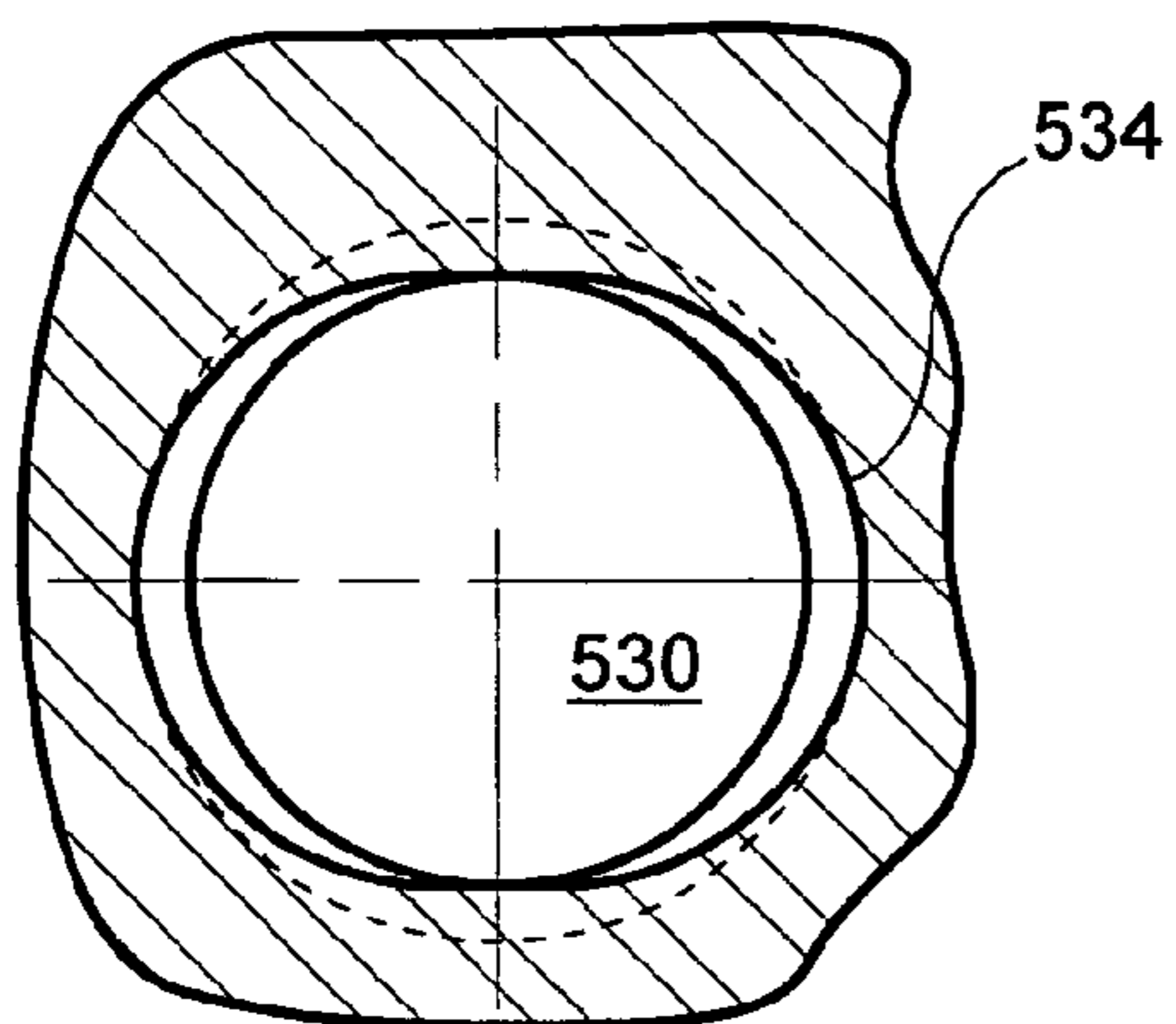
(Section D-D of Figure 7A) Figure 7D
