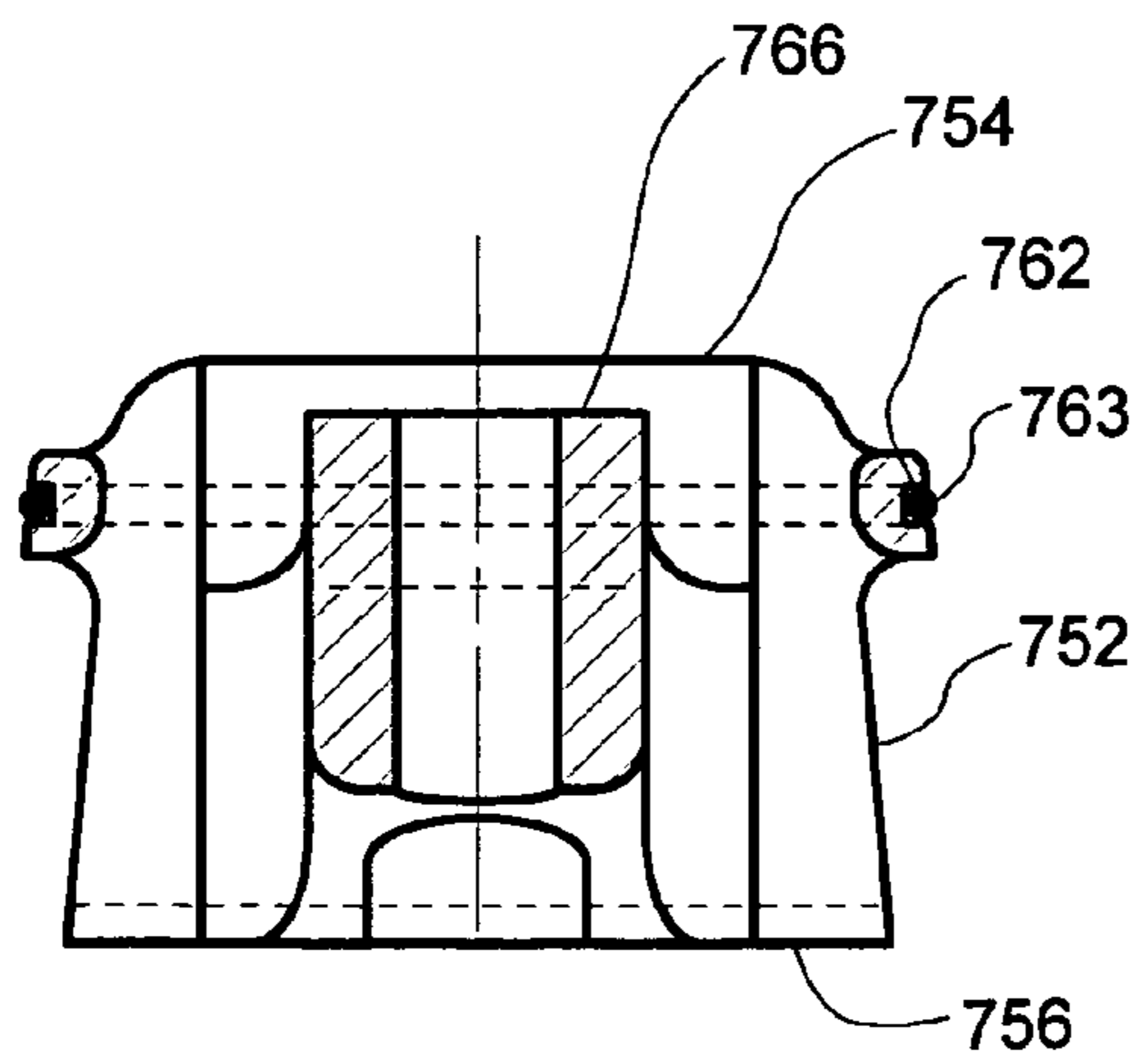
(Section C-C of Figure 12A)
