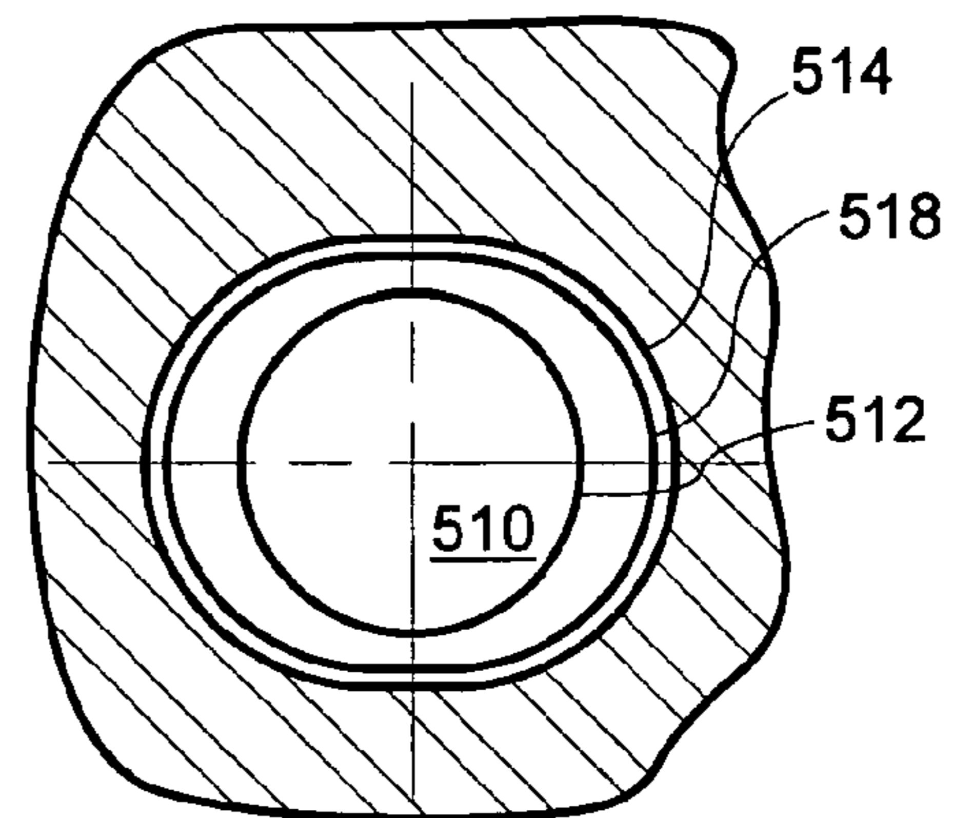
(Section E-E of Figure 7A) Figure 7E
