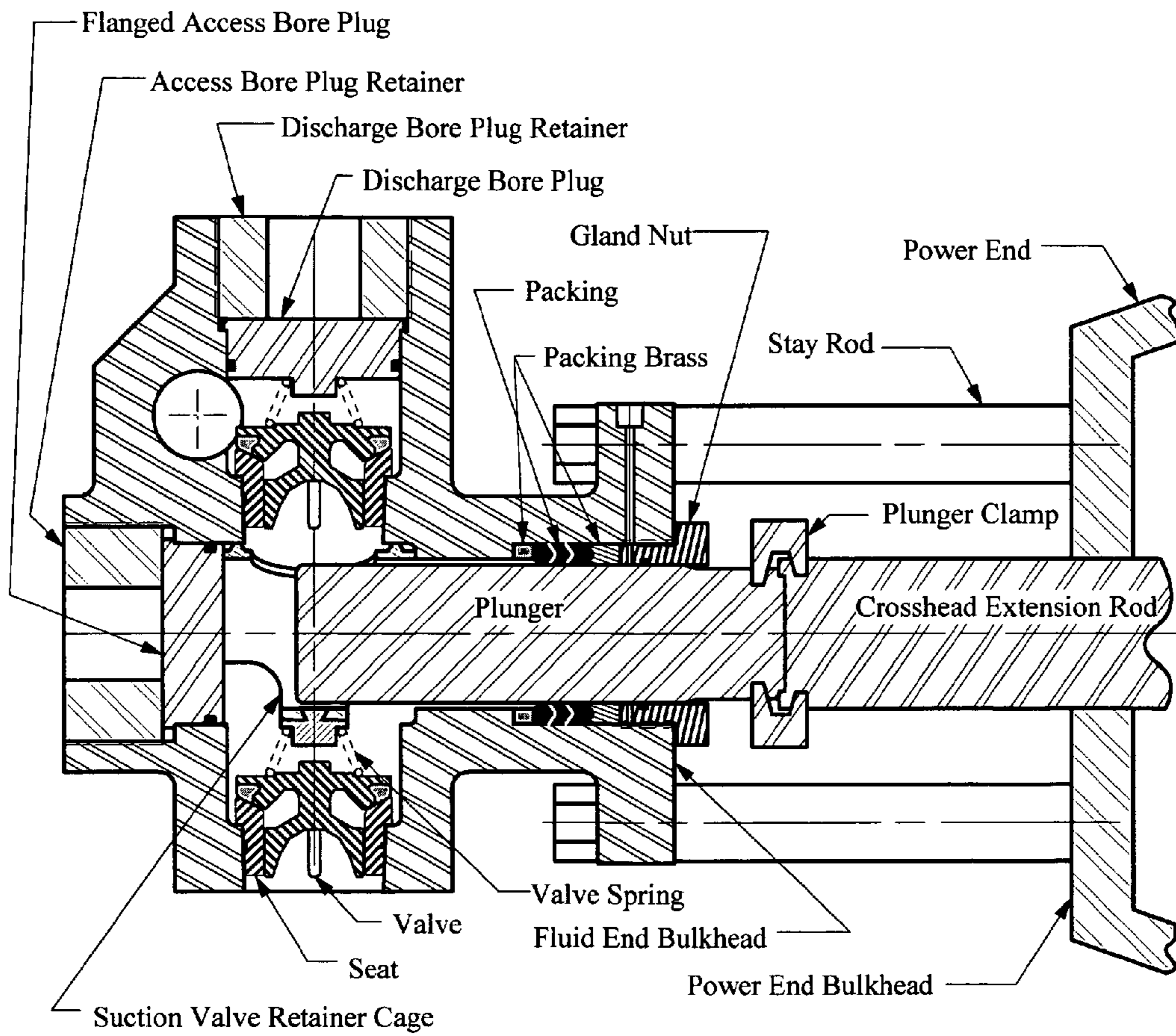
Typical Fluid Section Figure 1
