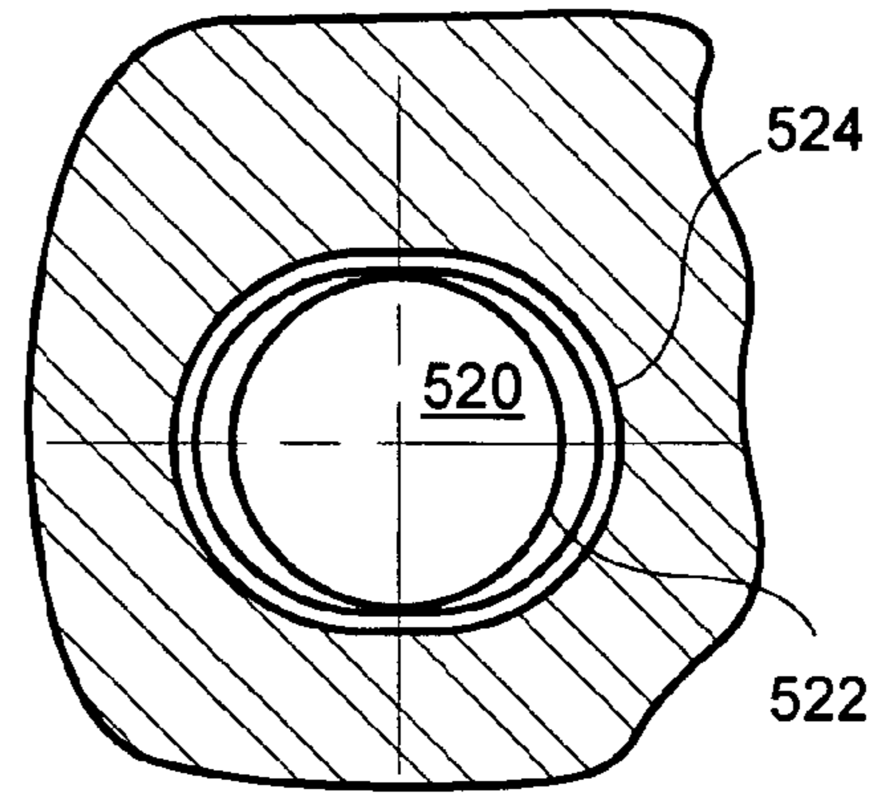
(Section C-C of Figure 7A) Figure 7C
