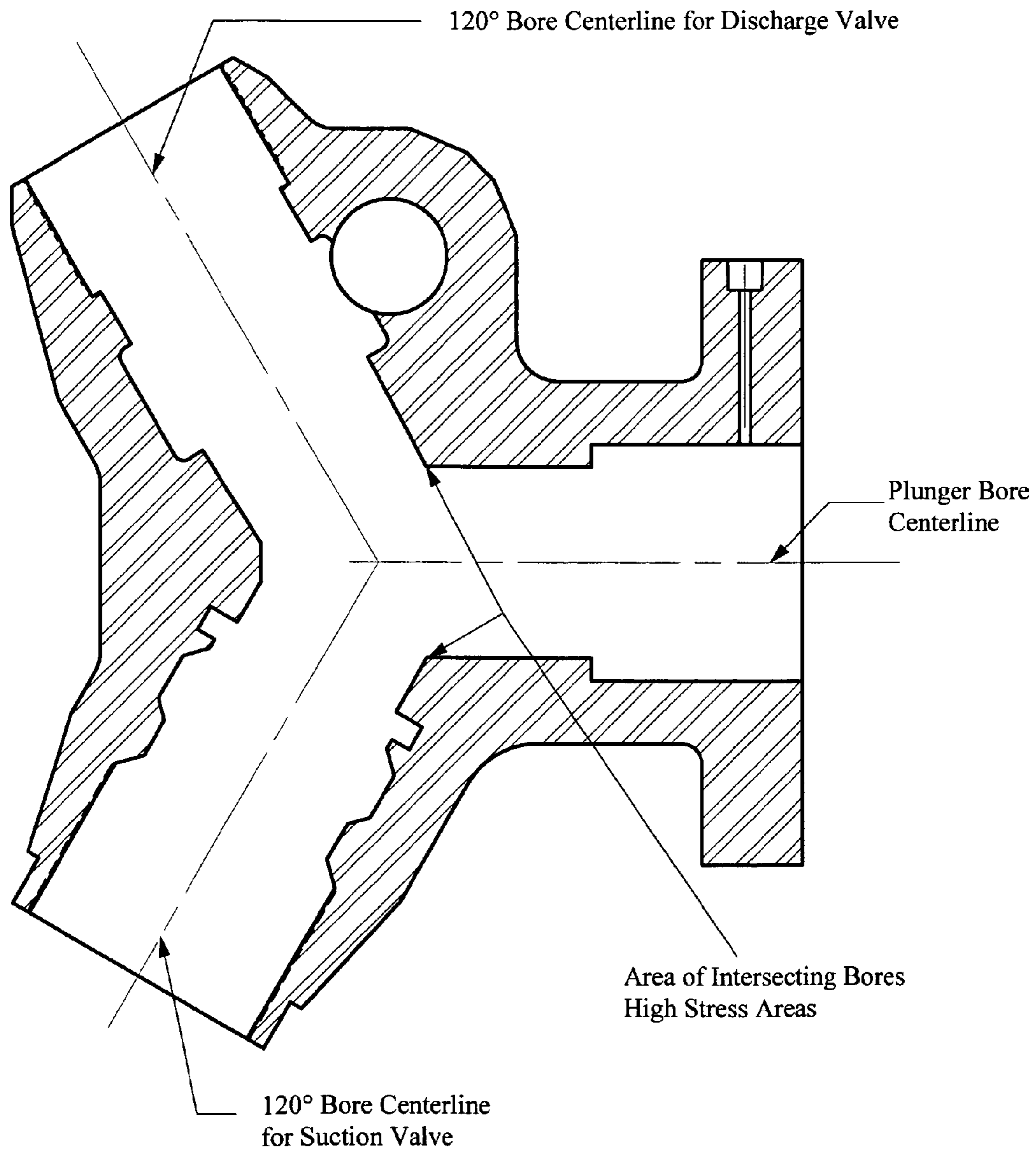
Y-Block Plunger Pump Housing
