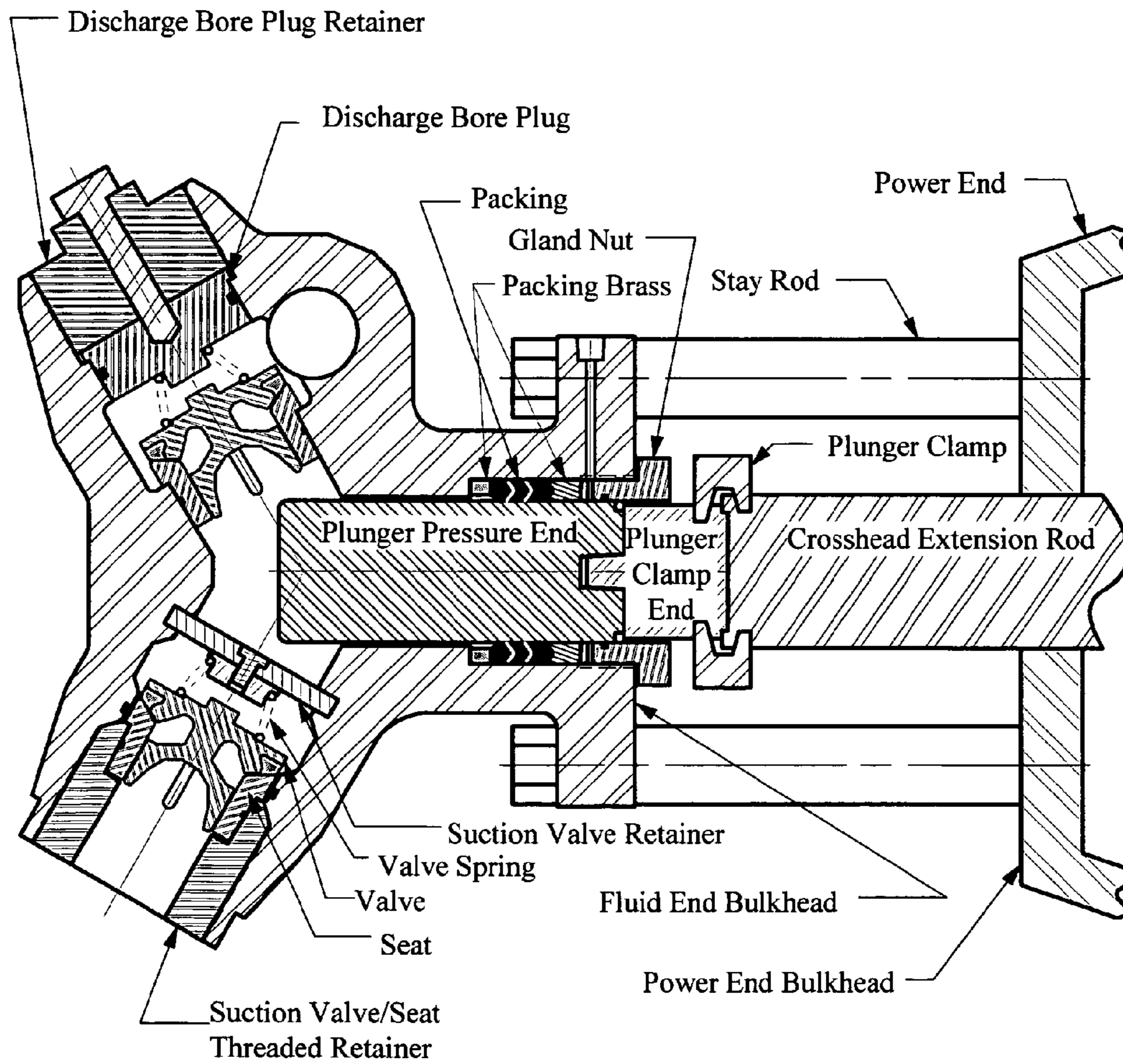
Y-Block Fluid Section
