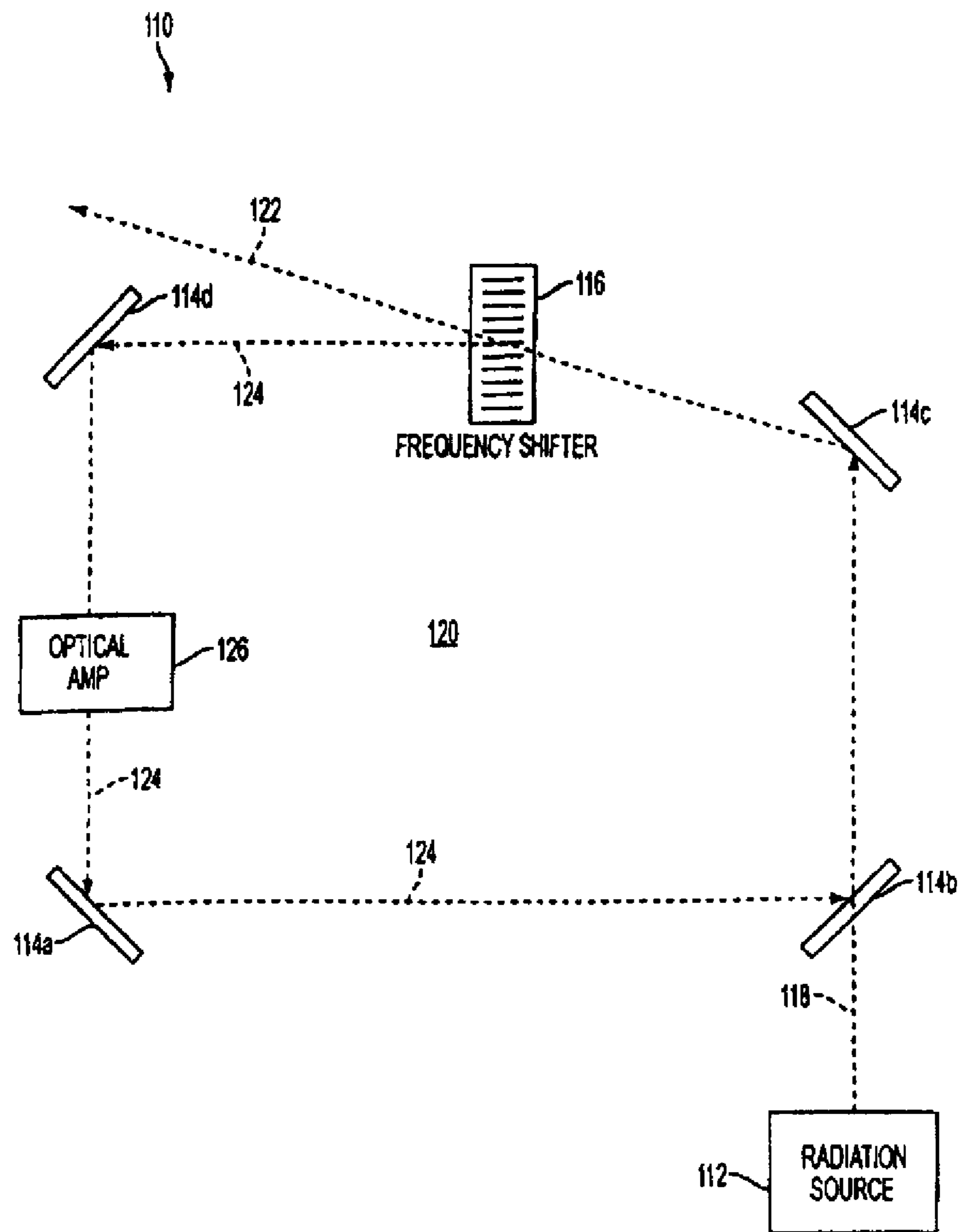
FIG. 1 (PRIOR ART)
