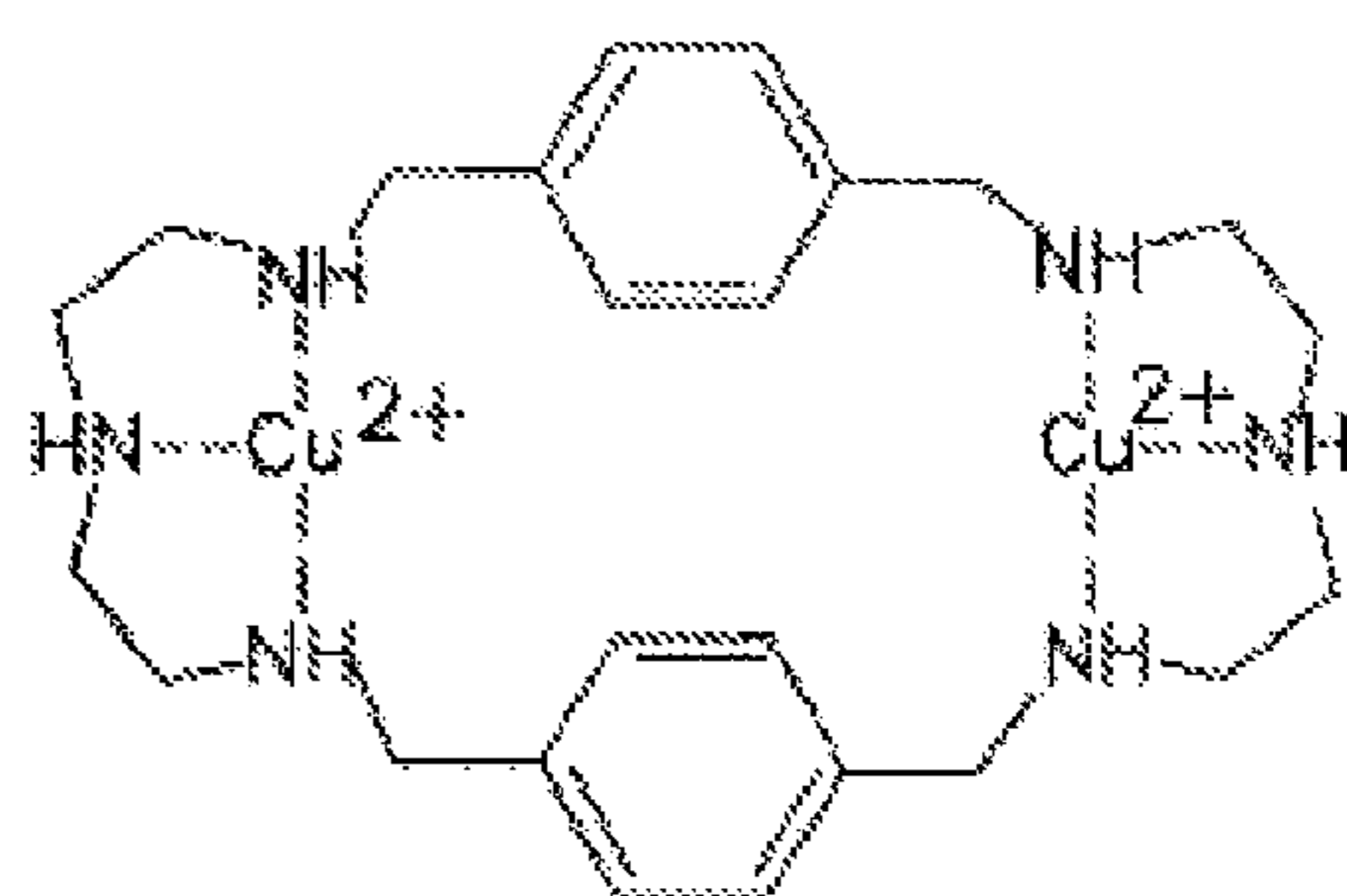
Compound 4
