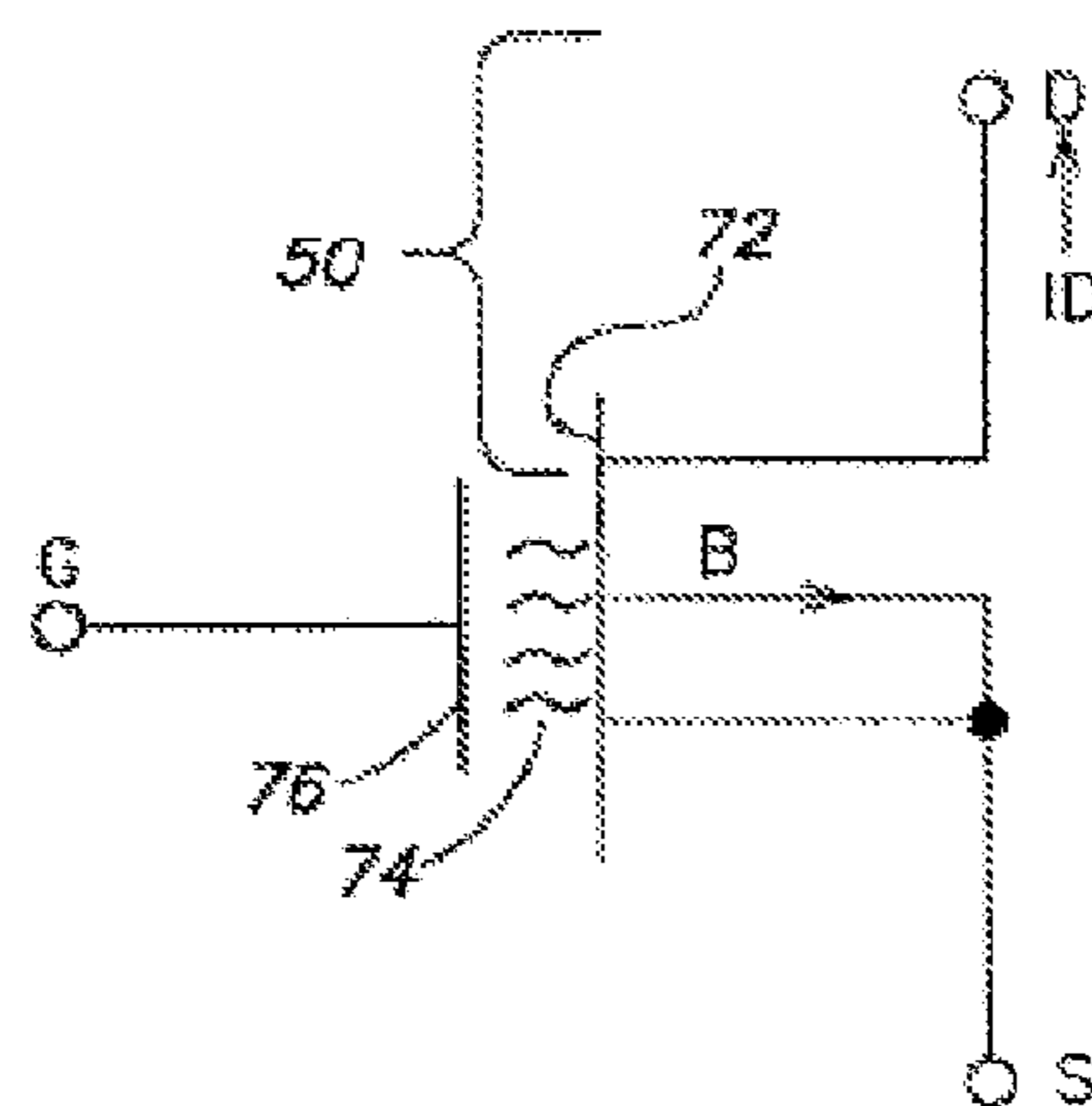
FIG. 2 (Prior Art)
