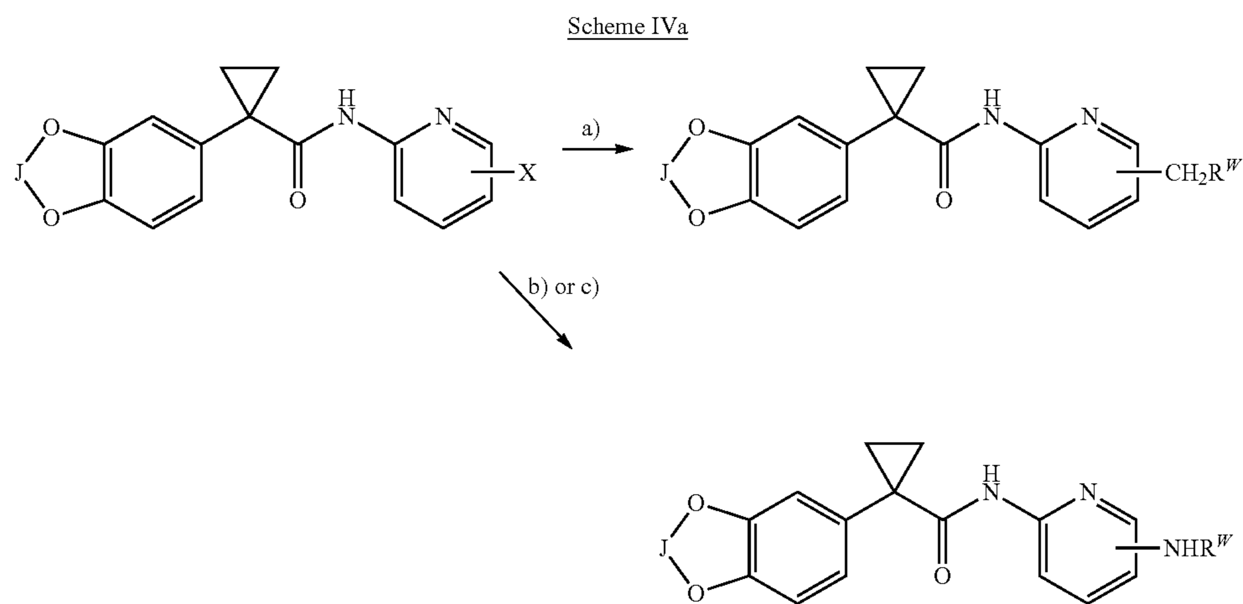
Scheme IV. Derivatization of Amides
