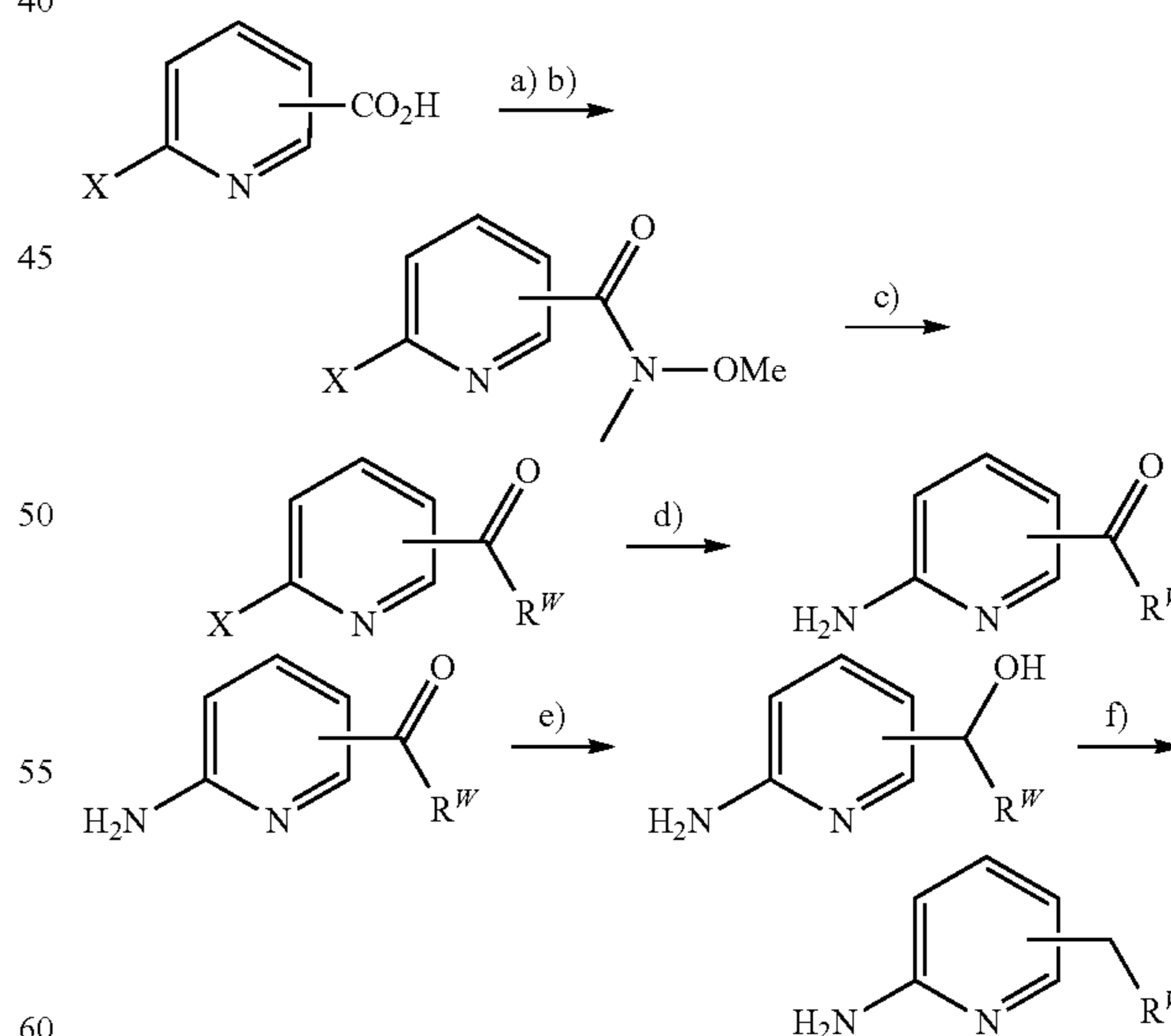
Scheme II. Preparation of amino pyridyl building blocks
