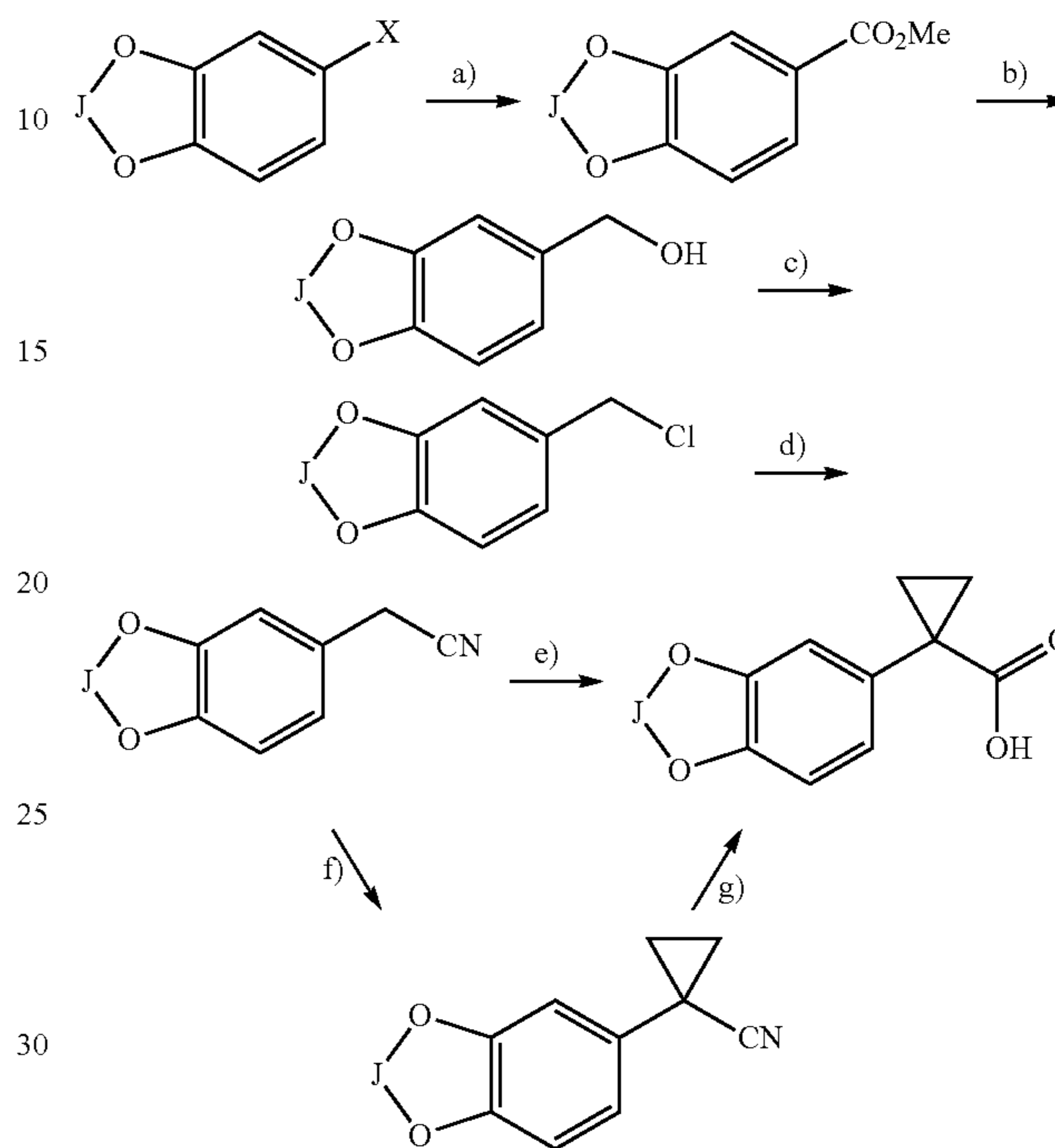
Scheme I. Preparation of cyclopropyl acids
