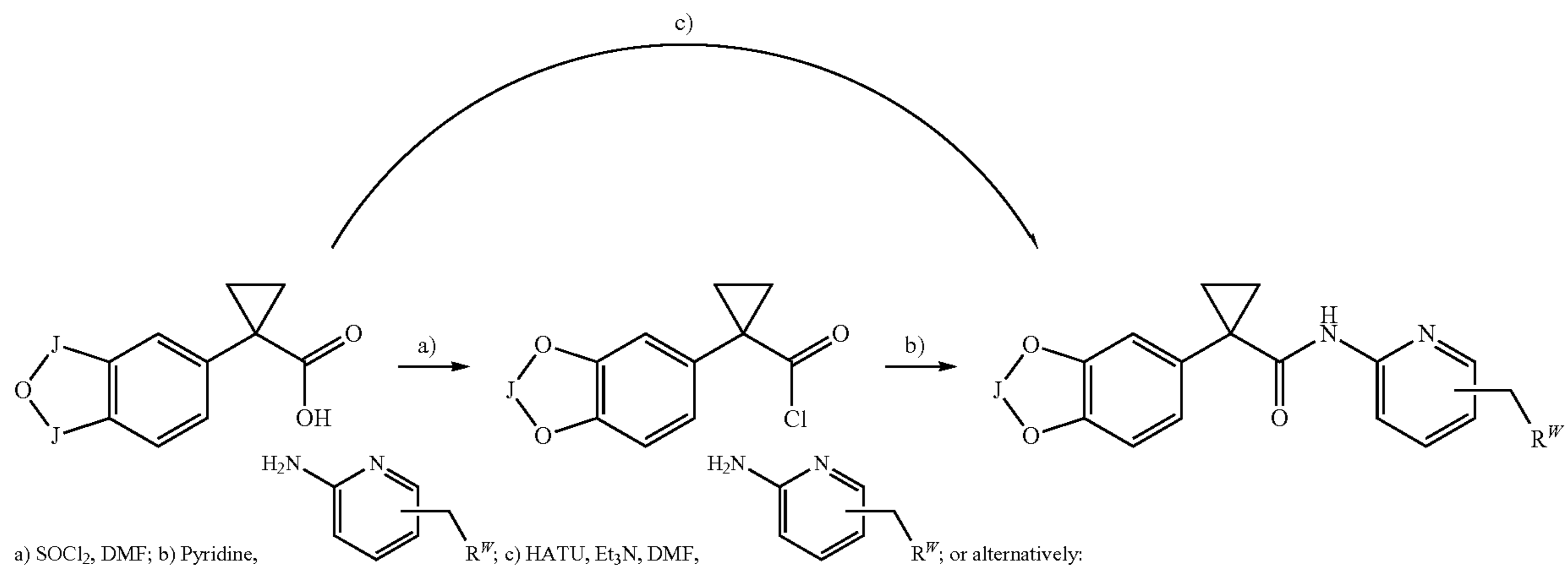
Scheme III. Amide coupling
