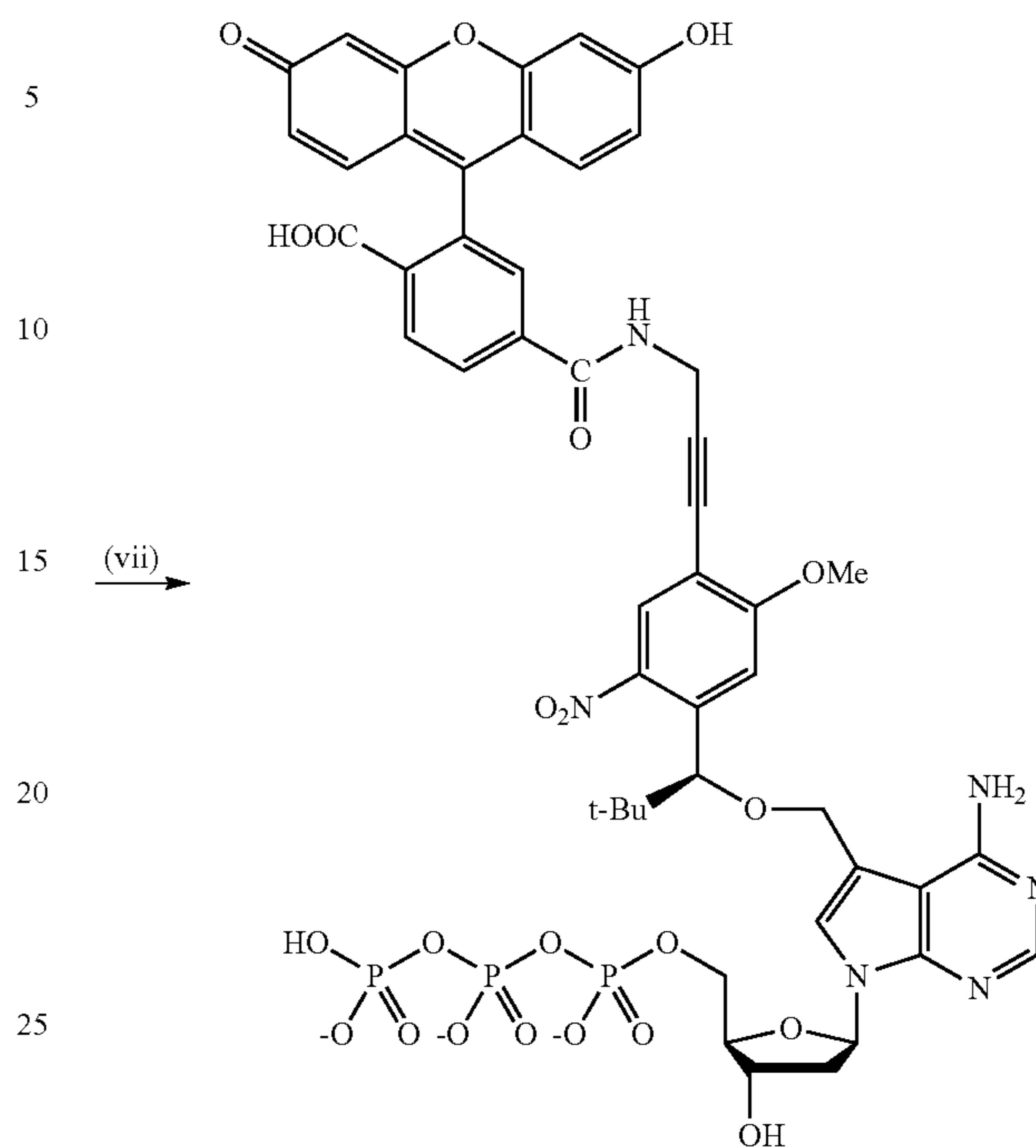
Scheme 2c.
