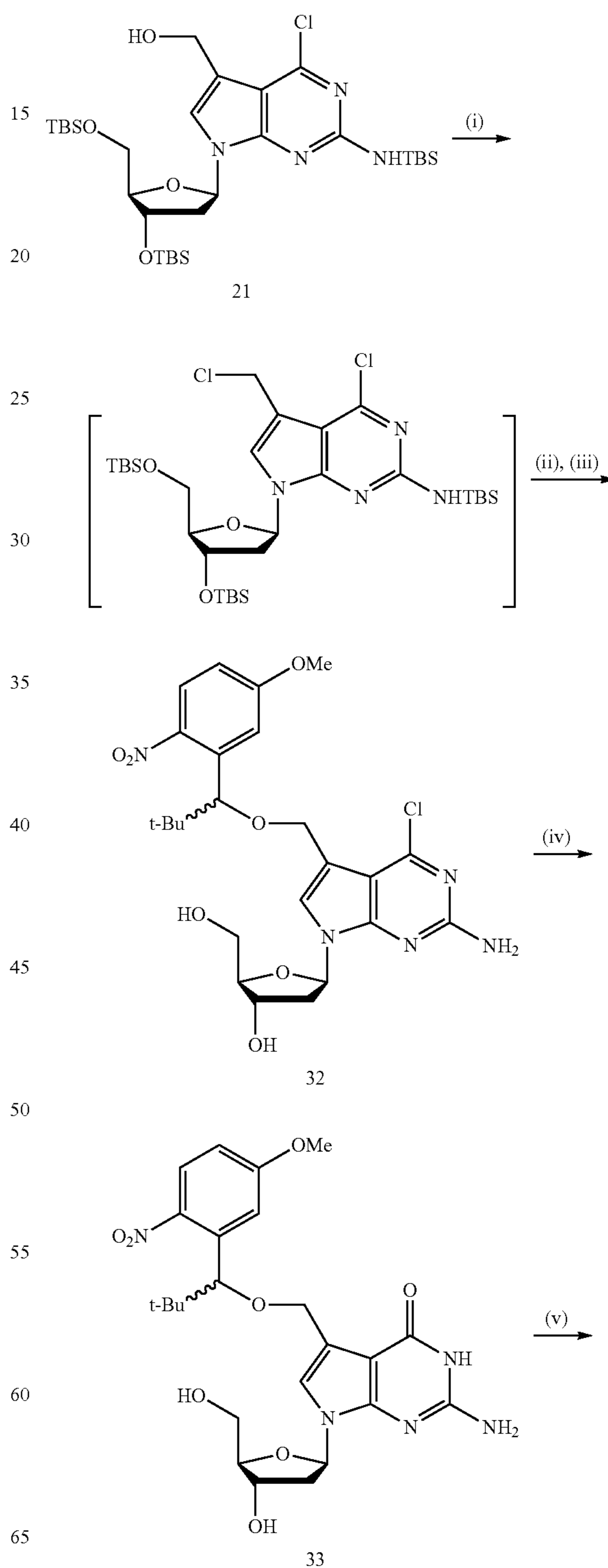
Scheme S16. Synthesis of 7-[1-(5-methoxy-2-nitrophenyl)-2,2-dimethyl-propyloxy]methyl-7-deaza-2'-deoxyguanosine-5'-triphosphate.
