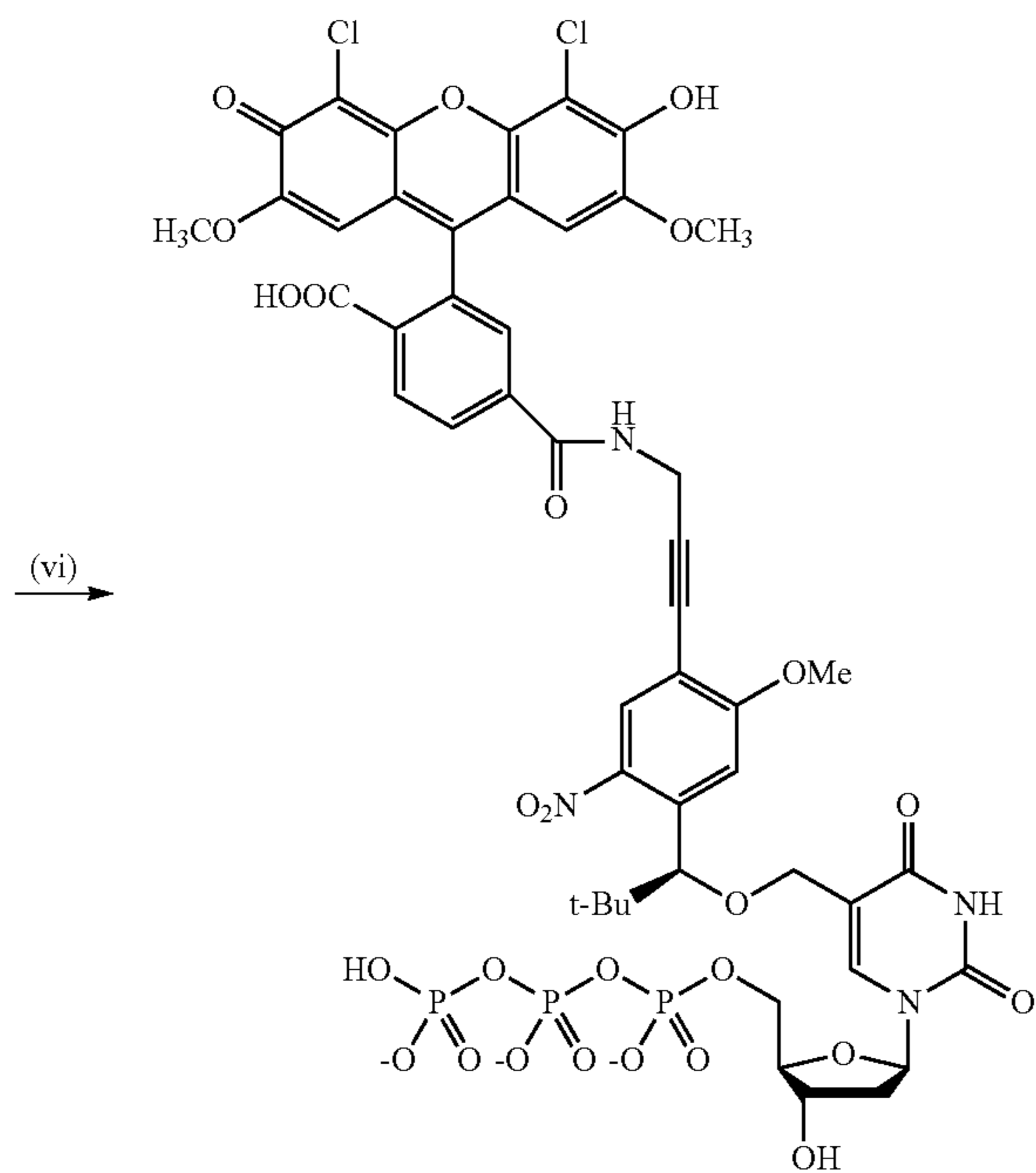
Scheme 3c.
