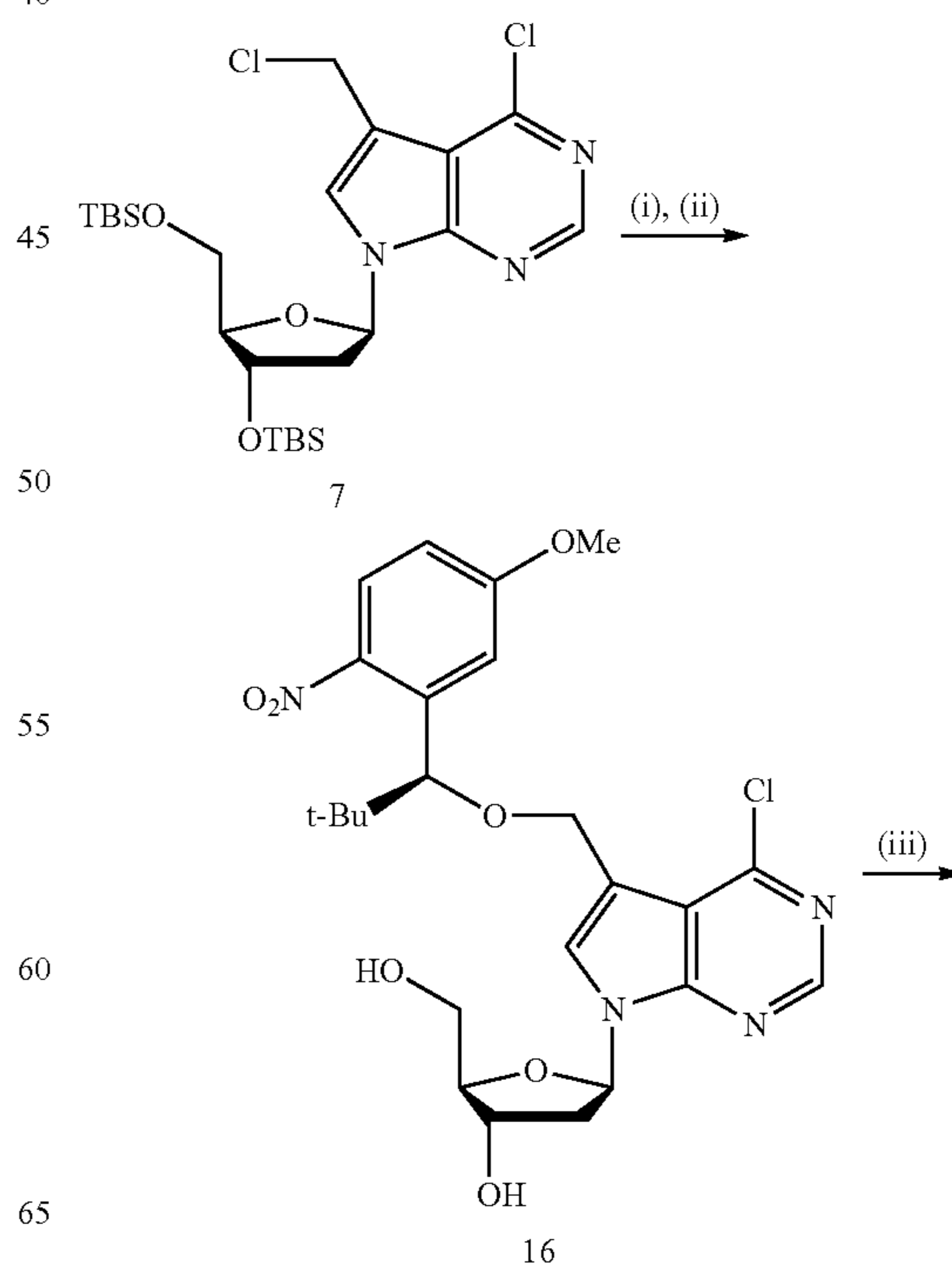
Scheme S11. Synthesis of 7-[(S)-1-(5-methoxy-2-nitrophenyl)-2,2-dimethyl-propyloxy]methyl-7-deaza-2'-deoxyadenosine-5'-triphosphate.
