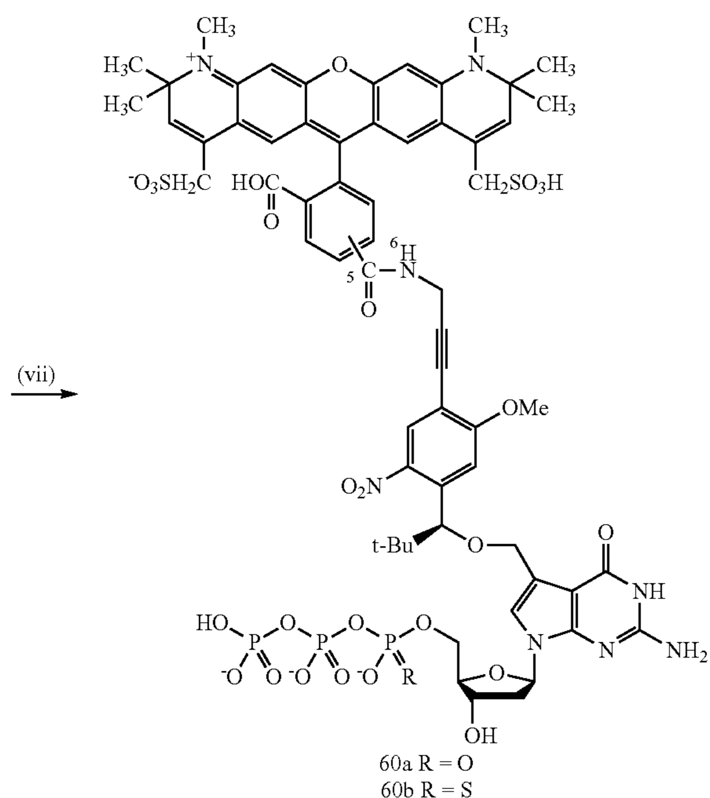
Scheme S26b.
