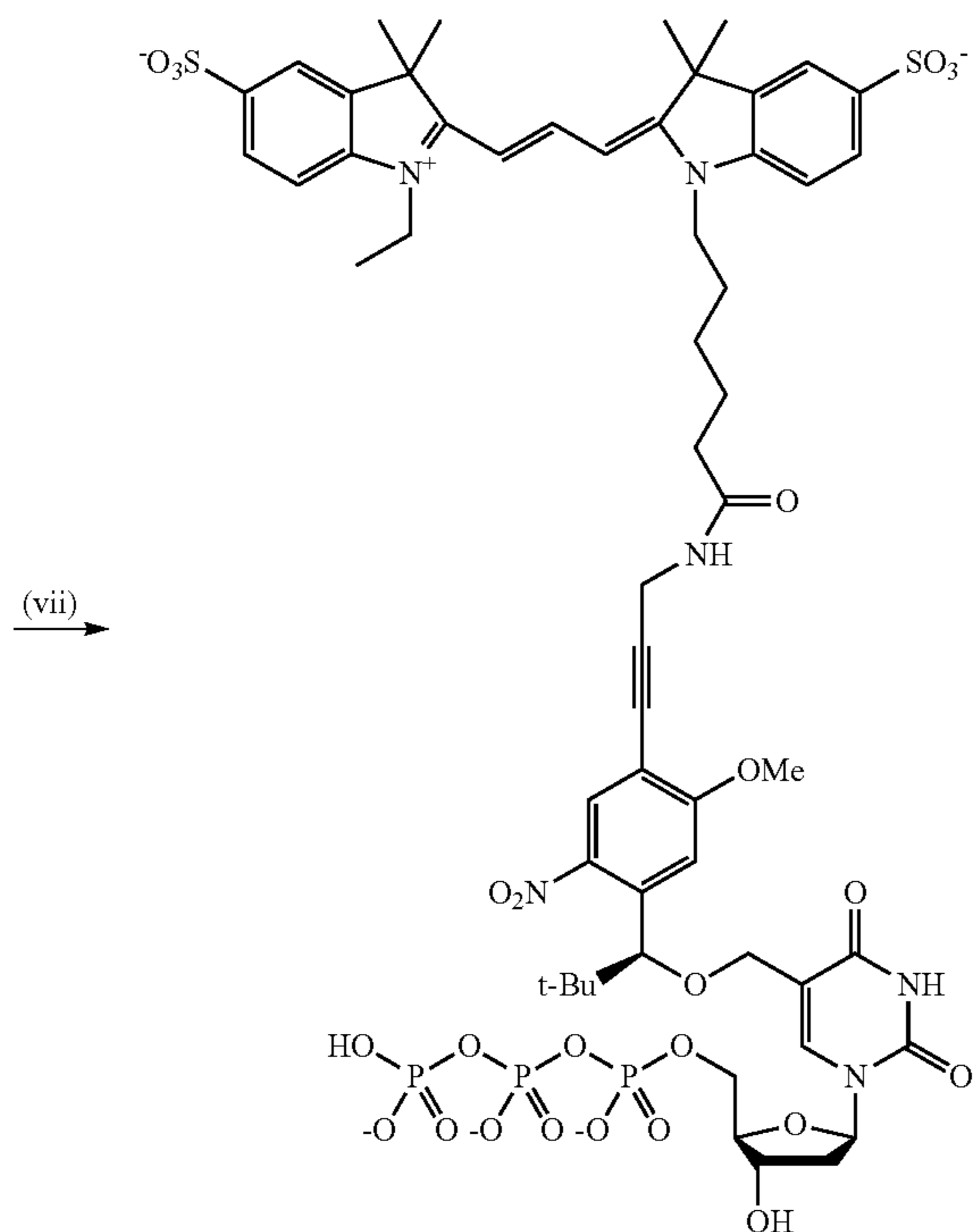
Scheme 3d.
