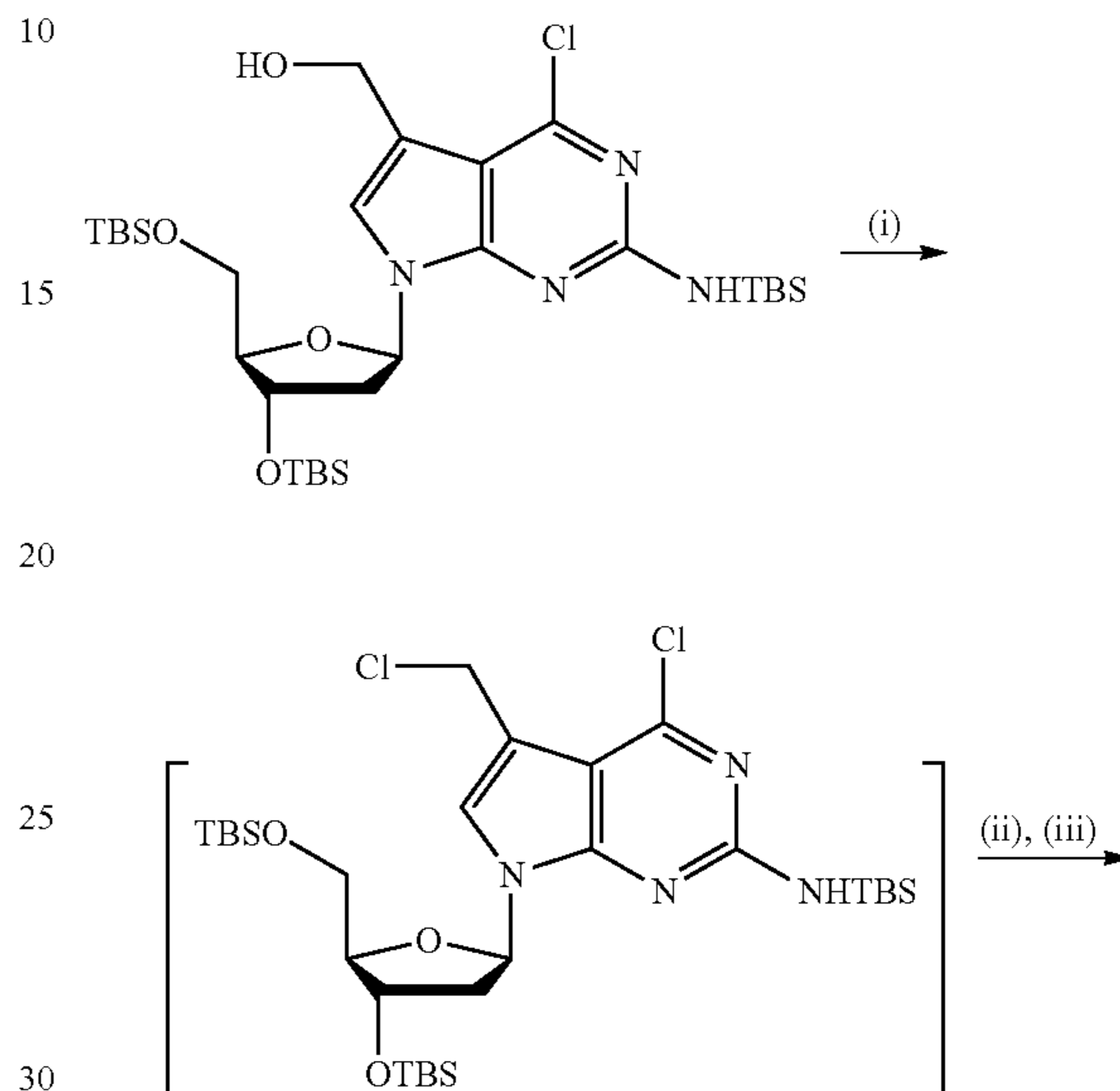
Scheme 4a. Synthesis of dye labeled 7-[(S)-1-(5-methoxy-2-nitrophenyl)-2,2-dimethyl-propyloxy]methyl-7-deaza-2'-deoxyguanosine-5'-triphosphate.
