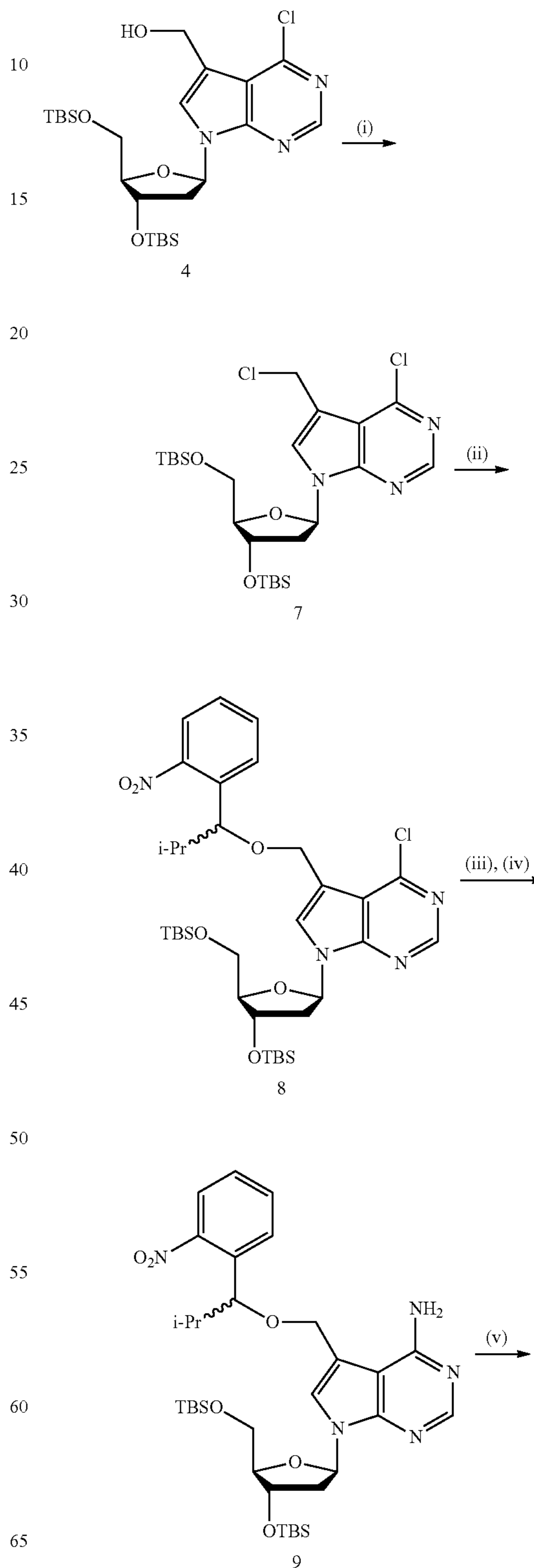
Scheme S7. Synthesis of 7-[1-(2-nitrophenyl)-2-methyl-propyloxy]methyl-7-deaza-2'-deoxyadenosine-5'-triphosphate.
