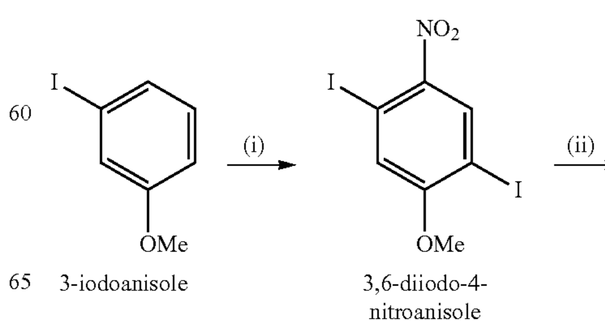
Scheme S24.
