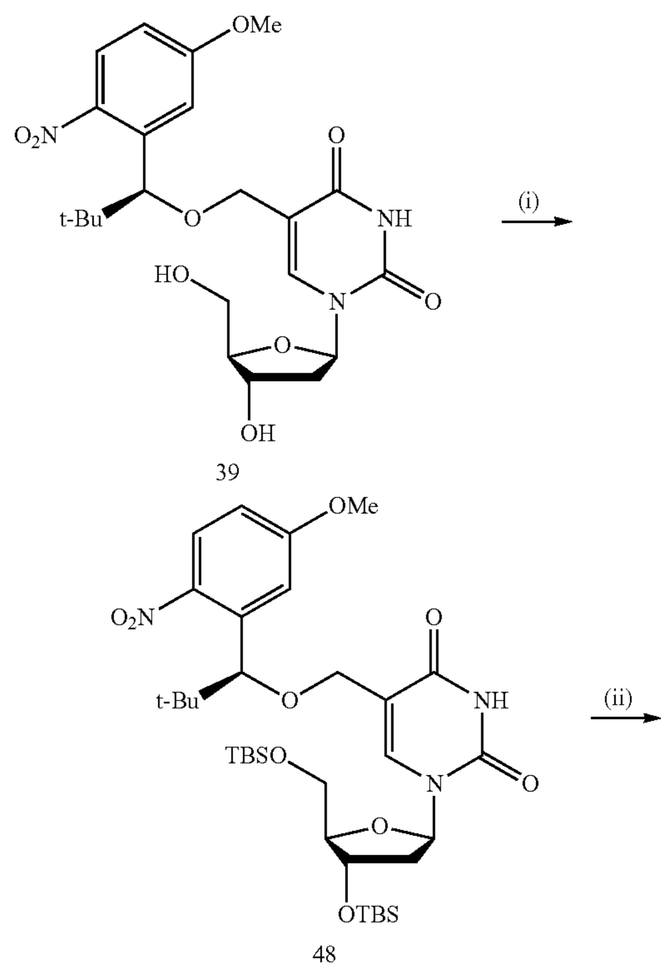
Scheme S22. Synthesis of 5-[(S)-1-(5-methoxy-2-nitrophenyl)-2,2-dimethyl-propyloxy]methyl-2'-deoxycytidine-5'-triphosphate.
