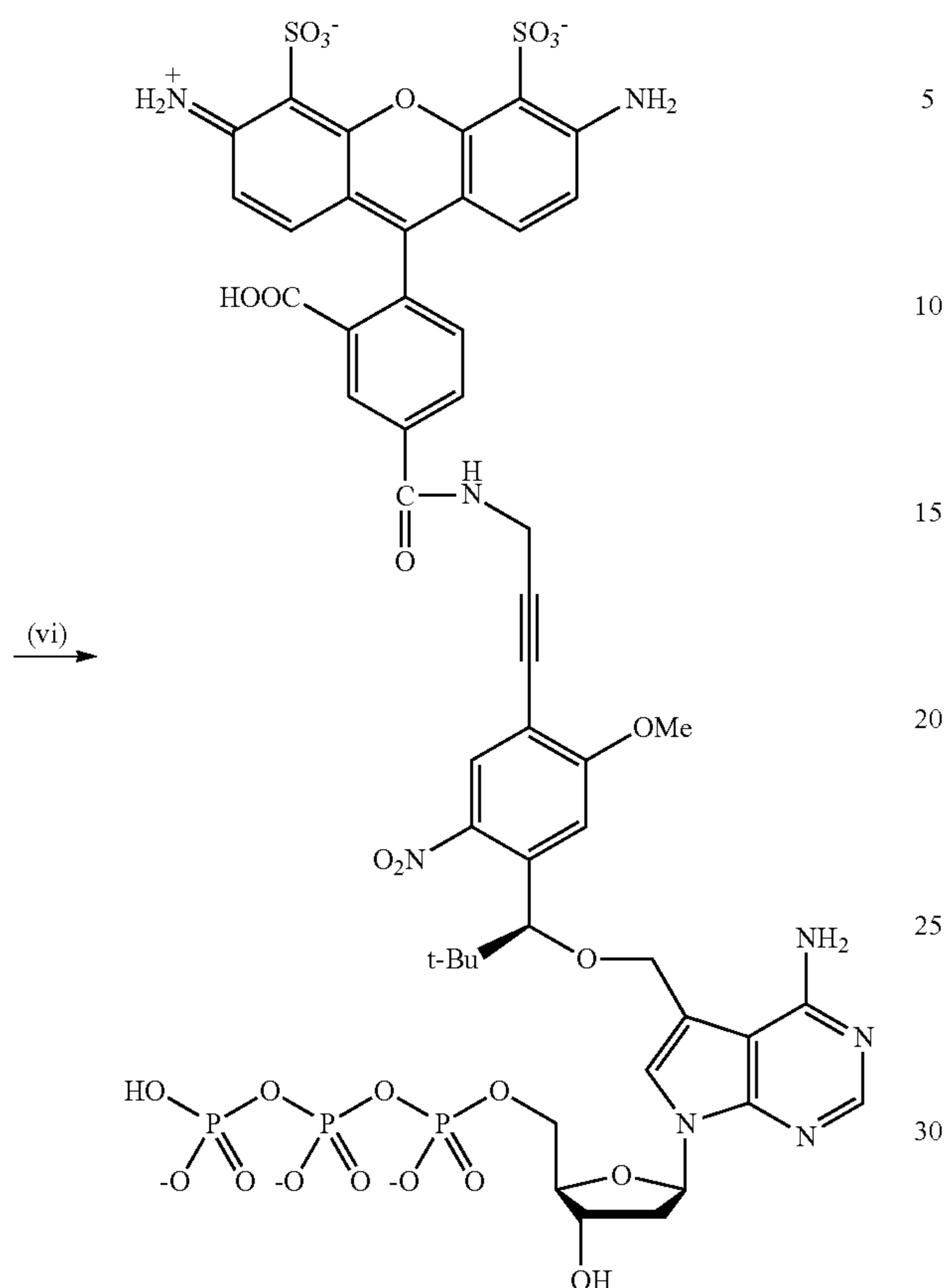
Scheme 2b.
