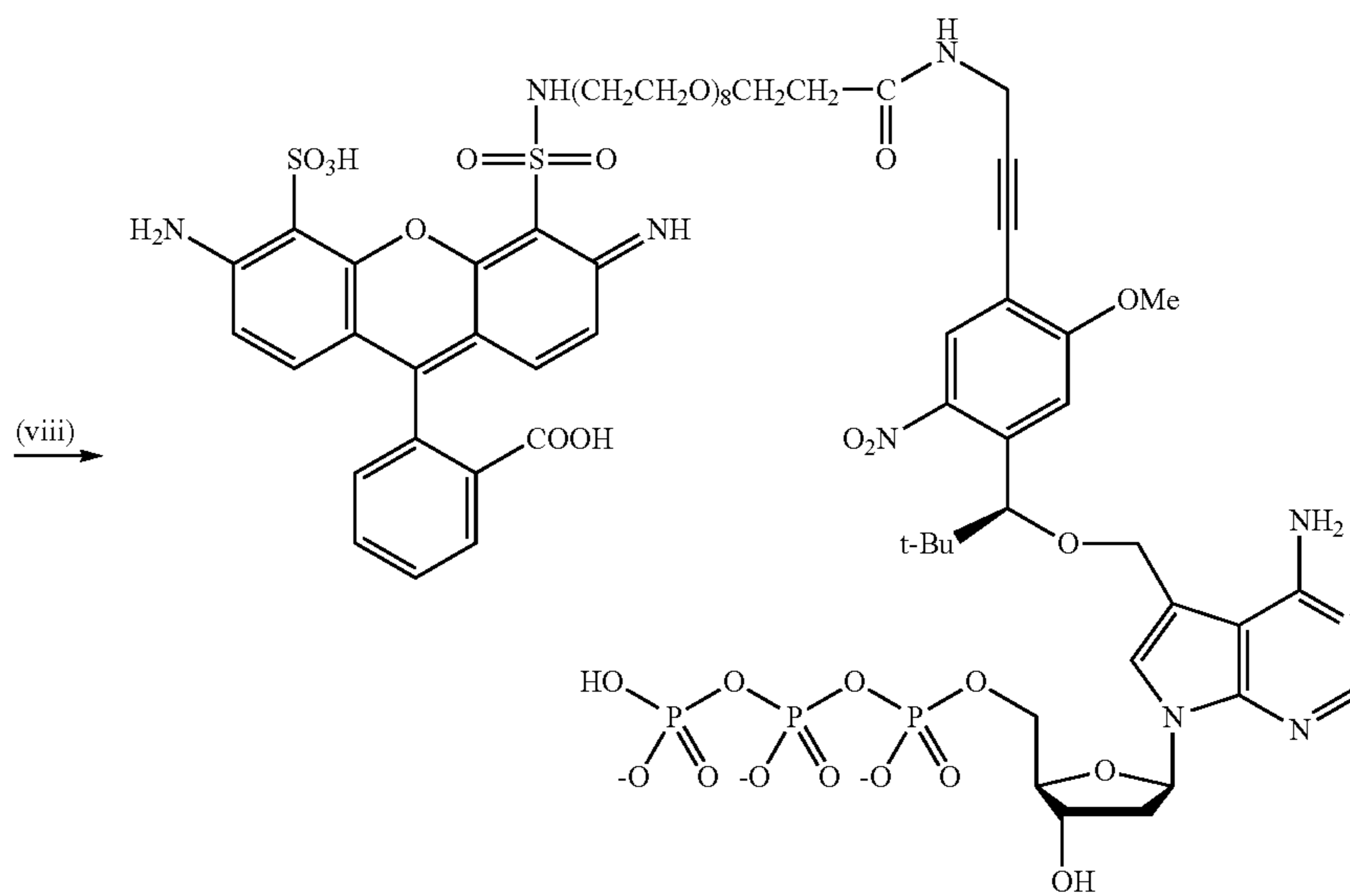
Scheme 2d.
