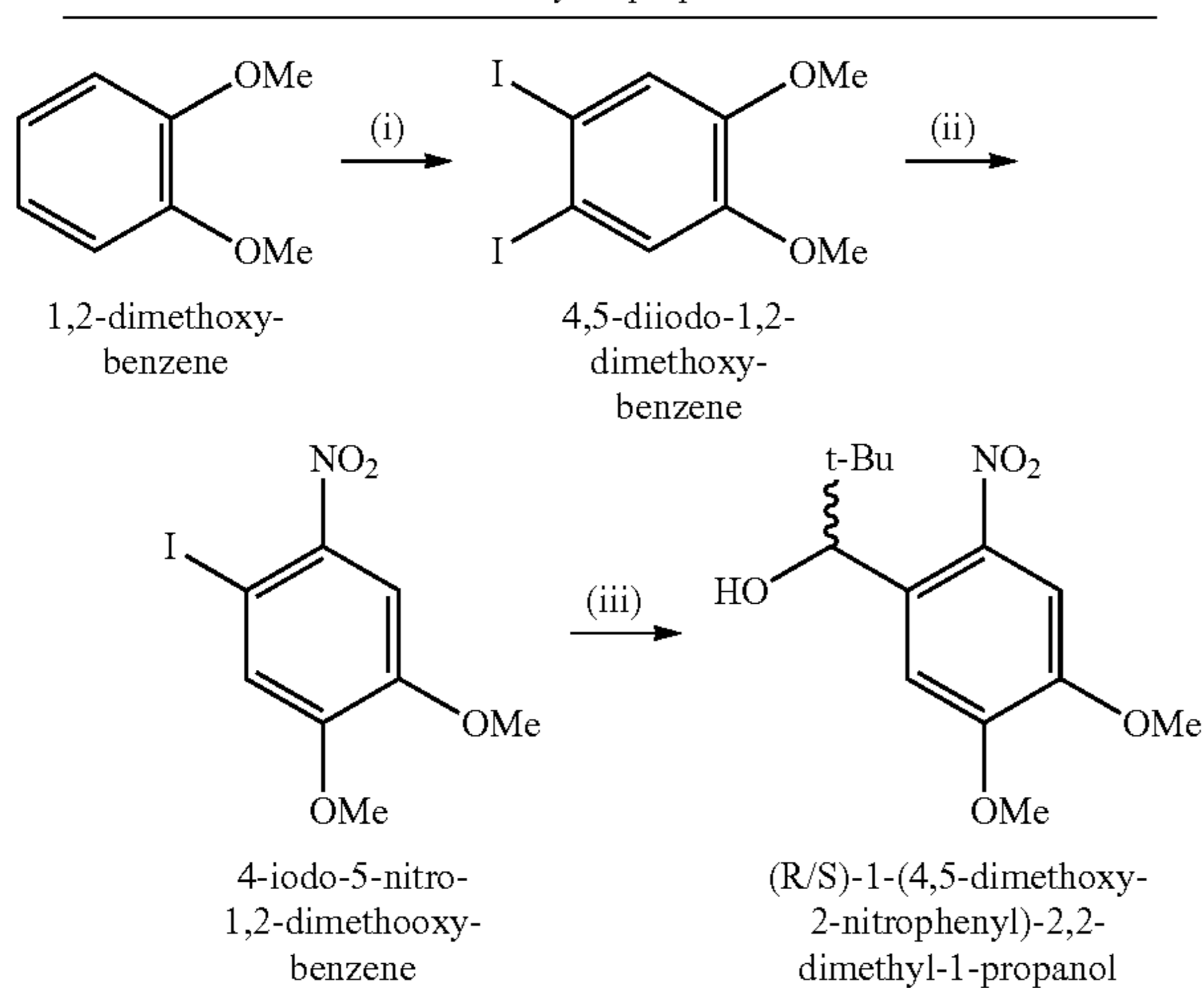
Scheme S5. Synthesis of (R/S)-1-(4,5-dimethoxy-2-nitrophenyl)-2,2-dimethyl-1-propanol.
