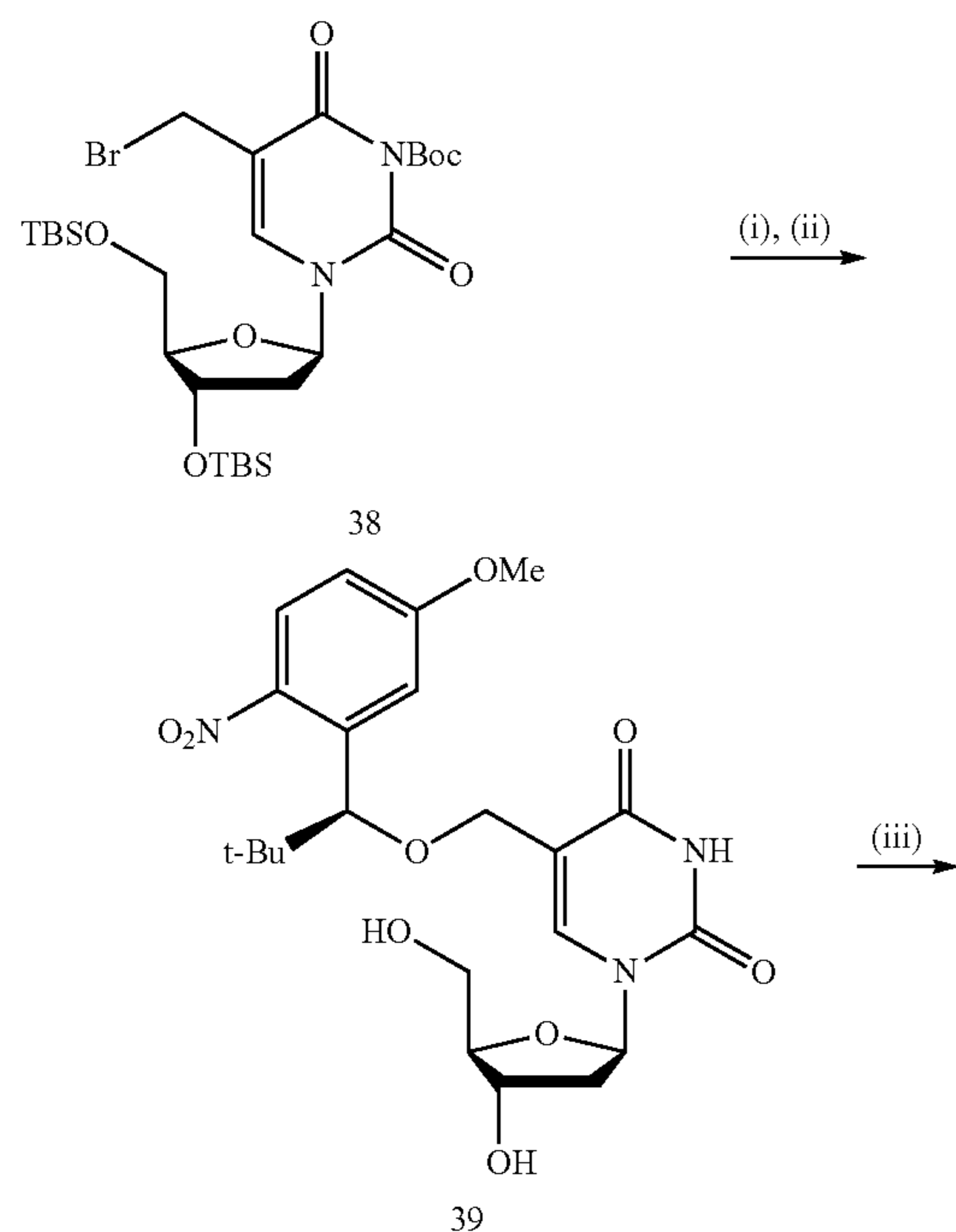
Scheme S19. Synthesis of 5-[(S)-1-(5-methoxy-2-nitrophenyl)-2,2-dimethyl-propyloxy]methyl-2'-deoxyuridine-5'-triphosphate.
