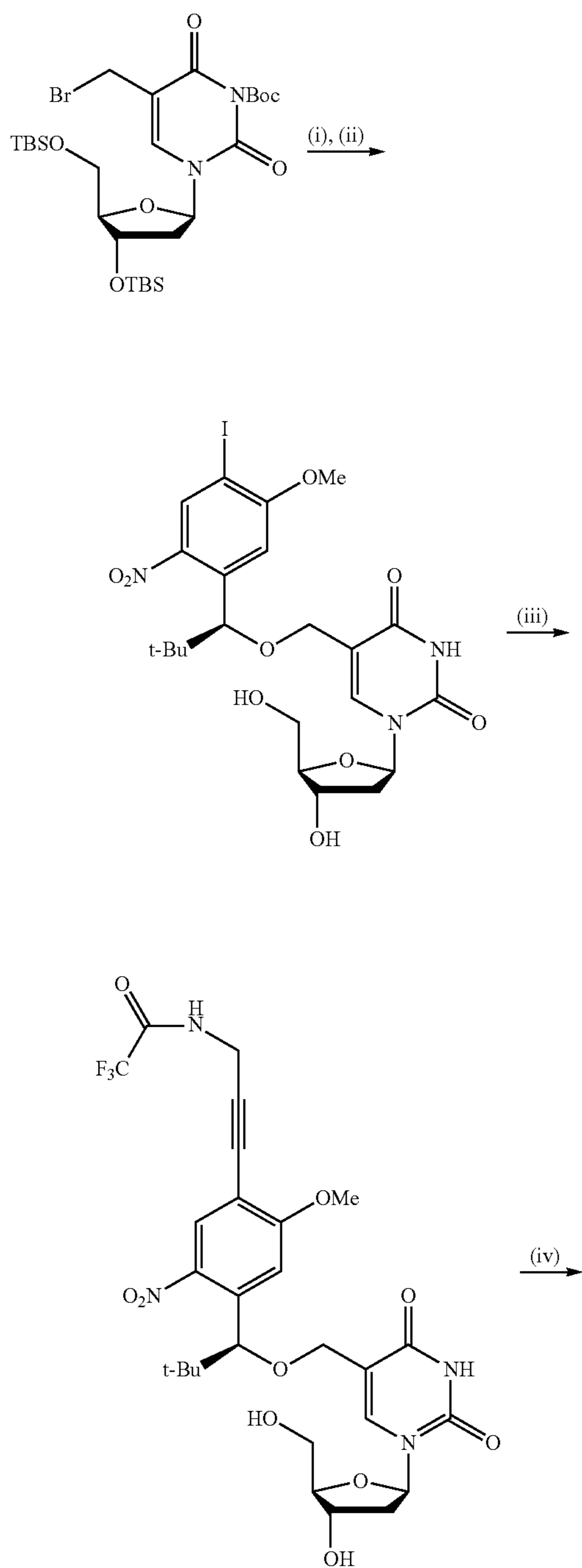
Scheme 3a. Synthesis of dye labeled 5-[(S)-1-(5-methoxy-2-nitrophenyl)-2,2-dimethyl-propyloxy]methyl-2'-deoxyuridine-5'-triphosphate.
