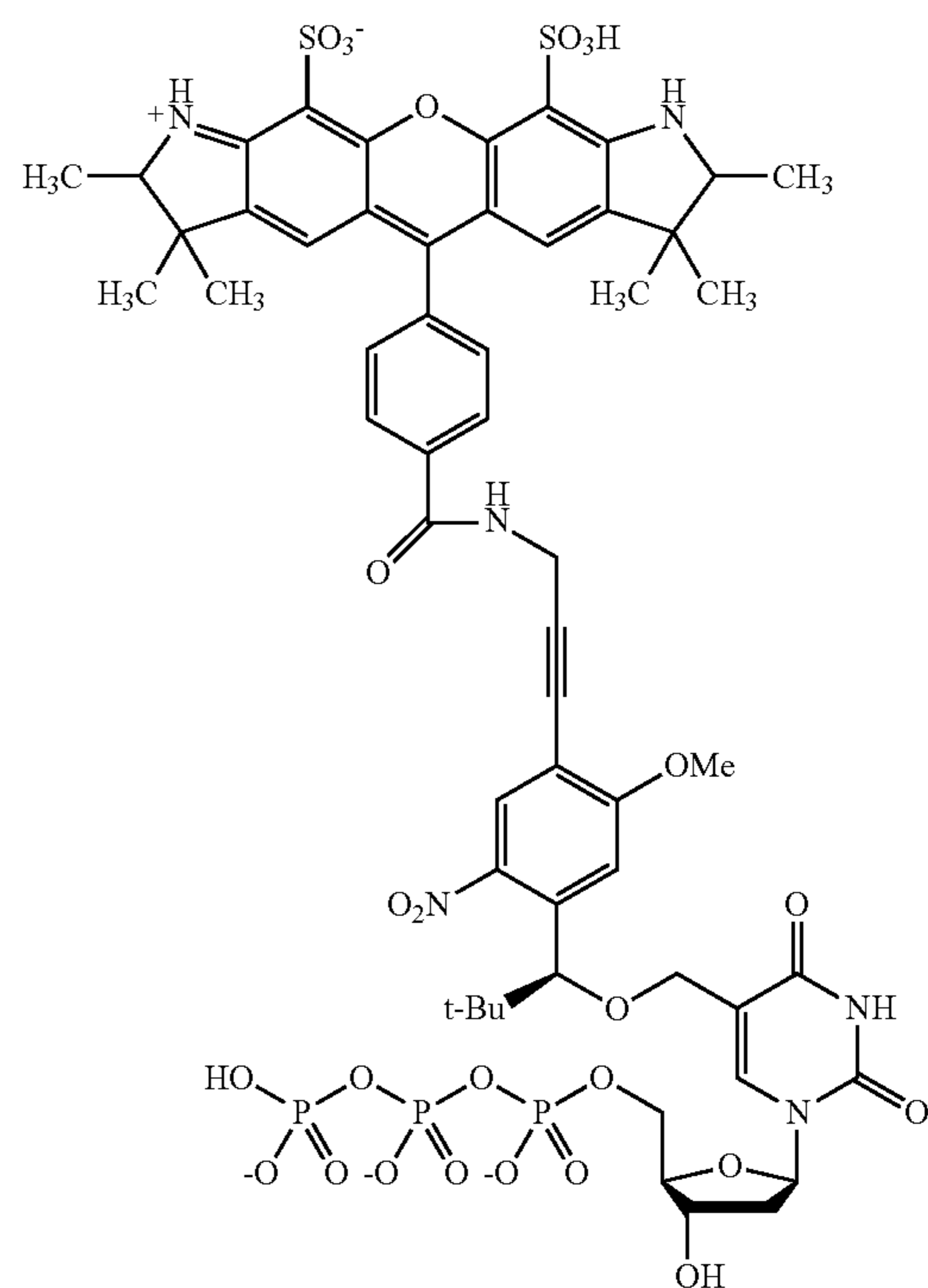
Scheme 3b.
