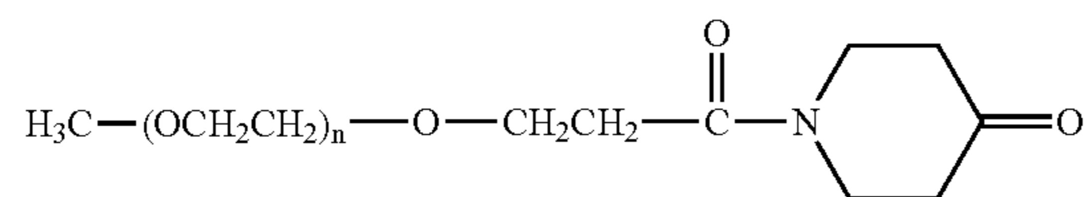
mPEG Piperidone
