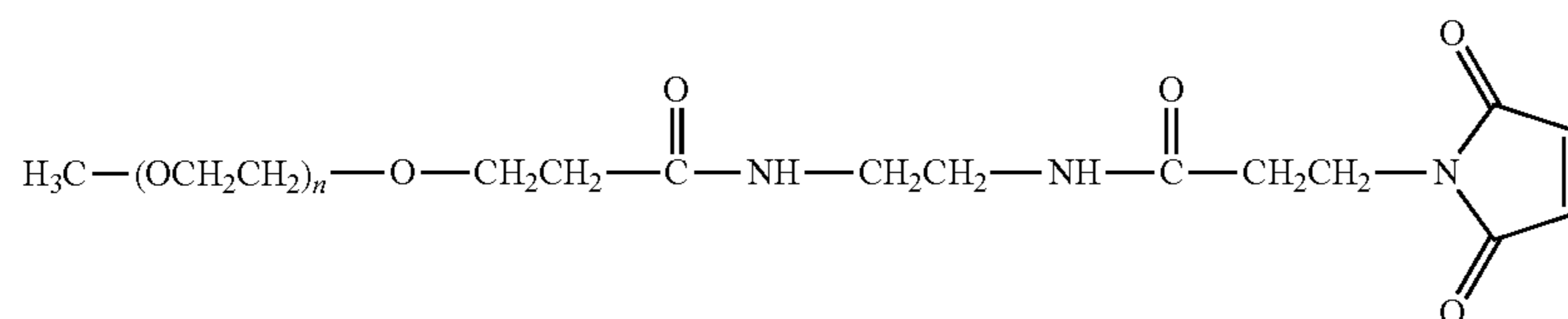
mPEG Maleimide Derivative (under certain reaction conditions such as pH >8)
