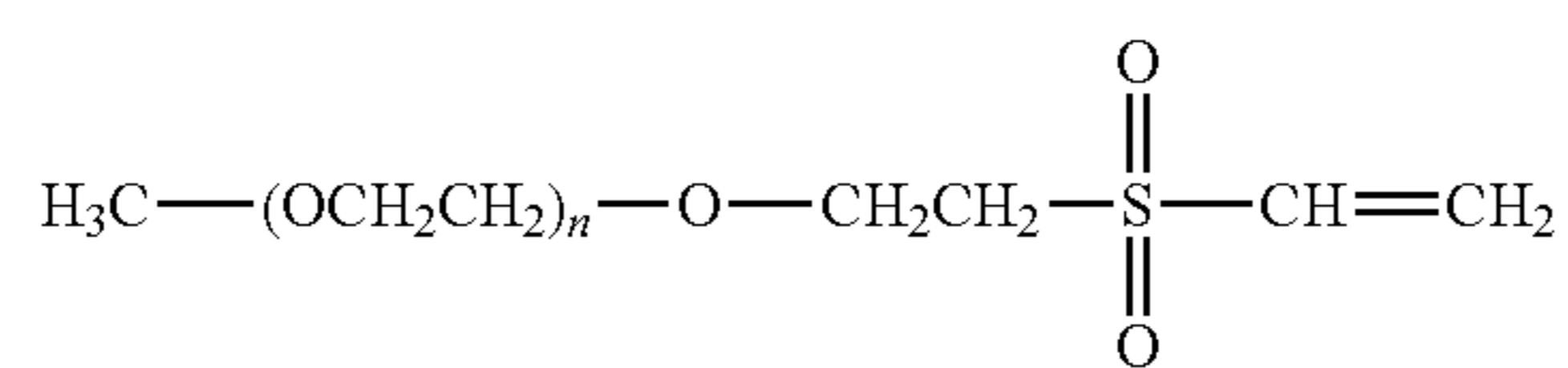
mPEG vinyl sulfone
