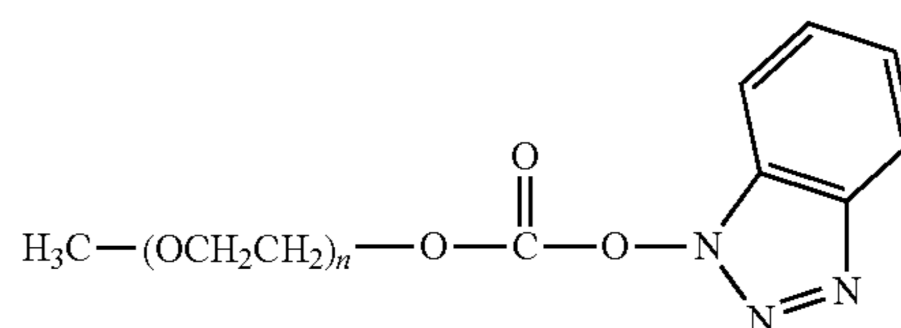
mPEG-Benzotriazole Carbonate
