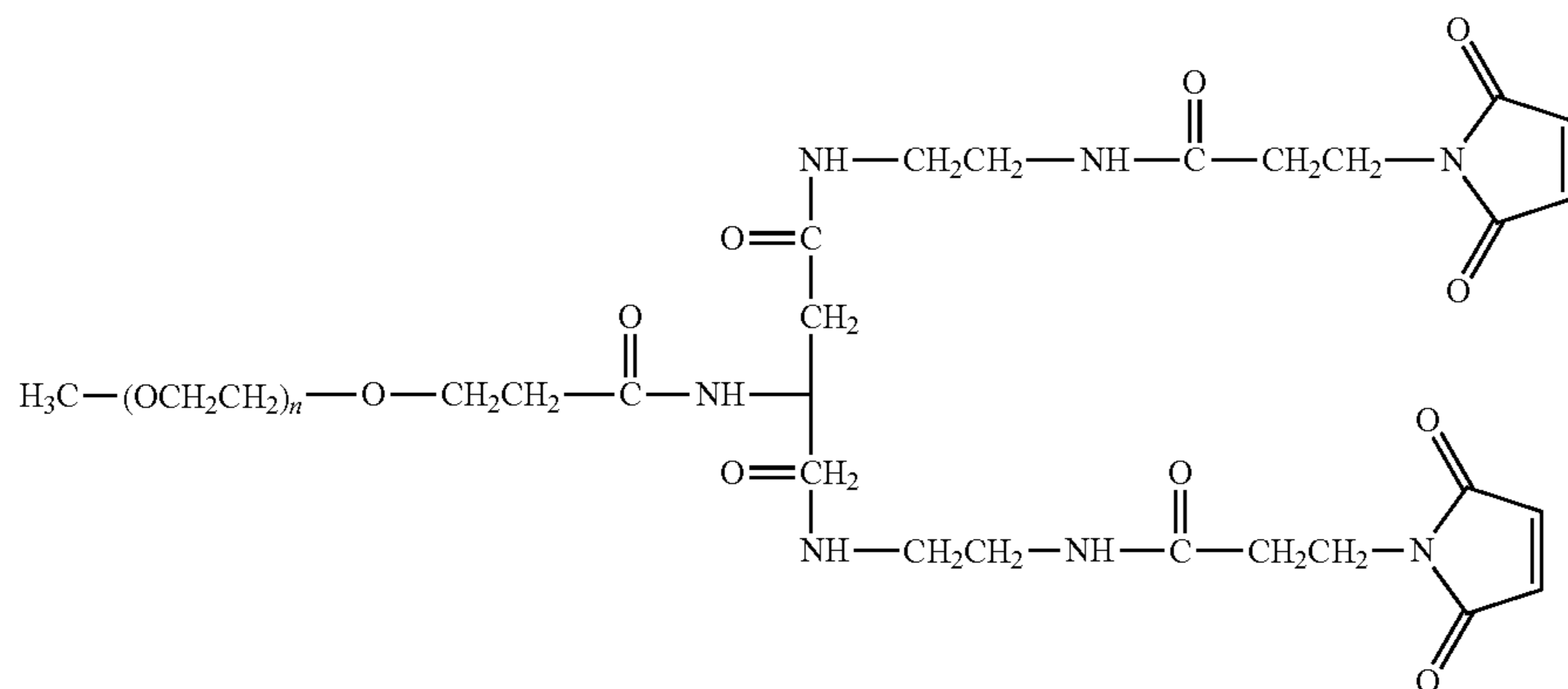
mPEG Forked Maleimide Derivative
