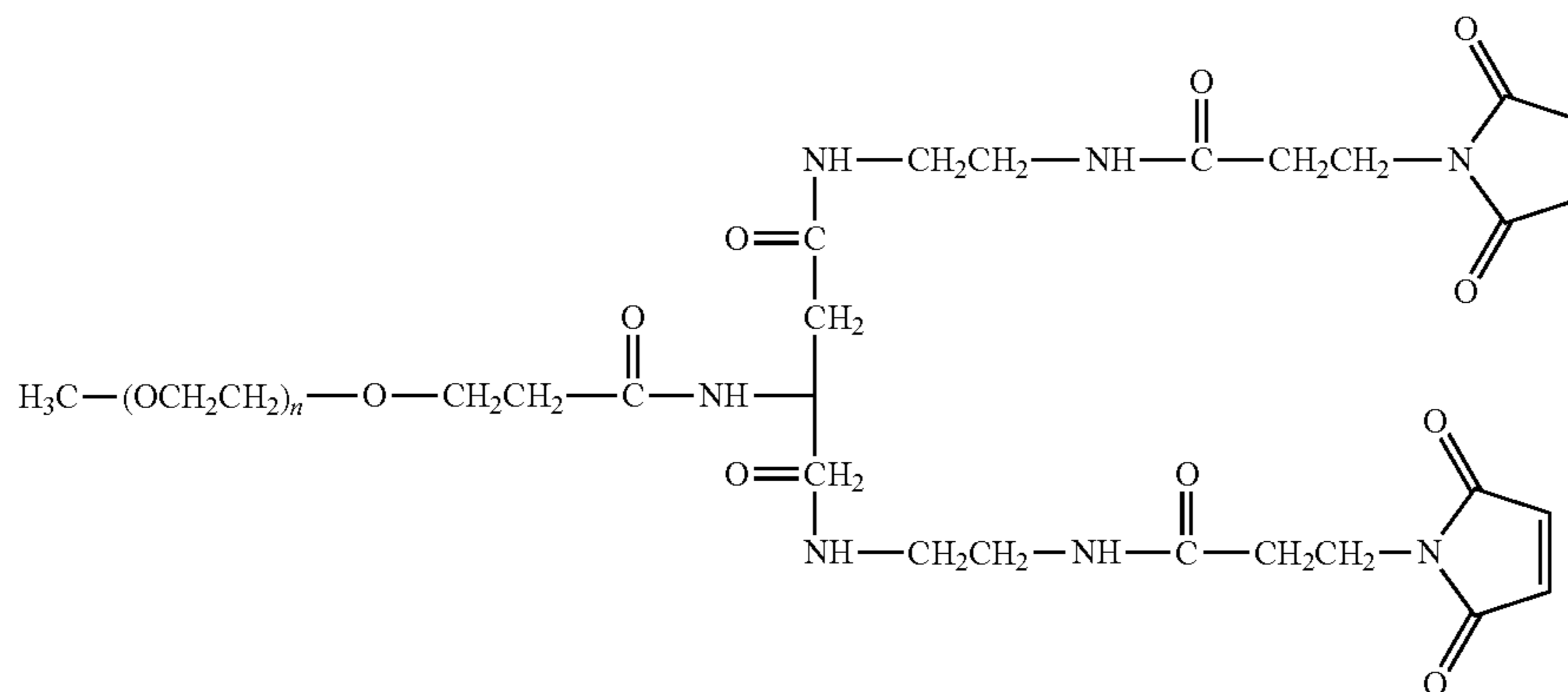
mPEG Forked Maleimide Derivative (under certain reaction conditions such as pH >8)
