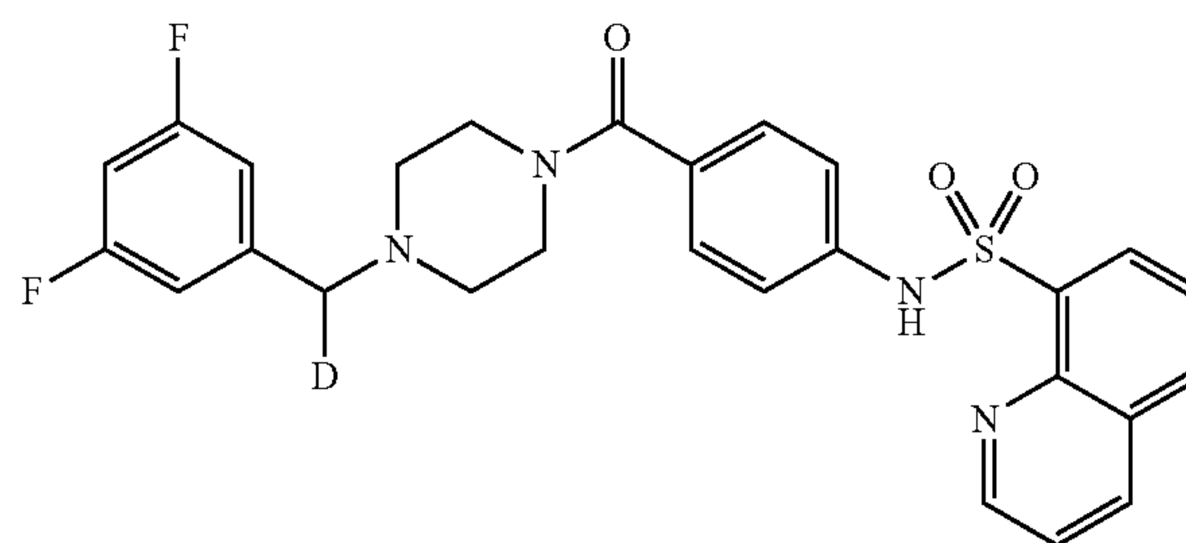
N-(4-(4-(3,5-difluorobenzyl)piperazine-1-carbonyl)phenyl)quinoline-8-sulfonamide-(D) (Compound 342)
