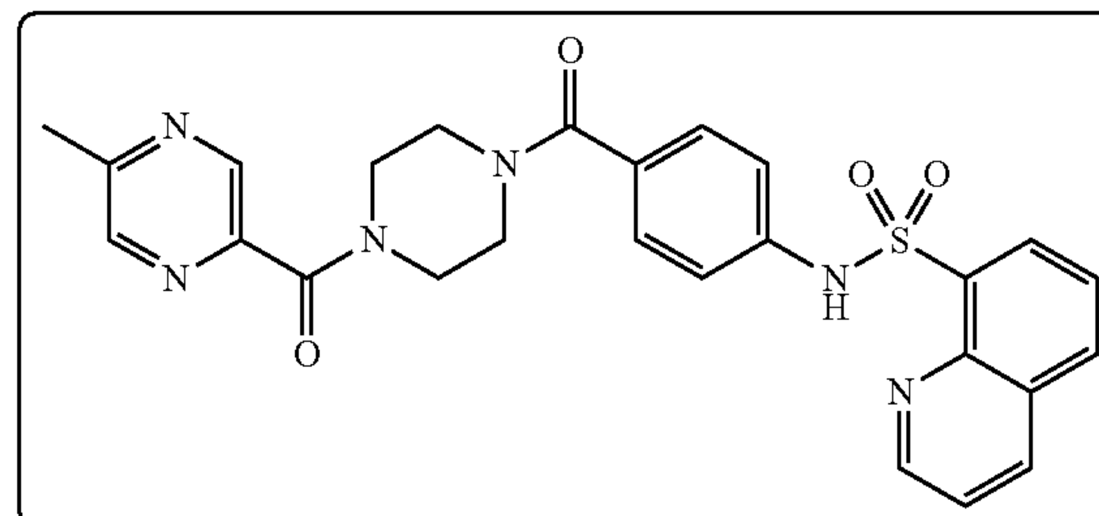
N-(4-(4-(5-methylpyrazine-2-carbonyl)piperazine-1-carbonyl)phenyl)quinoline-8-sulfonamide (Compound 346)
