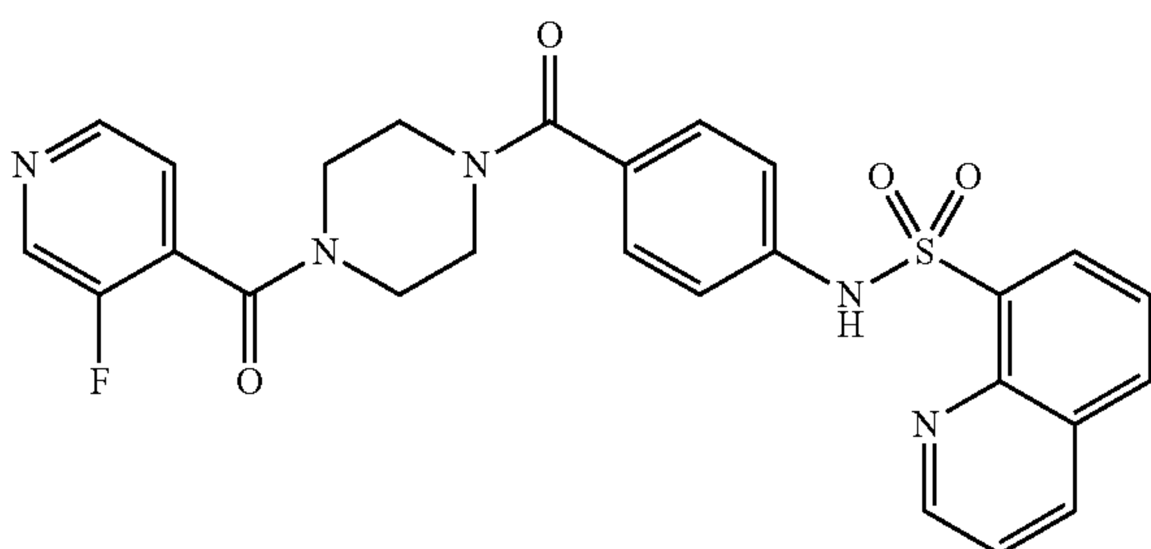
N-(4-(4-(3-fluoroisonicotinoyl)piperazine-1-carbonyl)phenyl)quinoline-8-sulfonamide (Compound 317)
