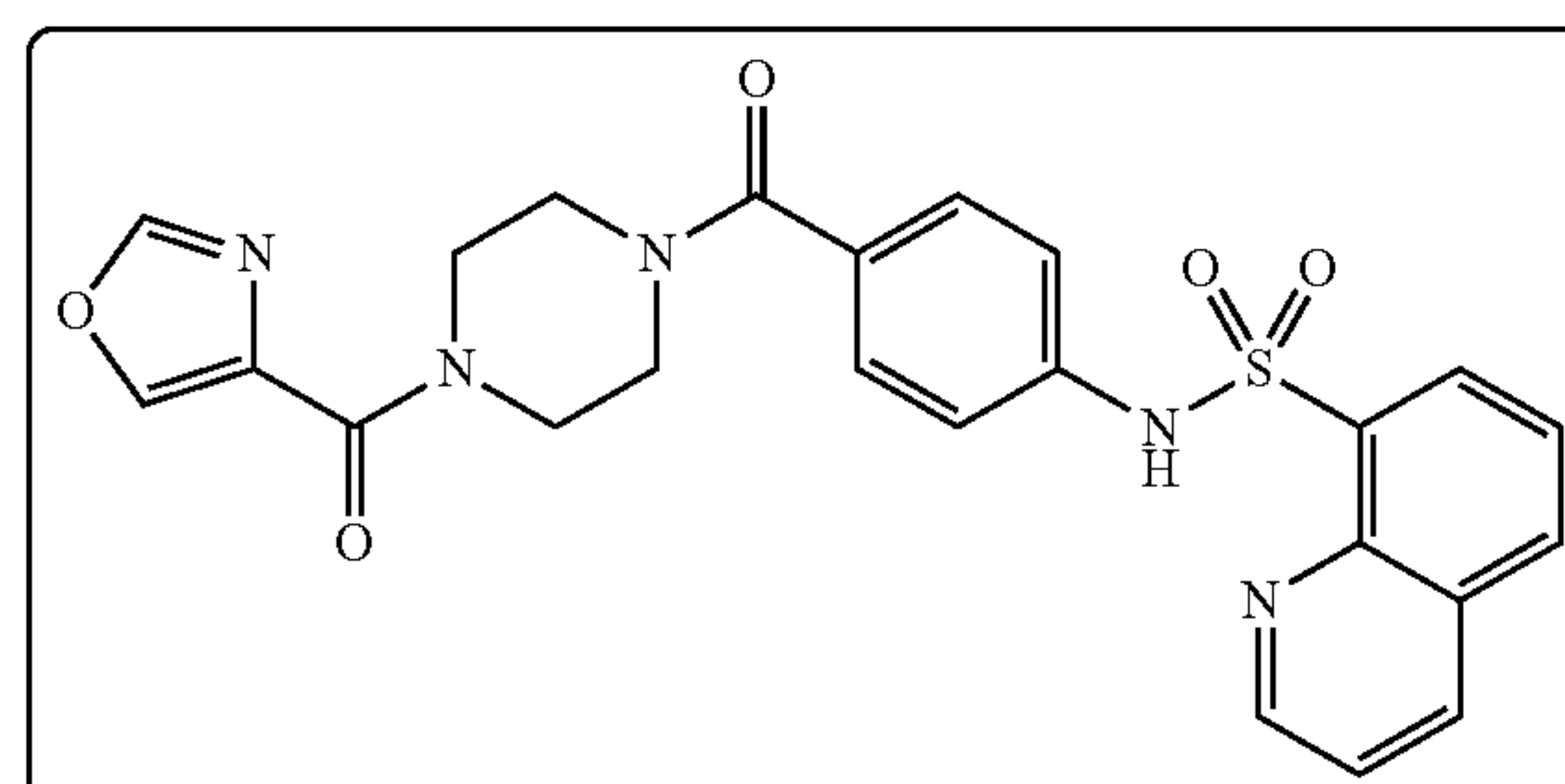
N-(4-(4-(oxazole-4-carbonyl)piperazine-1-carbonyl)phenyl)quinoline-8-sulfonamide (Compound 347)
