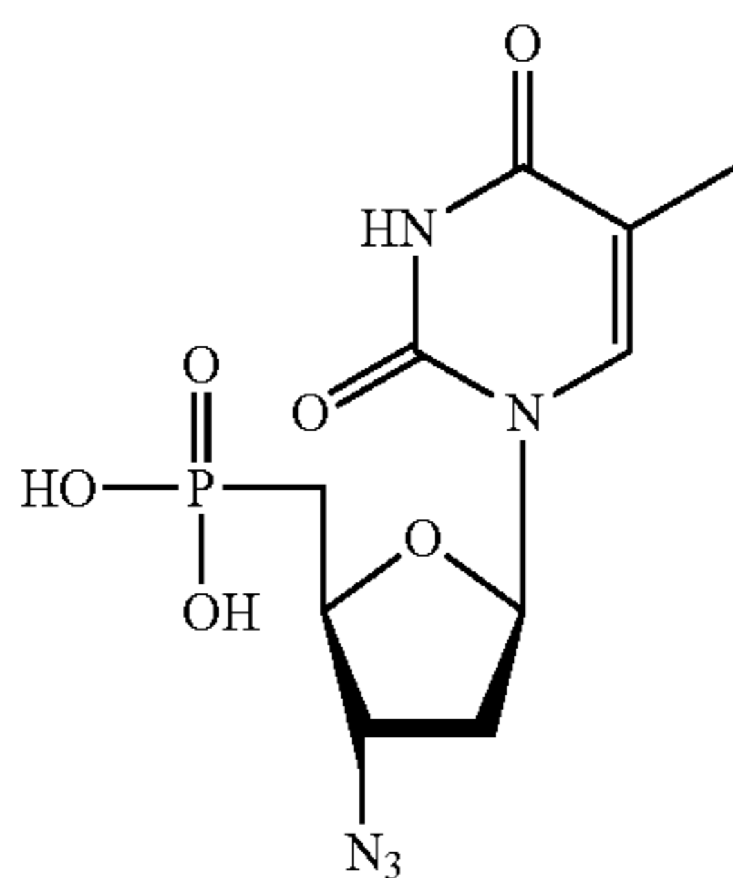
AZT 5'-phosphonate
