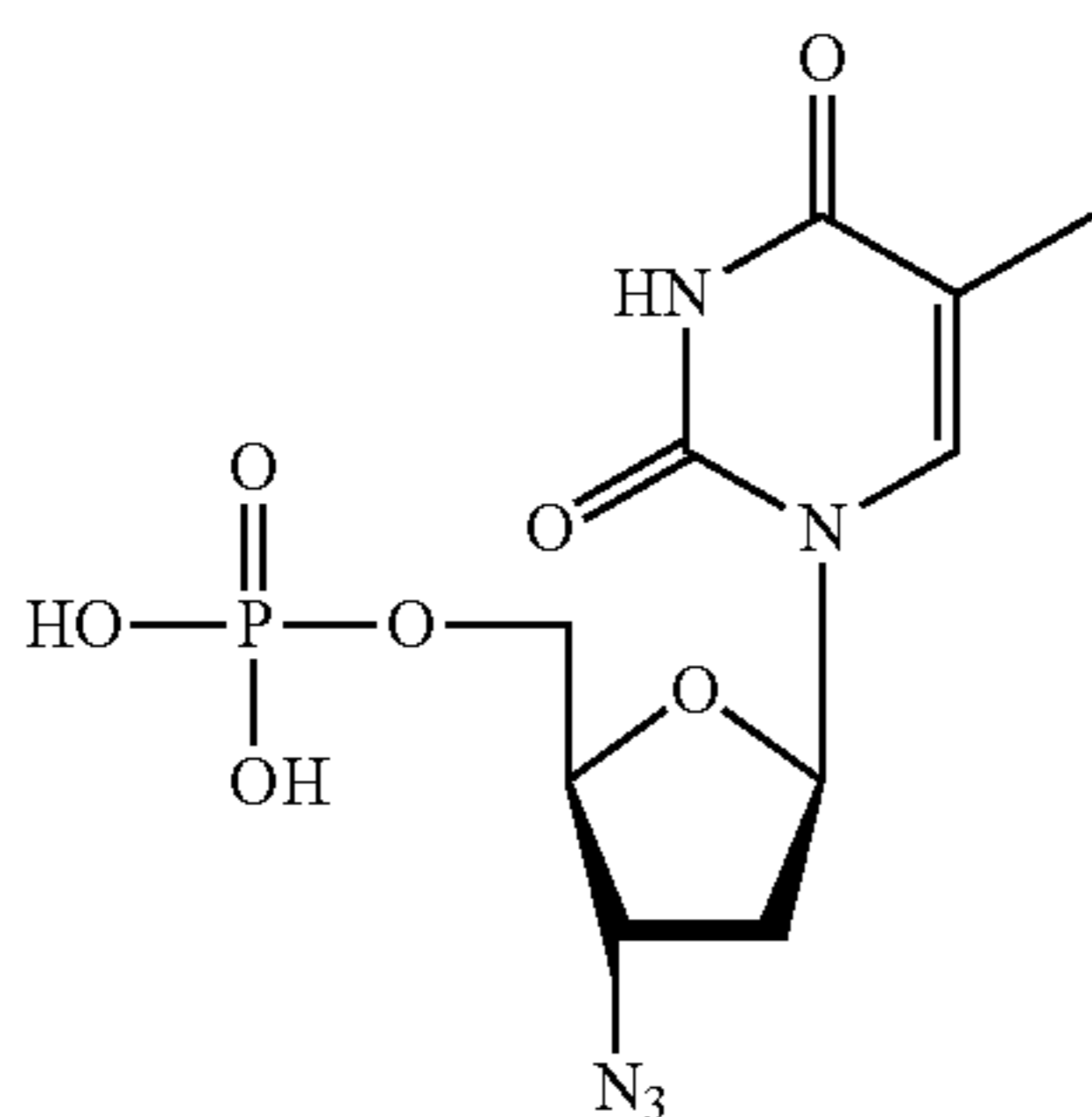
AZT 5'-phosphate
