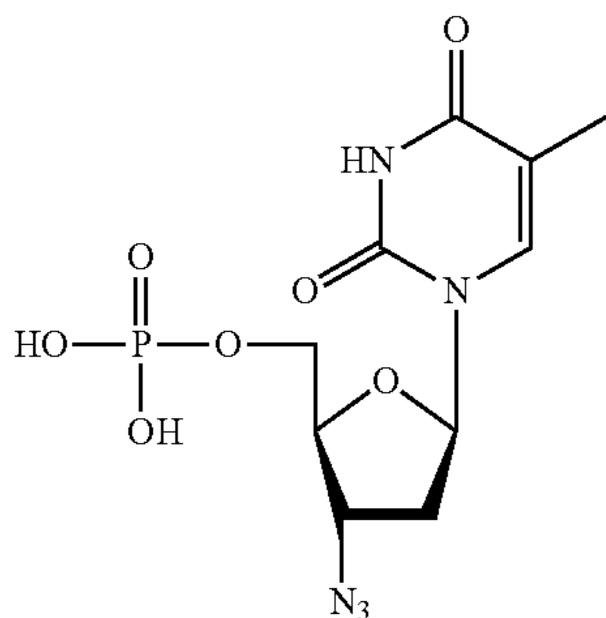
AZT 5'-phosphate
