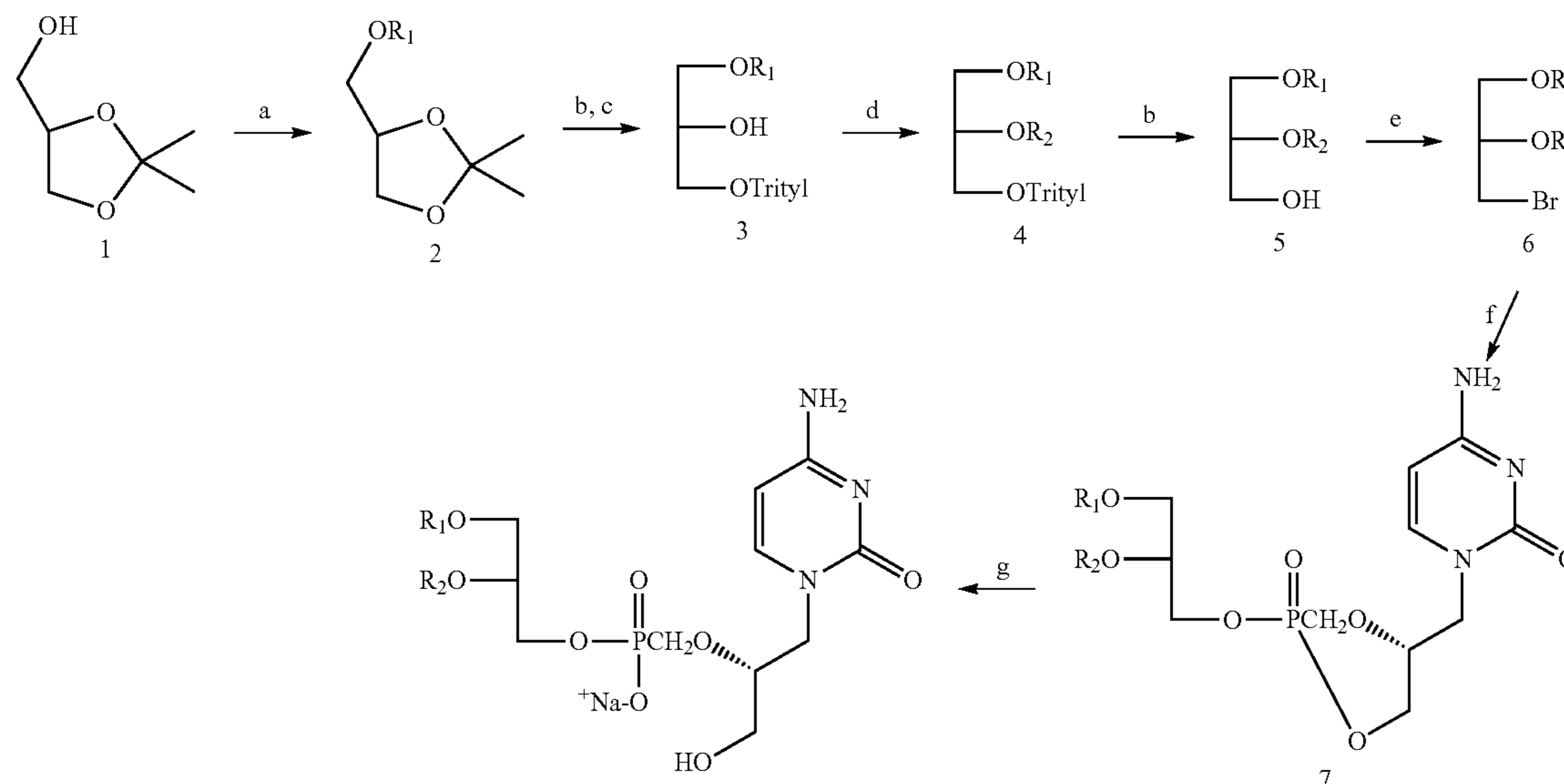
Scheme V
