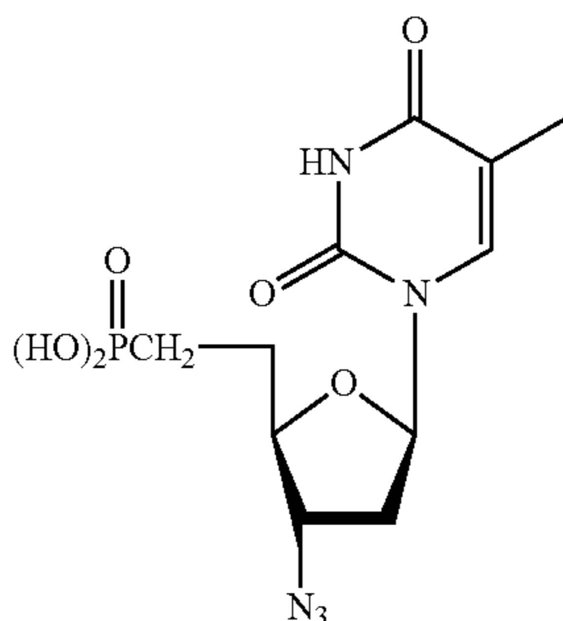
AZT 5'-methylene-phosphonate
