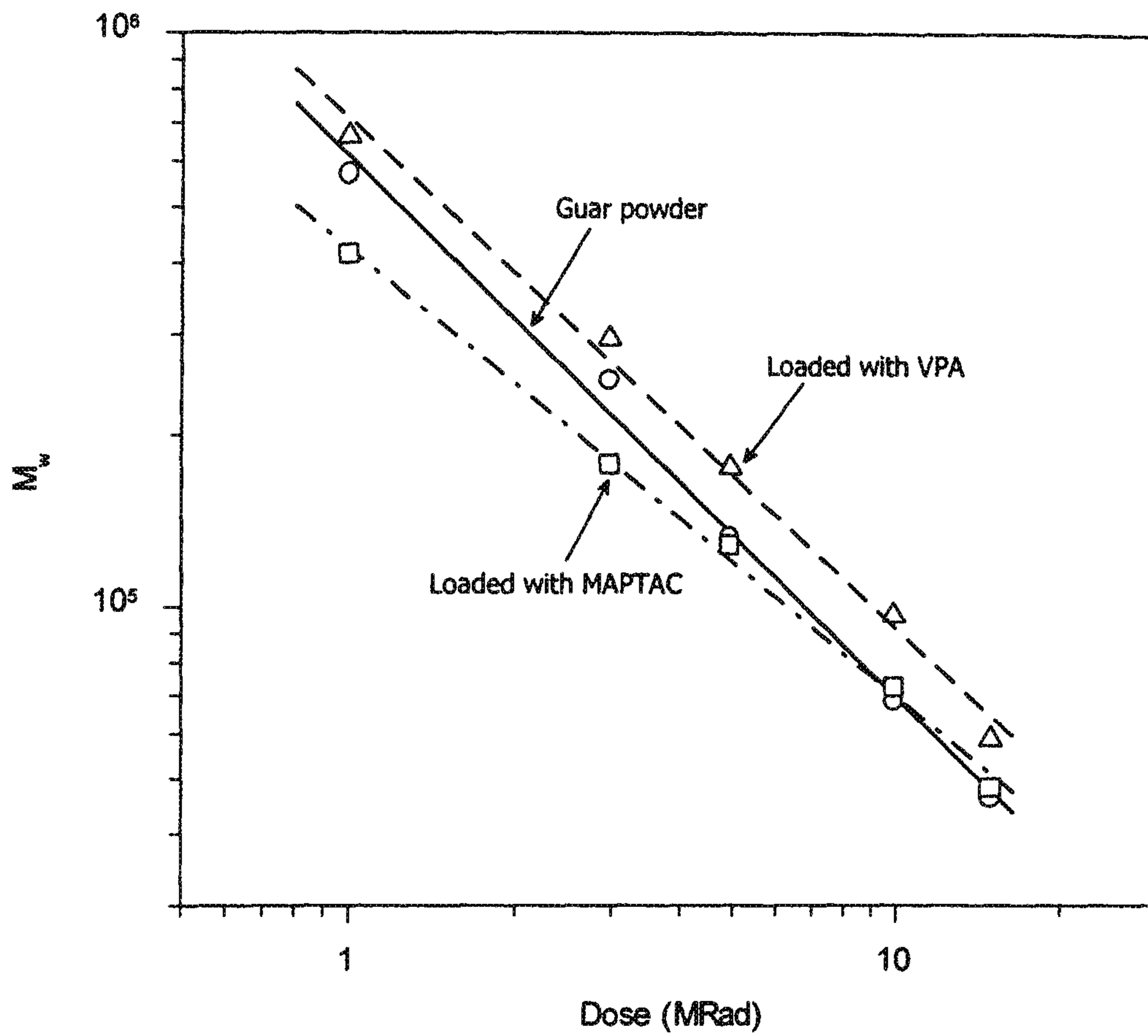
Depolymerization of Guar.
