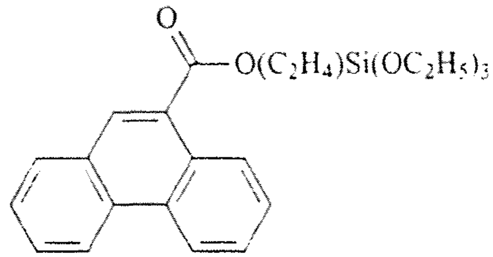
10-phenanthrene carboxy-ethyl triethoxysilane 30
