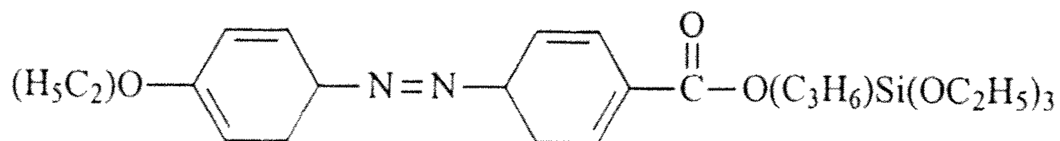
4-ethoxyphenylazobenzene-4-carboxy propyl triethoxysilane 36
