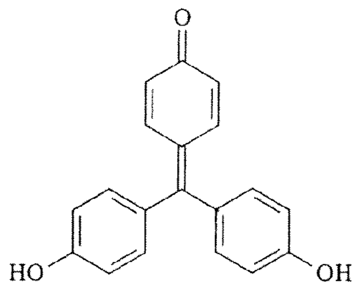
rosolic acid
