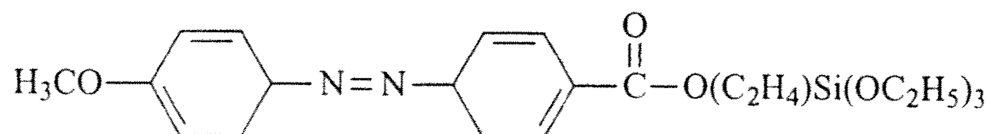
4-methoxyphenylazobenzene-4-carboxy ethyl triethoxysilane 40
