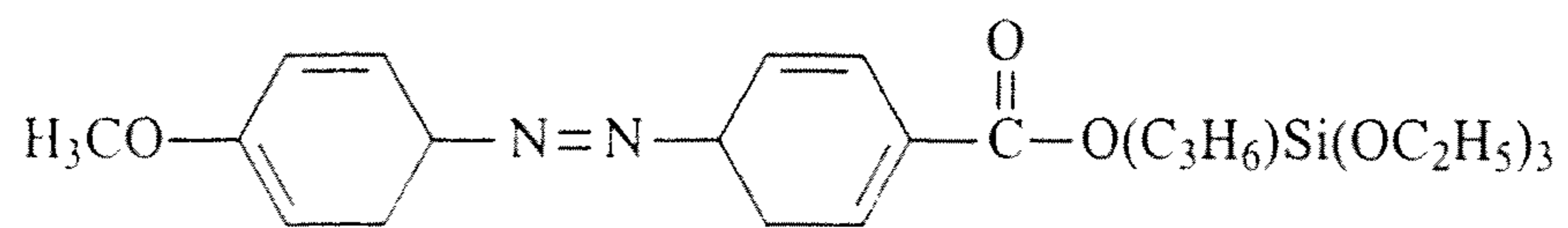
4-methoxyphenylazobenzene-4-carboxy propyl triethoxysilane
