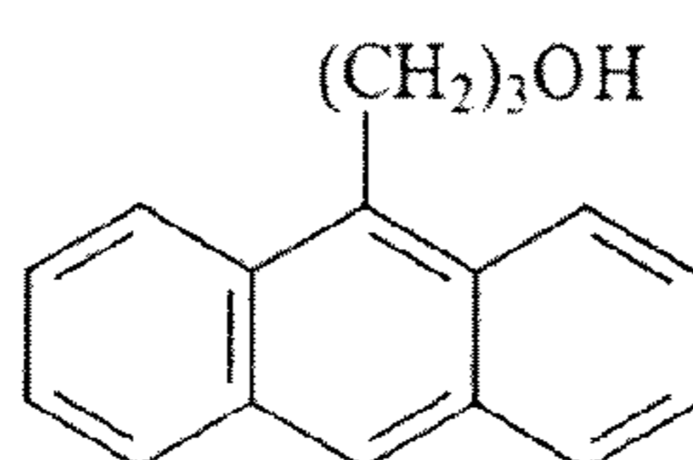
9-anthracene propanol 5
