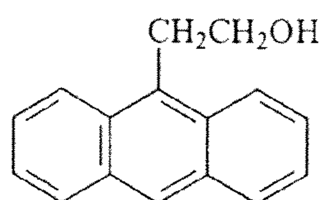
9-anthracene ethanol 4
