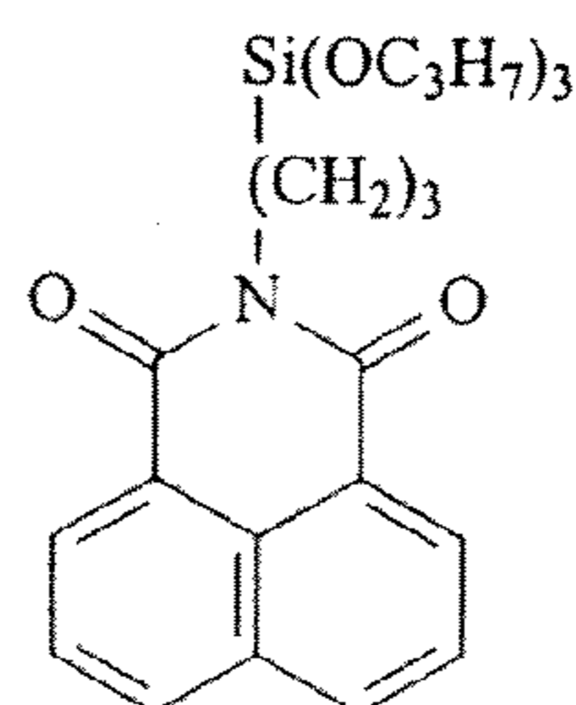
tripropoxysilylpropyl-1,8-naphthalimide
