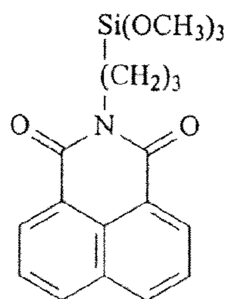
trimethoxysilylpropyl-1,8-naphthalimide
