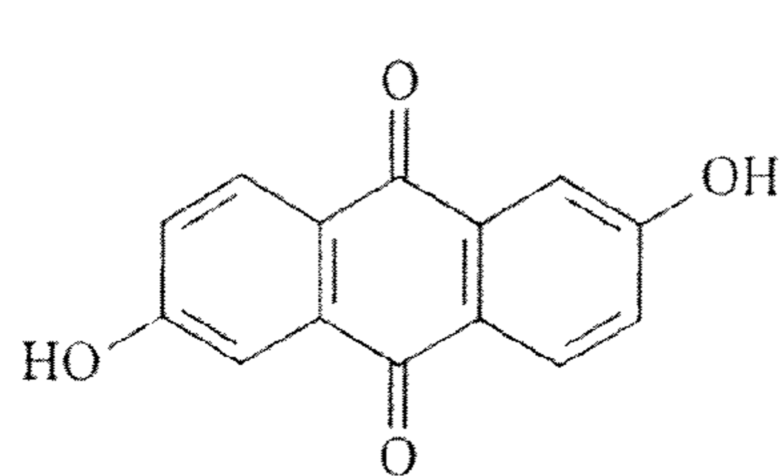
anthraflavic acid 1
