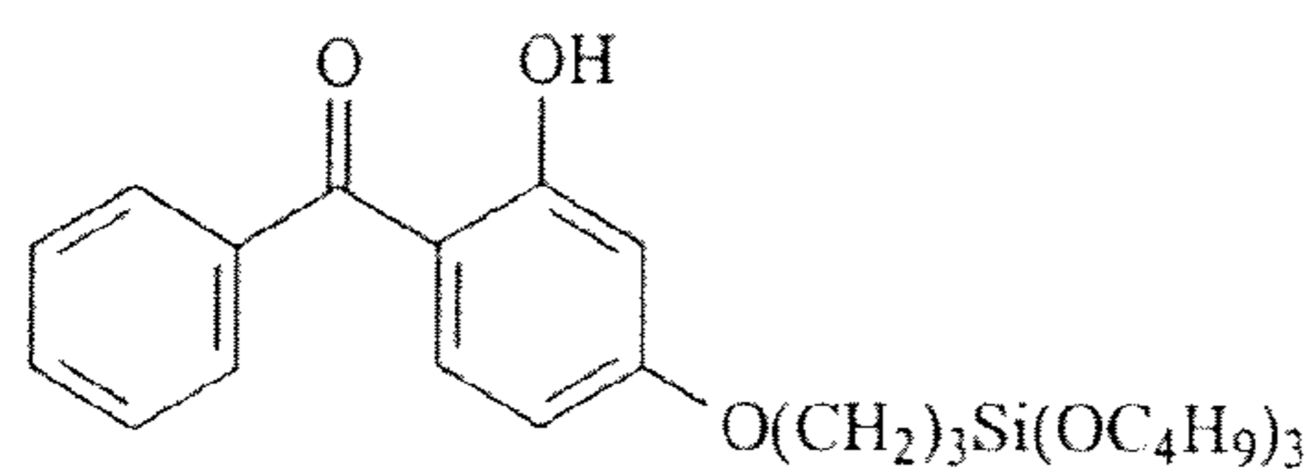
2-hydroxy-4-(3-tributoxysilylpropoxy)- diphenylketone
