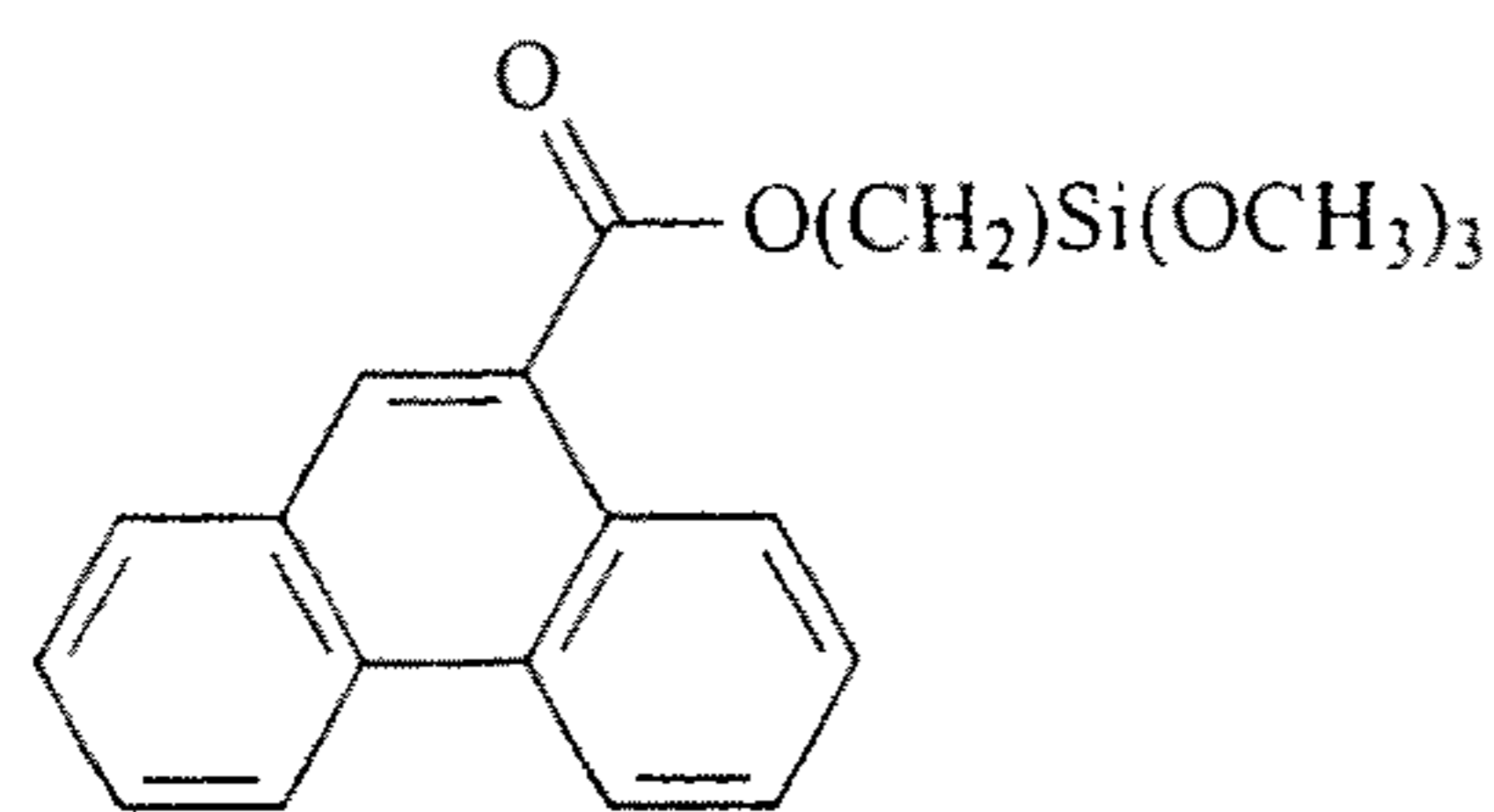
10-phenanthrene carboxy-methyl trimethoxysilane 31
