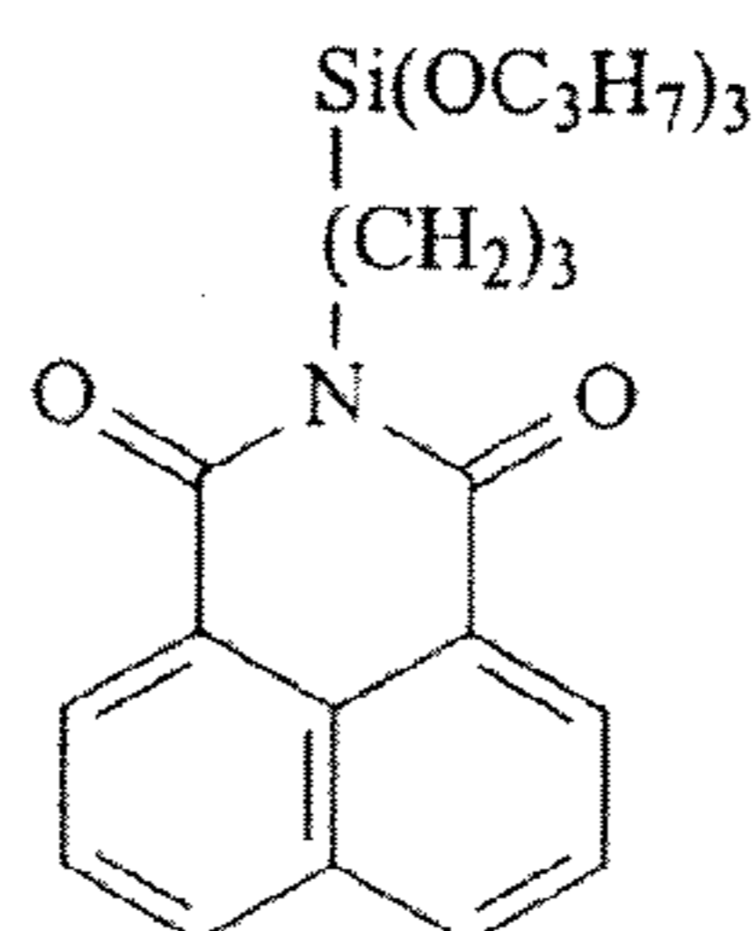
tripropoxysilylpropyl-1,8-naphthalimide
