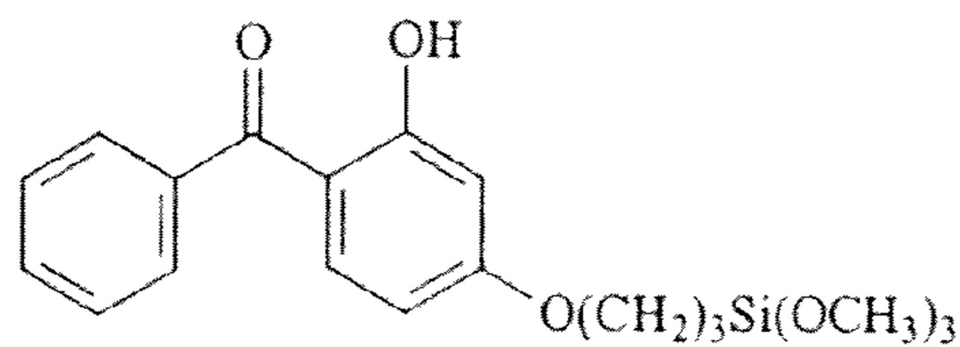
2-hydroxy-4-(3-trimethoxysilylpropoxy)- diphenylketone
