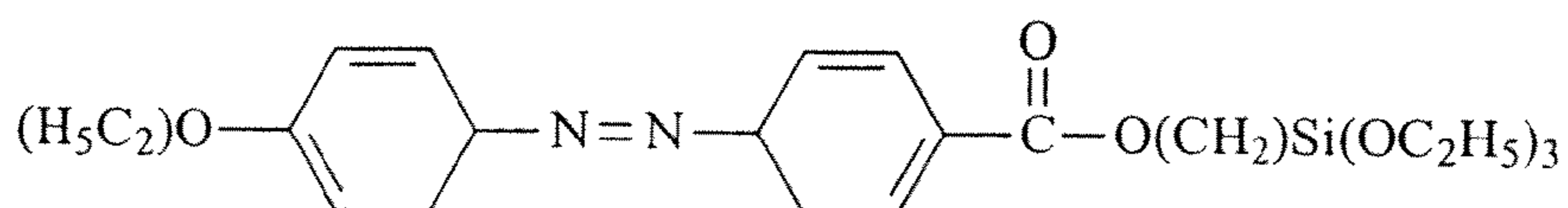
4-ethoxyphenylazobenzene-4-carboxy methyl triethoxysilane 39
