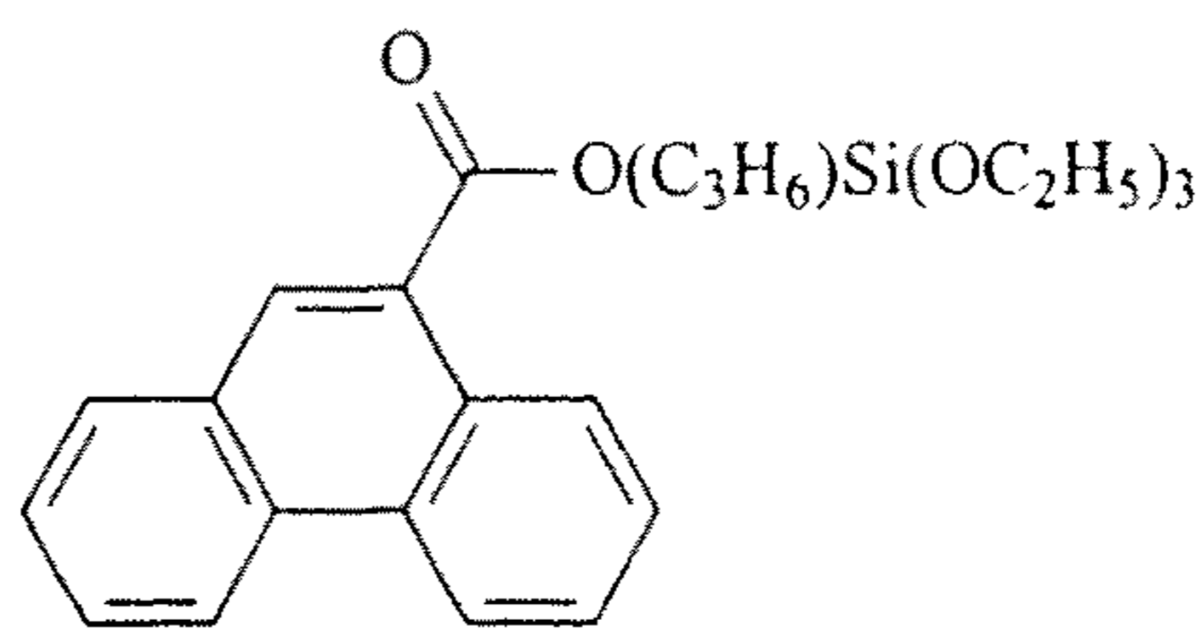
10-phenanthrene carboxy-propyl triethoxysilane 32
