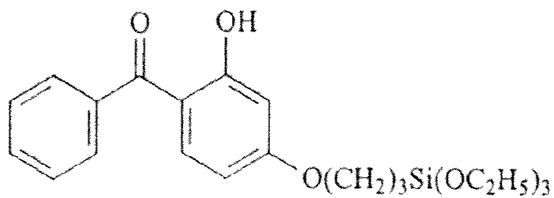
2-hydroxy-4-(3-triethoxysilylpropoxy)- diphenylketone
