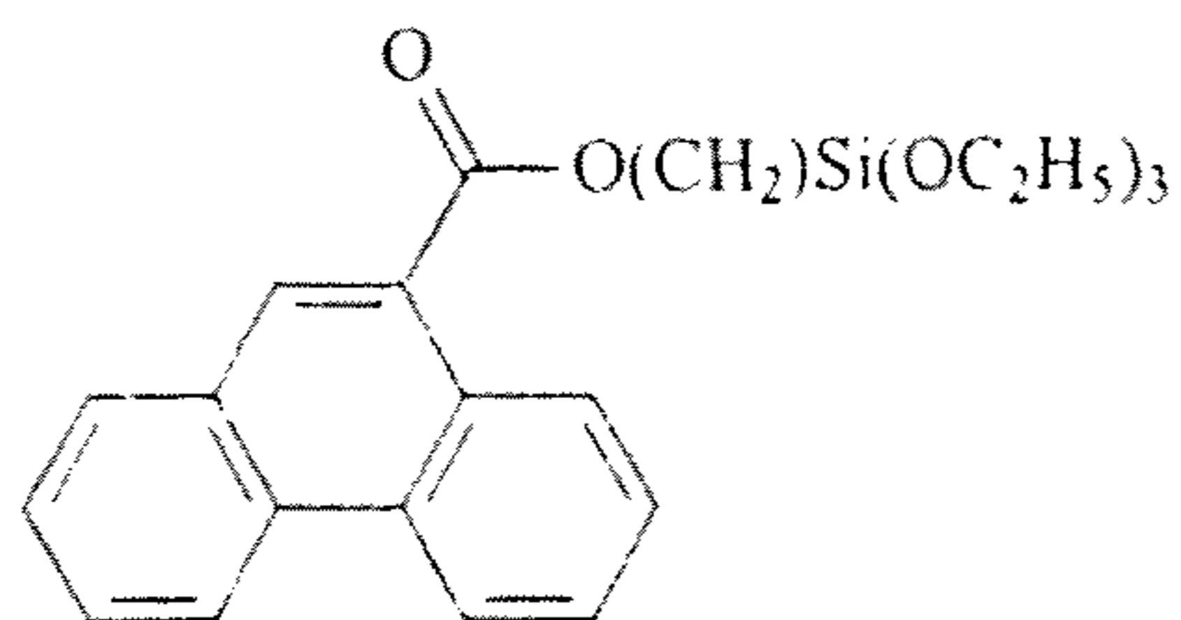
10-phenanthrene carboxy-methyl triethoxysilane 29
