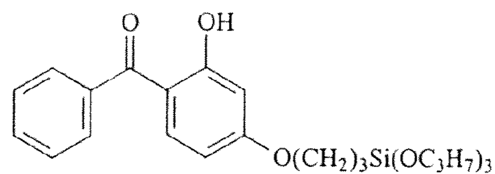
2-hydroxy-4-(3-tripropoxysilylpropoxy)- diphenylketone
