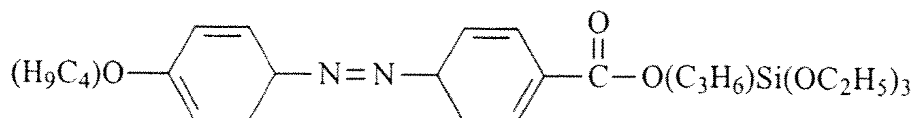
4-butoxyphenylazobenzene-4-carboxy propyl triethoxysilane 37
