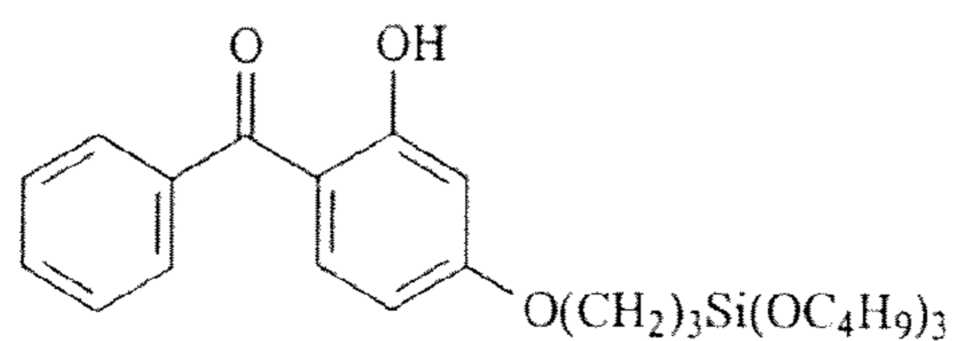
2-hydroxy-4-(3-tributoxysilylpropoxy)- diphenylketone
