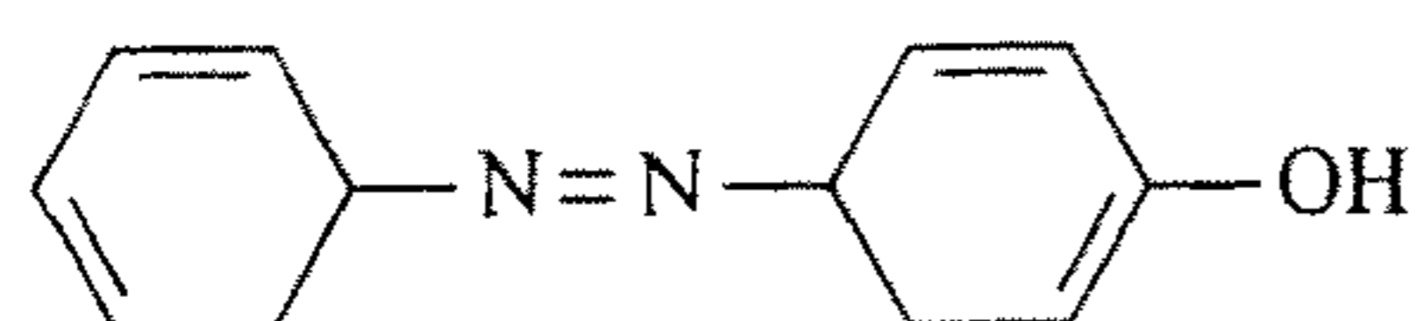
4-phenylazophenol 33
