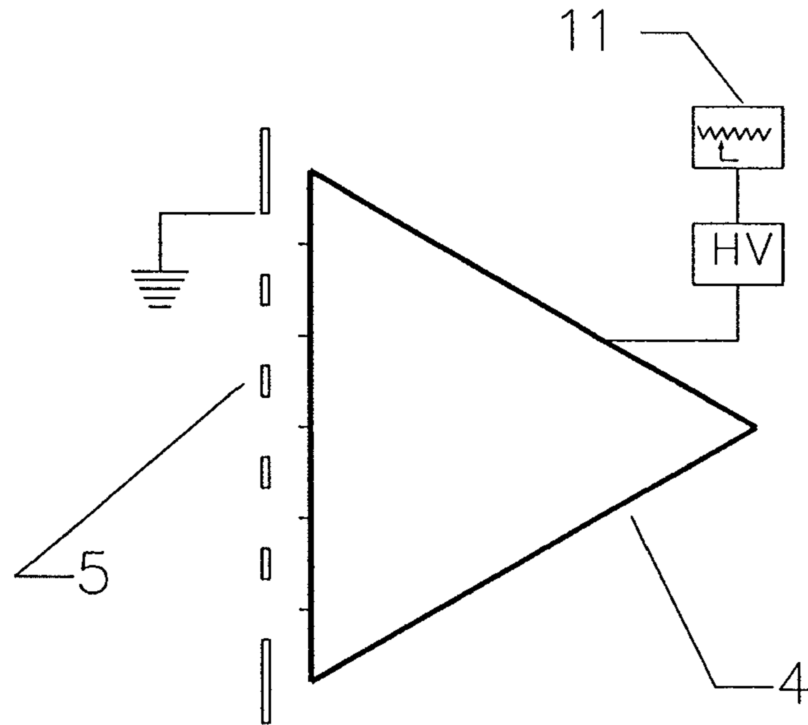
FIG. 7A: TOP VIEW OF ENERGIZING ELECTRODE
