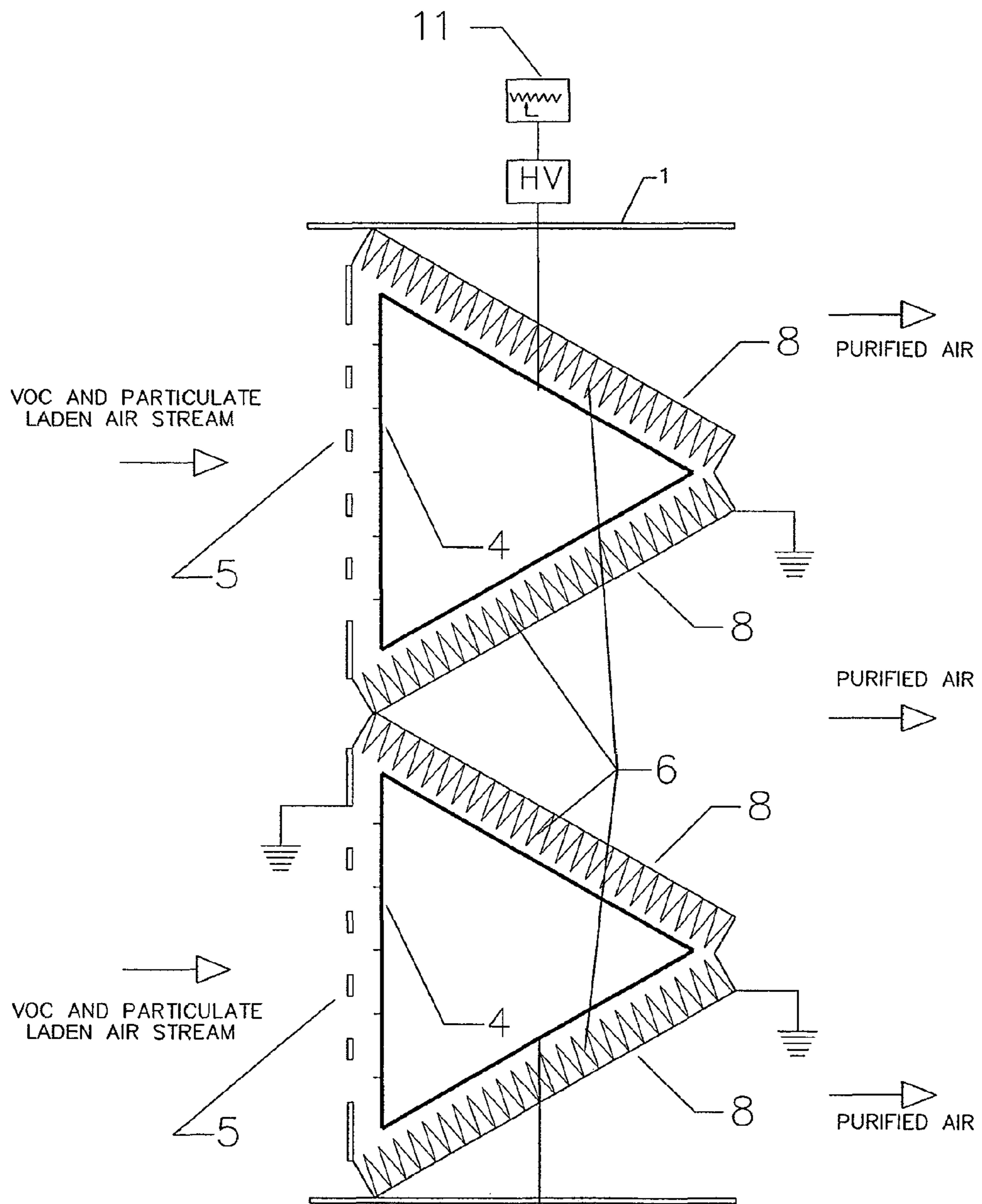
FIG. 6 TOP VIEW OF V-CELL FILTER
