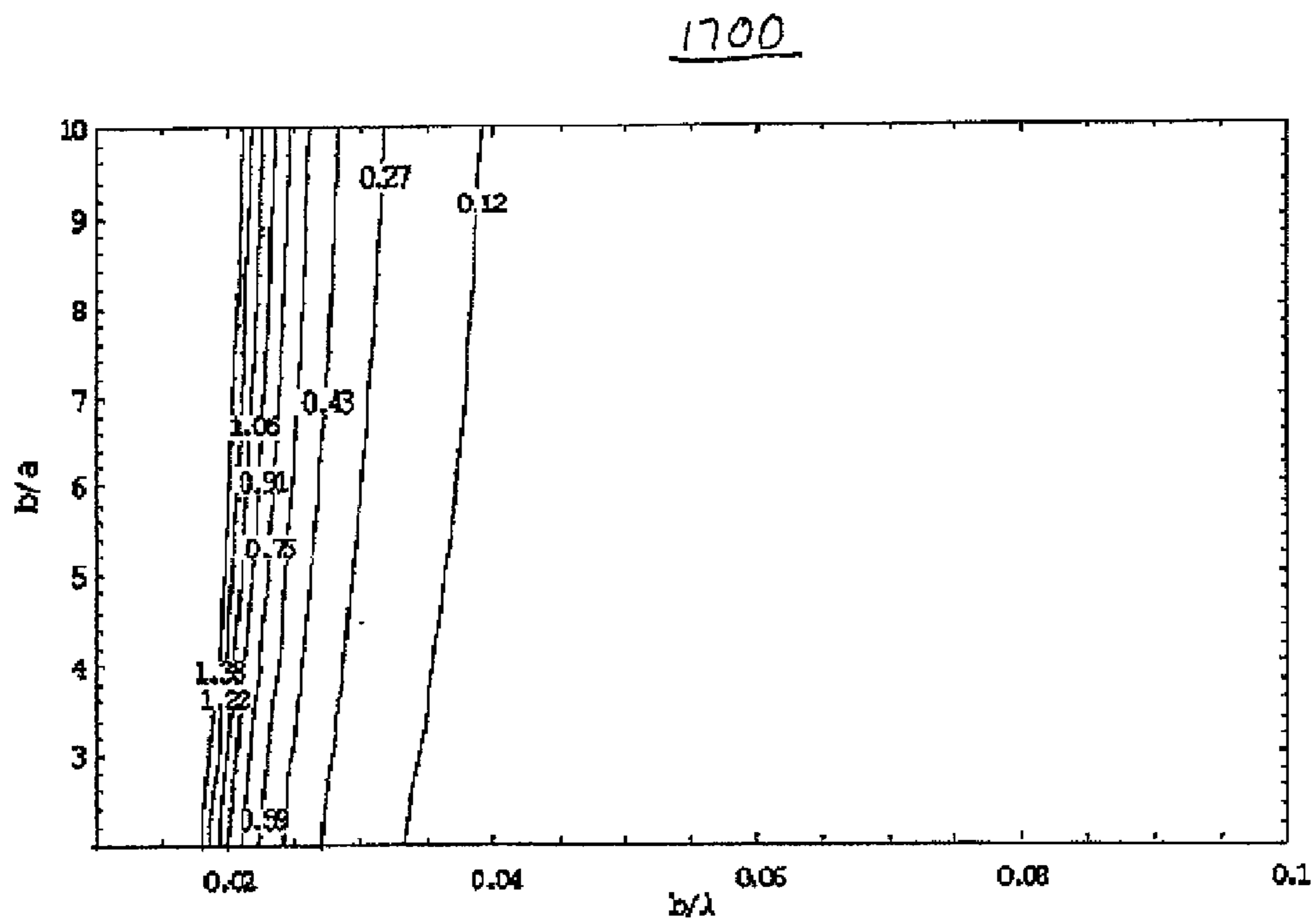
Figure 17 Contour plot of Q_{rad} \times 10^{-5}
