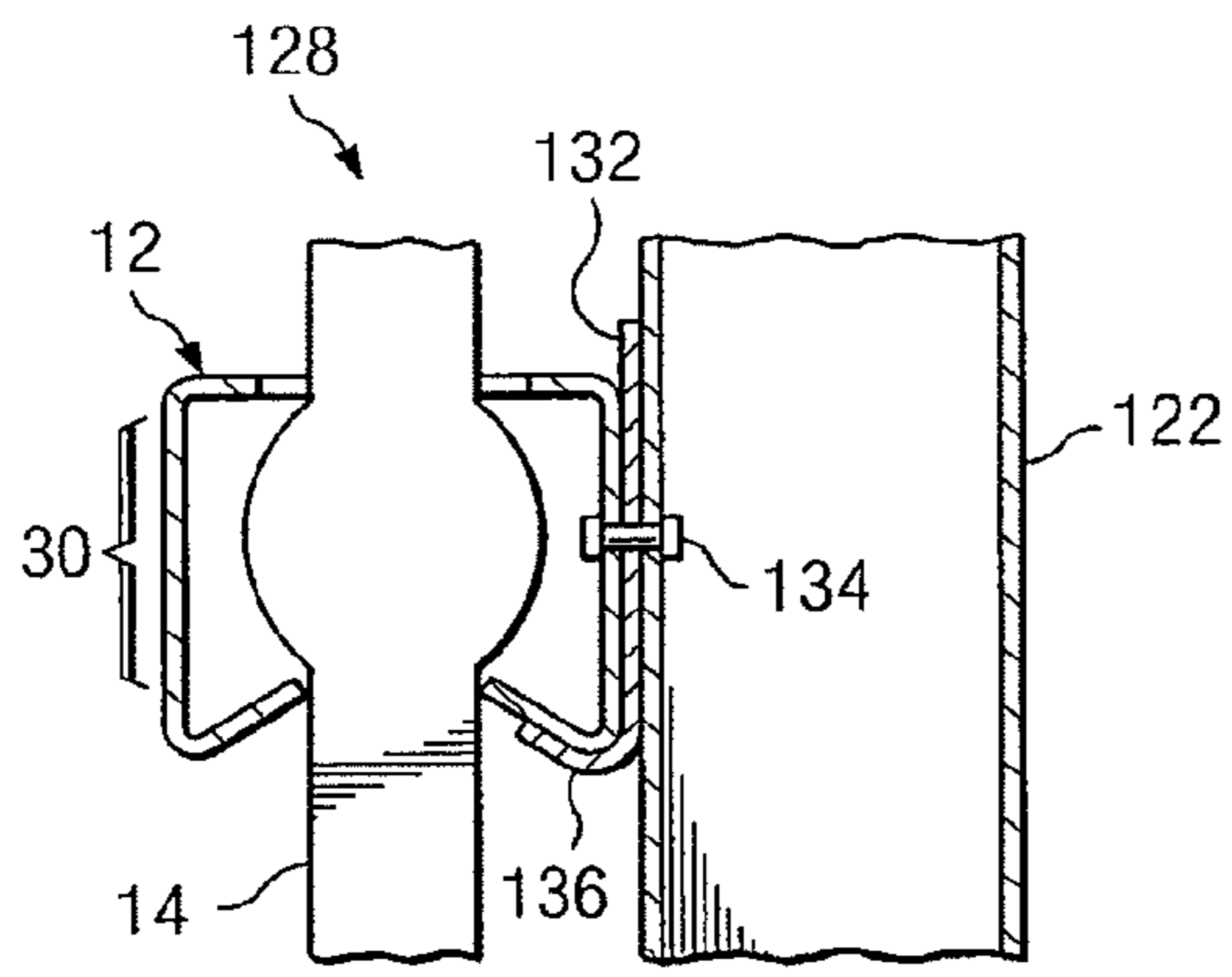
FIG. 11D
