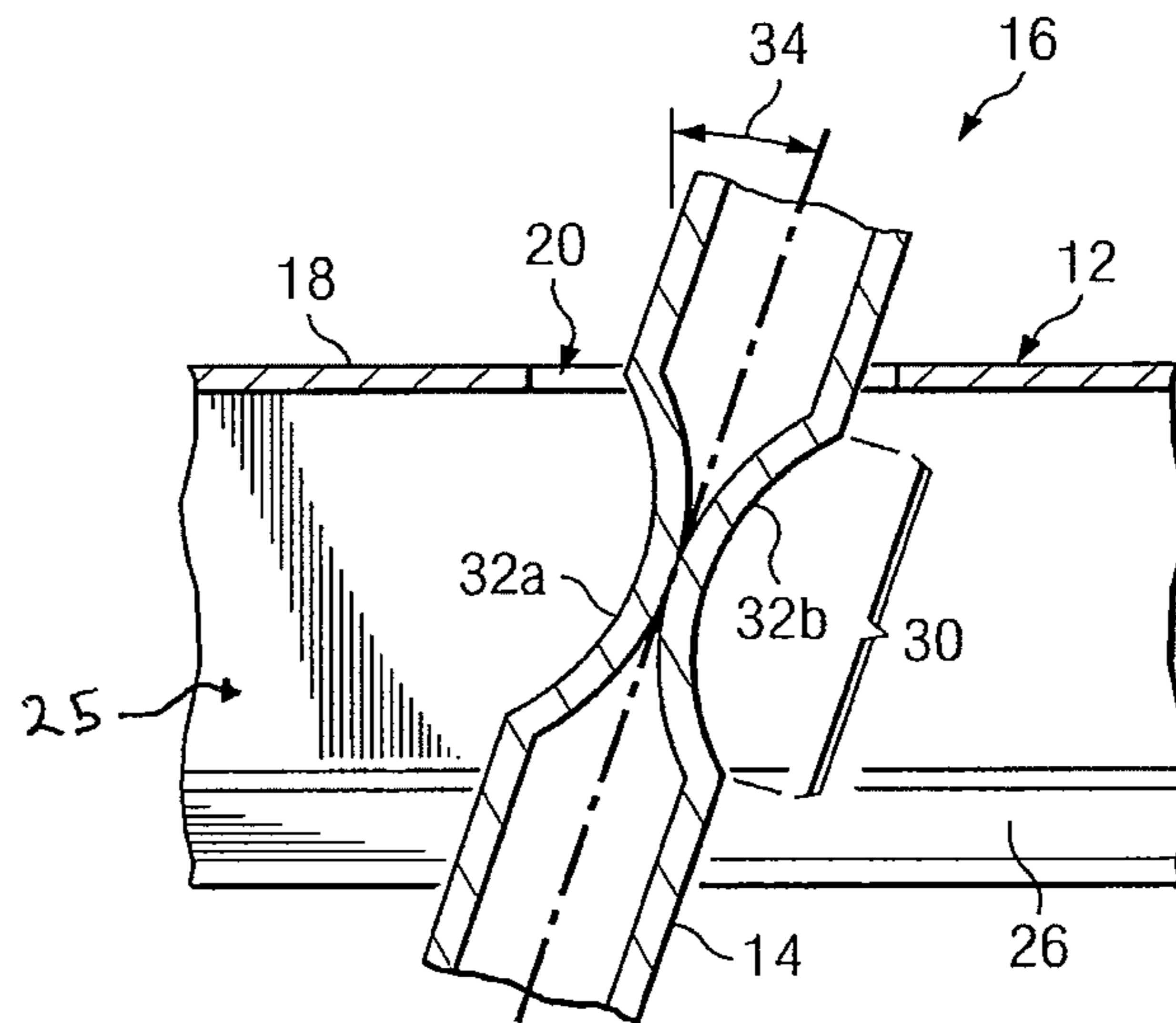
FIG. 2D
