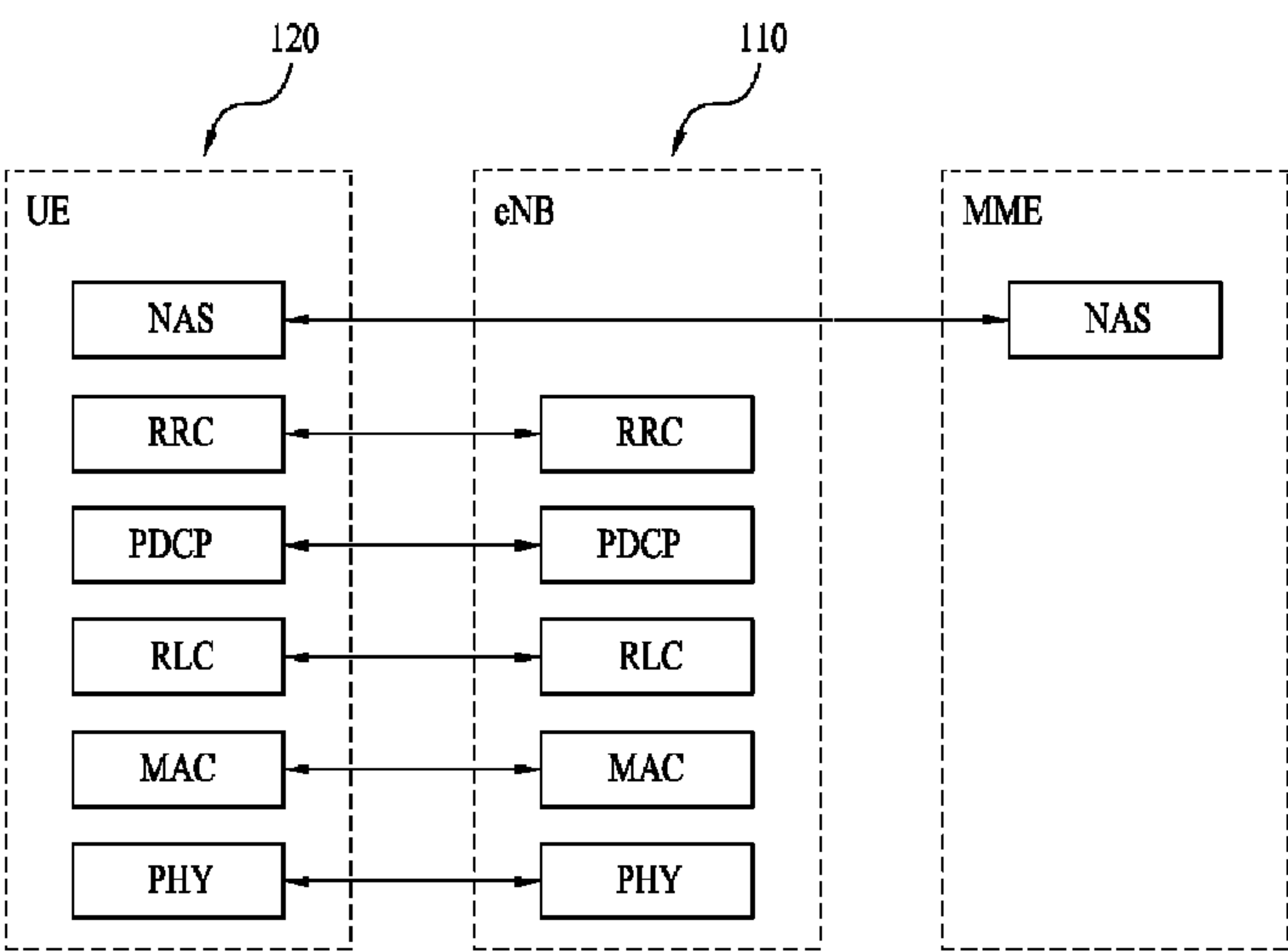
(a) Control-plane protocol stack
