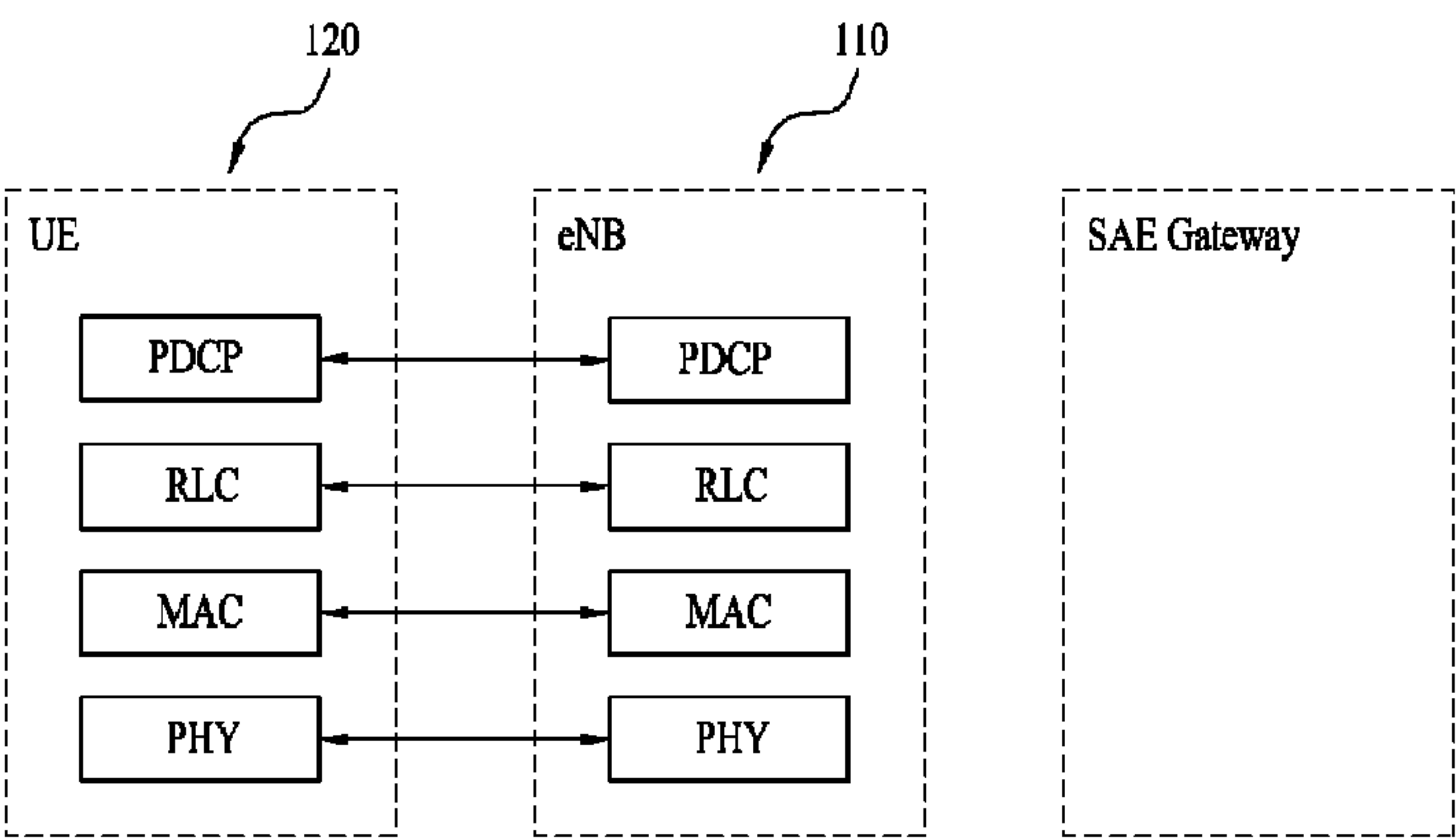
(b) User-plane protocol stack
