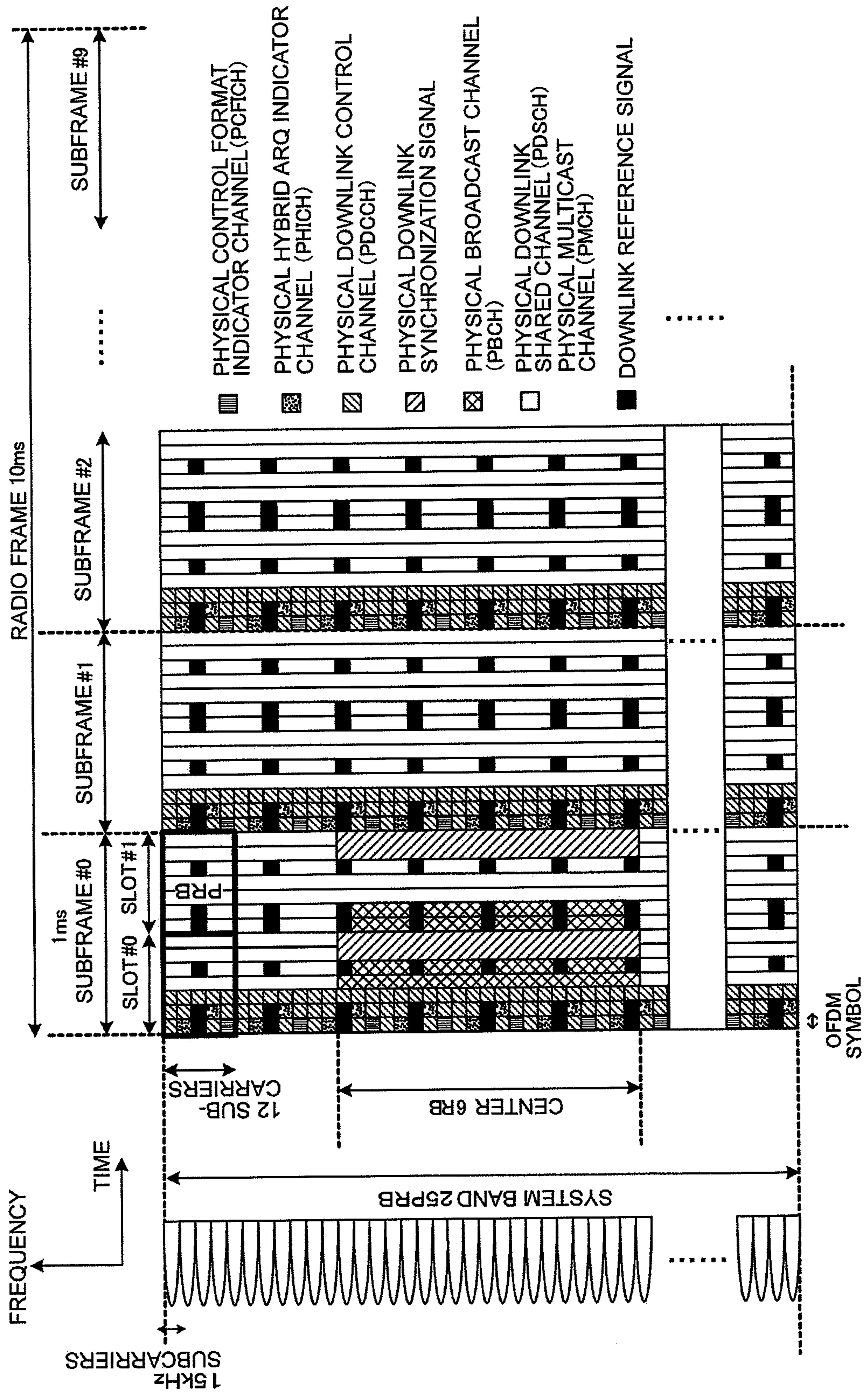
FIG. 3 PRIOR ART
