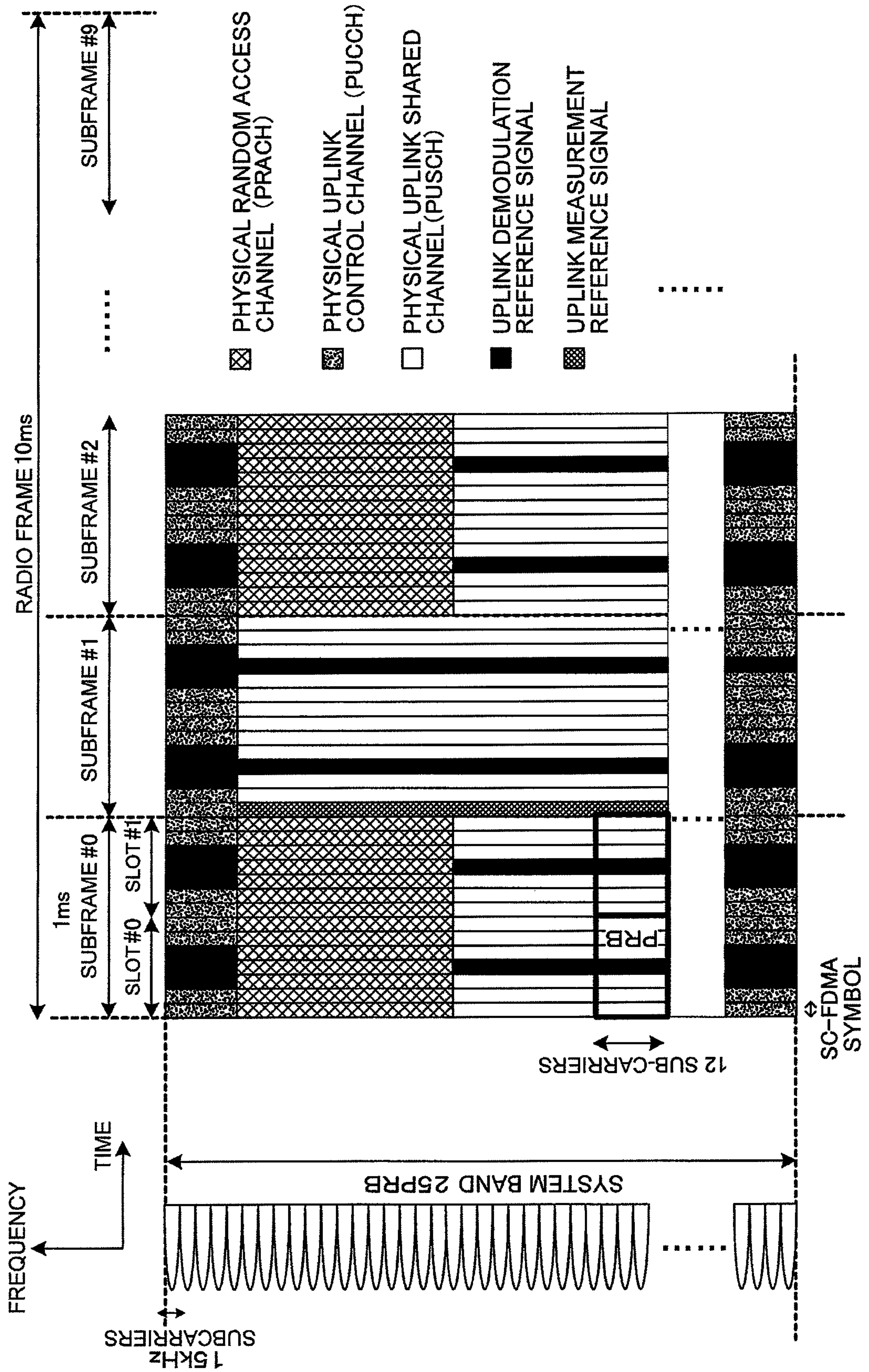
FIG. 4 PRIOR ART
