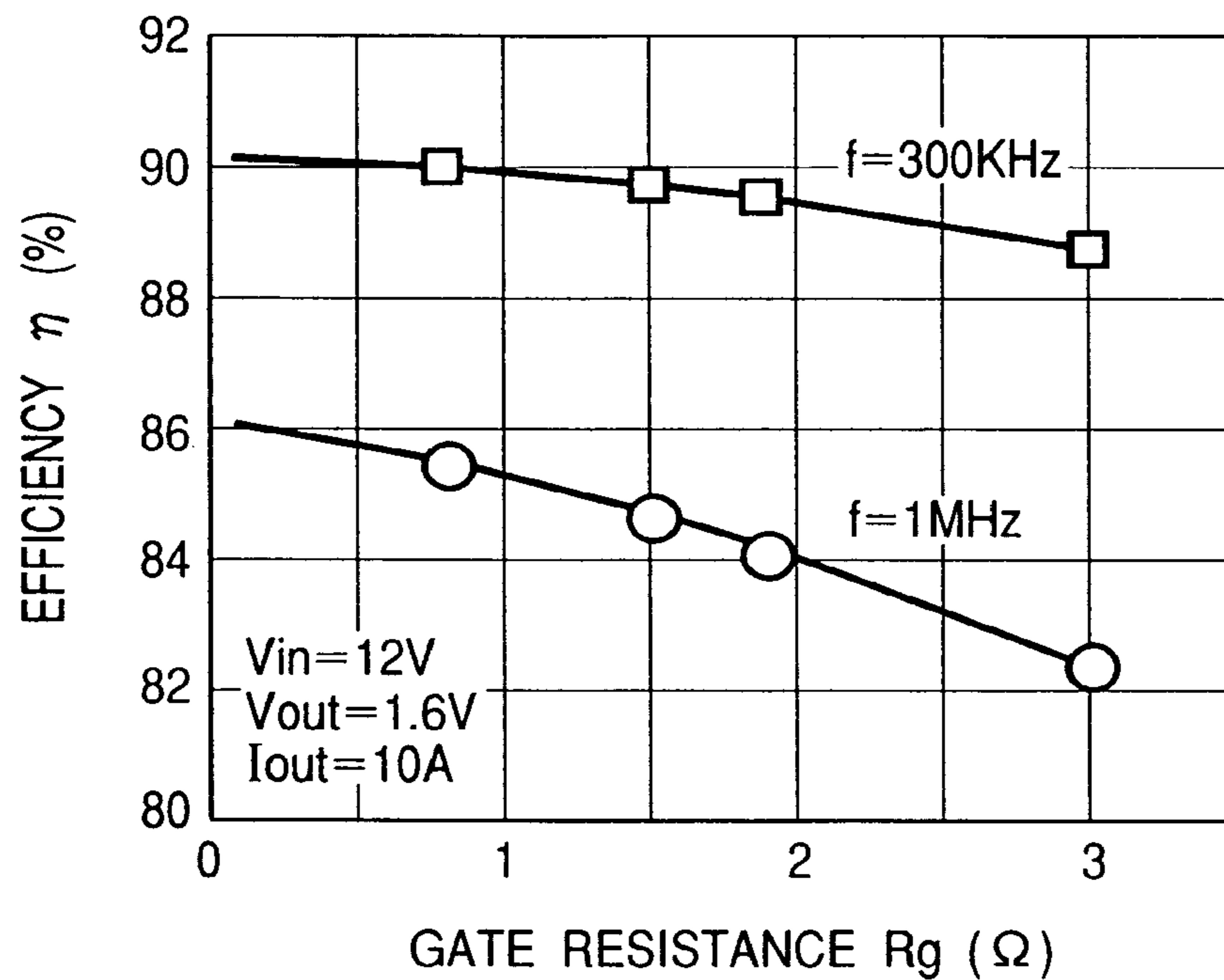
RELATION BETWEEN GATE RESISTANCE AND EFFICIENCY
