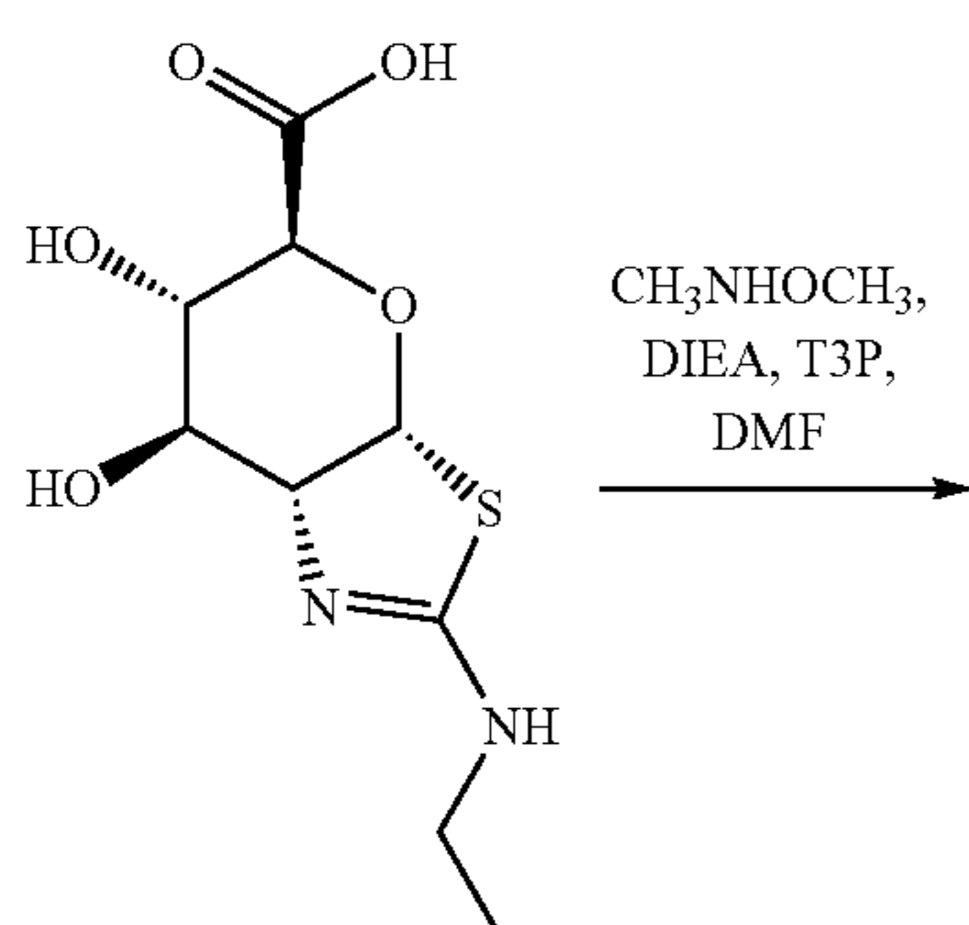
Scheme 4: Reaction sequence for compounds of sub-formula (IC)
