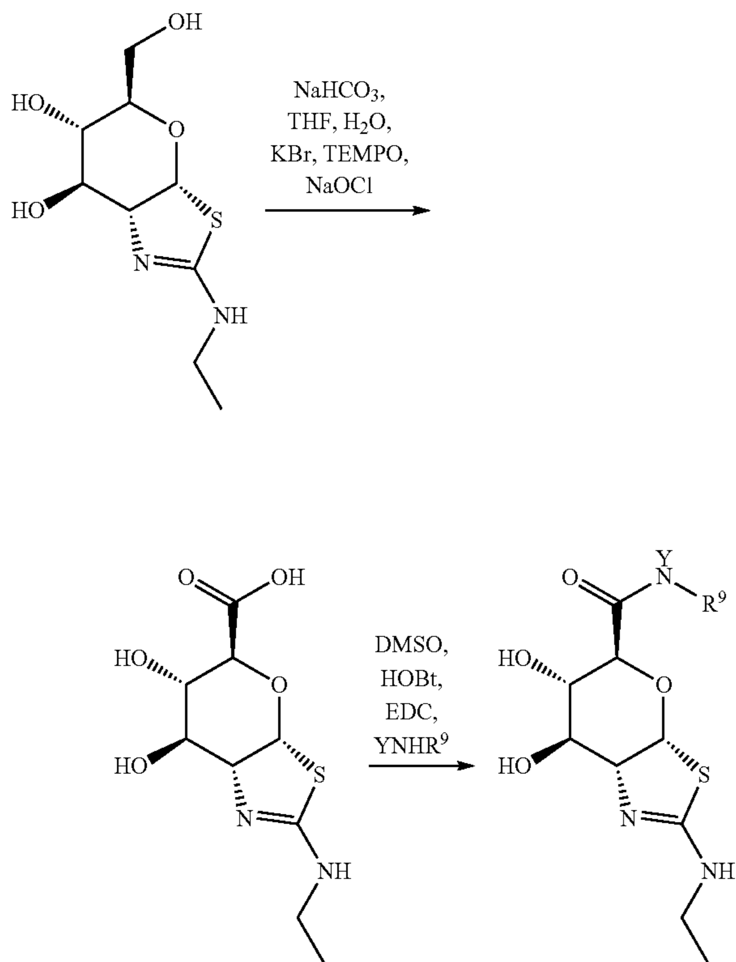
Scheme 3: Reaction sequence for compounds of sub-formula (IB-1)
