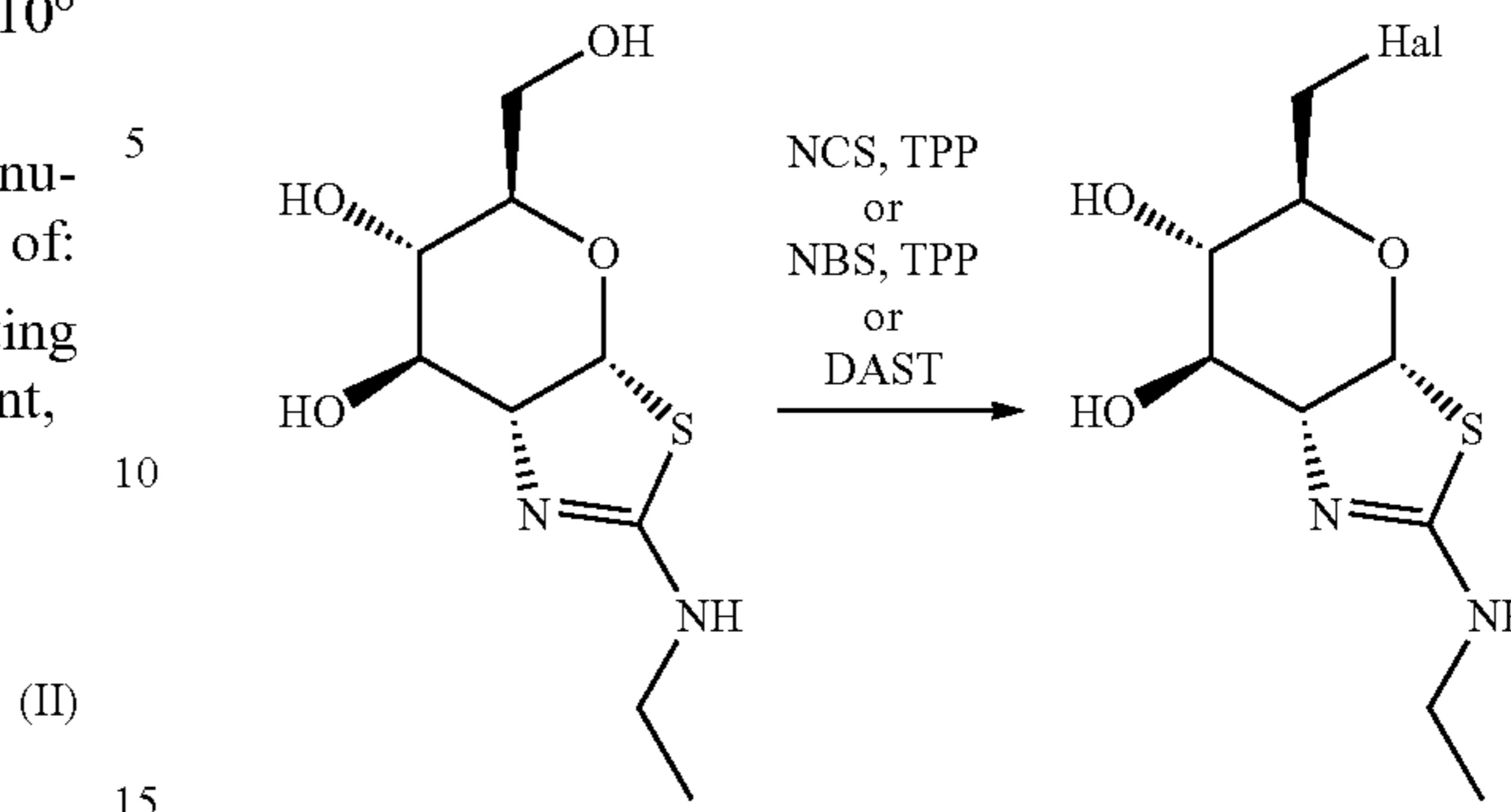
Scheme 1: Reaction sequence for compounds of sub-formula (IA-1)
