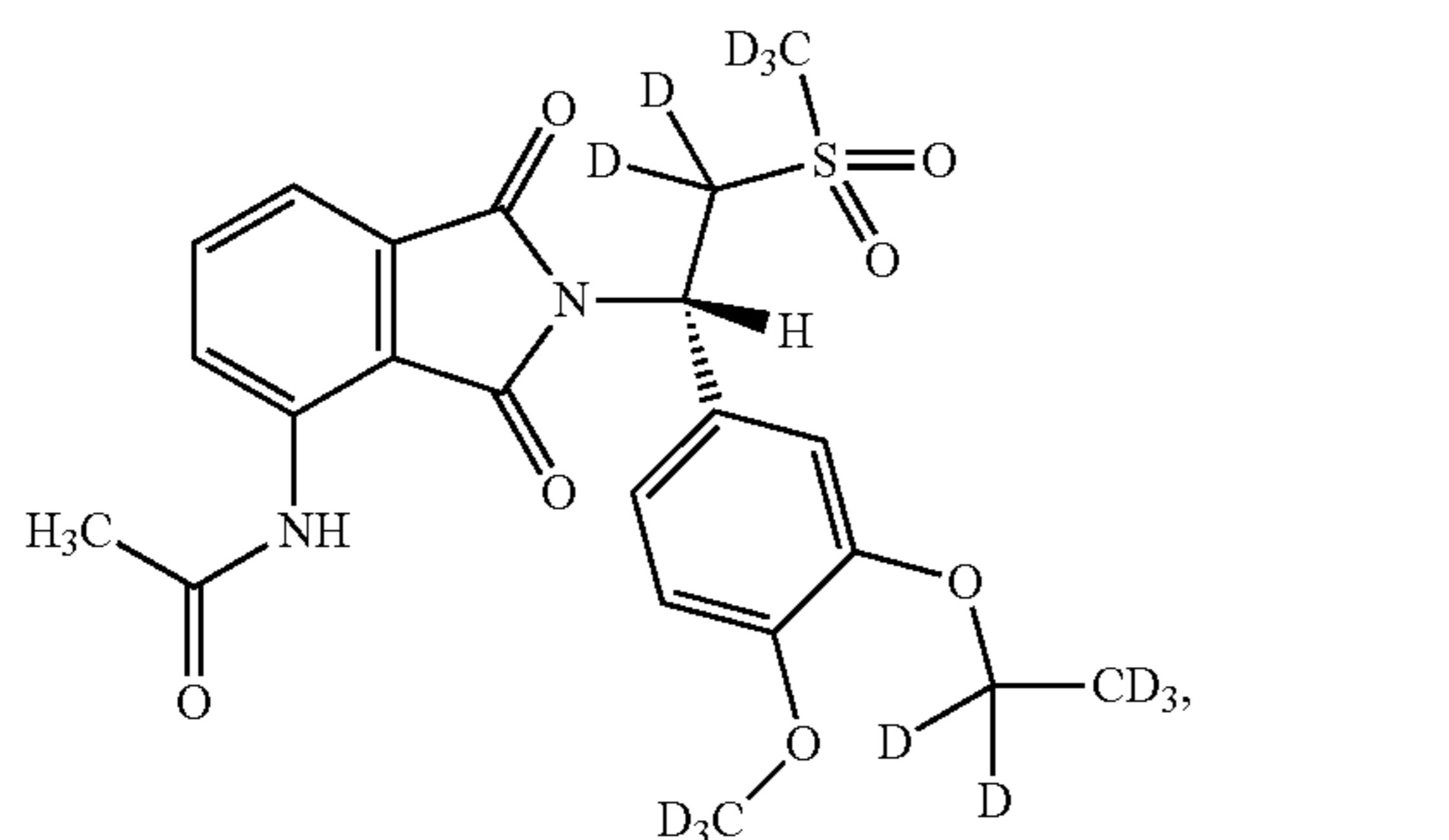
Compound 116a
