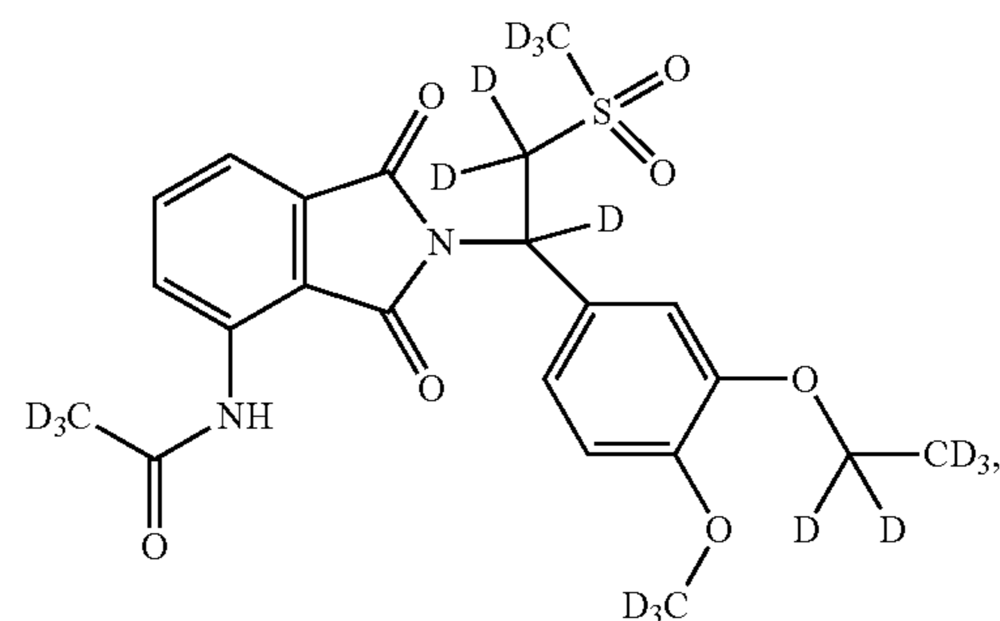
Compound 101
