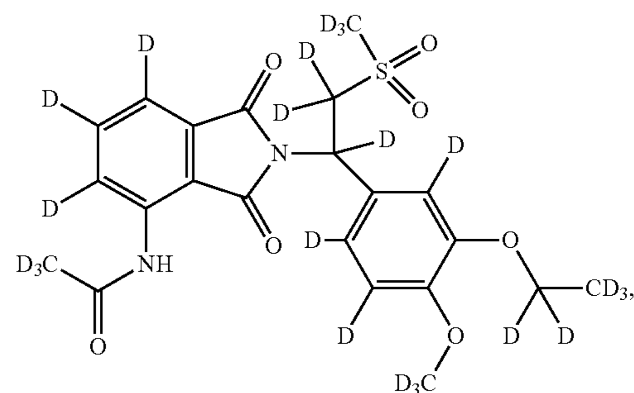
Compound 100
