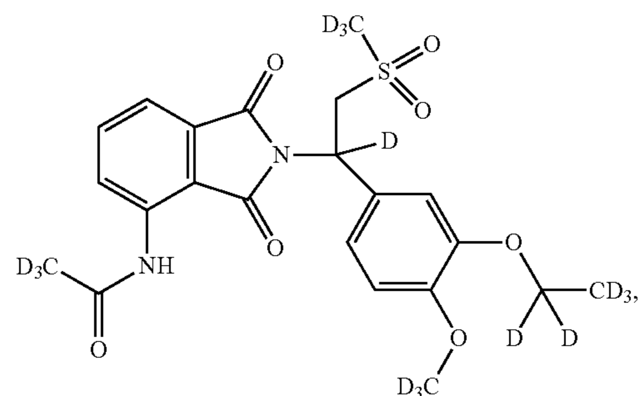
Compound 102
