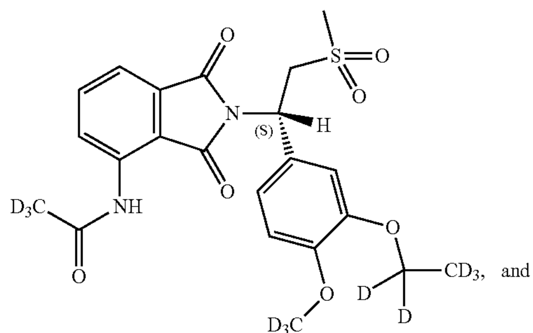
Compound 116a
