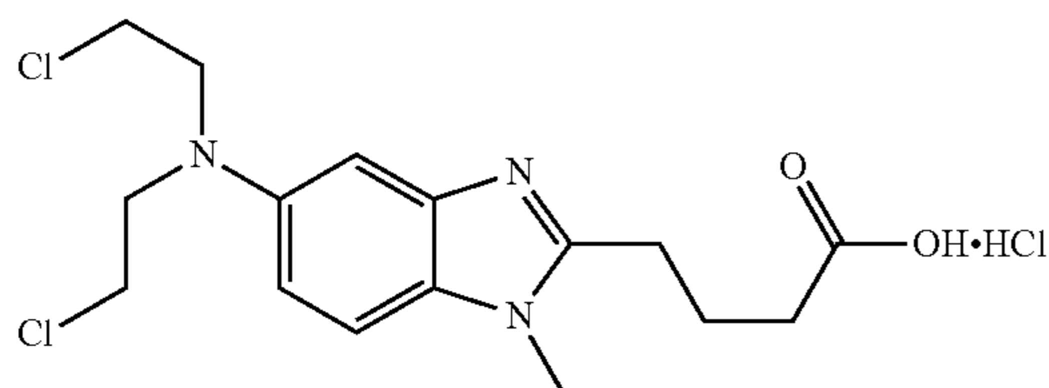
Bendamustine Hydrochloride
