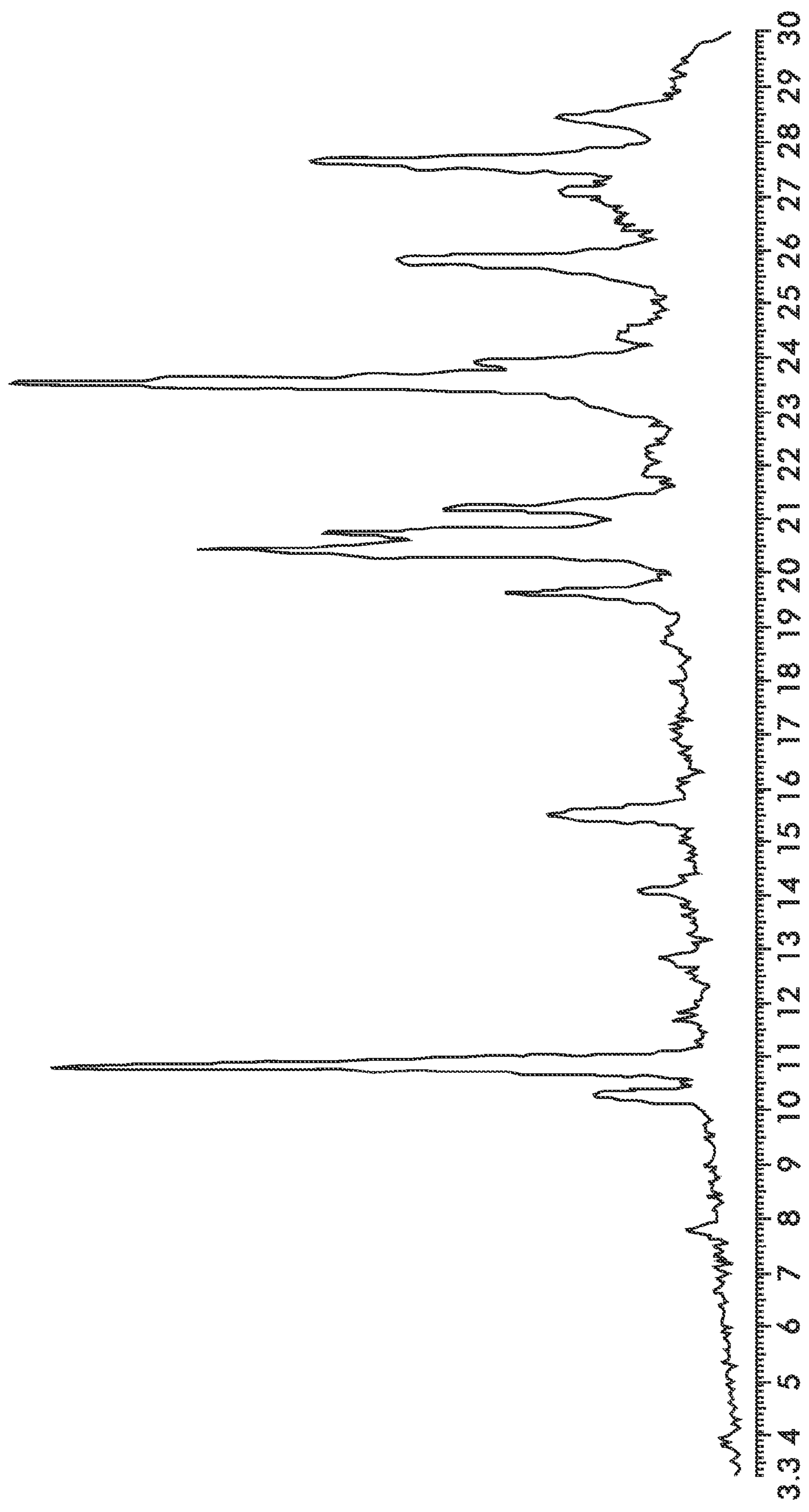
2 - Theta - Scale
