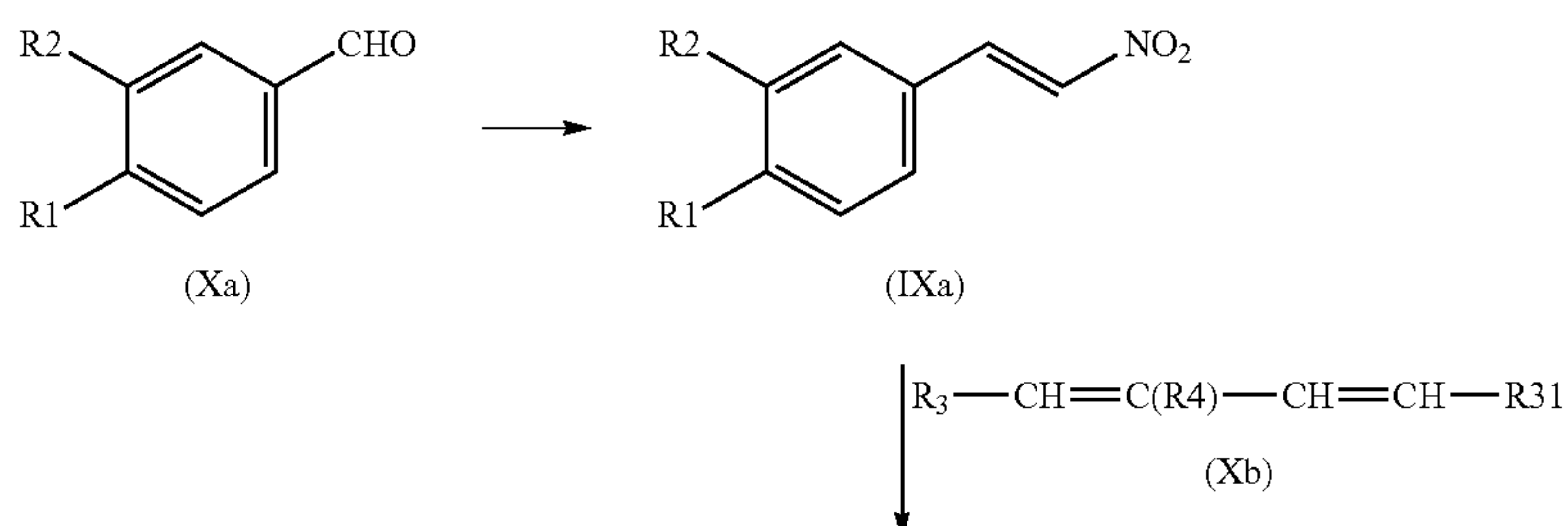
Reaction scheme 5:
