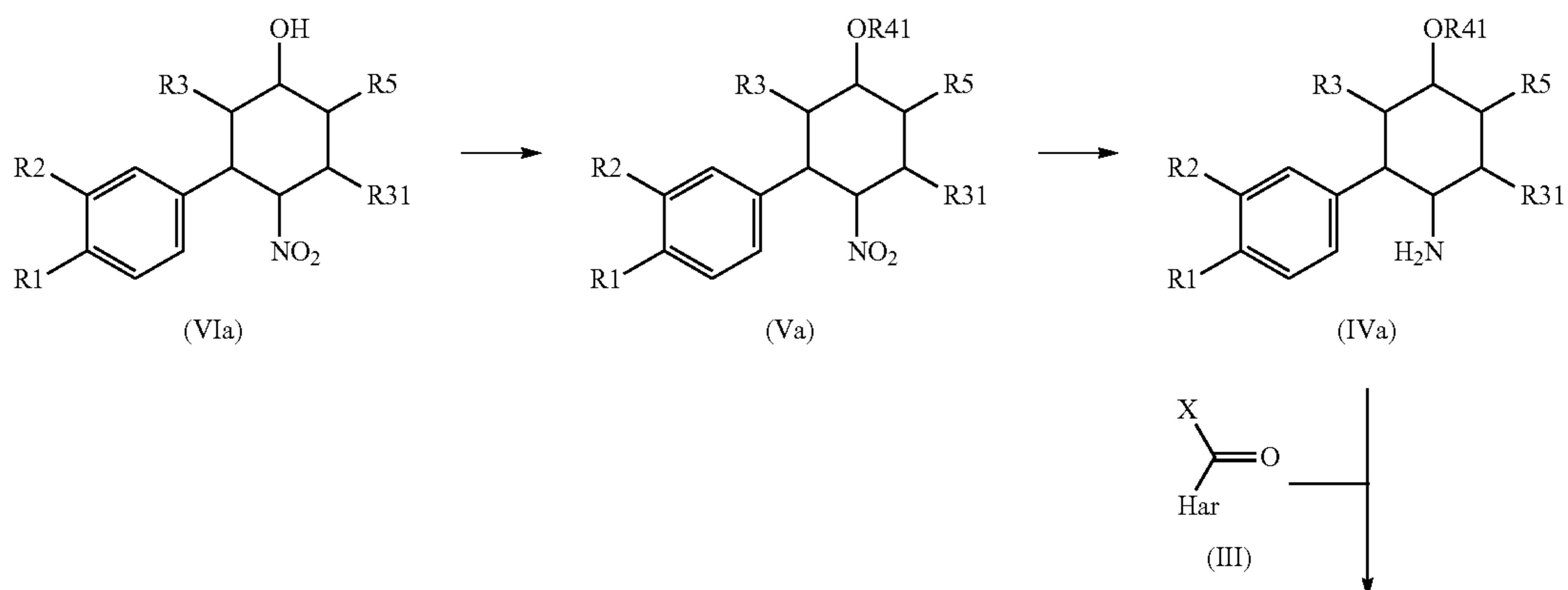
Reaction scheme 1:
