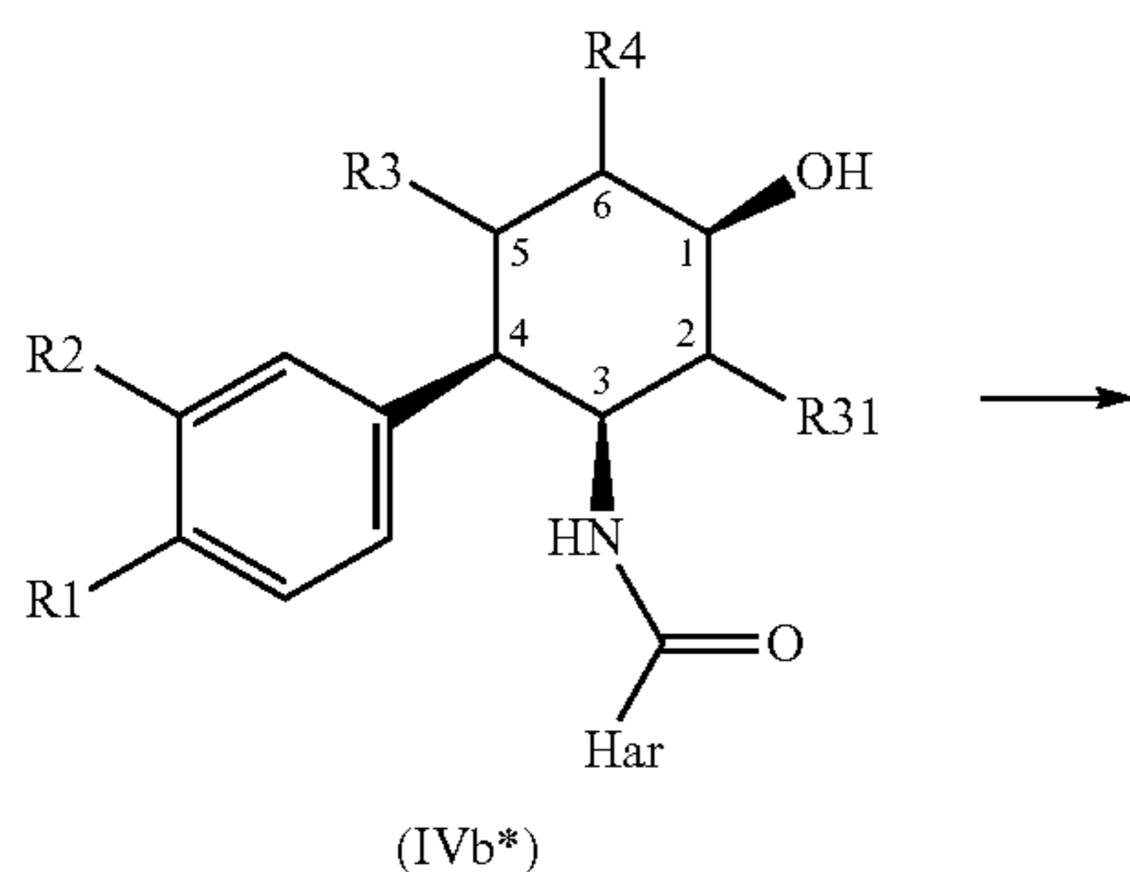
Reaction scheme 4:
