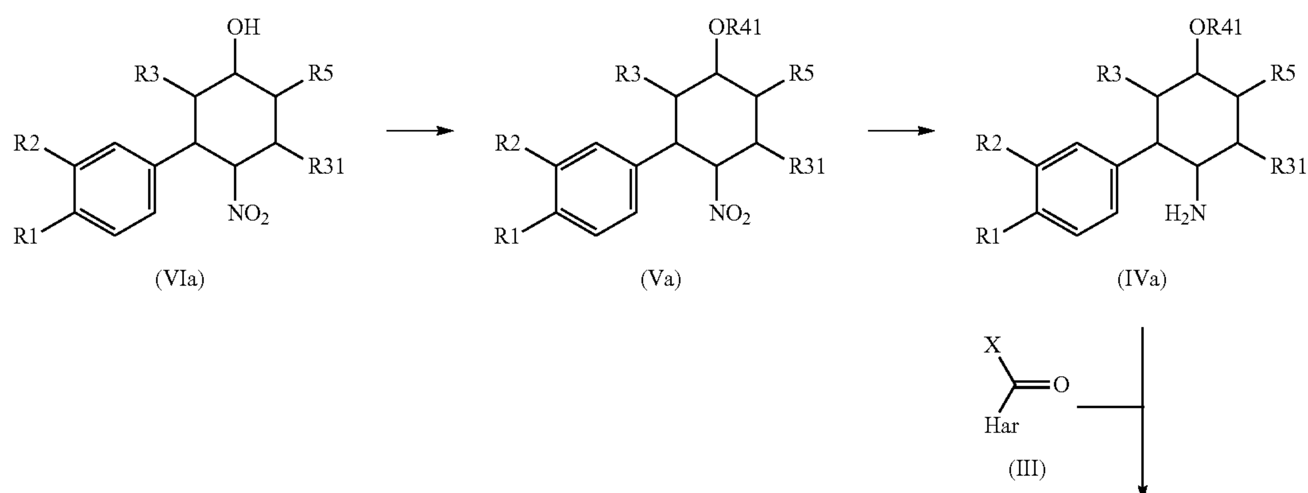
Reaction scheme 1:
