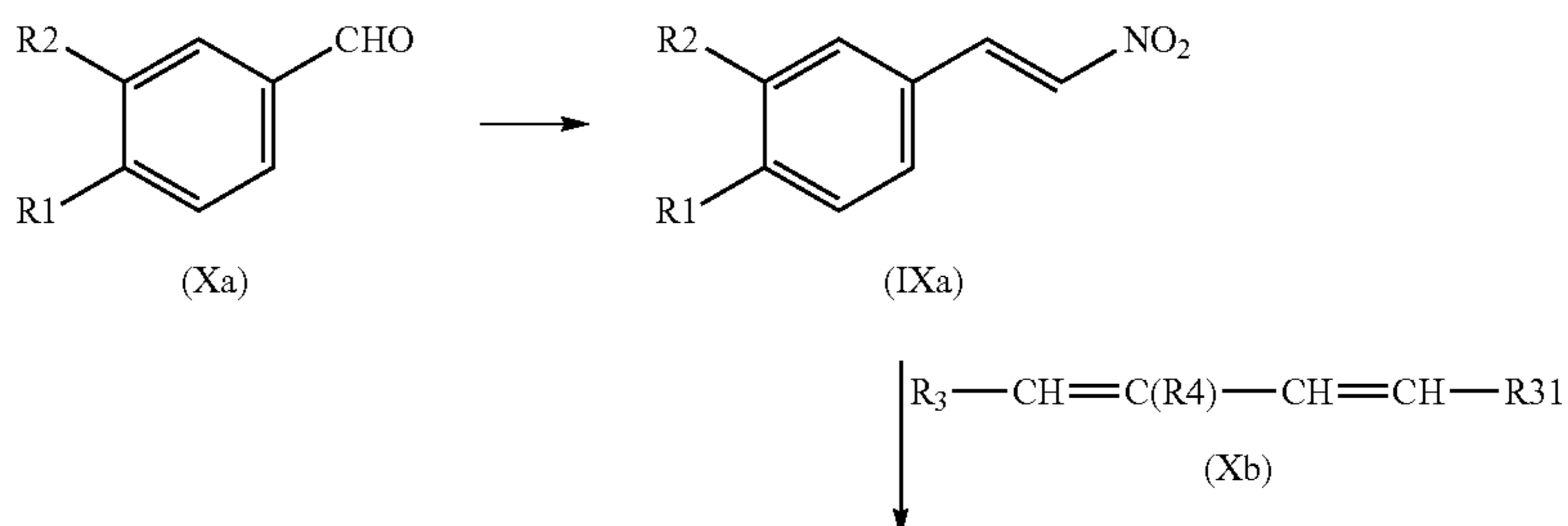
Reaction scheme 5:
