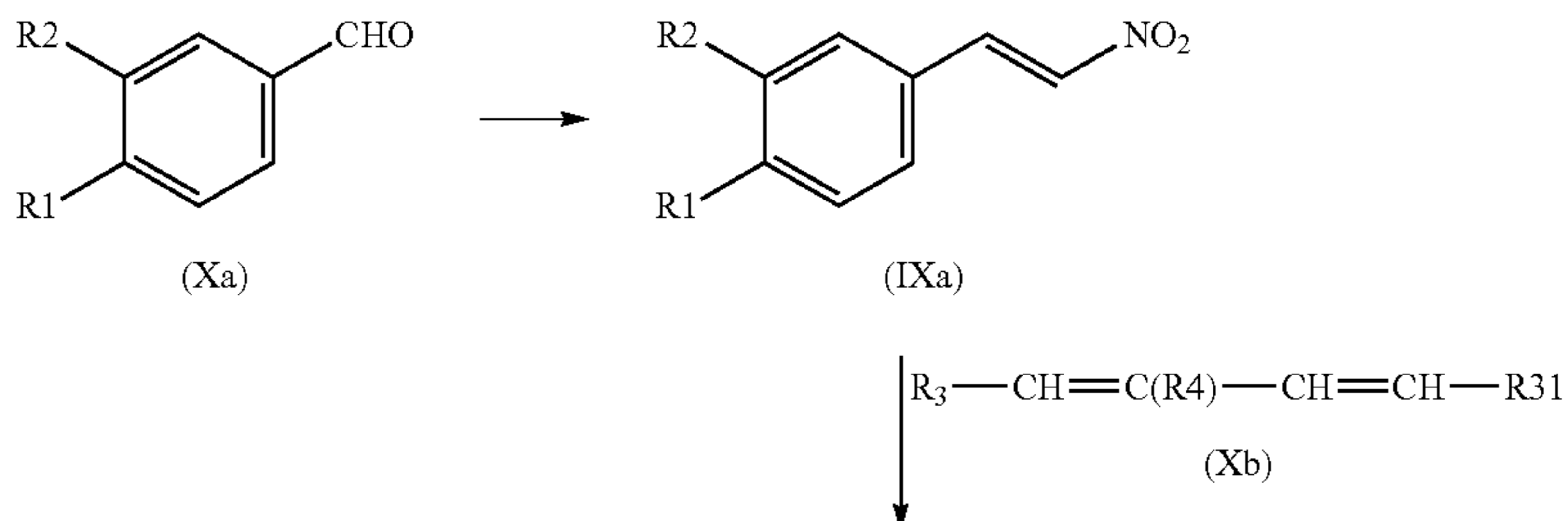
Reaction scheme 5:
