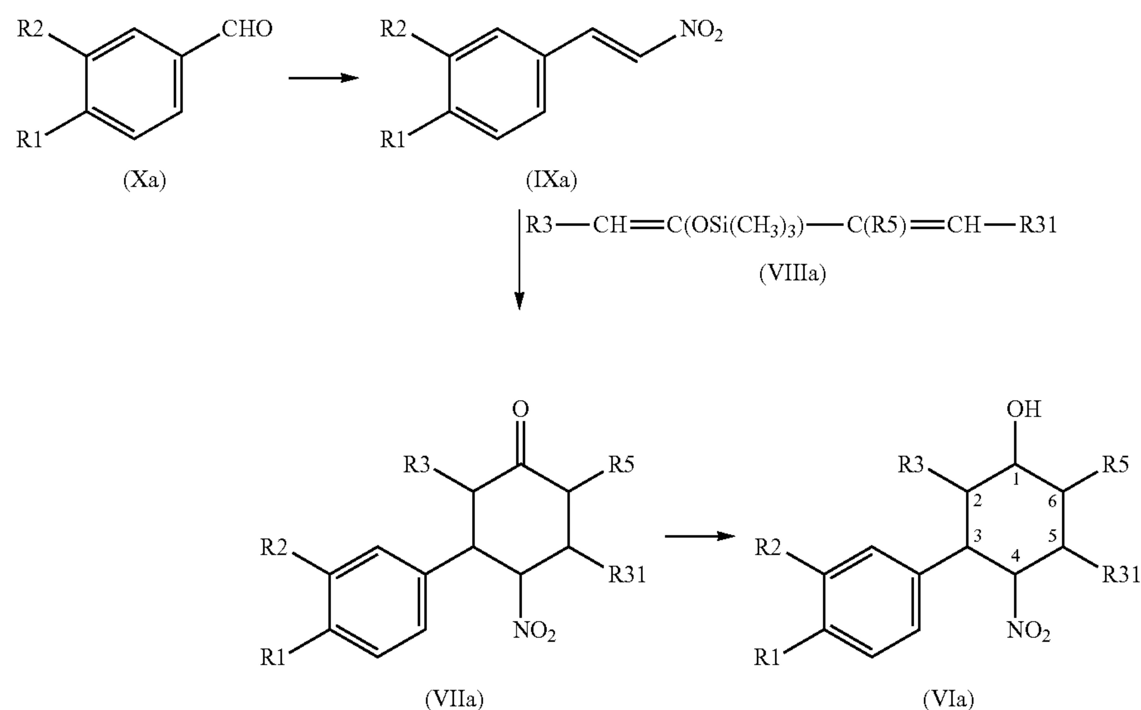
Reaction scheme 2:
