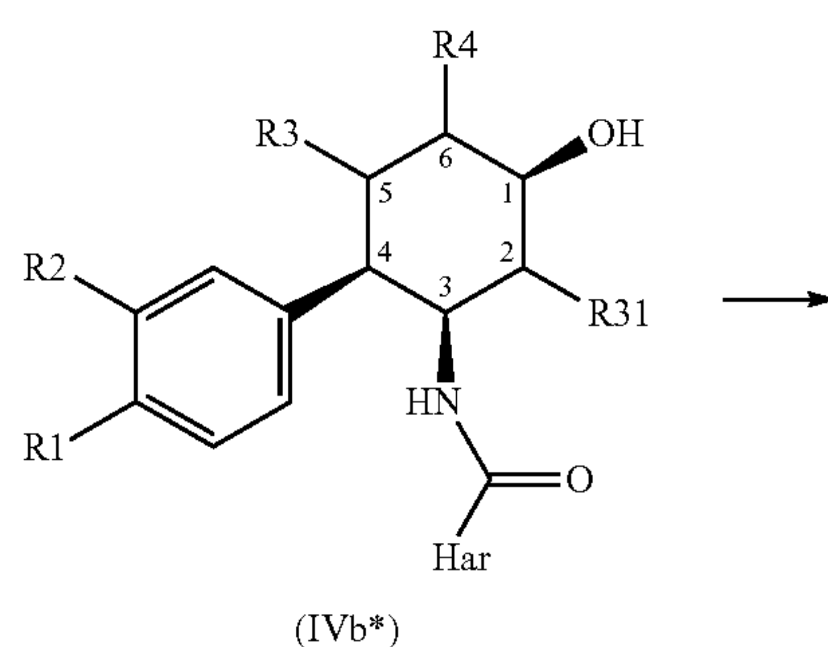
Reaction scheme 4:
