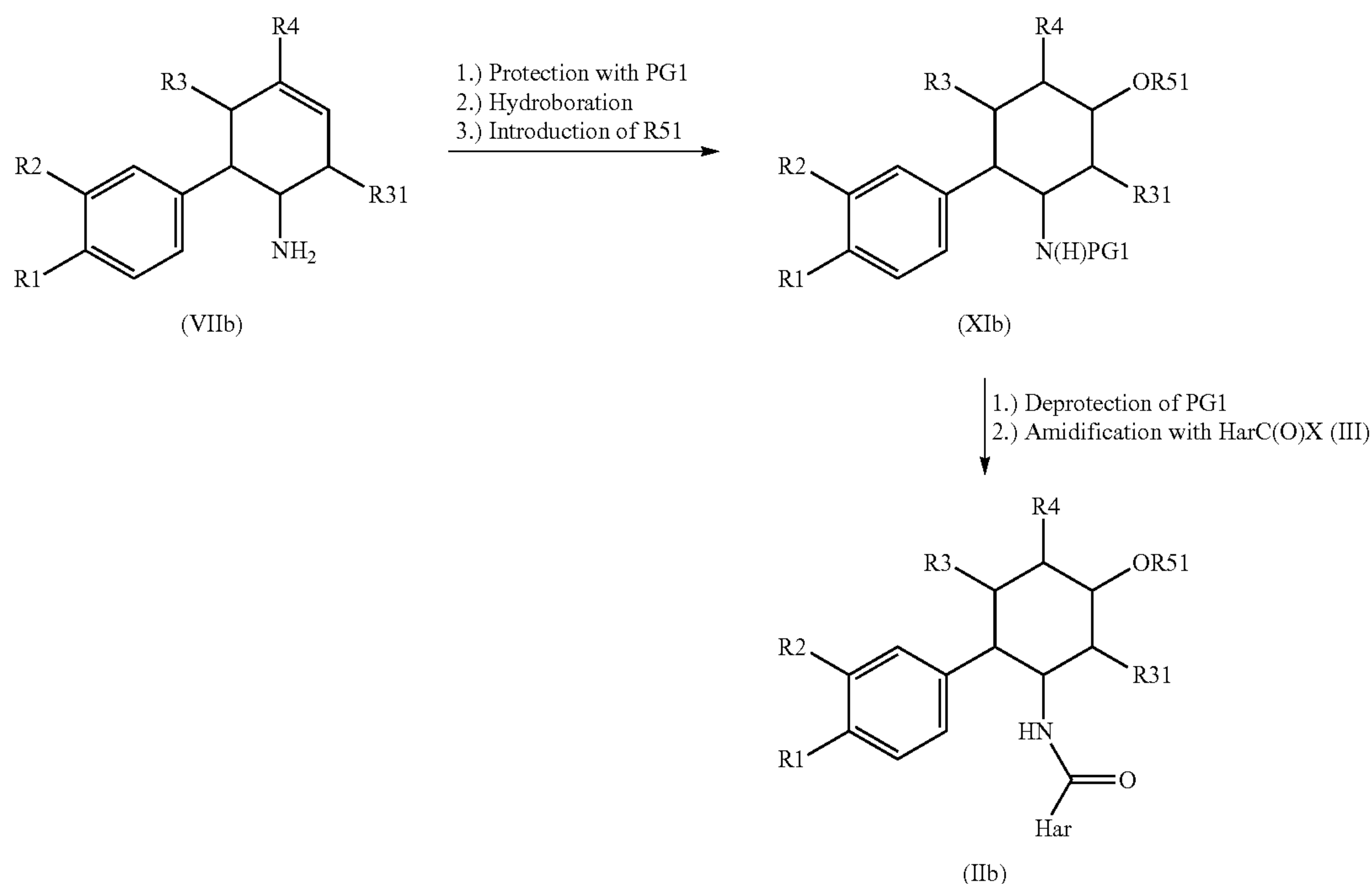
Reaction scheme 6:
