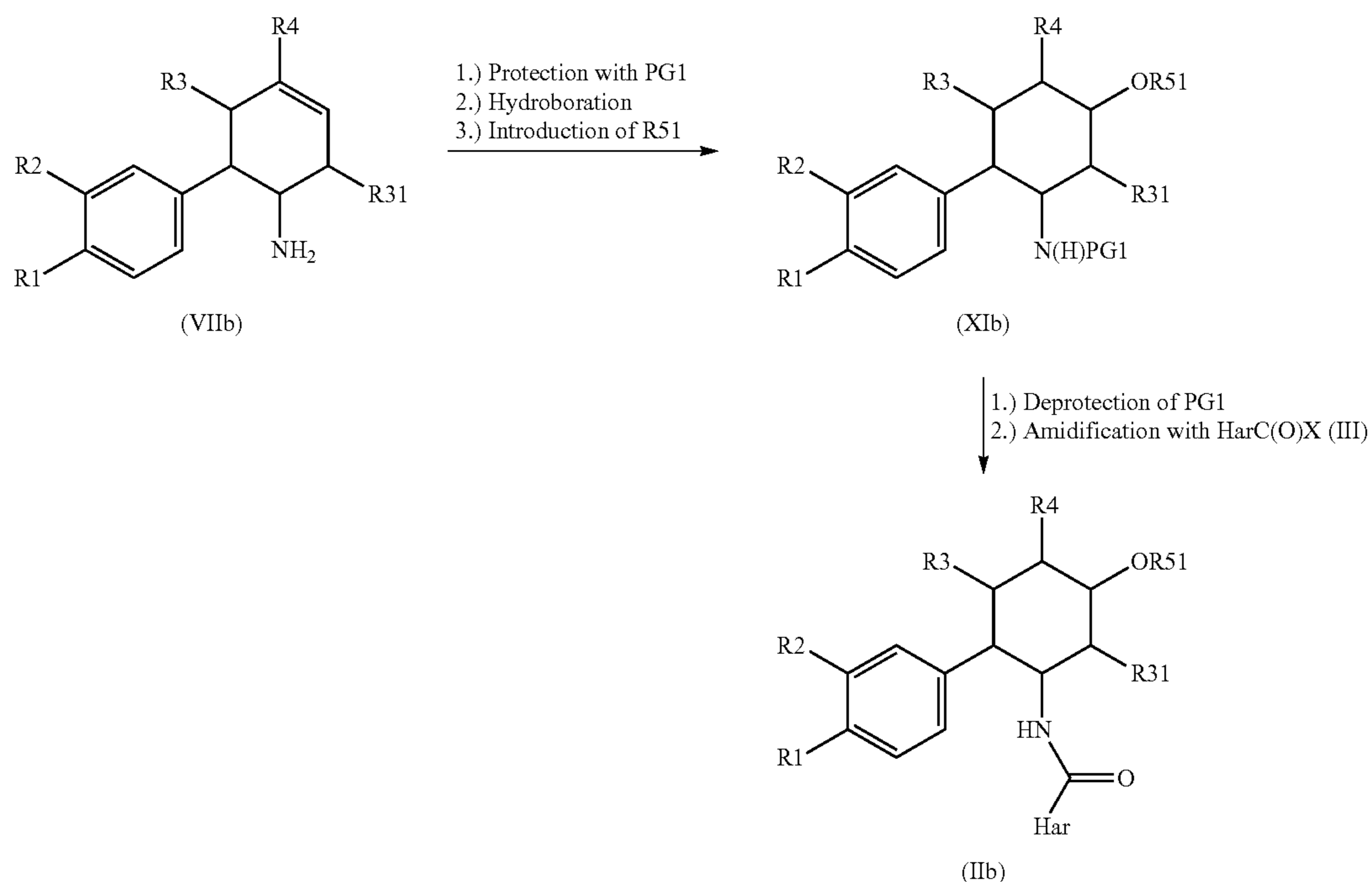
Reaction scheme 6:
