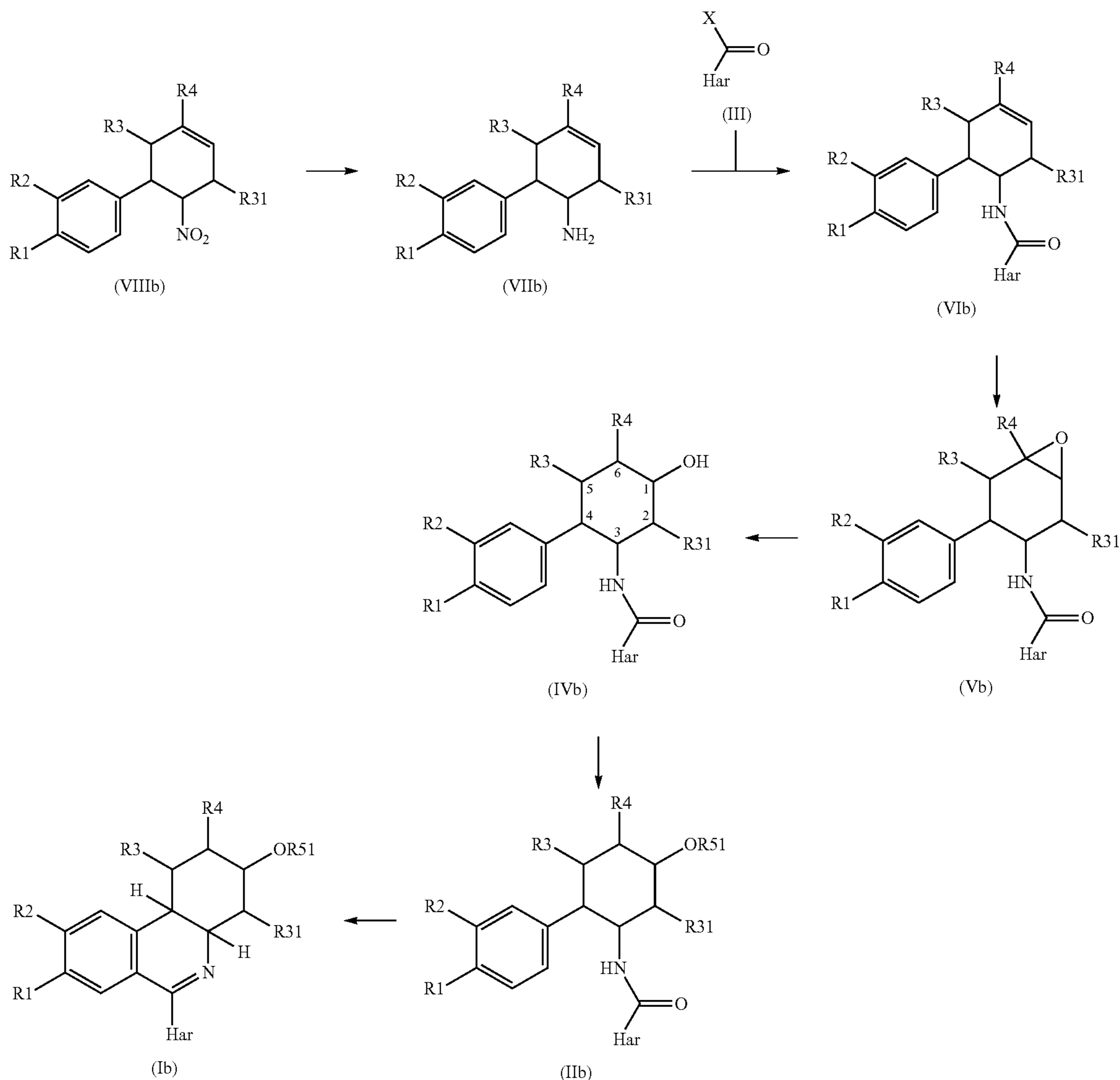
Reaction scheme 3:
