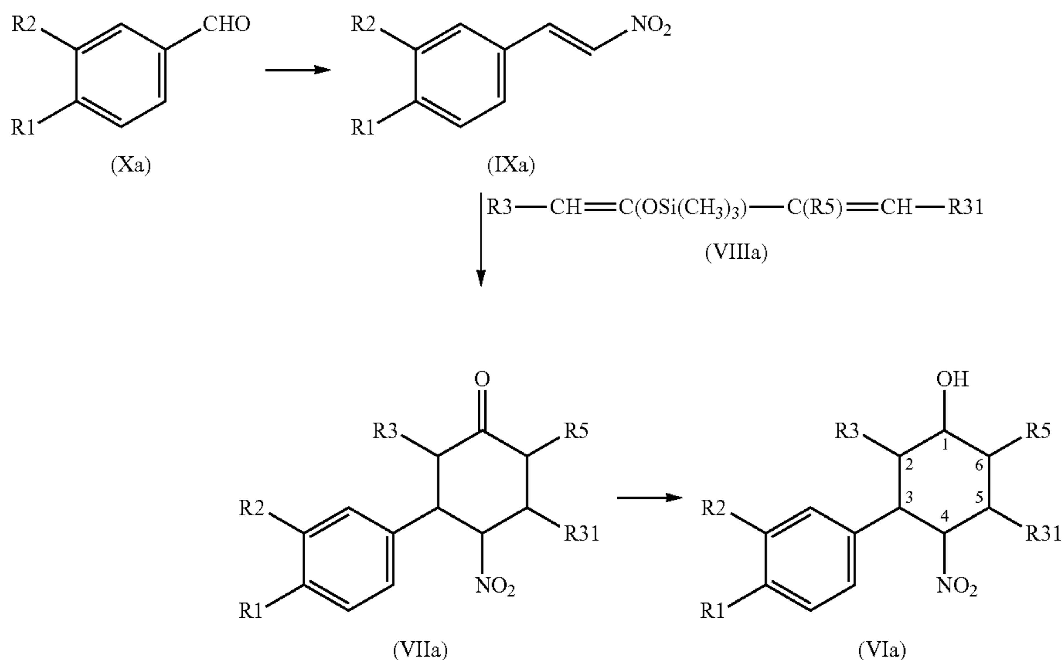
Reaction scheme 2:
