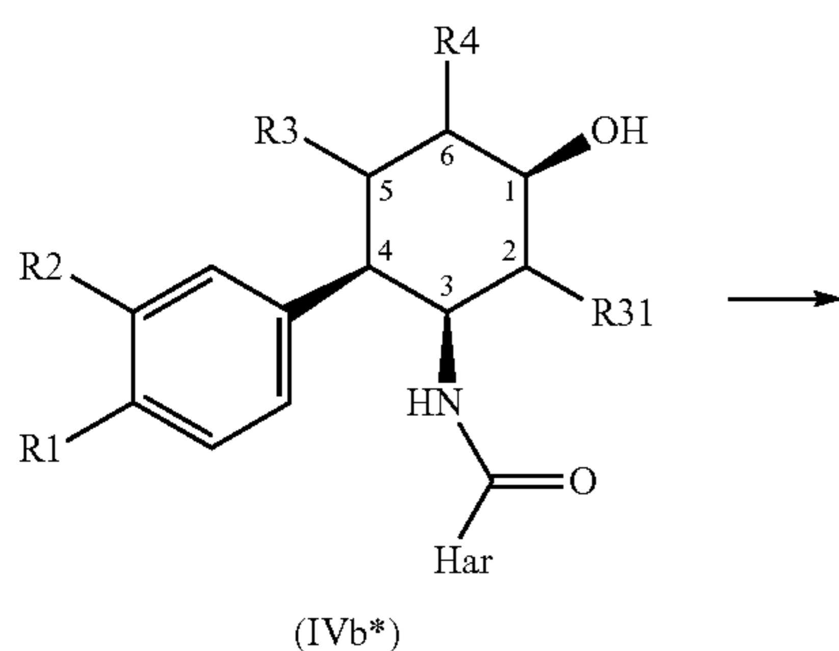
Reaction scheme 4:
