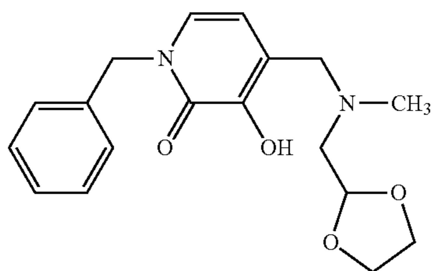
1-Benzyl-3-hydroxy-4-([(1,3]-dioxolan-2-ylmethylmethylamino)methyl)pyridin-2(1H)-one
