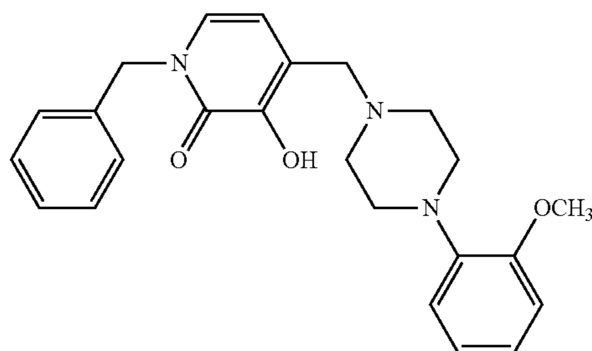
1-Benzyl-3-hydroxy-4-[4-(2-methoxyphenyl)piperazin-1-ylmethyl]pyridin-2(1H)-one
