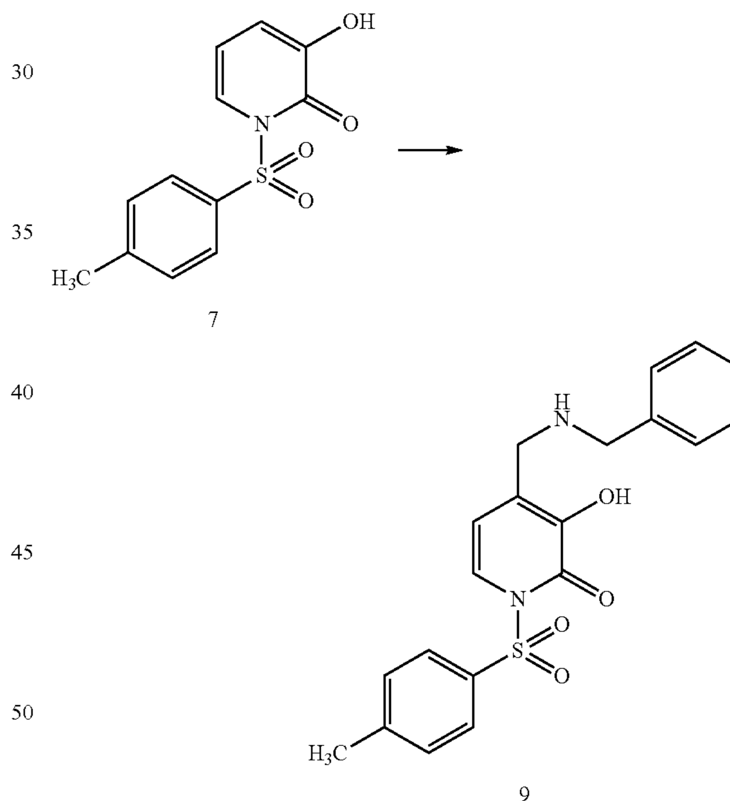
Scheme IV
