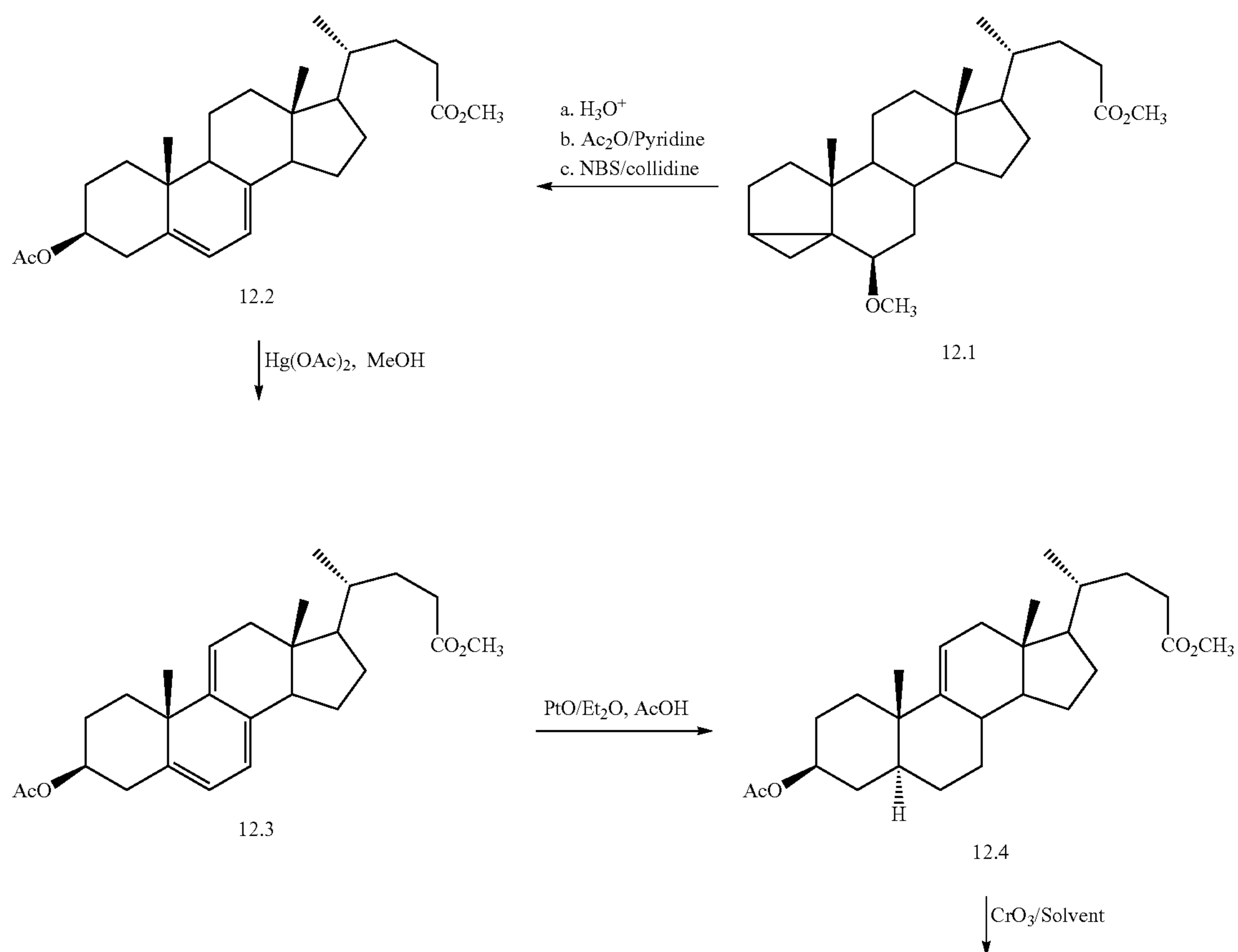
Scheme 12. Triene formation and allylic oxidation
