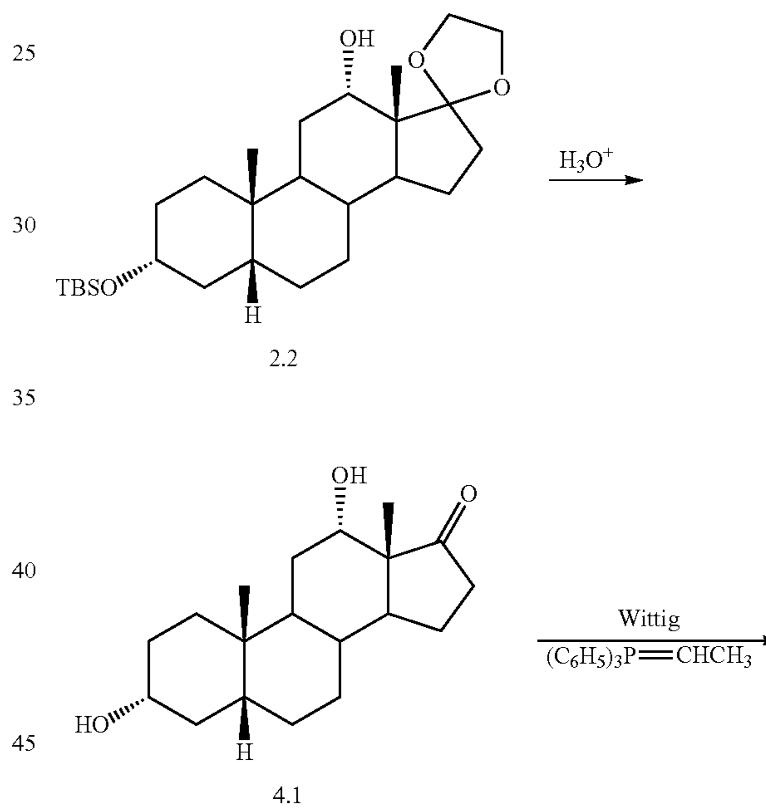
Scheme 4. Deprotection and Wittig Reaction
