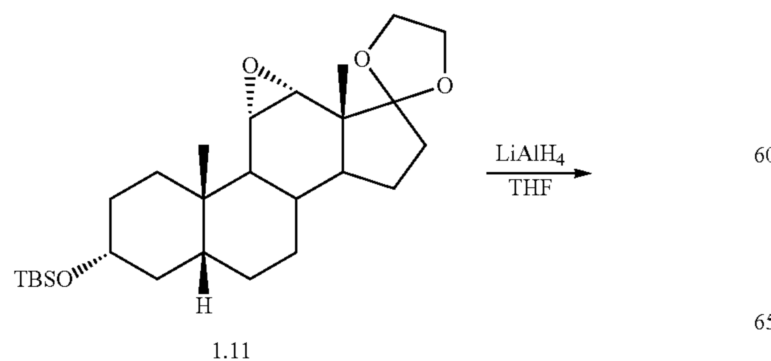
Scheme 3. Stereoselective Reduction of C 11 -C 12 epoxide.
