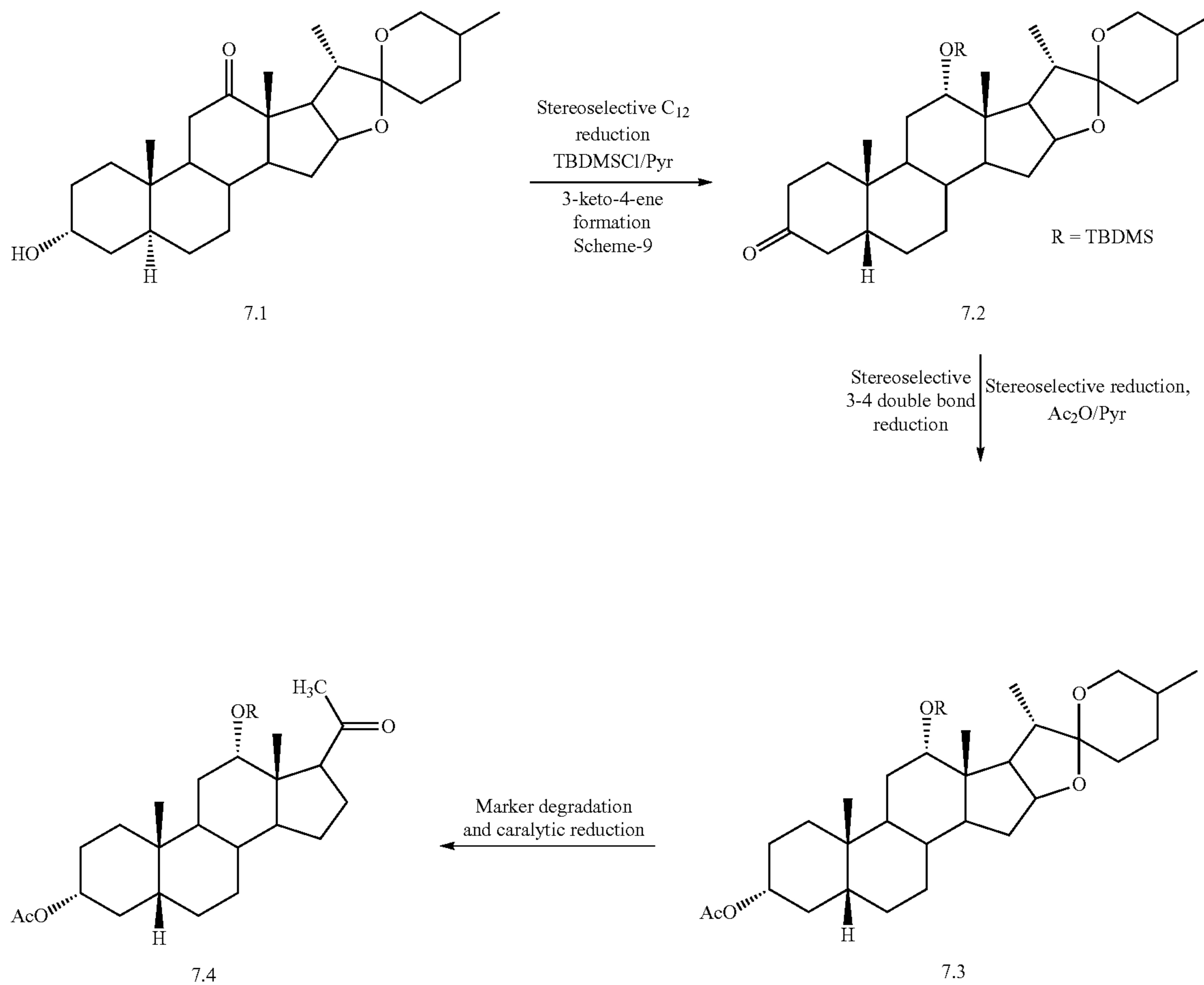
Scheme 7. C 12 -hydroxyl group introduction, AB ring modification and side chain cleavage
