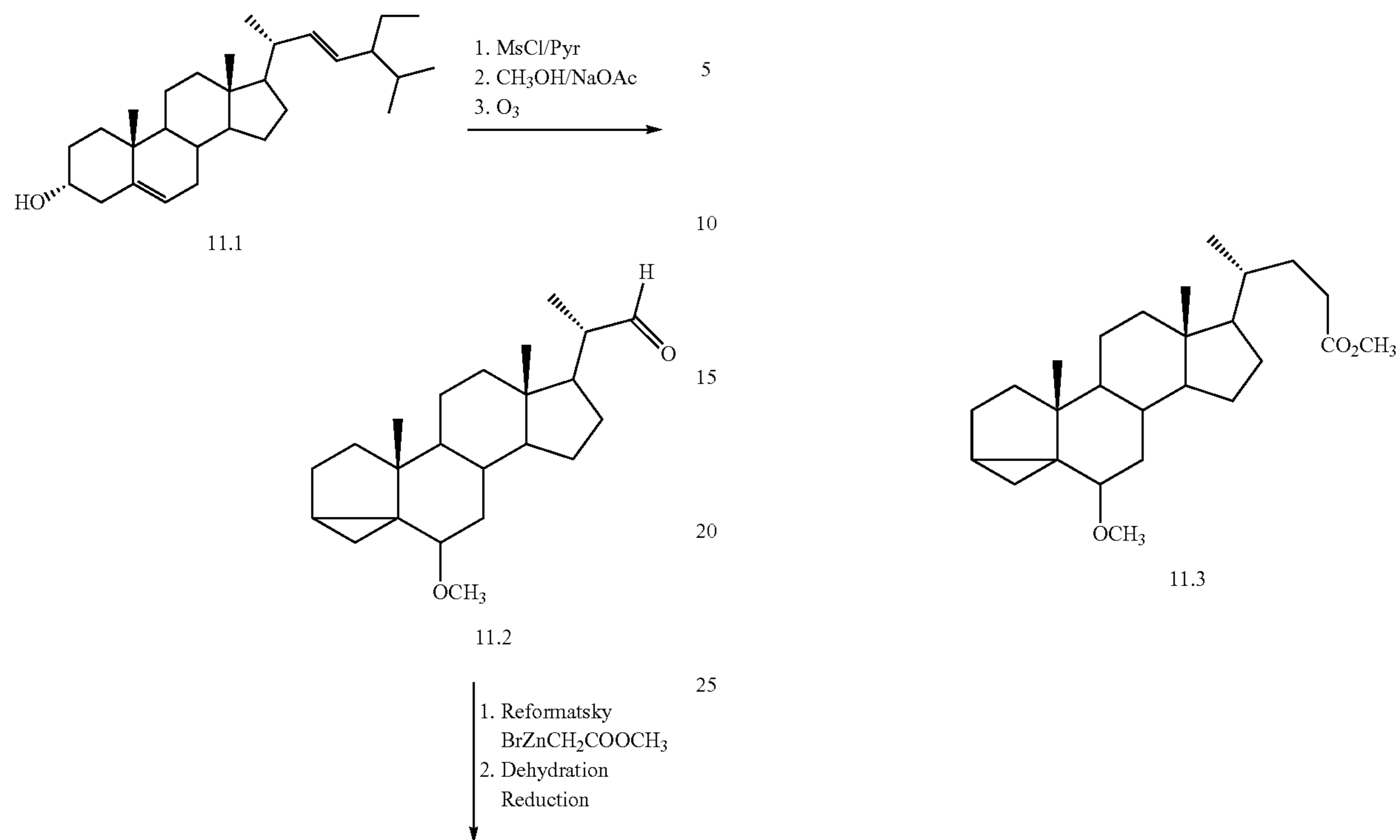
Scheme 11. Ozonolysis of i-steroid and side chain reduction
