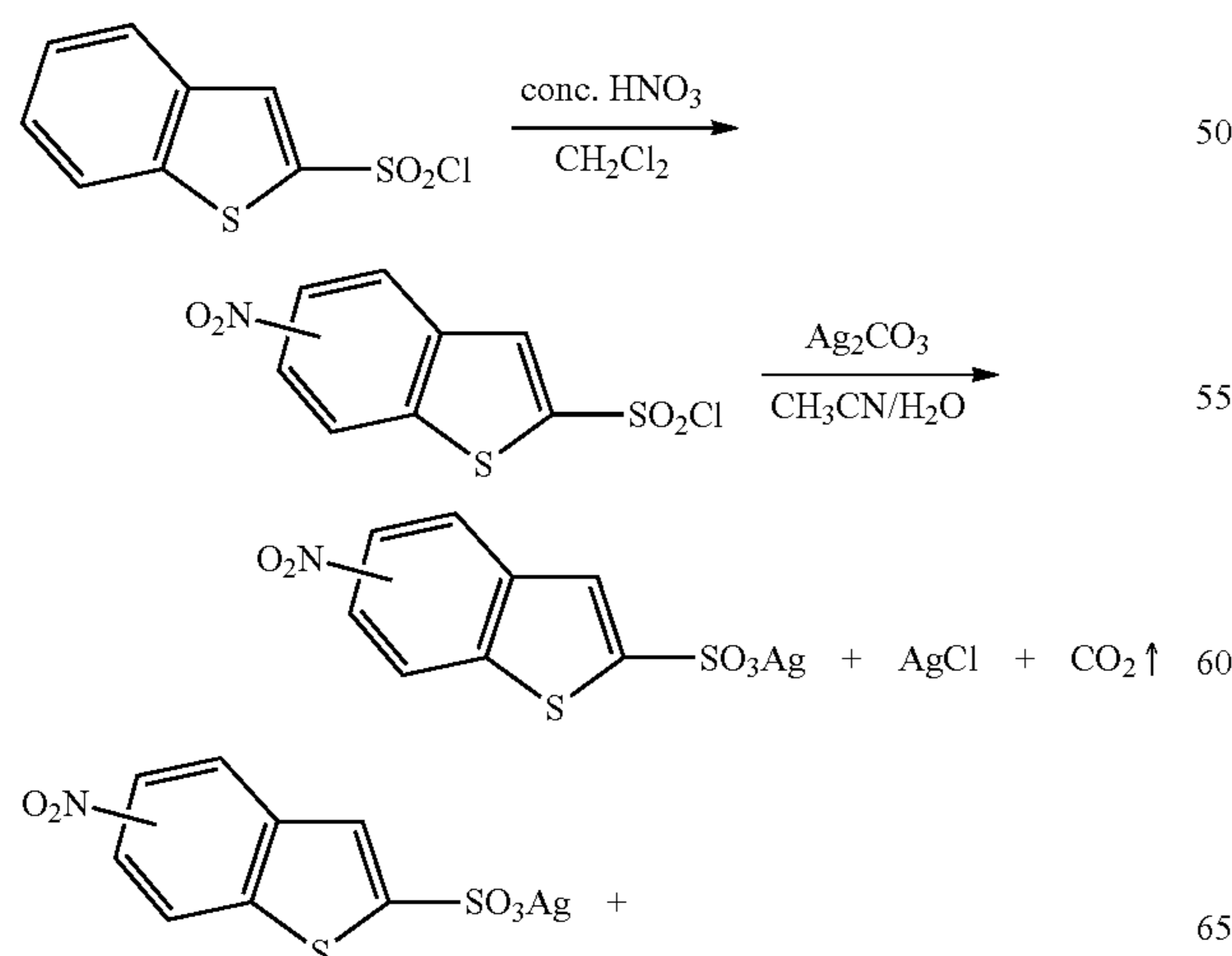
Scheme 1. Synthesis of fluorine-free fused-ring heteroaromatic PAGs.
